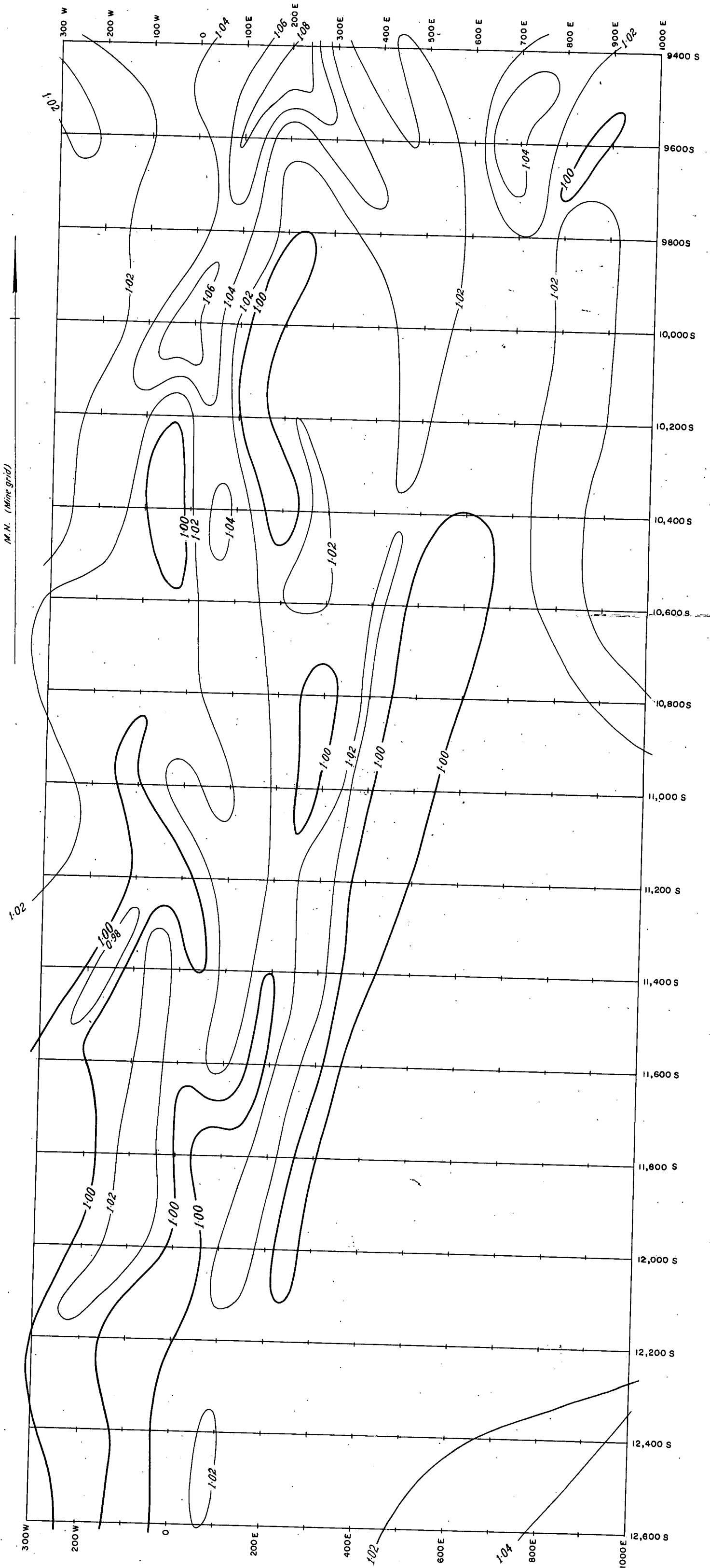
CAPTAINS FLAT, NSW. GOLF COURSE AREA TURAM RATIO CONTOURS
