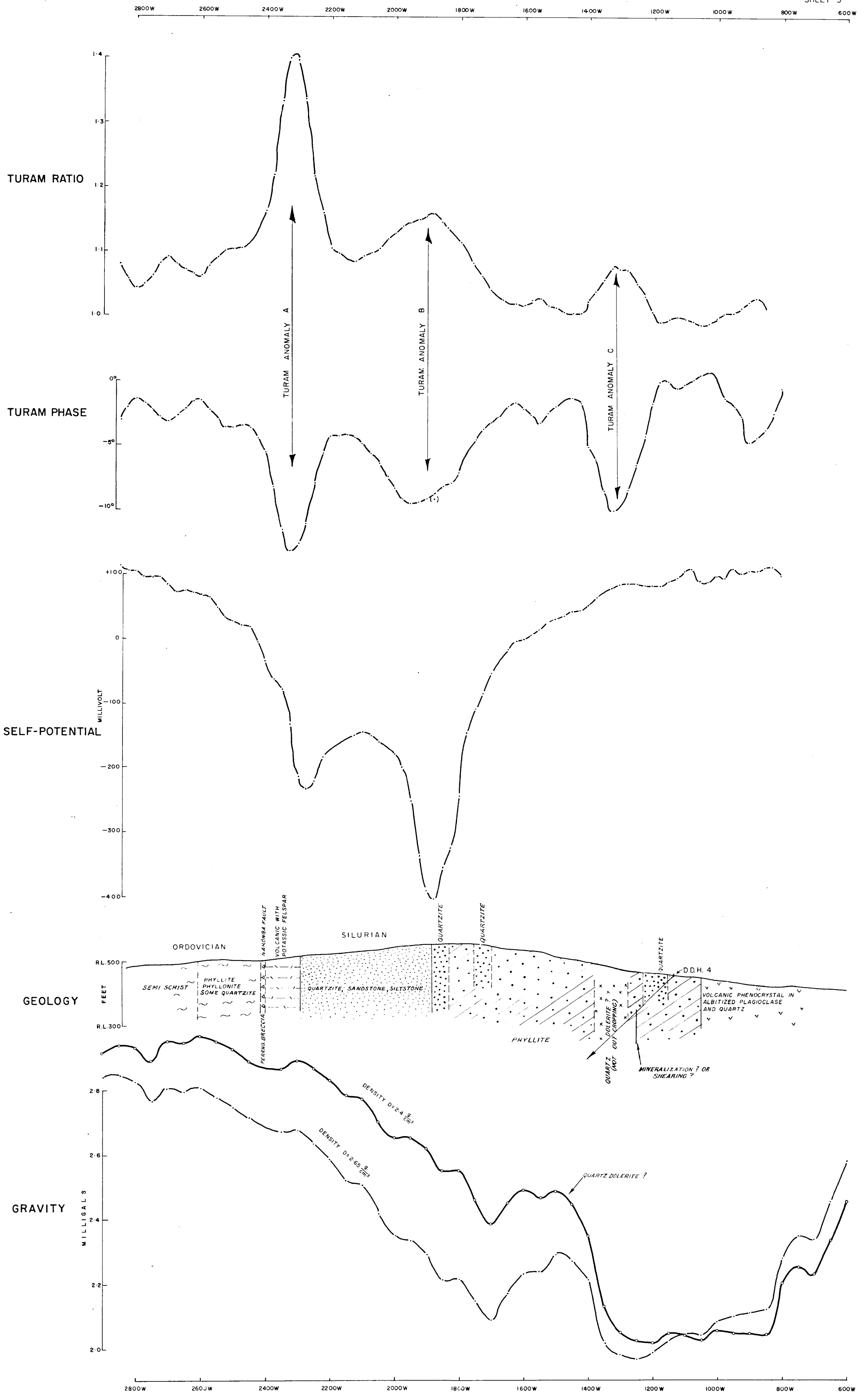
GOURLAY — HICKEY AREA TURAM, S.P., GEOLOGY, GRAVITY PROFILES, AND RECOMMENDED DRILL HOLE TRAVERSE 12,800 S. SCALE IN FEET
