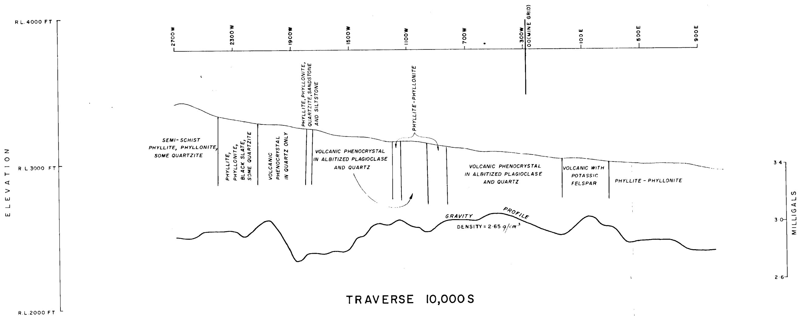
CAPTAINS FLAT N.S.W. TRAVERSES 1403 S, 5335 S, AND 10,000 S GRAVITY PROFILES AND GEOLOGICAL CROSS-SECTIONS SCALES
