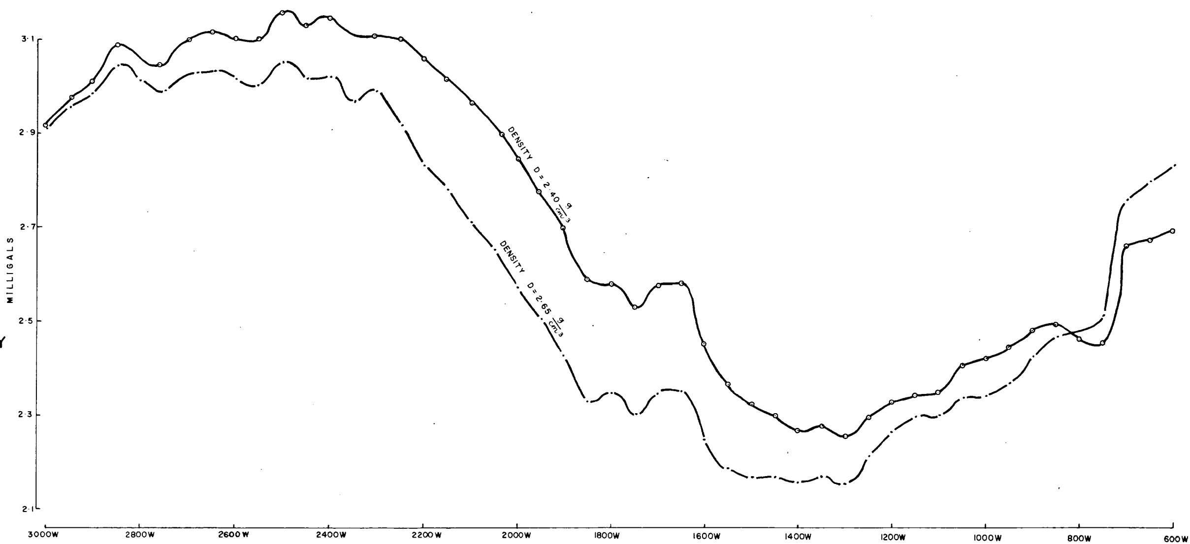
GOURLAY-HICKEY AREA TURAM, S.P., GEOLOGY, AND GRAVITY PROFILES TRAVERSE 12,200 S.
