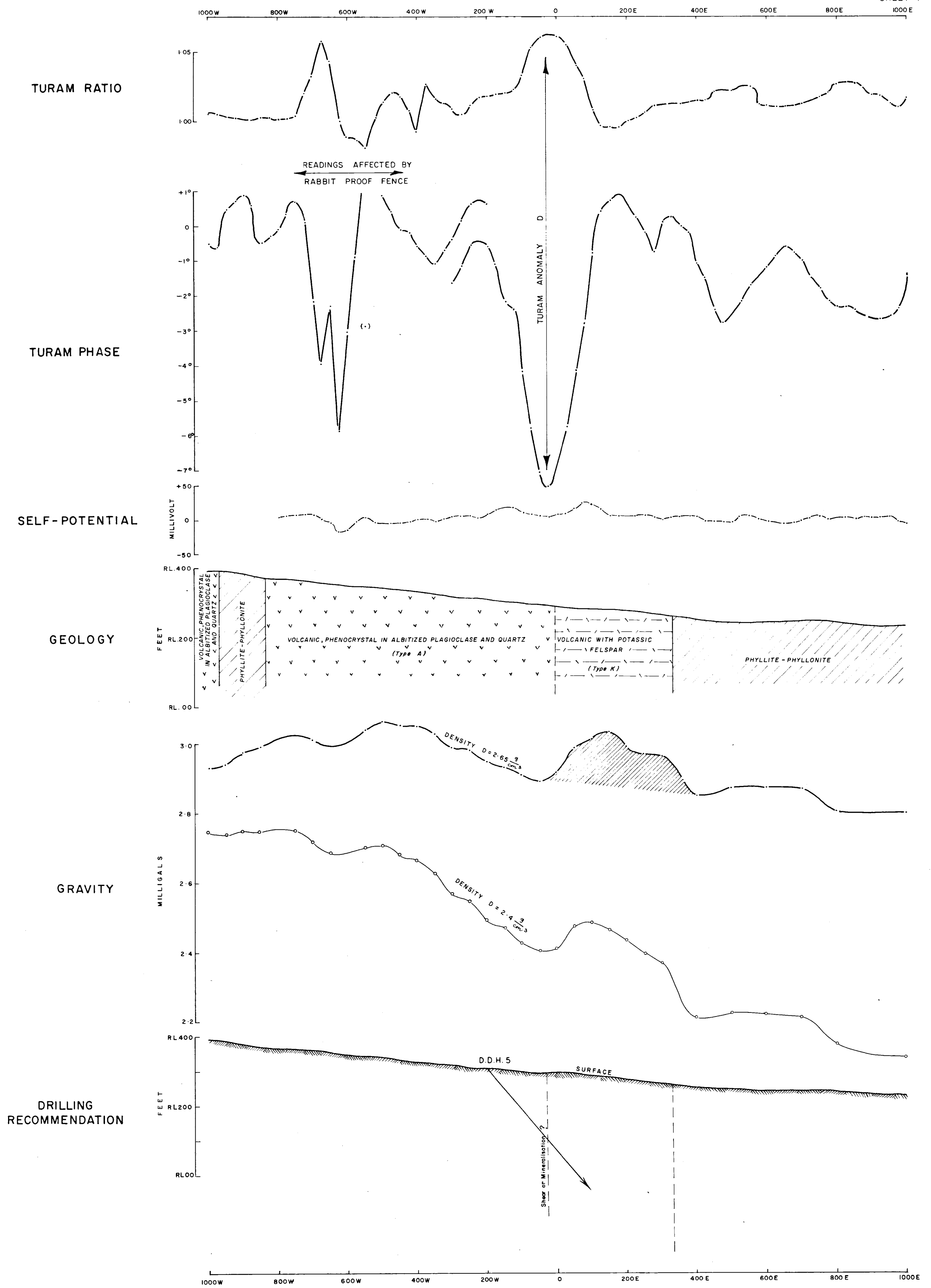
GOLF COURSE AREA TURAM, S.P., GEOLOGY, GRAVITY PROFILES, AND RECOMMENDED DRILL HOLE TRAVERSE 10,000 S.
