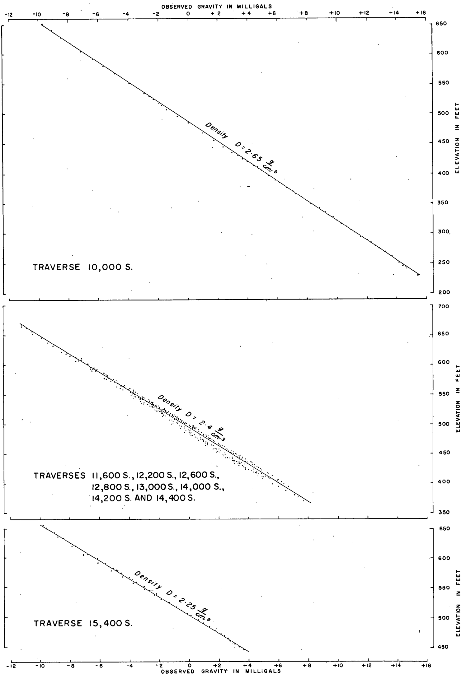
CAPTAINS FLAT, N.S.W. GOLF COURSE AND GOURLAY — HICKEY AREAS GRAPHS USED FOR DENSITY DETERMINATION BETWEEN TRAV. 10,000 S. AND TRAV. 15,400 S.
