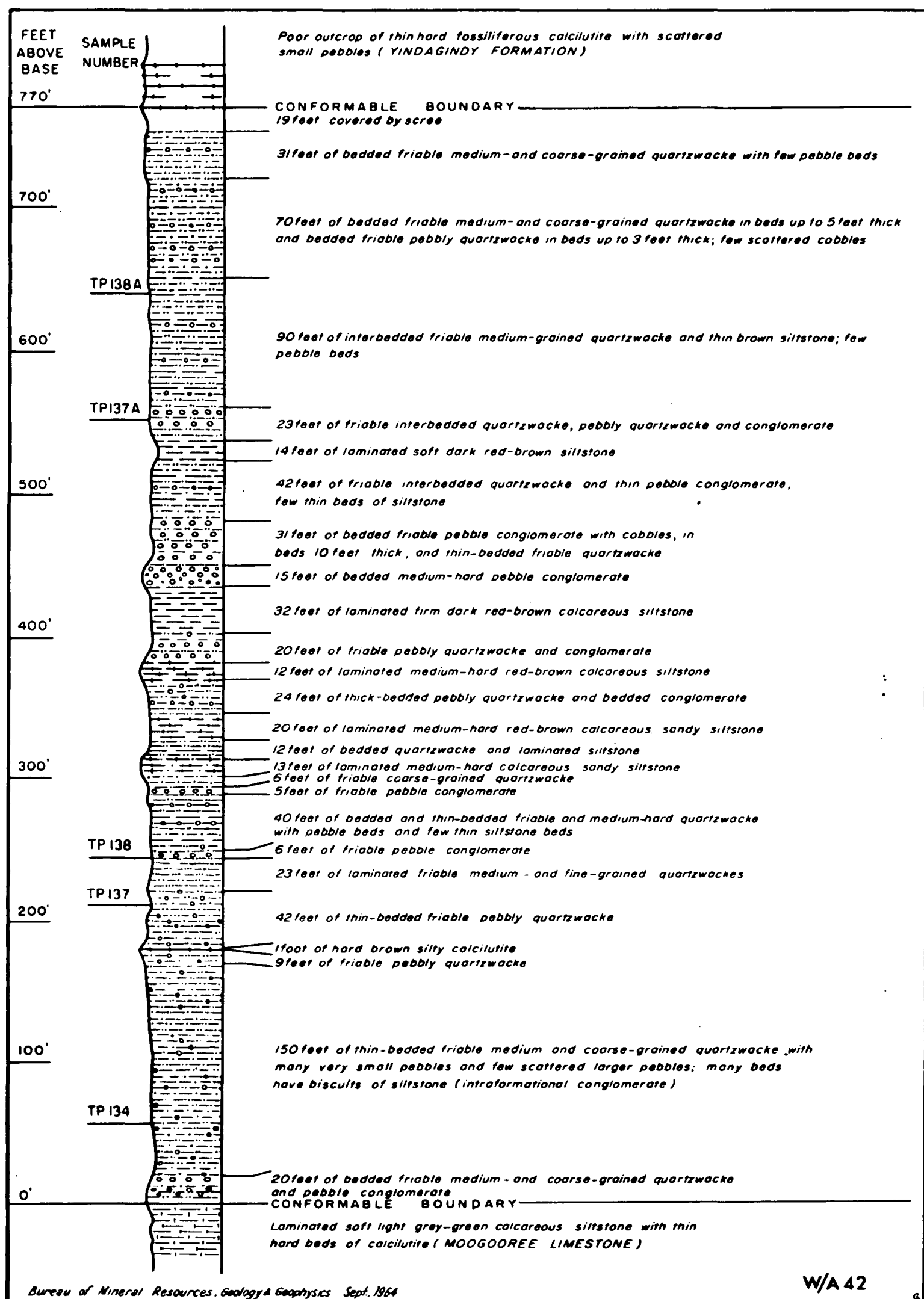
Fig. 28 Type section, Williambury Formation
