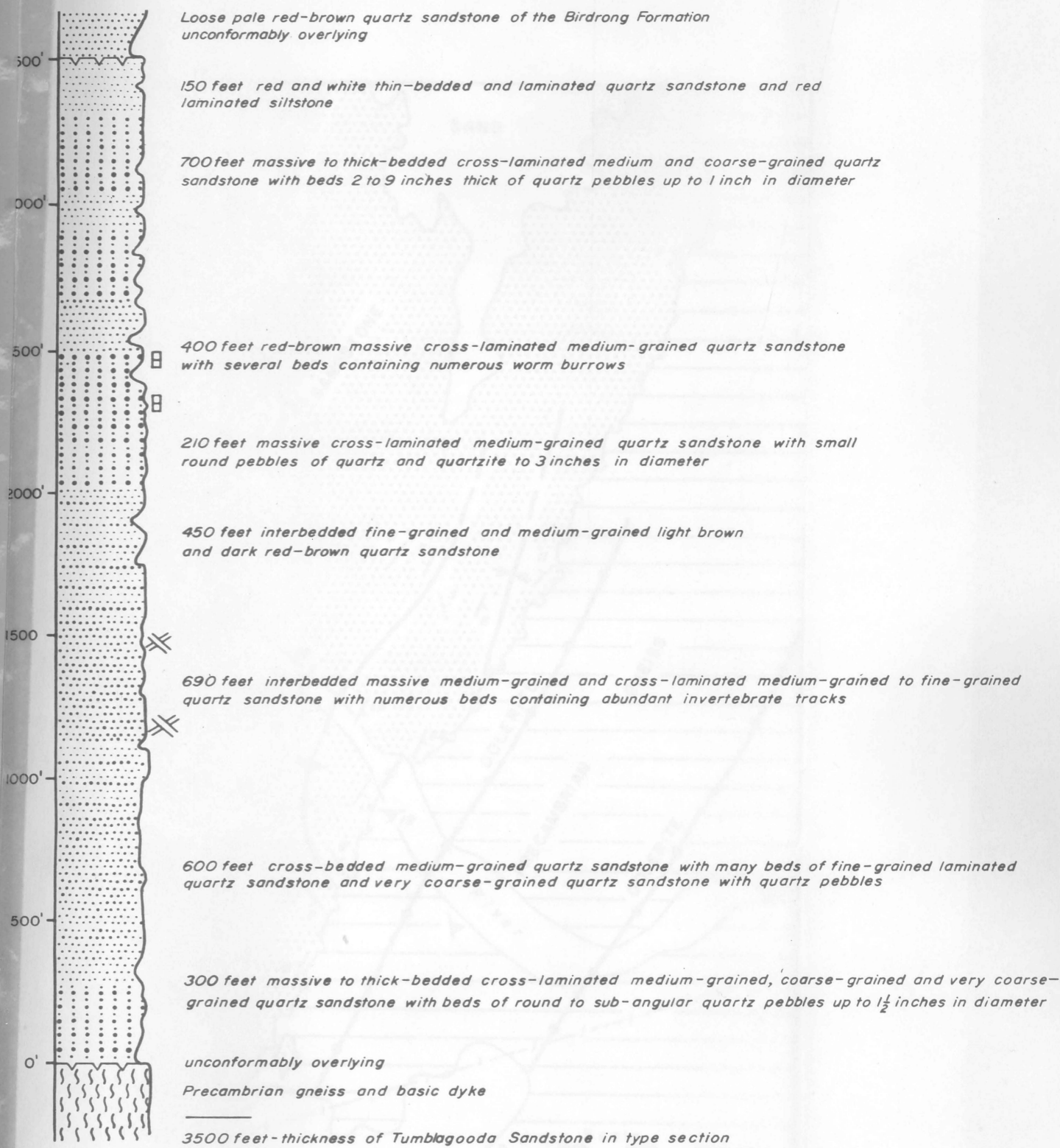
Fig. 7. Type section, Tumblagooda Sandstone
