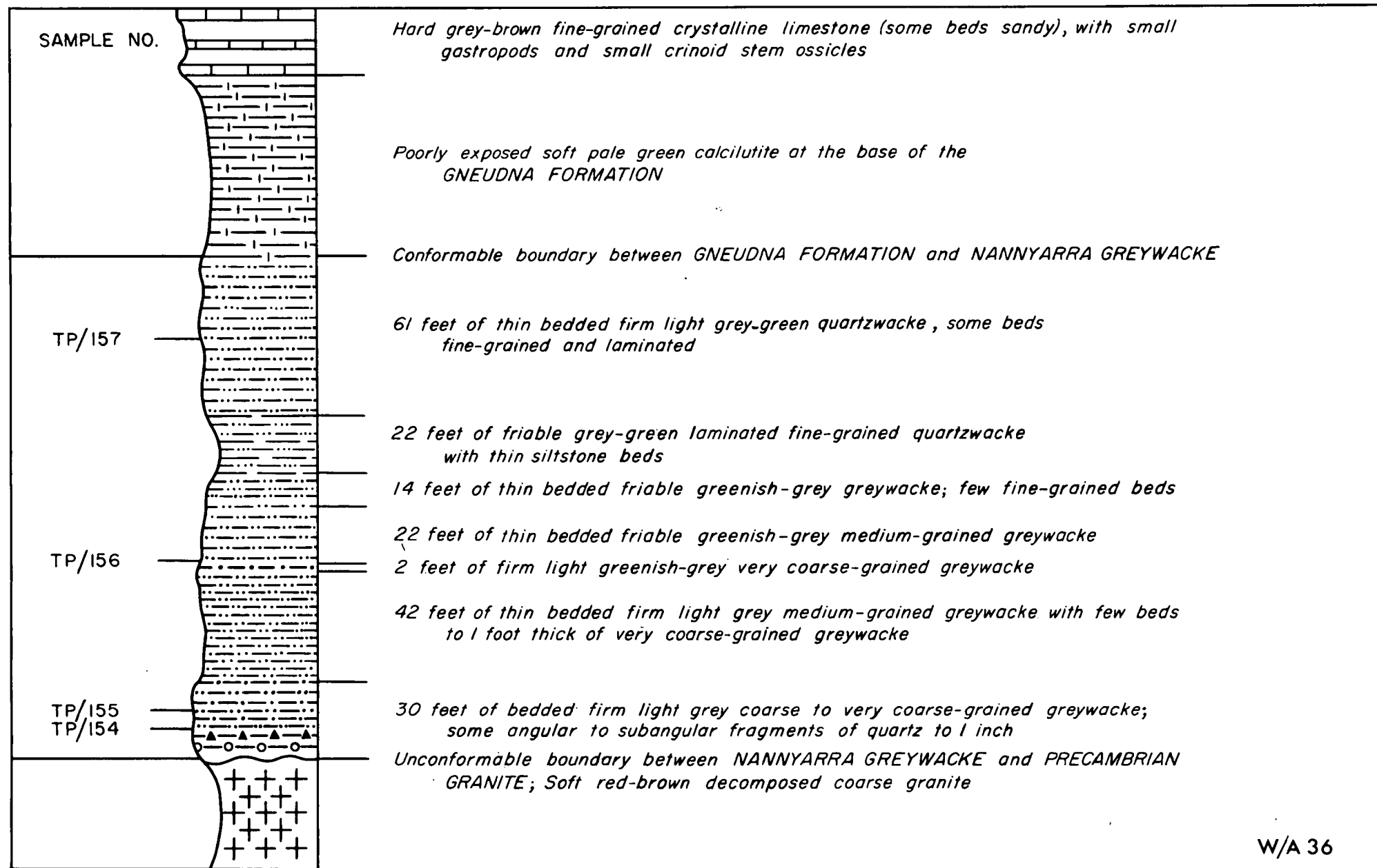
Fig. II - Type section, Nannyarra Greywacke
