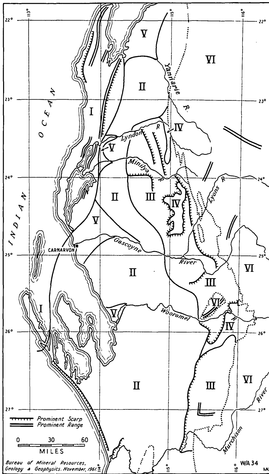
Fig.3 Physiographic subdivisions. Carnarvon Basin
