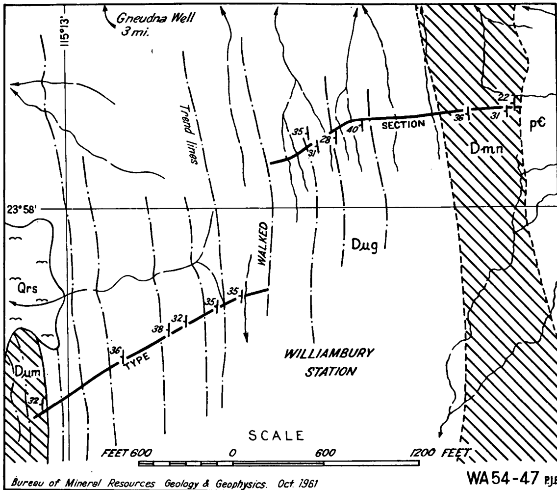
Fig. 10. Type locality, Nannyarra Greywacke (Dmn) and Gneudna Formation (Dug).
