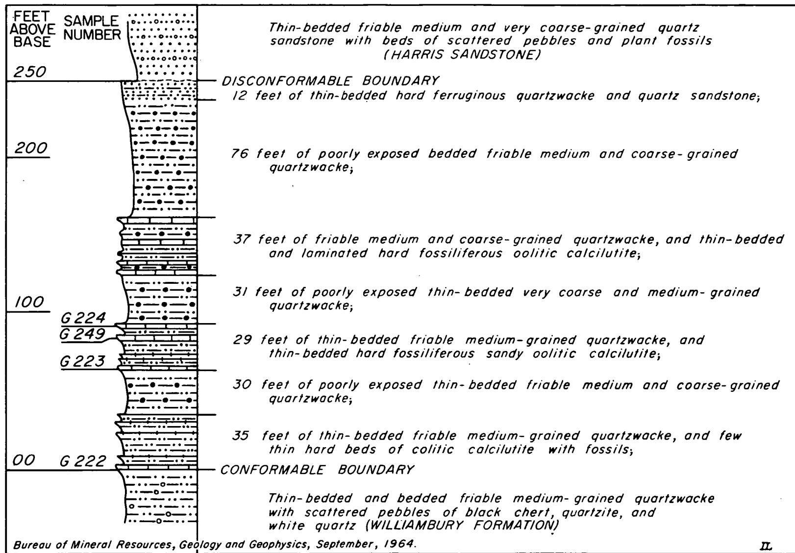
Fig. 31. Type section, Yindagindy Formation
