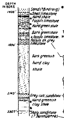
1 PELICAN HILL BORE 10 MILES N OF CARNARVON
