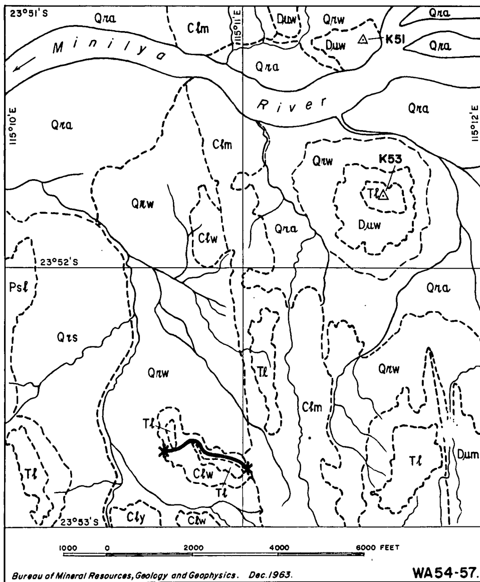
Fig. 27. Type locality, Williambury Formation
