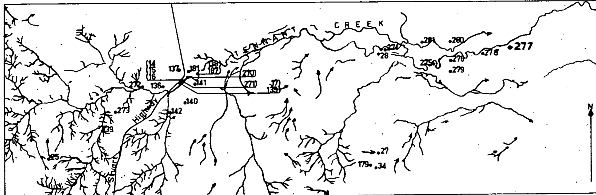
MAP OF TENNANT CREEK AND FLOODOUT AREA SHOWING LOCATIONS OF BORE SITES.
