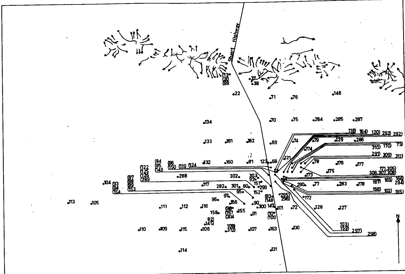
MAP OF CABBAGE GUM AREA, TENNANT CREEK, SHOWING LOCATIONS OF BORE SITES.
