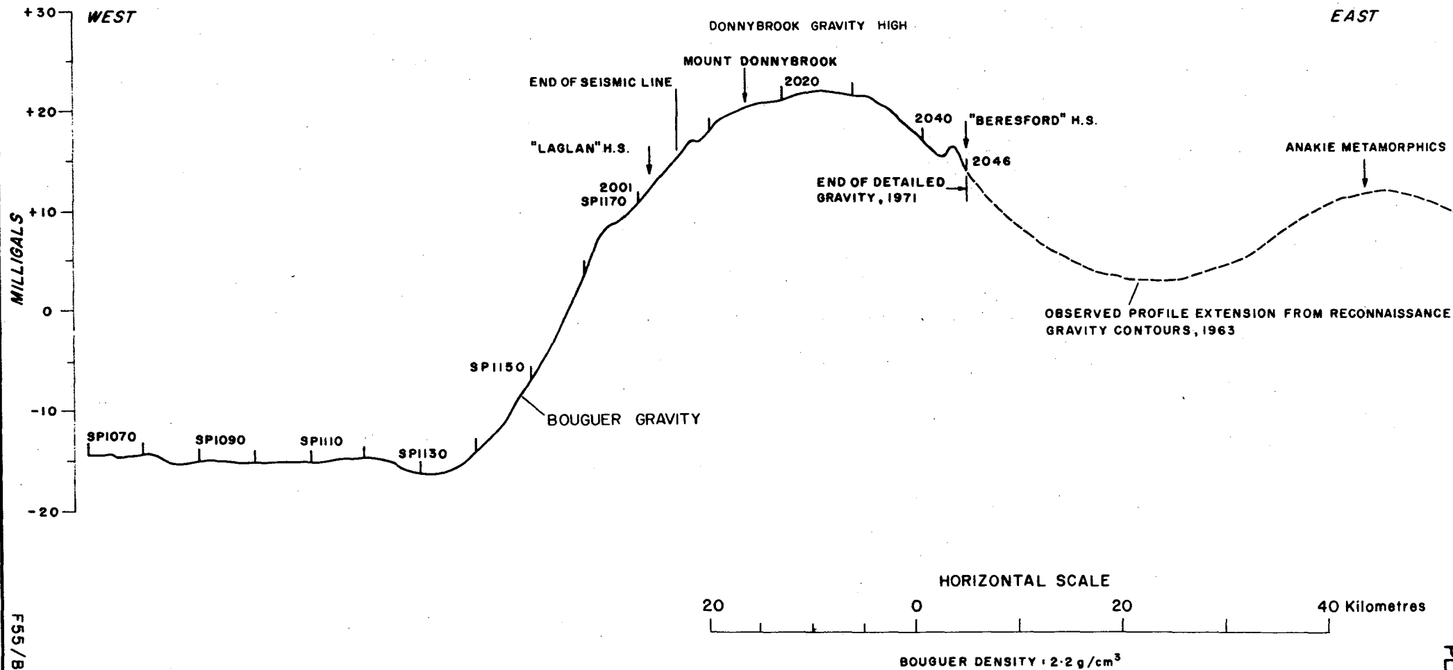
FINAL BOUGUER ANOMALY PROFILE
