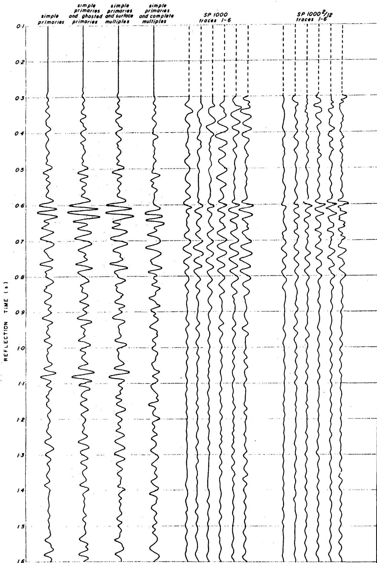
COMPARISON OF SYNTHETIC AND FIELD SEISMOGRAMS
