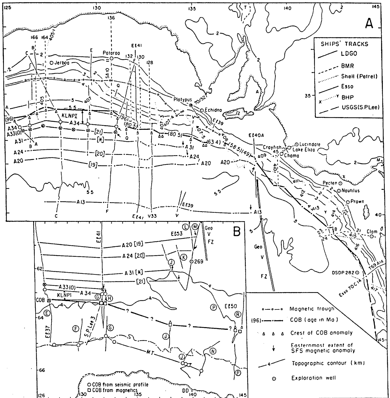
Figure 38: A. Southern Australian margin between 125 E and 145 E showing selected ships' tracks of L-DGO, BMR, Shell, Esso, and BHP, seafloor spreading magnetic anomalies, continent-ocean boundary, exploration wells, and bathymetry. B. Wilkes Land, Antarctica, margin, at similar scale to A, and conjugate with Australian sector west of line 408, showing locations of ships' tracks, seafloor spreading magnetic anomalies, continent-ocean boundary, COB anomaly crest, and magnetic trough (MT). (After Veevers, 1987.)
