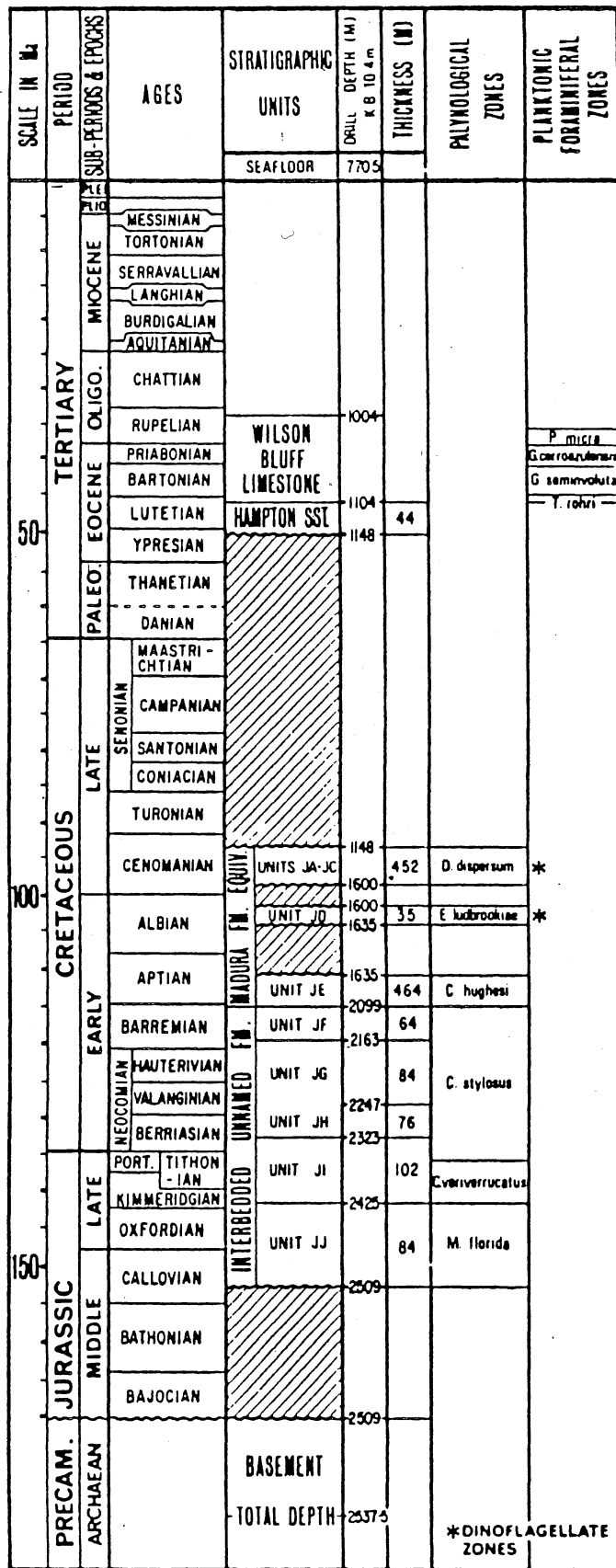
Figure 5: Stratigraphic chart for Jerboa-1 (after Bein & Taylor, 1981).
