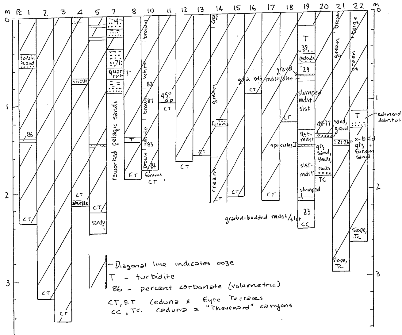
Figure 45: Summary graphic logs of all cores illustrate predominance of calcareous pelagic ooze on terraces and upper slope. Cores from canyons (GC 19-22) show that turbidite and debris flow deposits in canyons are buried beneath a cover of pelagic ooze. ET Eyre Terrace; CT Ceduna Terrace; CC Ceduna Canyon; TC 'Thevenard' Canyon. Summary of core locations: 8 Eyre Terrace; 5 and 7 Ceduna Terrace on seismic line 65/2; PC 1, GC 2-4 and 10-18 Ceduna Terrace line 65/15; 19 Ceduna Canyon; 20-22 'Thevenard' Canyon on floor, bench on east slope, and east slope respectively.
