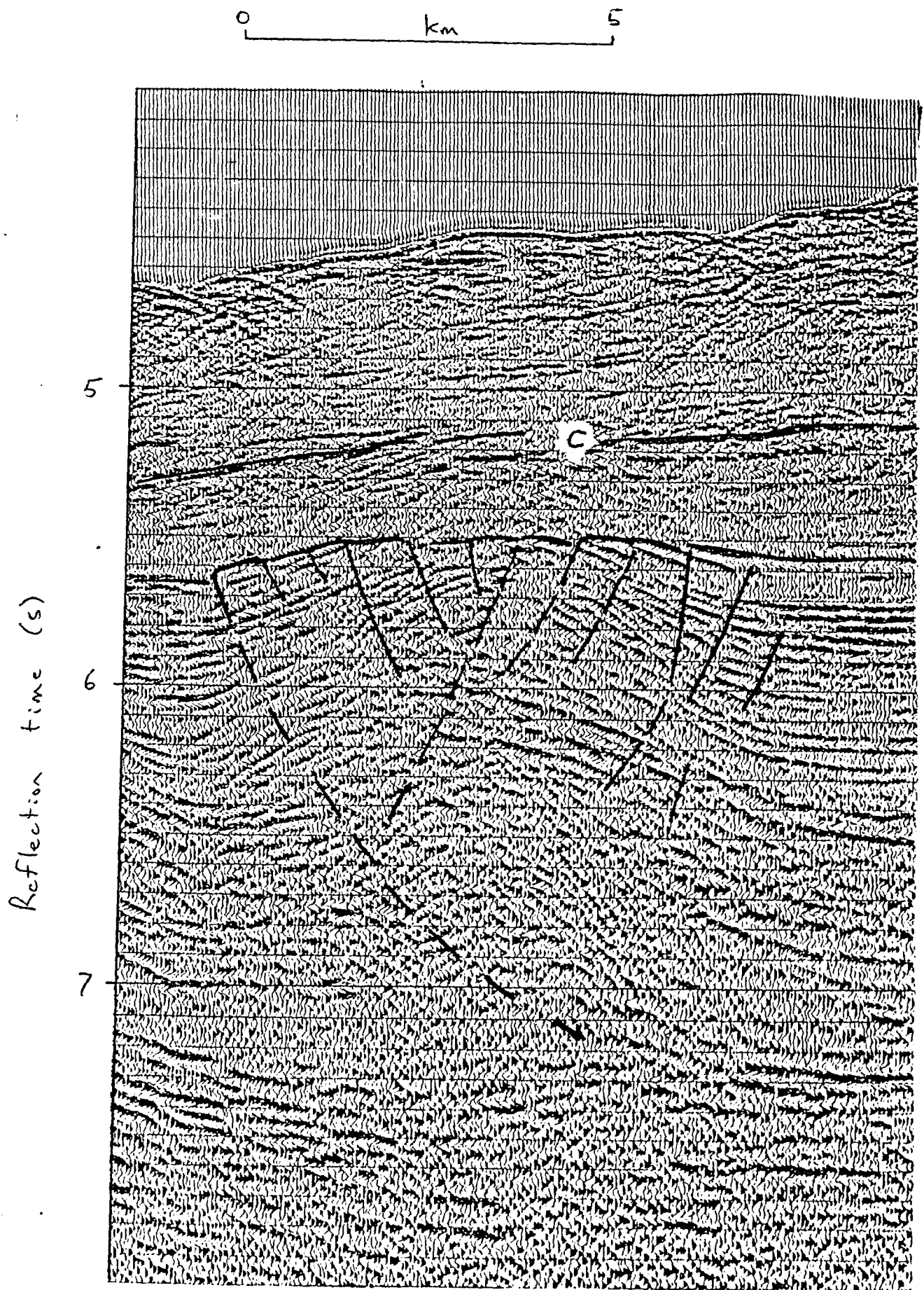
Figure 27: A portion of stacked seismic data for line 65/7 across the southwest flank of the Ceduna Terrace (GAB Basin), showing a faulted anticline and thrust plane possibly generated by transpressional tectonism.
