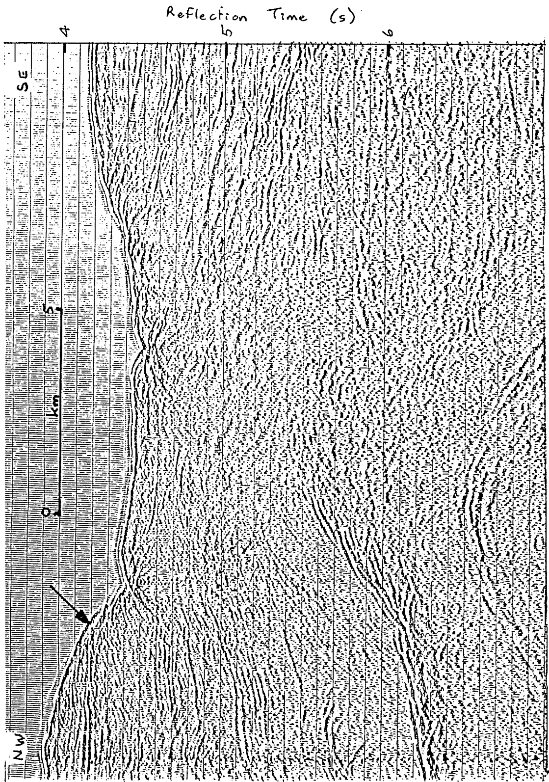
Figure 44: Stacked multichannel seismic reflection profile across 'Eucla' Canyon at about 33° 55'S, 128° 38'E, shows partly eroded anticline in Mesozoic strata. Dredge 1 recovered Maastrichtian, Paleocene and Early to Middle Eocene siliciclastic and carbonate/phosphate-siliciclastic sediments with some Tertiary? alkali basalt lava, and Late Eocene and younger foraminiferal spicular wackestone (fine pelagic limestone) from NW slope. Strong reflector (arrow) may represent unconformity at base of Late Eocene and younger fine limestone. Dredge 3 encountered a similar rock suite down canyon to SW.
