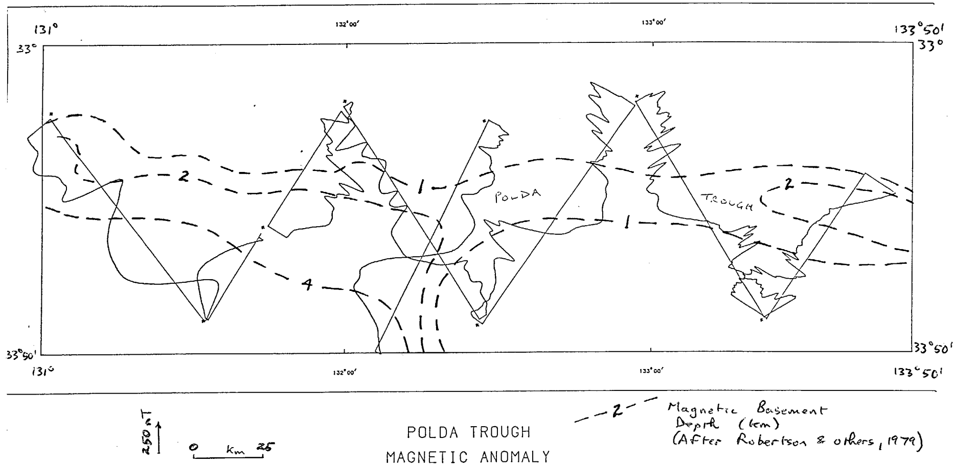
Figure 35: Magnetic anomaly profiles across the Polda Trough acquired during Leg 1. Major tectonic features are also shown.
