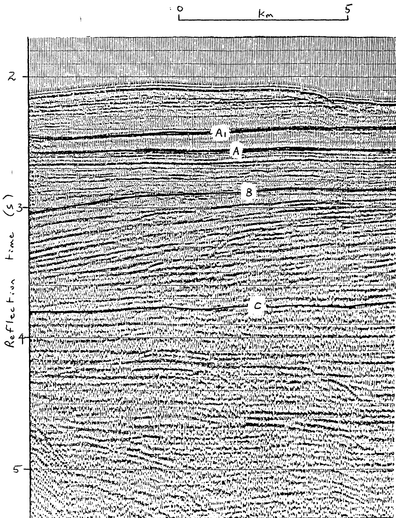
Figure 26: A portion of stacked seismic data for line 65/7 showing a prograding deltaic sequence (B-C) bounded by Maastrichtian and Cenomanian unconformities (as discussed by Tilbury & Fraser, 1979).
