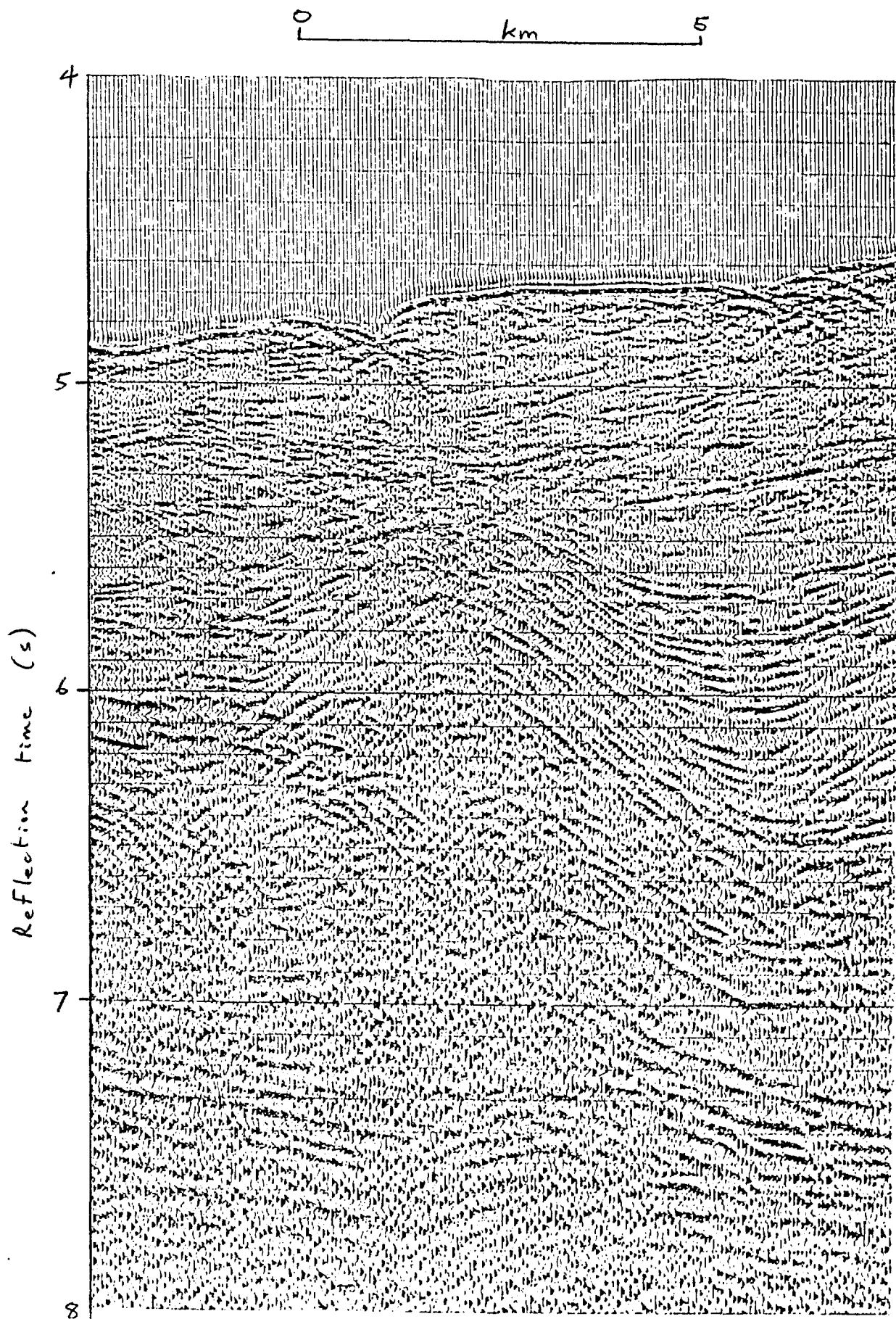
Figure 28: Possible transpressional structure on the southwest flank of the Ceduna Terrace (see also Fig. 27); stacked seismic data line 65/7.
