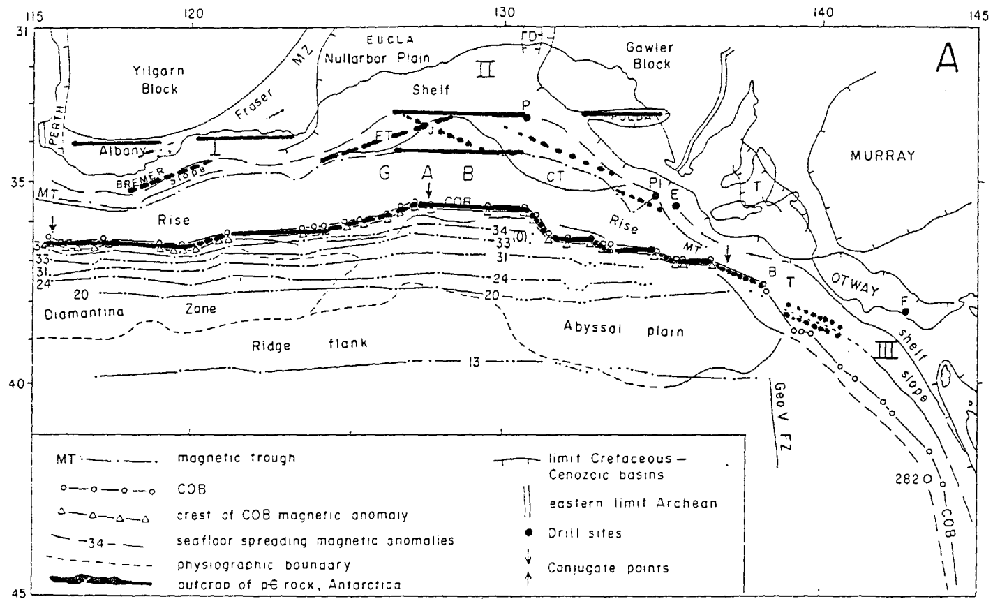
Figure 39: Southern margin of Australia showing the magnetic trough, COB, COB magnetic anomaly, seafloor spreading magnetic anomalies, and the principal physiographic boundaries (modified after Veever, 1987).
