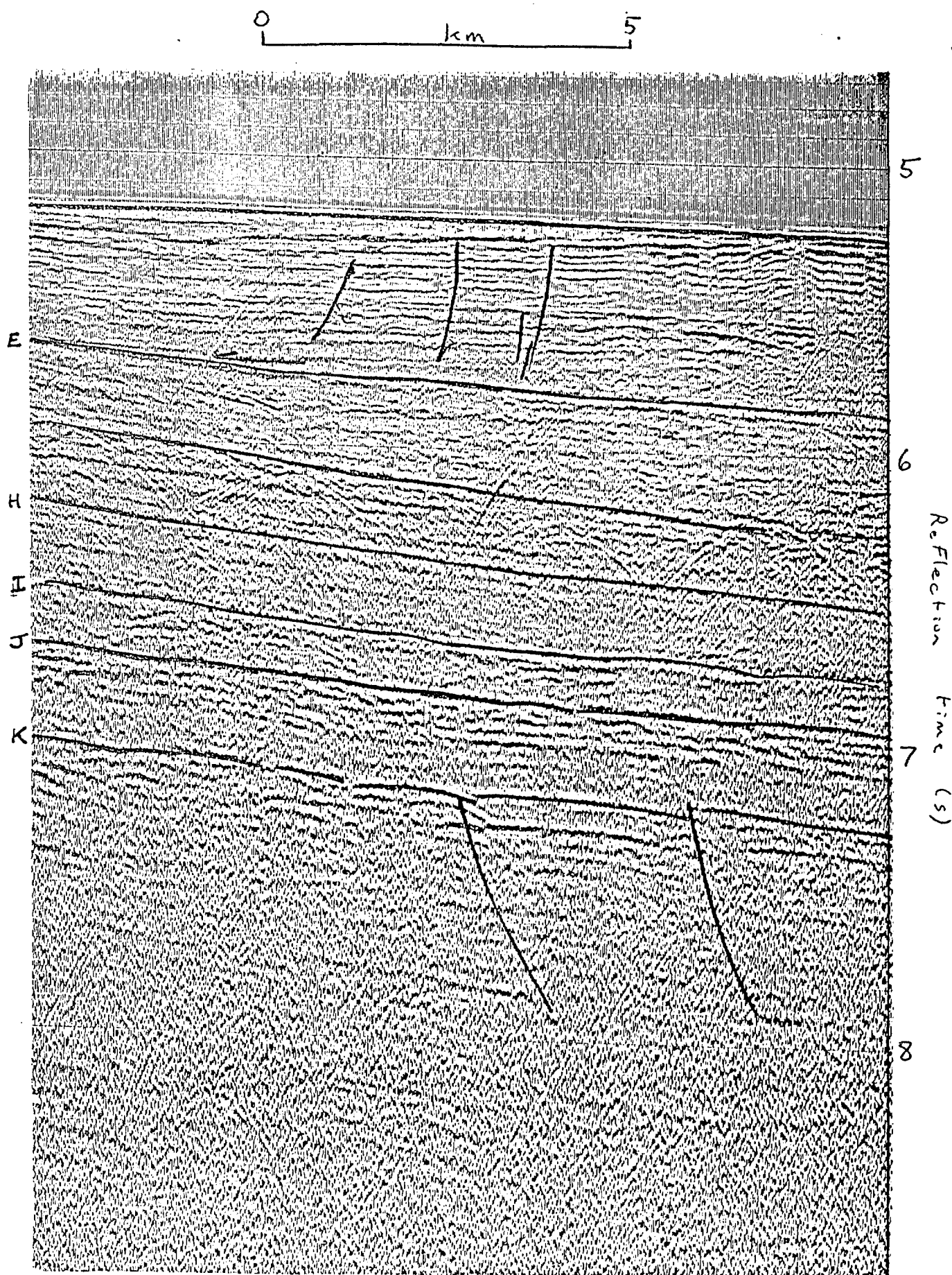
Figure 30: Unconformities beneath the continental rise south of the Eyre Terrace; stacked seismic data from line 65/4.
