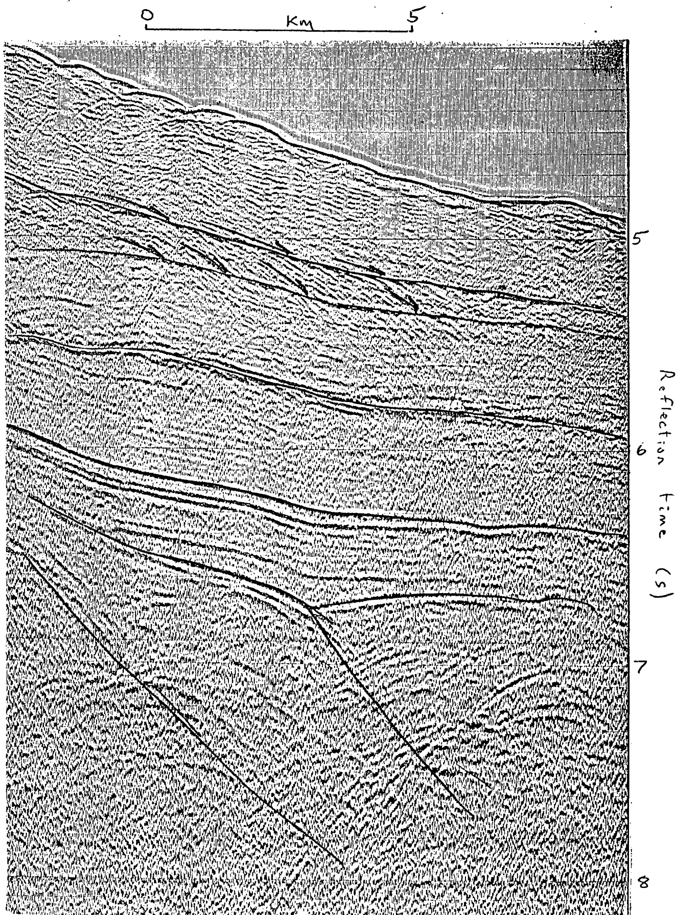
Figure 31: Unconformities beneath the inner continental rise, south of the Eyre Terrace, bounding sediment wedges, some of which show progradation. Note the possible underlying rotated fault blocks; stacked seismic data from line 65/4.
