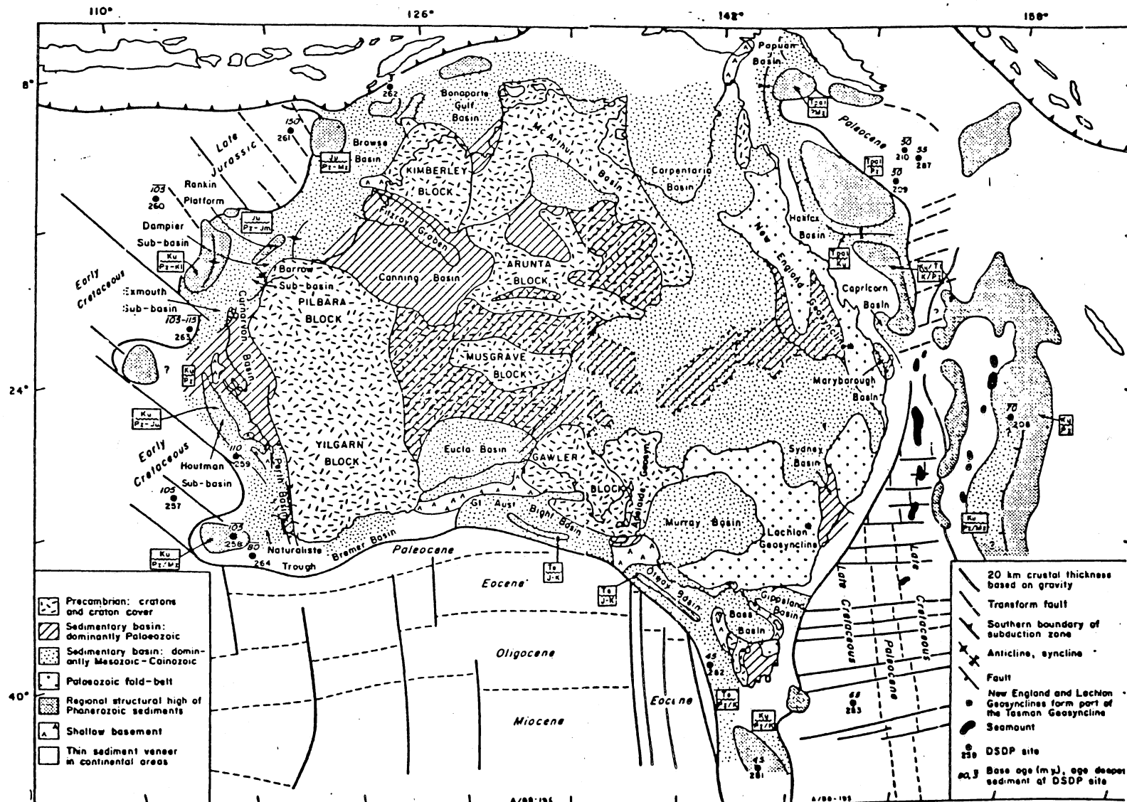
Figure 1: Structural elements in and around Australia (after Willcox, 1981), showing the location of the sedimentary basins along the southern margin. Note that the age of the oldest oceanic crust adjacent to the southern margin has been revised from the Palaeocene-Eocene shown in the figure, to Late Cretaceous.
