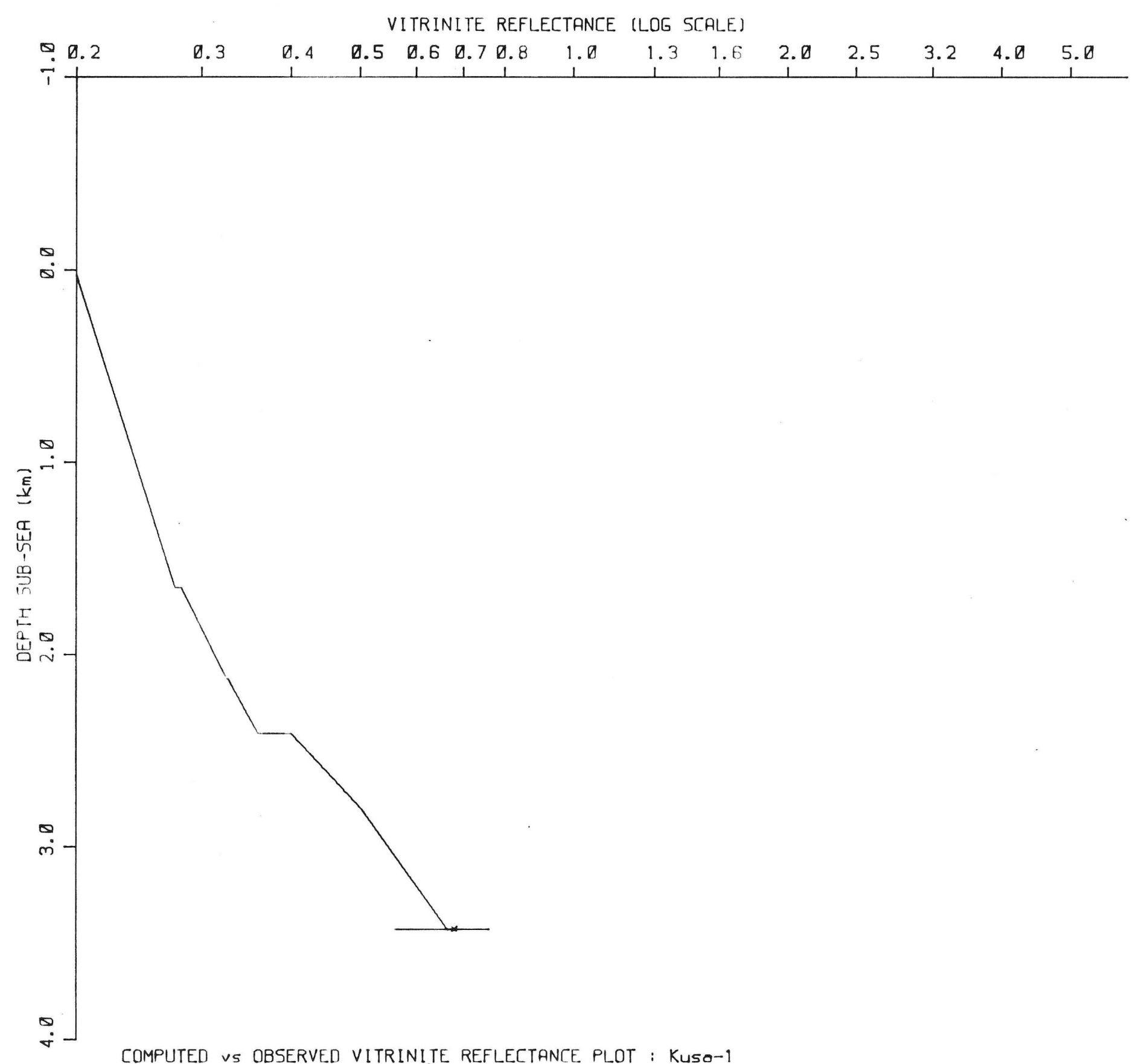
COMPUTED vs OBSERVED VITRINITE REFLECTANCE PLOT : Kusa-1
