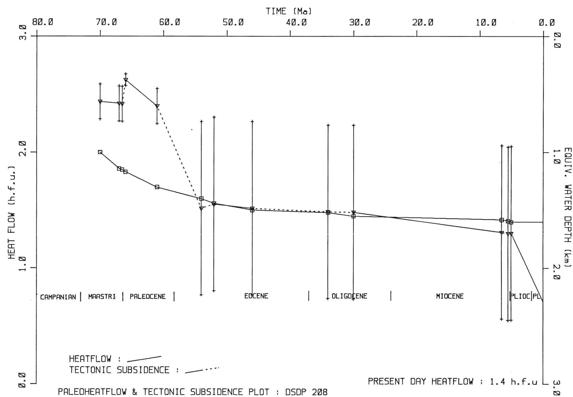
PALEOHEATFLOW & TECTONIC SUBSIDENCE PLOT : DSDP 208
