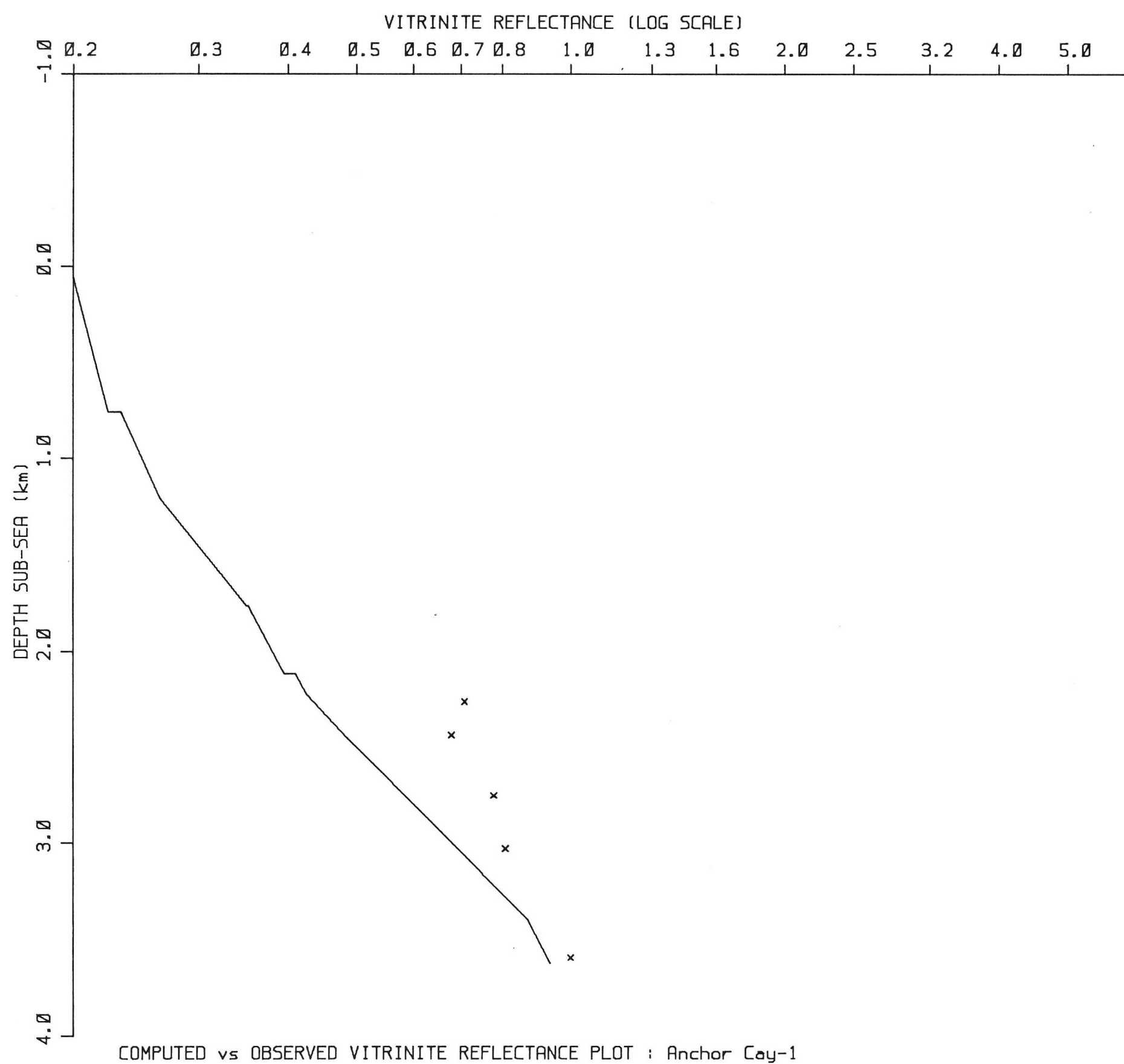
COMPUTED vs OBSERVED VITRINITE REFLECTANCE PLOT : Anchor Cay-1
