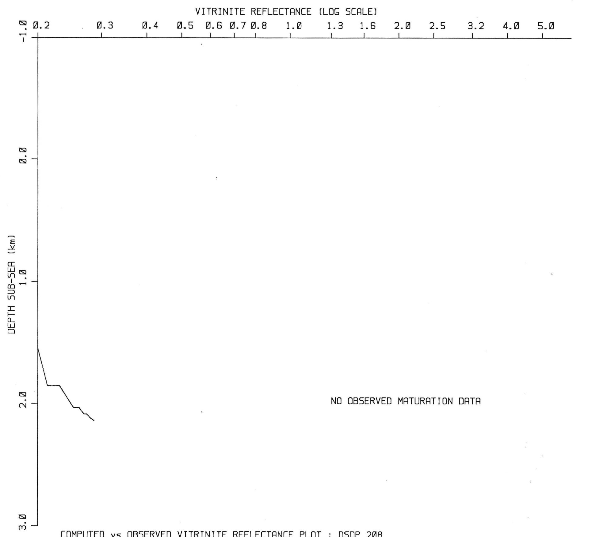
COMPUTED vs OBSERVED VITRINITE REFLECTANCE PLOT : DSDP 208
