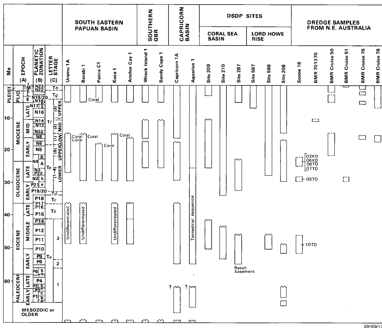
Figure 2. Biostratigraphic summary for all localities used in this study. (A) after Berggren et al., (1985a, b); (B) after Blow (1969), Berggren (1969), Kennett and Srinivasan (1983; (C) after Adams (1984), Adams et al., (1986), Chaproniere (1981, 1983) and Jenkins et al., (1985).
