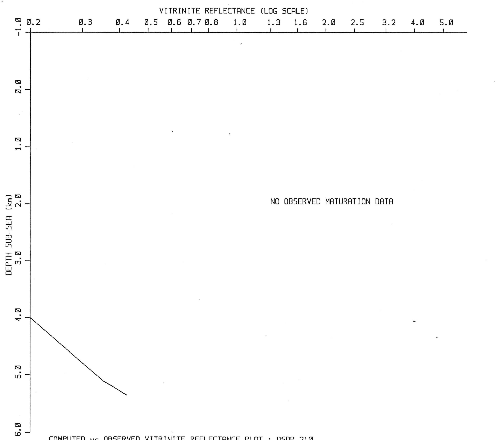
COMPUTED vs OBSERVED VITRINITE REFLECTANCE PLOT : DSDP 210
