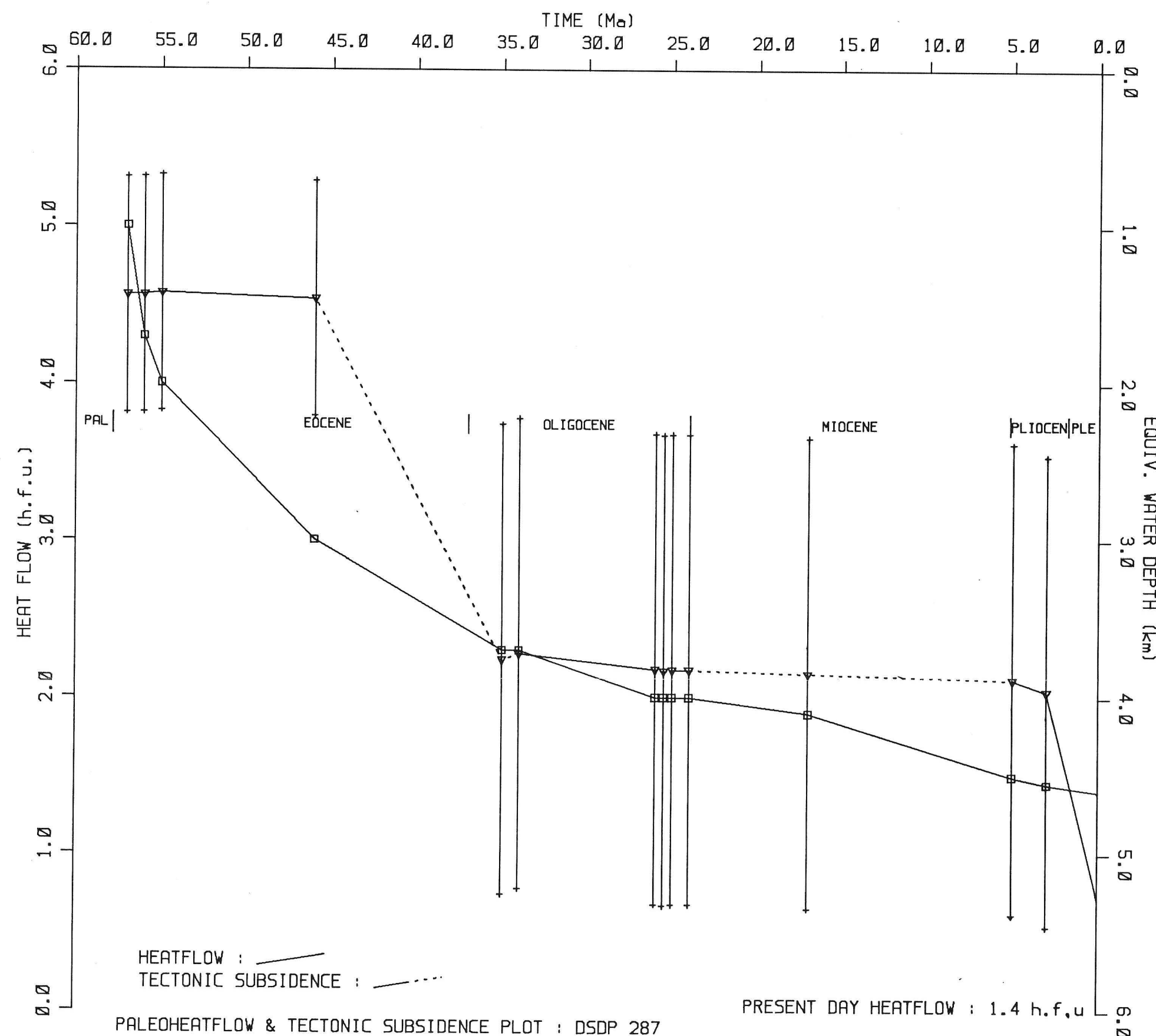
PALEOHEATFLOW & TECTONIC SUBSIDENCE PLOT : DSDP 287
