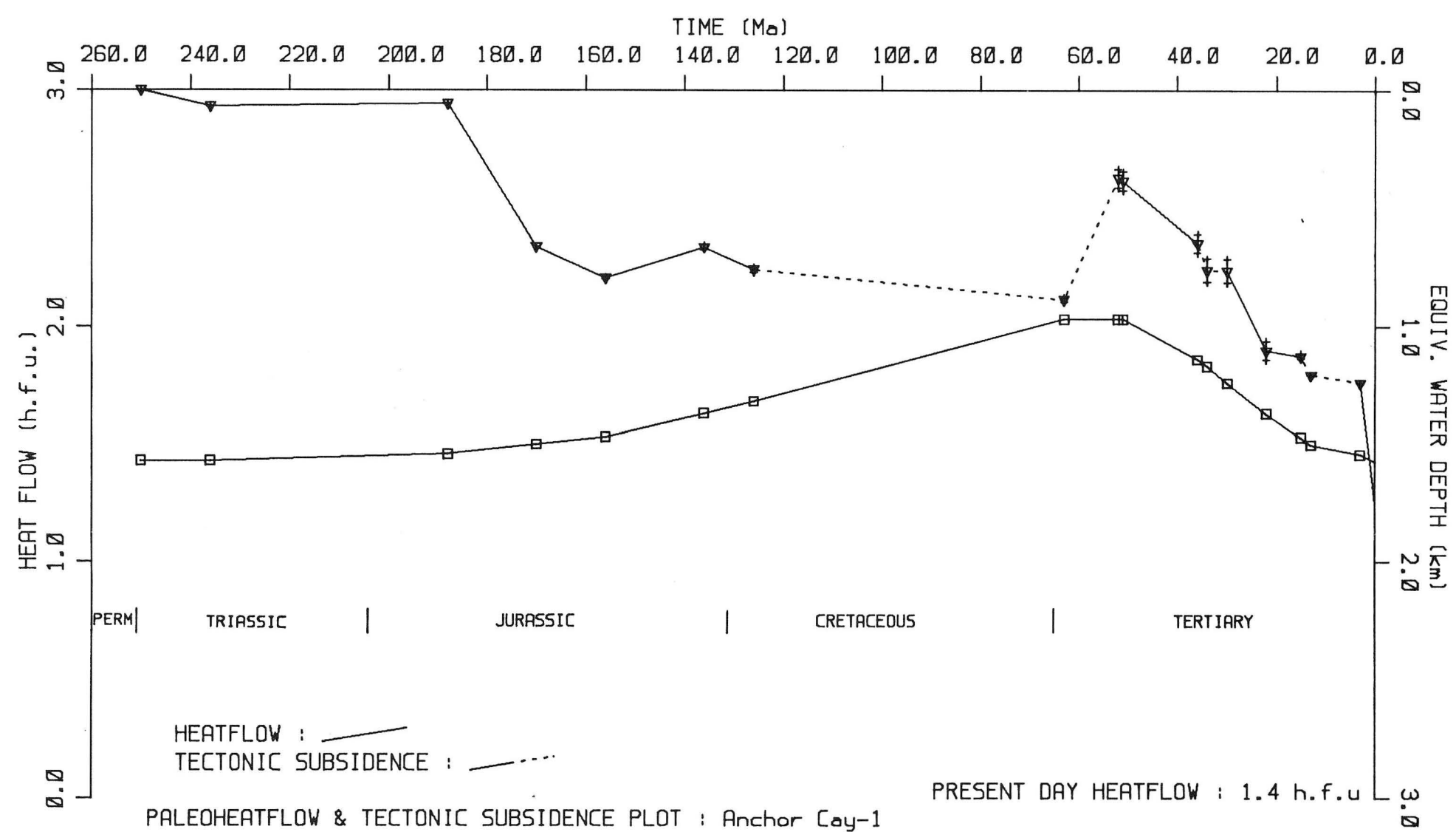
PALEOHEATFLOW &amp; TECTONIC SUBSIDENCE PLOT : Anchor Cay-1
