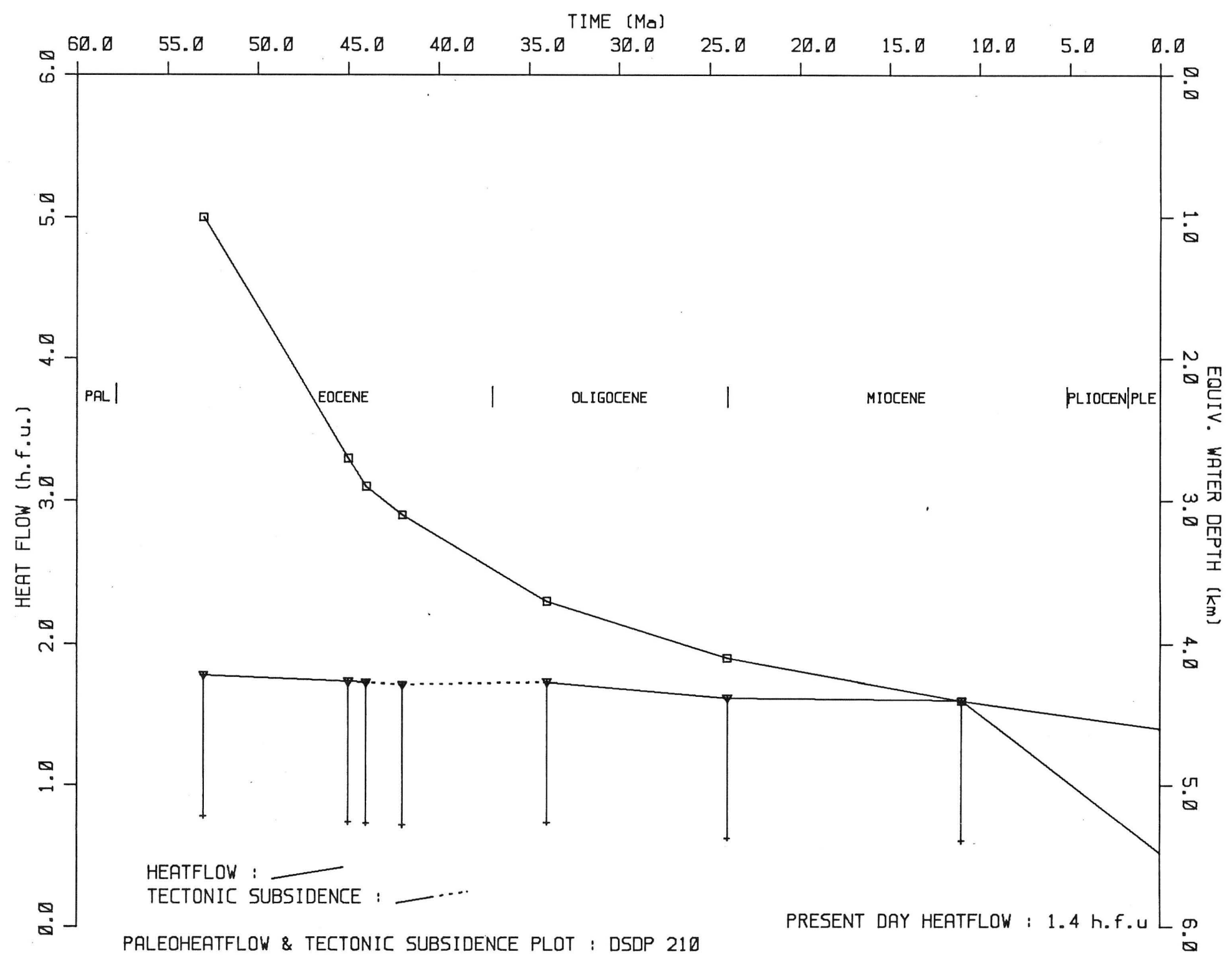
PALEOHEATFLOW & TECTONIC SUBSIDENCE PLOT : DSDP 210
