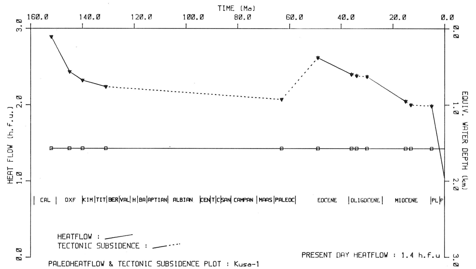
PALEOHEATFLOW & TECTONIC SUBSIDENCE PLOT : Kusa-1
