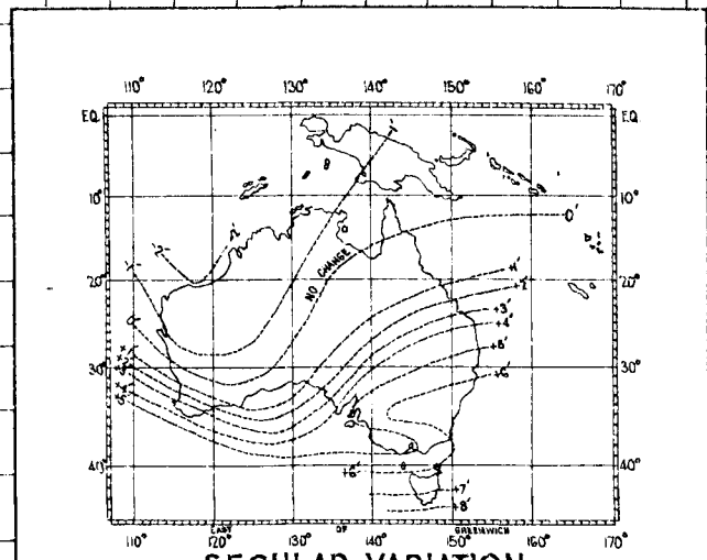
SECULAR VARIATION OF THE MAGNETIC DECLINATION FOR THE EPOCH 1955.5 The lines of equal Annual Change of Declination over the mainland of Australia and Tasmania are based on very limited information. The extension of the lines over seas and islands, in particular, must be regarded as very doubtful. Values are given in minutes. + Indicates that the North-Seeking End of the Magnetic Needle is moving Eastward. - Indicates that the North-Seeking End of the Magnetic Needle is moving Westward.
