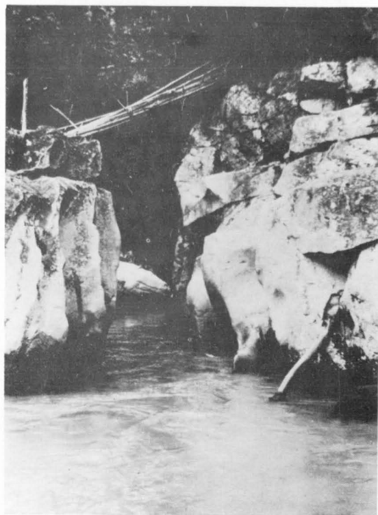
Fig. 1: Ramu gorge, showing strongly jointed gabbro.
