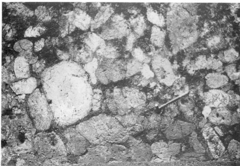
Fig. 1: Lamari Conglomerate in road cutting.
