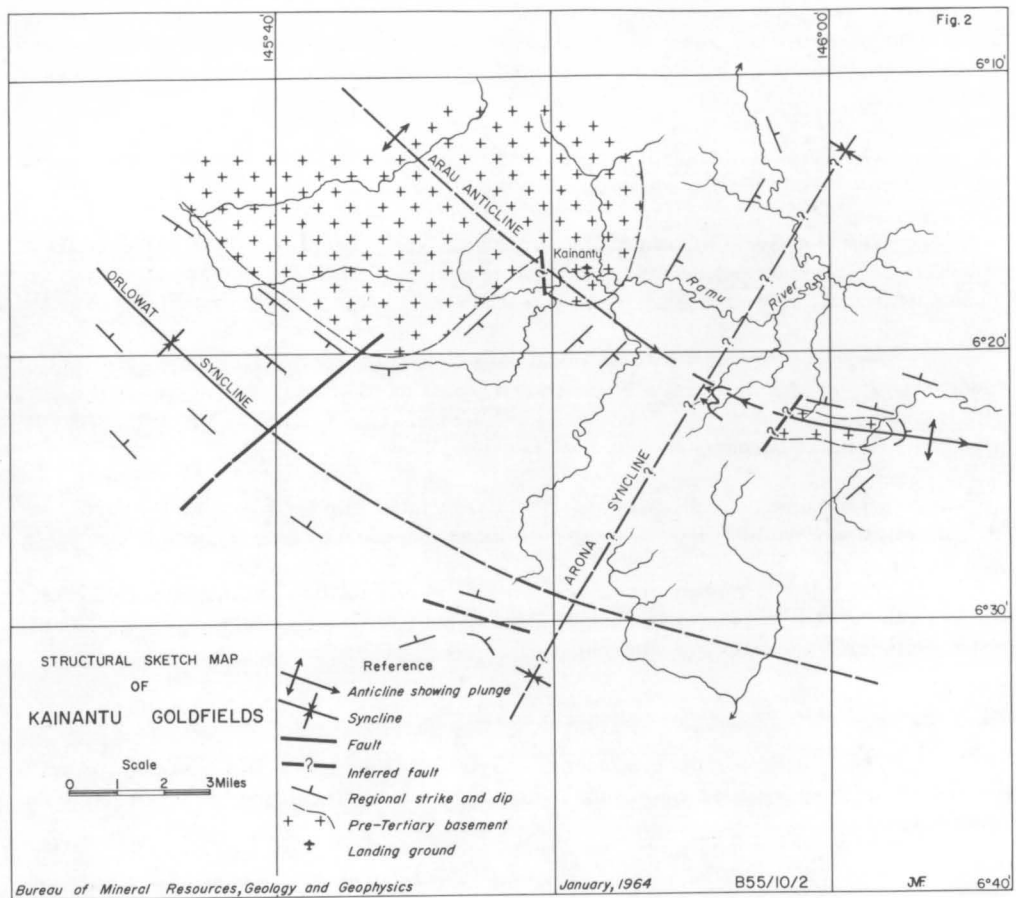
Figure 2: Structural sketch map of Kainantu Goldfields.
