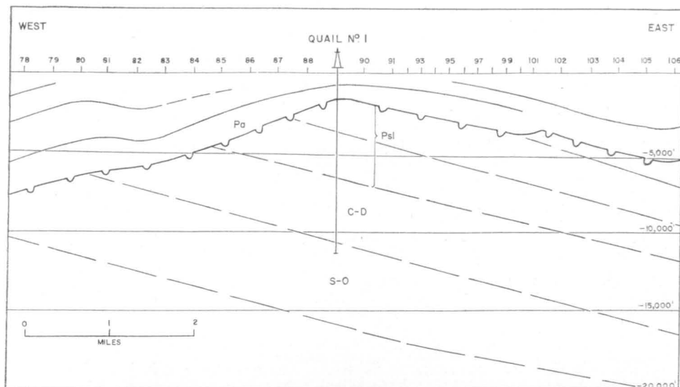
Fig. 161. Interpretation of seismic section through Quail No. 1 Well. Pa—Artinskian; Psl—Lyons Group; C-D—Carboniferous and Devonian; S-O—Silurian and Ordovician.
