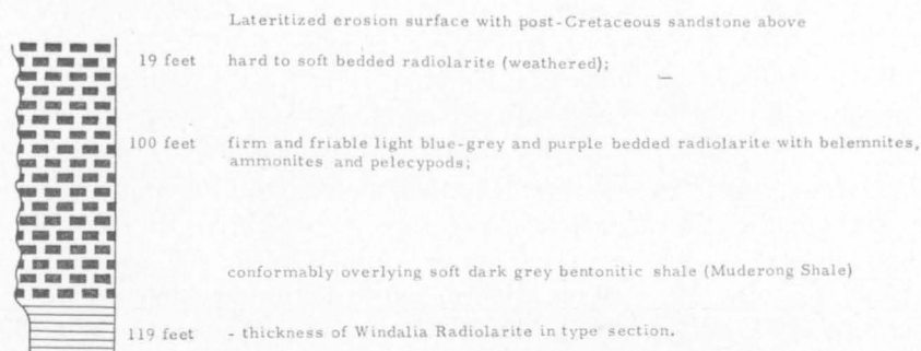
Fig. 152. Type section, Windalia Radiolarite.
