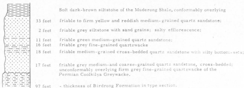
Fig. 148. Type section, Birdrong Formation.
