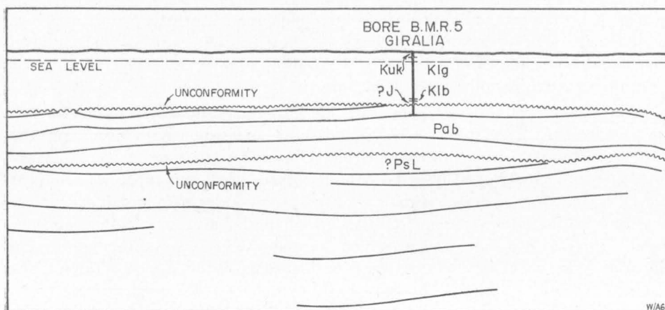
Fig. 160. Section across Giralia Anticline showing structural discordance between Lyons Group (Psl) and Byro Group (Pab). Structure based on seismic reflections; stratigraphy from BMR 5.
