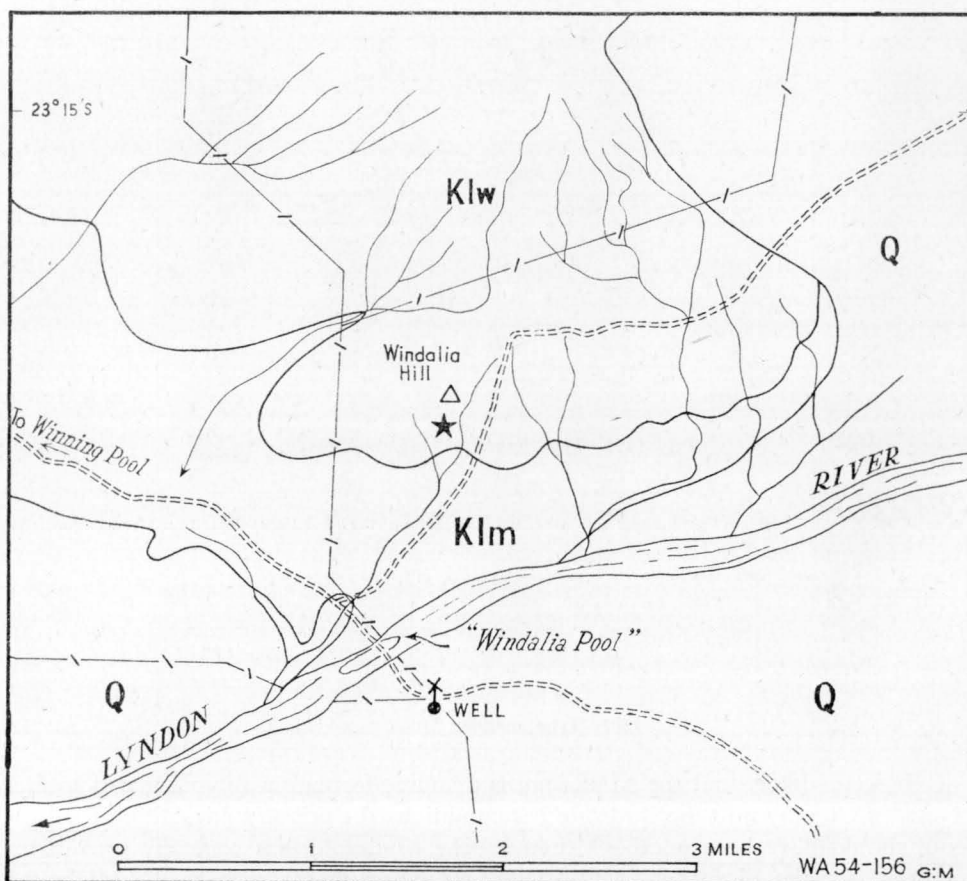
Fig. 151. Type locality, Windalia Radiolarite.
