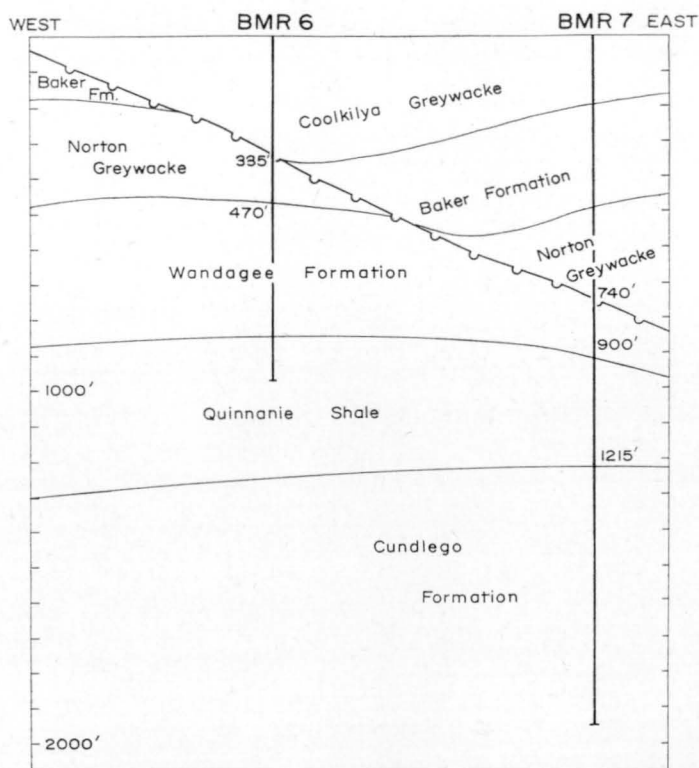
Fig. 159. Structural interpretation, BMR 6 and 7.
