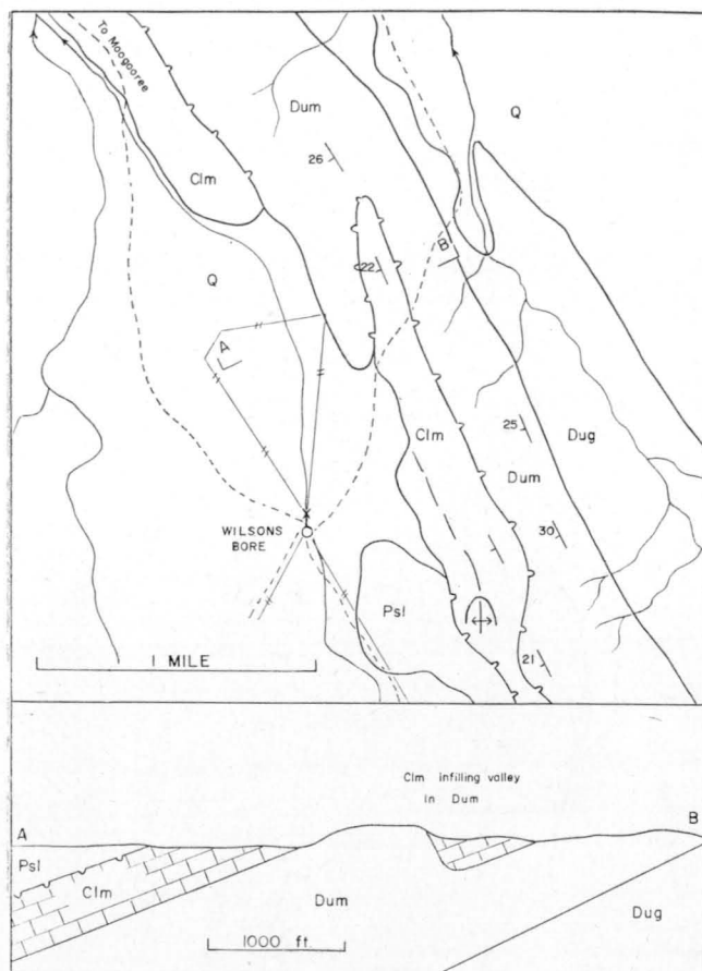
Fig. 157. Unconformity between Devonian and Carboniferous, Moogooree station. Q—superficial cover; Psl—Lyons Group; Clm—Moogooree Limestone; Dum—Munabia sandstone; Dug—Gneudna Formation.
