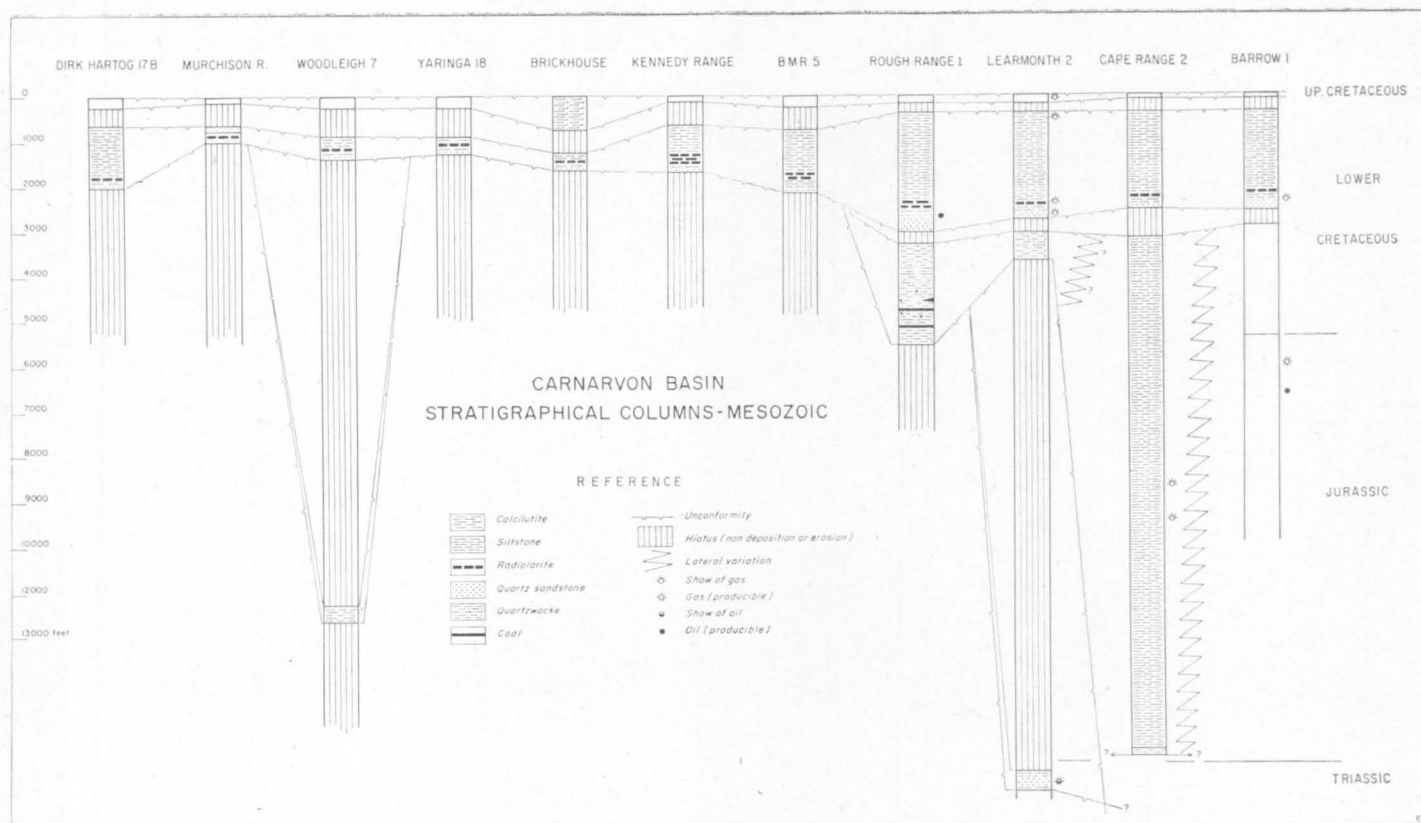
Fig. 144. Stratigraphical columns of the Mesozoic.
