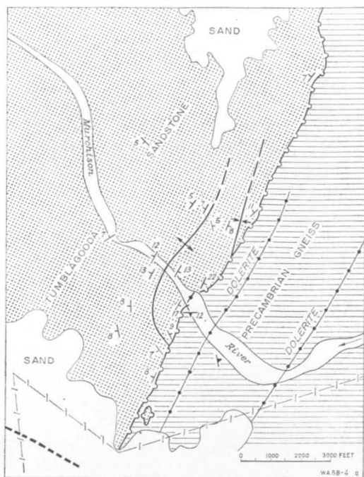
Fig. 155. Contact between Tumblagooda Sandstone and Precambrian gneiss.
