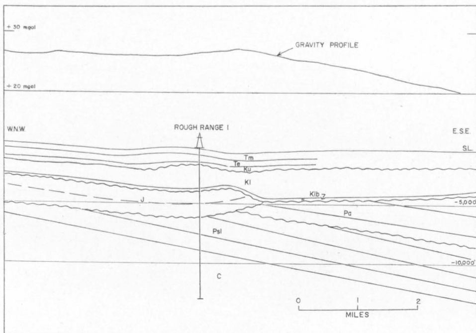
Fig. 162. Interpretative section through Rough Range No. 1 Well. Tm—Miocene; Te—Eocene; Ku—Upper Cretaceous; Kl—Lower Cretaceous; Klb—Birdrong Formation; J—Jurassic; Pa—Artinskian; Psl—Lyons Group; C—Carboniferous.
