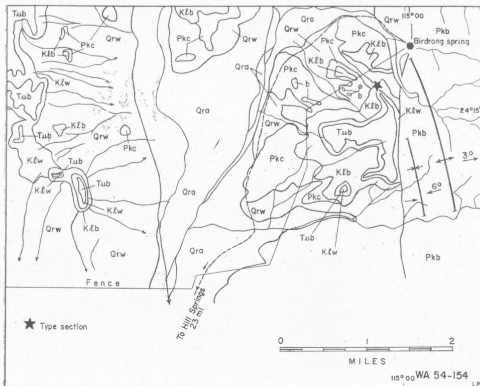
Fig. 147. Type locality, Birdrong Formation.
