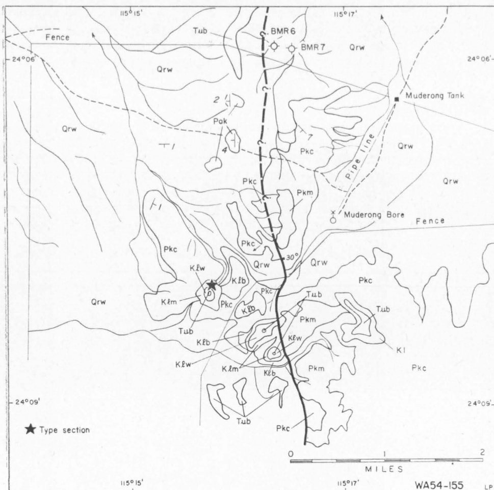
Fig. 149. Type locality, Muderong Shale.
