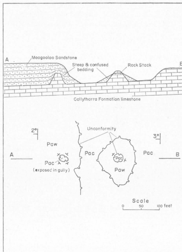
Fig. 158. Rock-stack unconformity between Callytharra Formation (Pac) and Moogooloo Sandstone (Paw).
