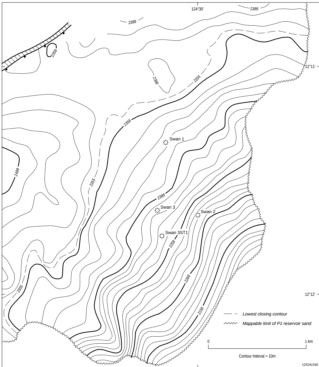
Swan, Intra Puffin Formation, depth map
