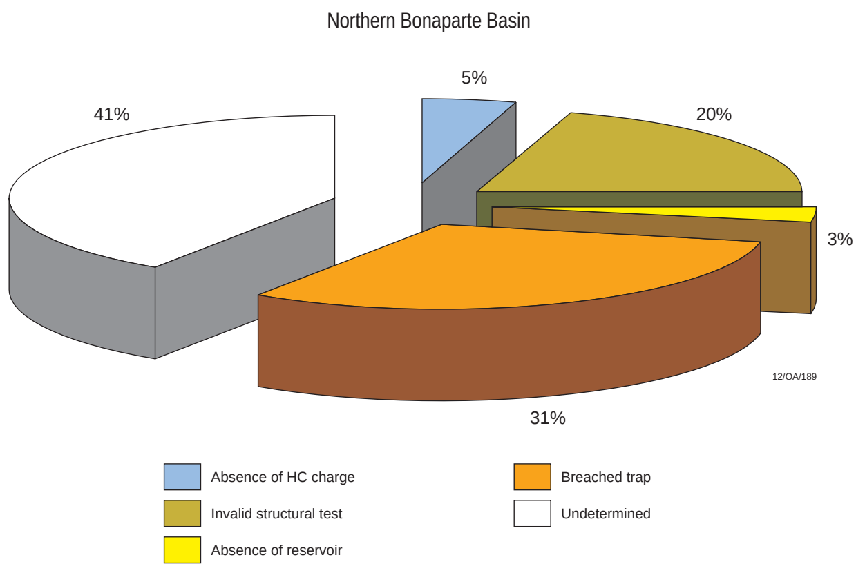
Figure 8.5 Dry hole analysis, Northern Bonaparte Basin.
