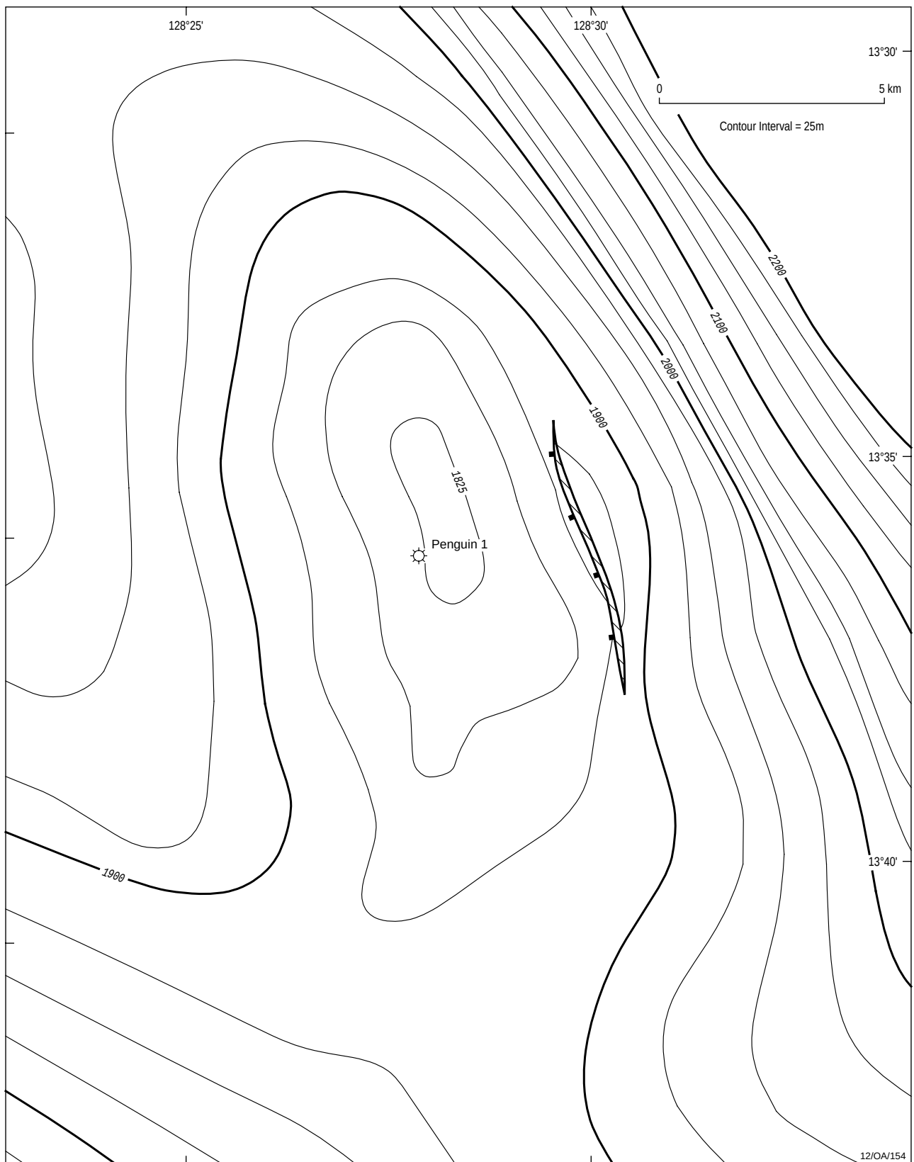
Penguin, Near Base of Upper Permian, TWT map
