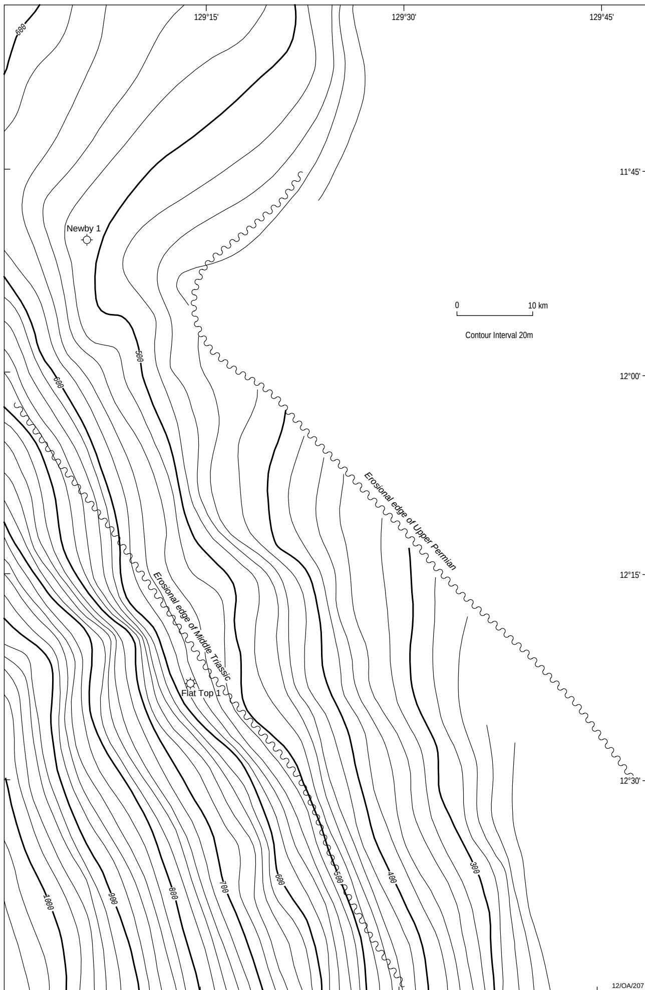
Flat Top, Near Top Permian, OWT map
