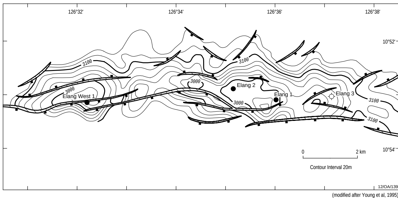
Elang, Near 'Breakup Unconformity', depth map
