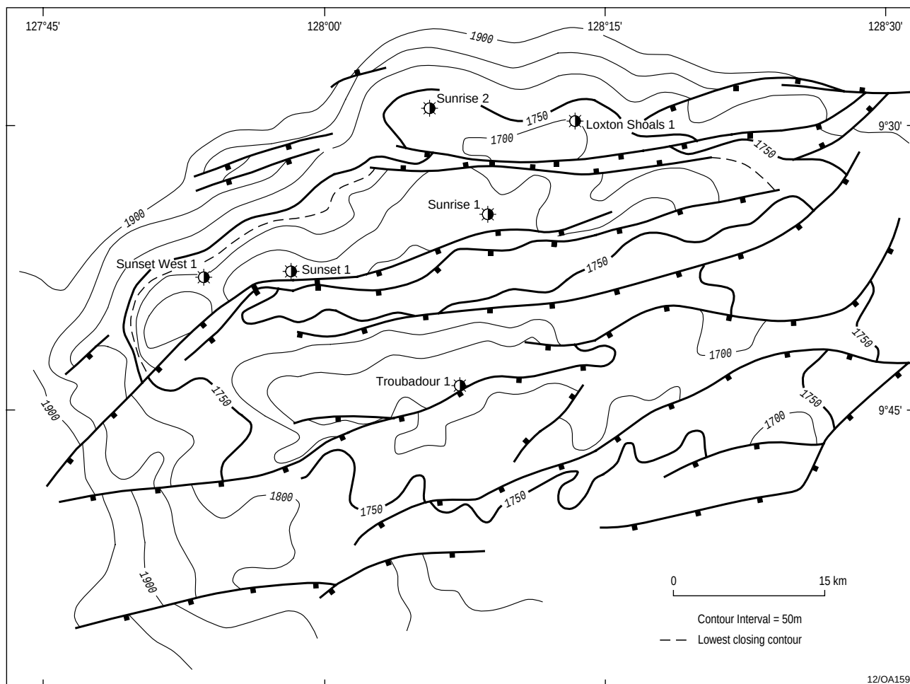
Sunset, Near Base Cretaceous, depth map
