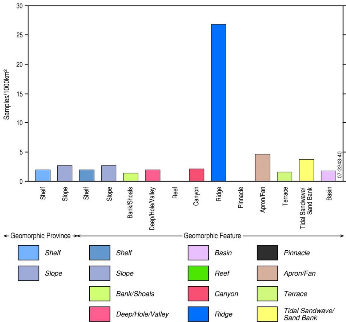
Figure 4.25. Sample densities of geomorphic provinces and features for the NNMR (y axis shows average density measured as samples per 1,000 km²).
