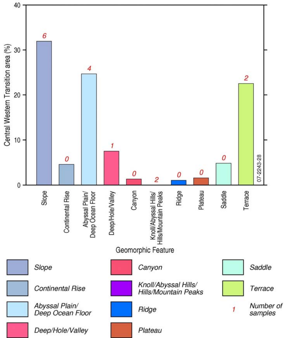
Figure 5.32. a) Geomorphology of the Central Western Transition (CWT) with location of sediment samples; and b) Percentage area of each geomorphic feature within the CWT with number of corresponding sediment samples.
