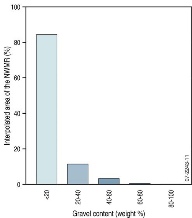
Figure 4.12. a) Gravel distribution in the NWMR and b) the area covered by each gravel class expressed as % of the interpolated area of the NWMR.
