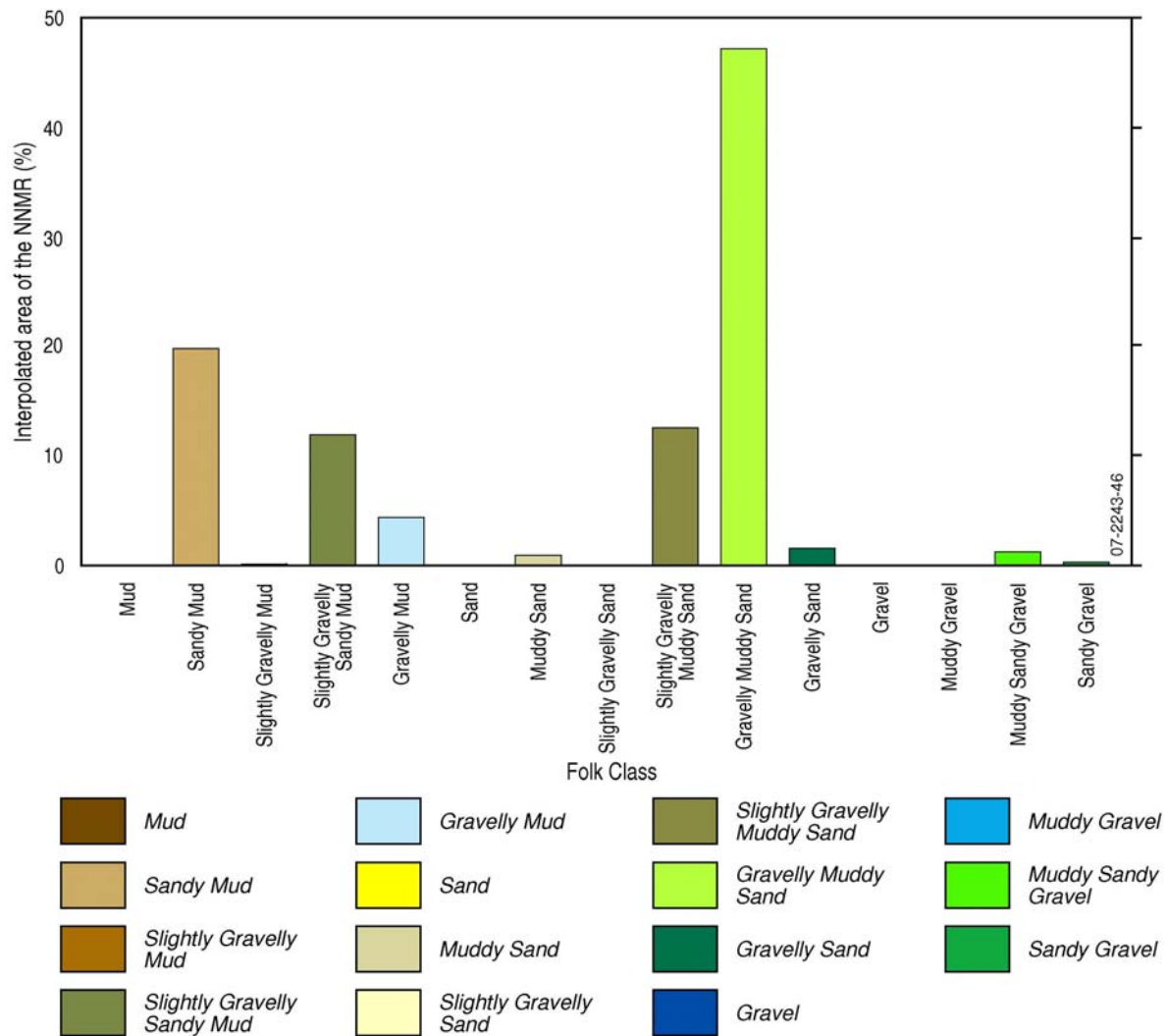
Figure 4.33. Interpolated grainsize data displayed as Folk Classes with b) the area covered by each class expressed as % of the interpolated area of the NNMR.
