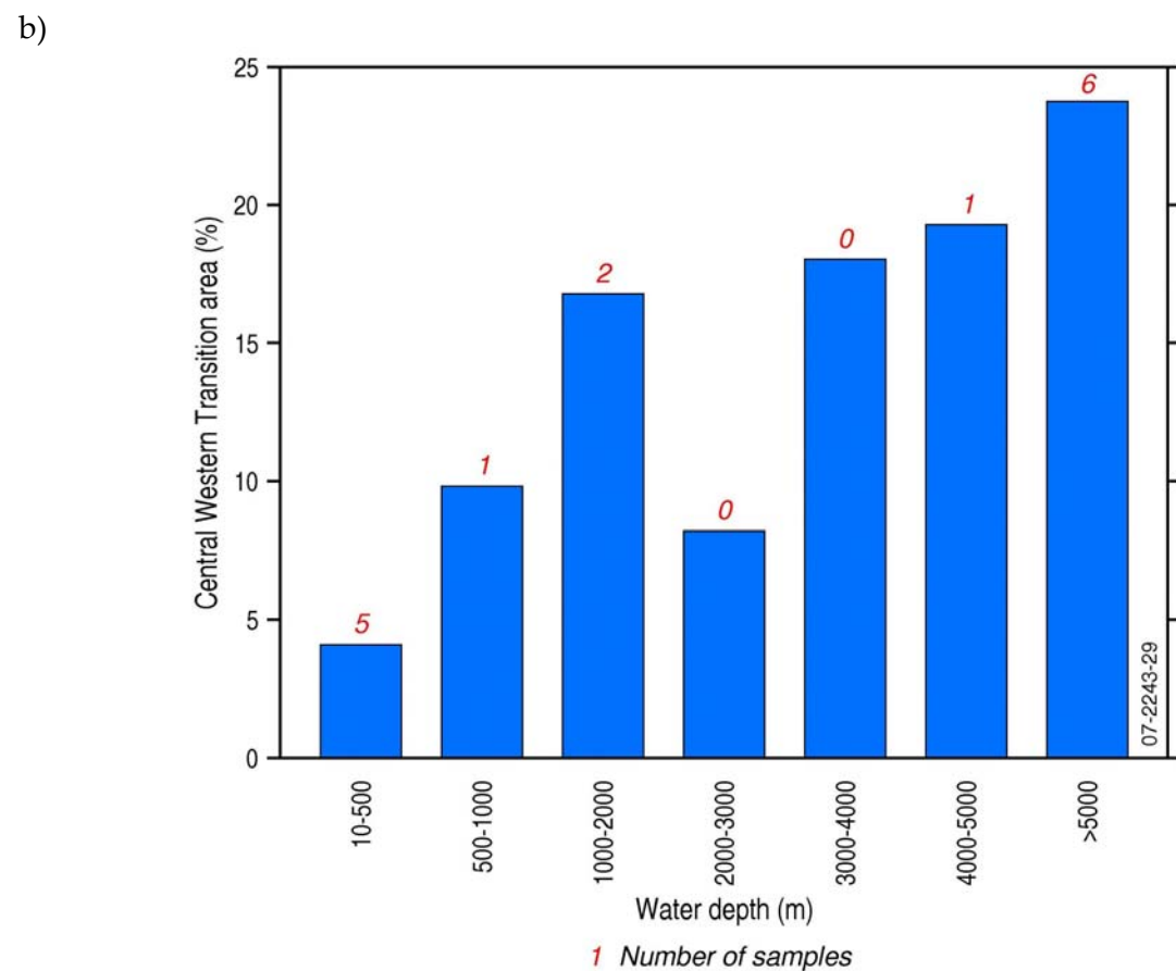
Figure 5.33. a) Bathymetry of the Central Western Transition (CWT) with location of sediment samples; and b) Percentage area of each bathymetry class within the CWT with number of corresponding sediment samples.
