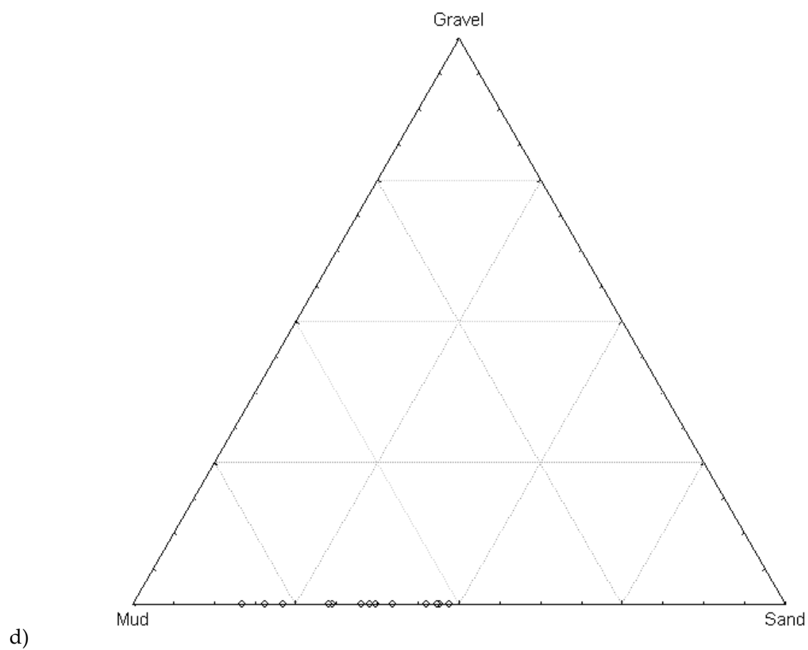
Figure 5.30. Textural composition (mud:sand:gravel ratio) of a) deep/hole/valley; and b) slope c)Trench/troughs d)Deep water plateaus sediments within the NWP.
