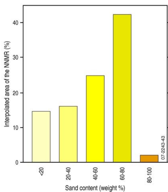
Figure 4.30. a) Sand distribution with b) the area covered by each class expressed as % of the interpolated area of the NNMR.
