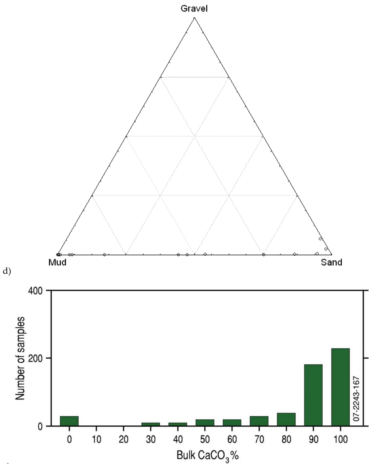
e) Figure 5.3. a) Textural composition (mud:sand:gravel ratio) of sediments in the offshore bioregions of the NWMR; a) Central Western Transition, b) Timor Province, c) Northwest Transition, d) Northwest Province, and e) Carbonate content of all the above offshore bioregion sediments in the NWMR.
