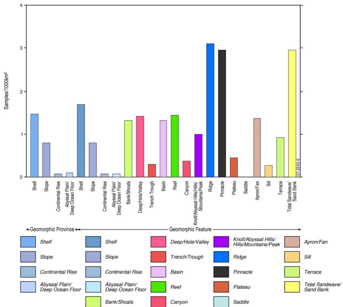
Figure 4.6. Sample density of geomorphic provinces and features in the NWMR (y axis shows average density measured as samples per 1,000 km²).
