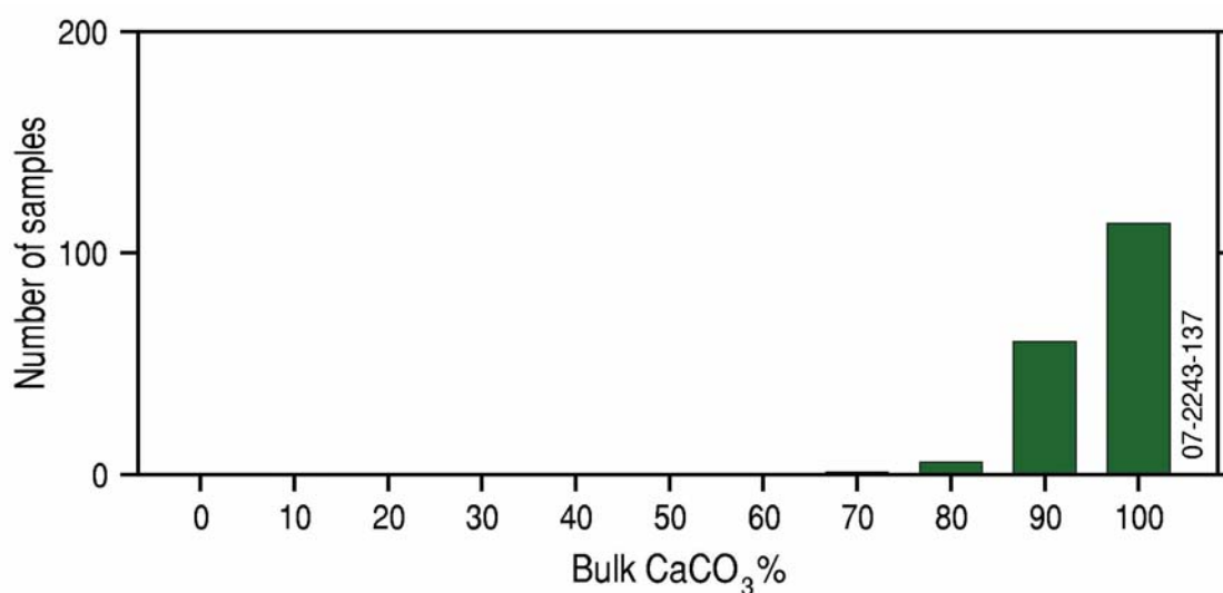
Figure 5.15. Carbonate content of a) bank/shoal; b) deep/hole/valley; c) plateau; d) ridge; e) shallow water terrace; and f) shelf/slope sediments within the NWSP.
