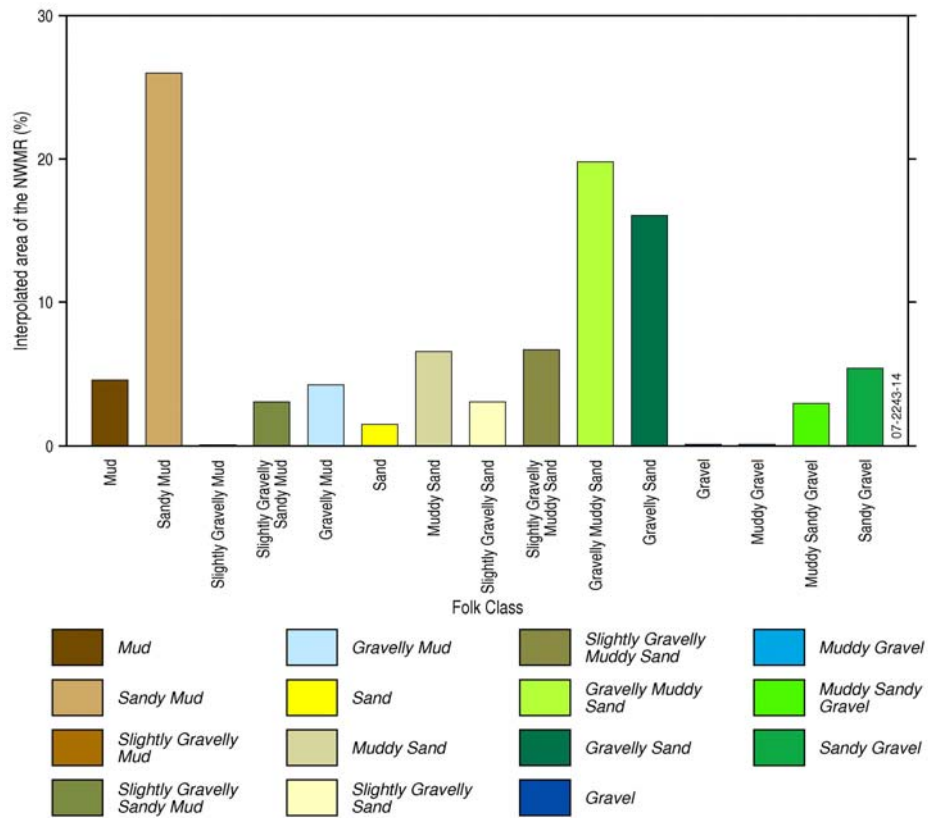
Figure 4.15. a) Interpolated grainsize data displayed as Folk Classes and b) area covered by each class expressed as % of the interpolated area of the NWMR.
