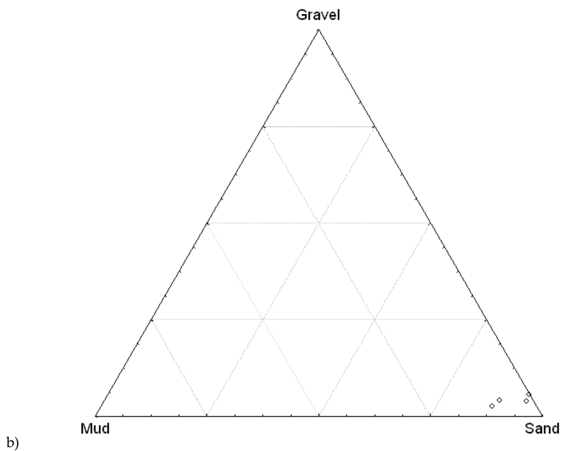
Figure 5.10. Textural composition (mud:sand:gravel ratio) of a) shelf and b) slope sediments within the CWSP.
