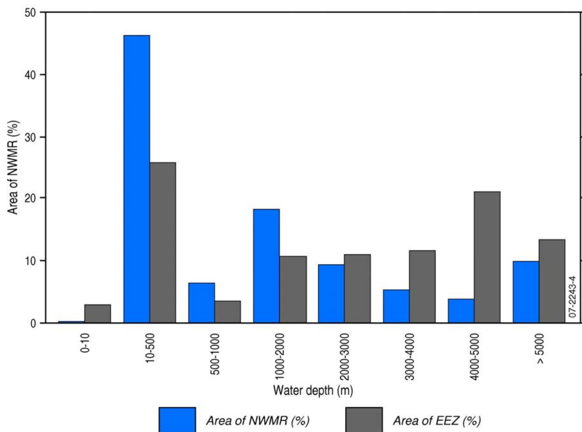
Figure 4.3. Distribution of water depths for the NWMR (blue bars) and EEZ (grey bars) expressed as percentages.
