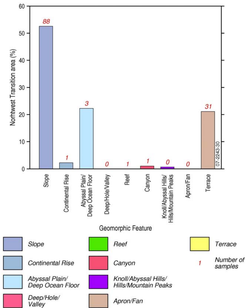
Figure 5.24. a) Geomorphology of the Northwest Transition (NWT) with location of sediment samples; and b) Percentage area of each geomorphic feature within the NWT with number of corresponding sediment samples.
