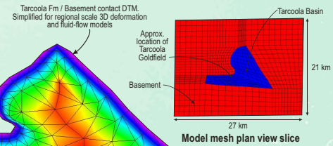
Model geometry and simplified basin architecture
