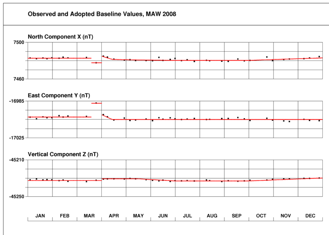
Figure 9.1. Mawson baseline plots.
