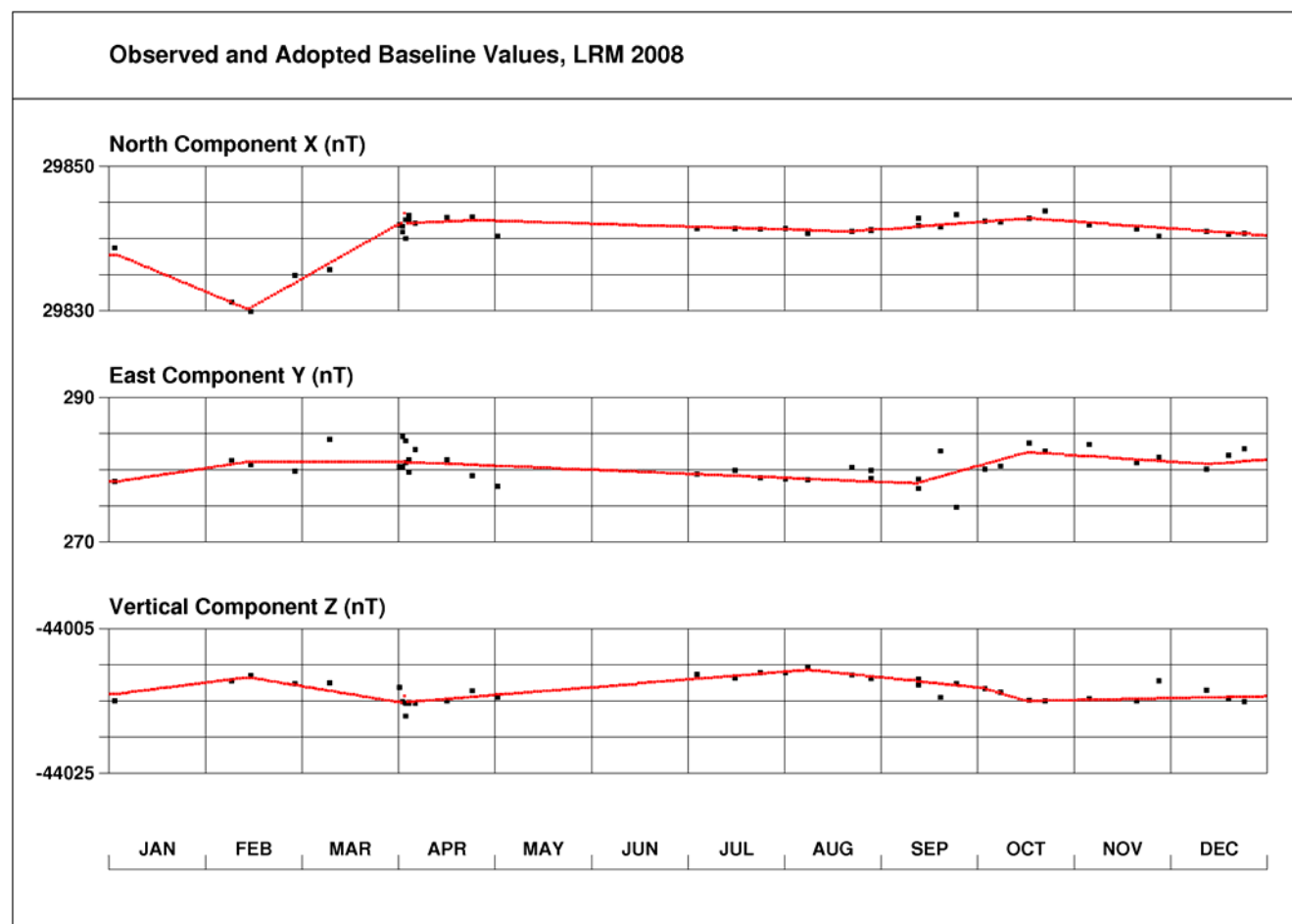
Figure 3.1. Learmonth baseline plots.
