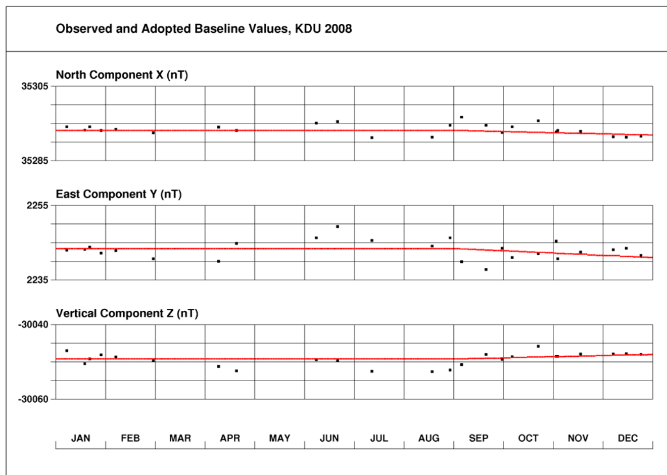
Figure 1.1. Kakadu baseline plots.
