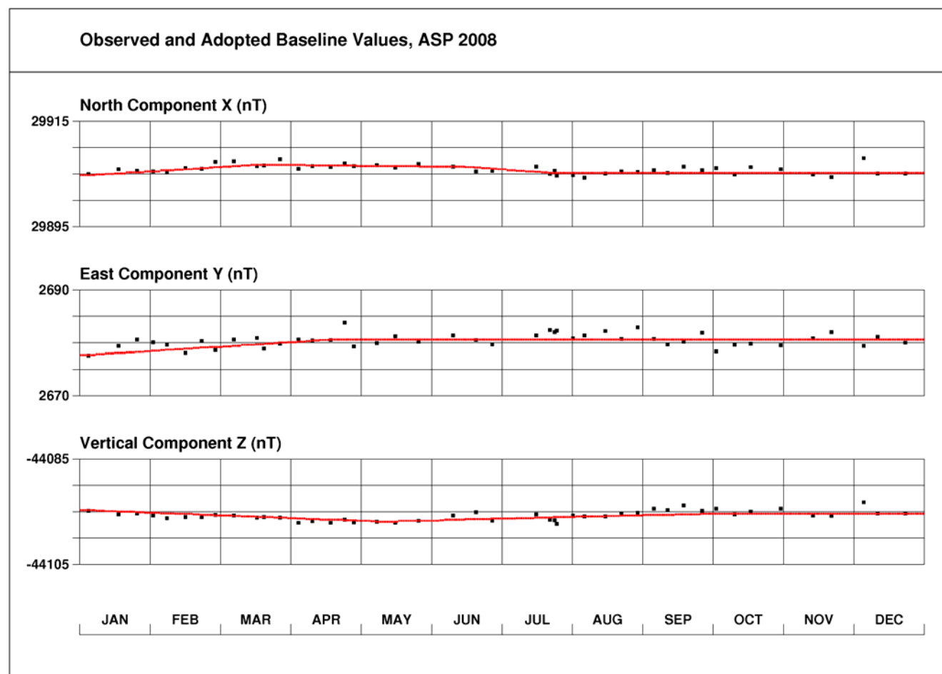
Figure 4.1. Alice Springs baseline plots.
