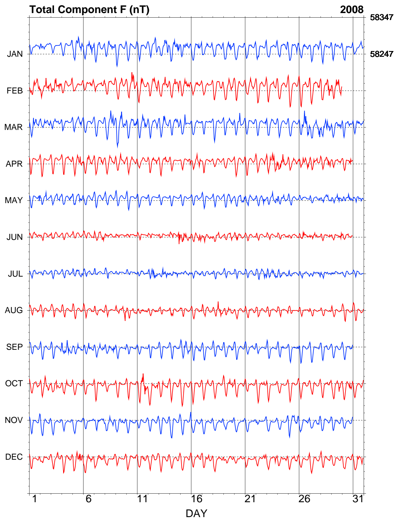
Figure 5.3. Gngara 2008 hourly mean values in X, Y, Z and F.
