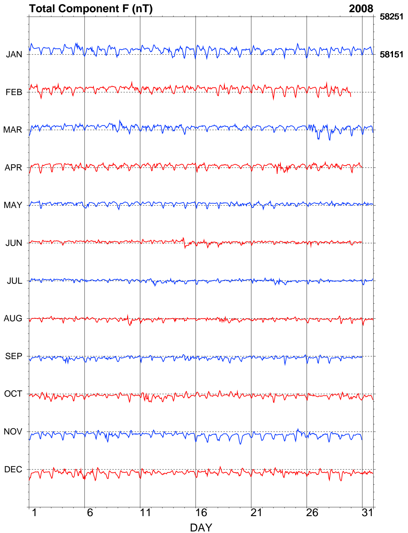
Figure 6.3. Canberra 2008 hourly mean values in X, Y, Z and F.
