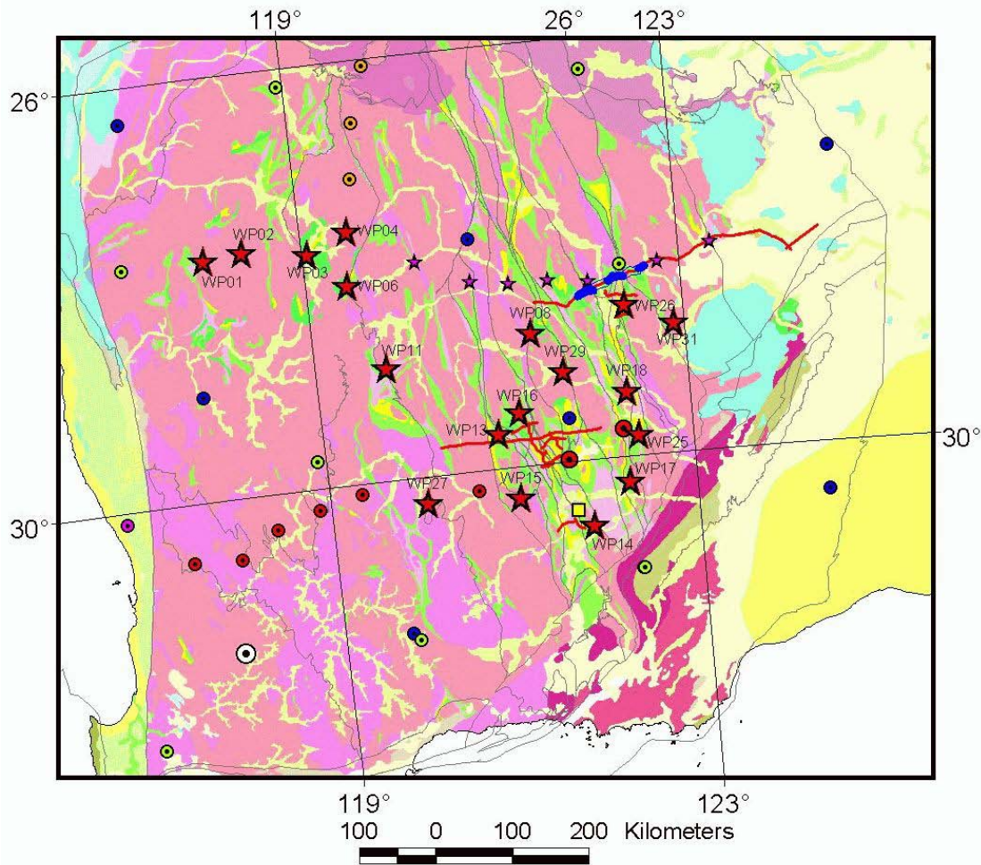
Figure 4-3: Geological map of the Yilgarn Craton showing final locations of broadband recorders (red stars). The large red stars are successful deployment sites; the small purple stars show the initial east-west deployment. Coloured dots are earlier sites used in conjunction with the purple stars to assess craton-scale velocity variation. The yellow square is the Kambalda seismological station. The blue dotted line is the position of the passive-listening experiment aimed at collecting wide-angle reflection data (see later).
