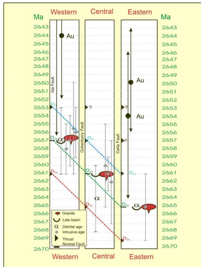
Figure 8-4: ‘ D_2 ’ orogenesis time lines across the EYC. Published ages for direct gold from Brown et al. (2002), Veilricher et al. (2003) and Salier et al. (2004). ‘ D_2 ’ ages young diachronously to the west (SW). Syn-gold ages overlap the last stages of ‘ D_{2b} ’ contraction.
