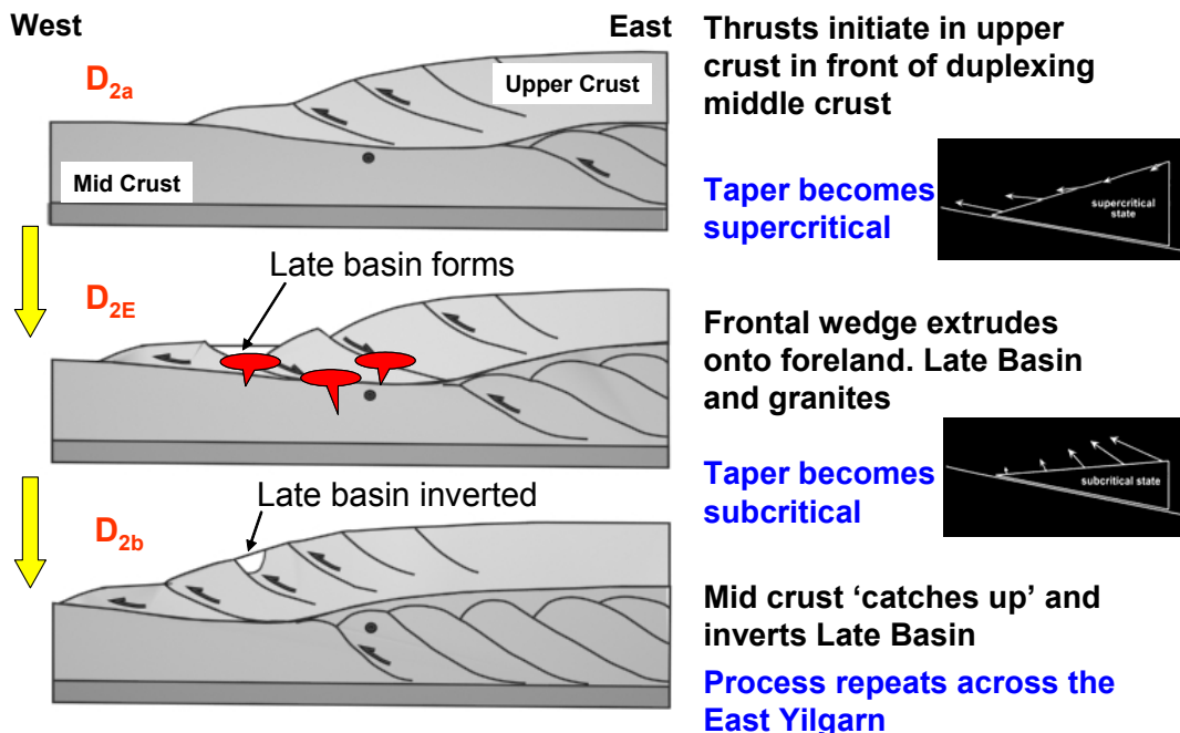
Figure 8-5: A schematic diagram illustrating the surging of the foreland above a duplexing mid-crust. During the surge, localised extension occurs on previous thrusts and permits mafic-type granite intrusion and space for Late Basins to be deposited. The mid crust “catches up” with the upper crust and inverts the basins and reactivates faults as thrusts. The process repeats across the EYC. Deep fluids are driven from below and behind the upper crust which is out of phase with the mid crust. This means that orogenic gold will occur late in the cycle in a pre-prepared upper-crustal architecture.
