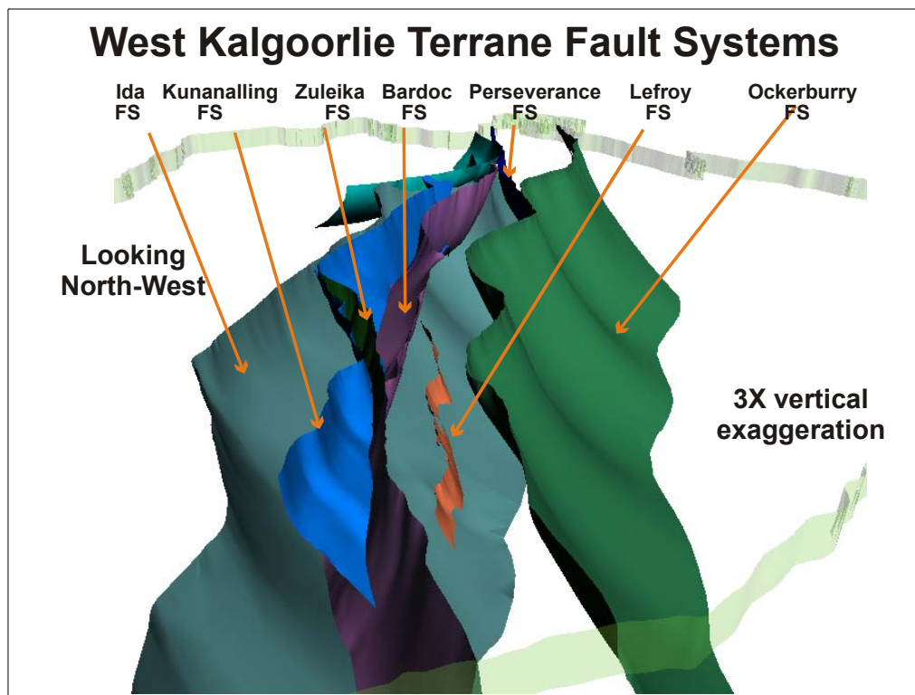
Figure 1-36: 3D interpretation of the terrane- and domain-bounding fault systems of the western part of the Kalgoorlie Terrane.
