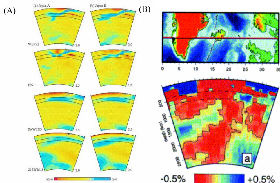
Figure 8-2: (A) The fast velocity structure associated with the subduction of the Pacific plate beneath the Japanese arc (Fukao et al., 2001); (B) Cross section through the model of Bijwaard et al. (2004) showing a large plume-shaped anomaly (with respect to reference model ak135 [Kennett et al., 1995]) in the mantle below Iceland. A 0.15% velocity contour is indicated in black for clarity. The separate layers are well-resolved in the lower mantle, but less well-resolved in the upper mantle. Dashed lines indicate the 410 and 660 km discontinuities.
