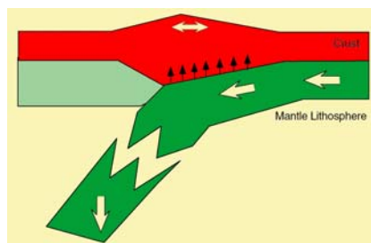
Figure 8-3: Five alternative models for switching between contraction and extension. Models include channel flow, underplating with wedge extension, slab roll back, post-orogenic collapse, and slab break off. Difficulties with these alternative models include: the likely flat subduction in the Archaean, the wide orogen, the whole crust is involved, the rapid and diachronous switches, and the few high-pressure rocks exposed.
