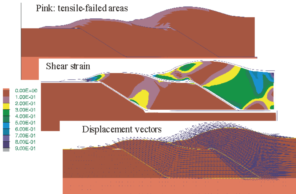
Figure 8-17: Final deformation features of the thrusting slabs. a) Failure patterns. b) Shear strain contours. c) Displacement vectors.
