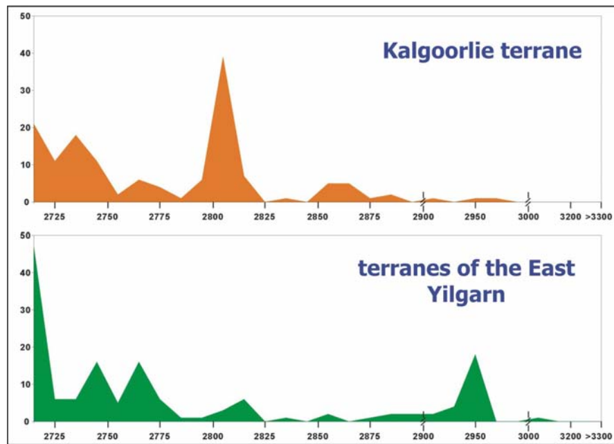
Figure 1-6: Histogram of zircon inheritance ages for plutonic rocks of the EYC (modified from Cassidy and Champion, 2004).
