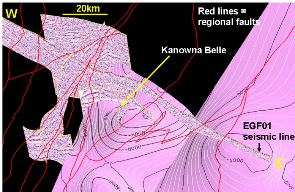
Figure 8-61: Screen capture from Gocad displaying a series of seismic reflection lines (purple and white surfaces) in the Kanowna Belle region. The pink surfaces are domical structures interpreted from seismic reflections.
