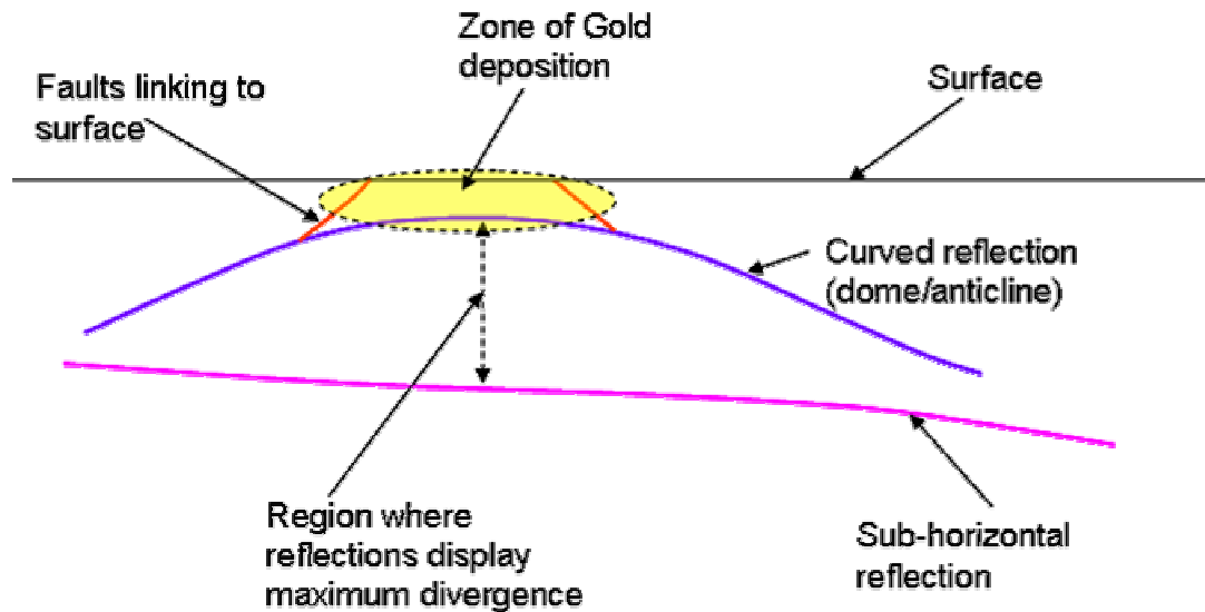
Figure 8-70: Schematic diagram of diverging reflectors and structures associated with gold deposition (see seismic data in Figures 8-71 and 8-72). Gold deposits are located above the region of maximum divergence. Is the location of gold here related to crustal level and/or the geometry of the dome and underlying sub-horizontal reflector?
