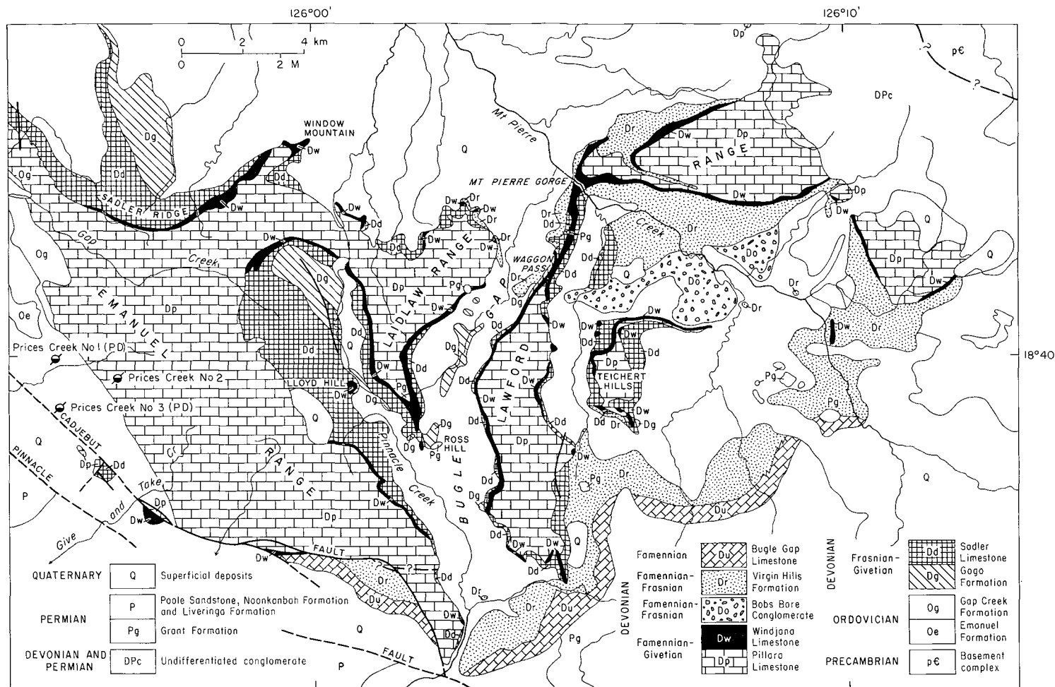
Fig. 28. Geology of the Laidlaw Range, Emanuel Range and Lawford Range Area — Canning Basin.
