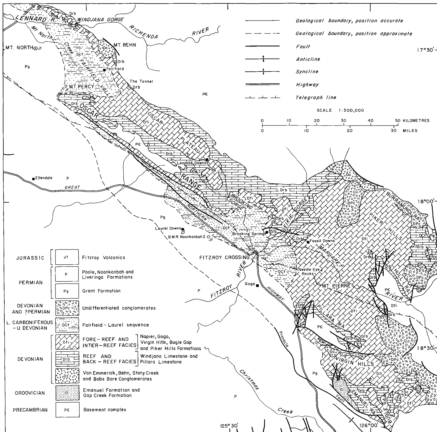
Fig. 27. Map of the solid geology of the Northern Canning Basin.
