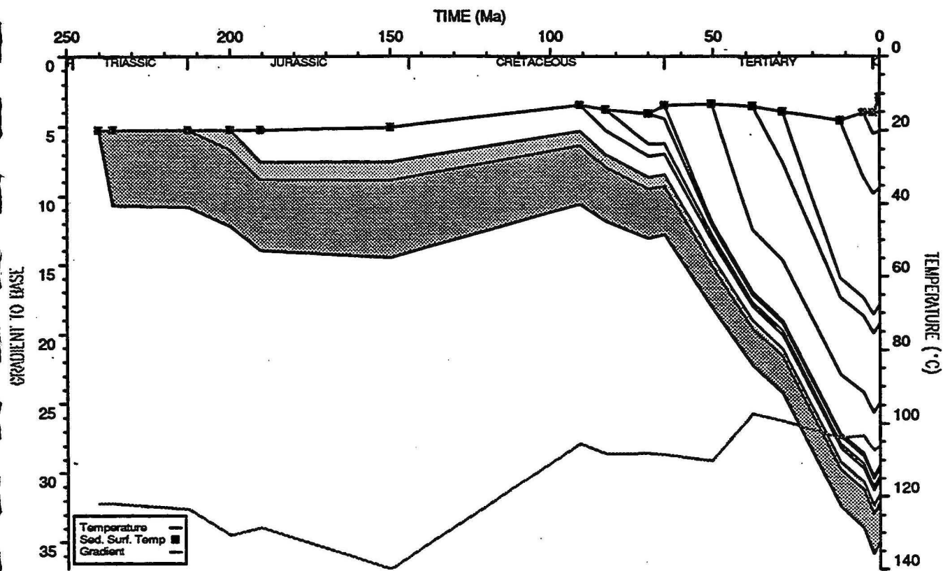
BED TEMPERATURE PLOT : North Scott Reef 1
