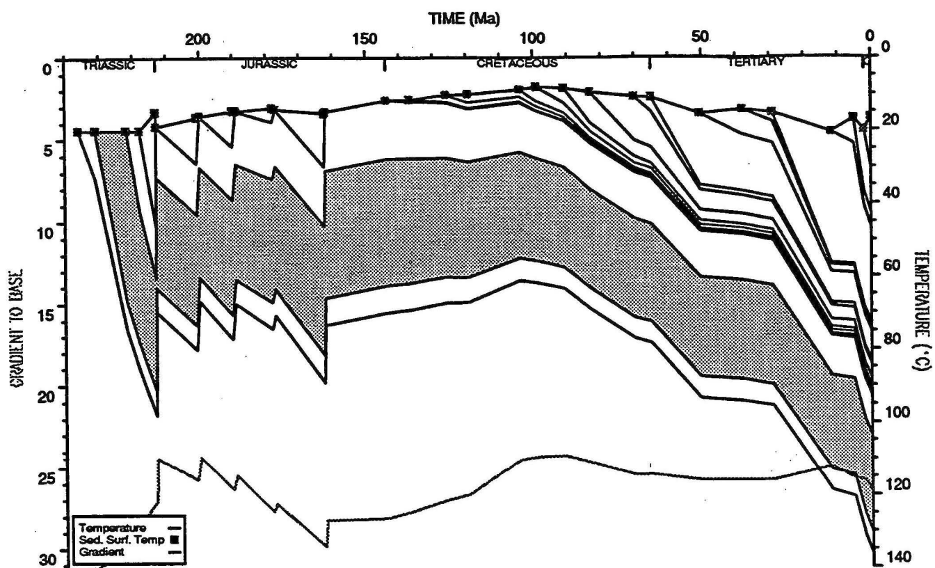
BED TEMPERATURE PLOT : Goodwyn 6
