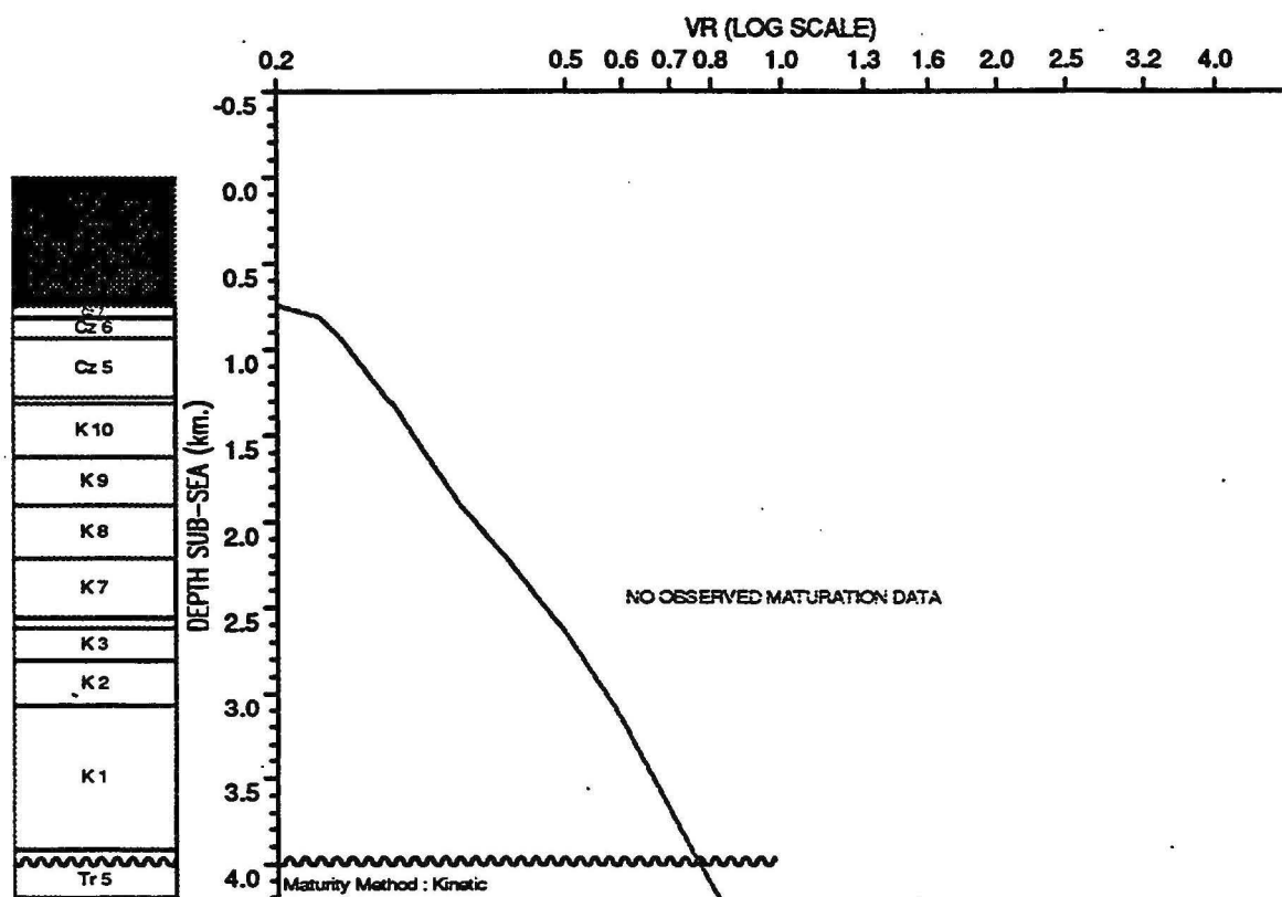
OBSERVED vs COMPUTED MATURITY PLOT : Zeepaard 1
