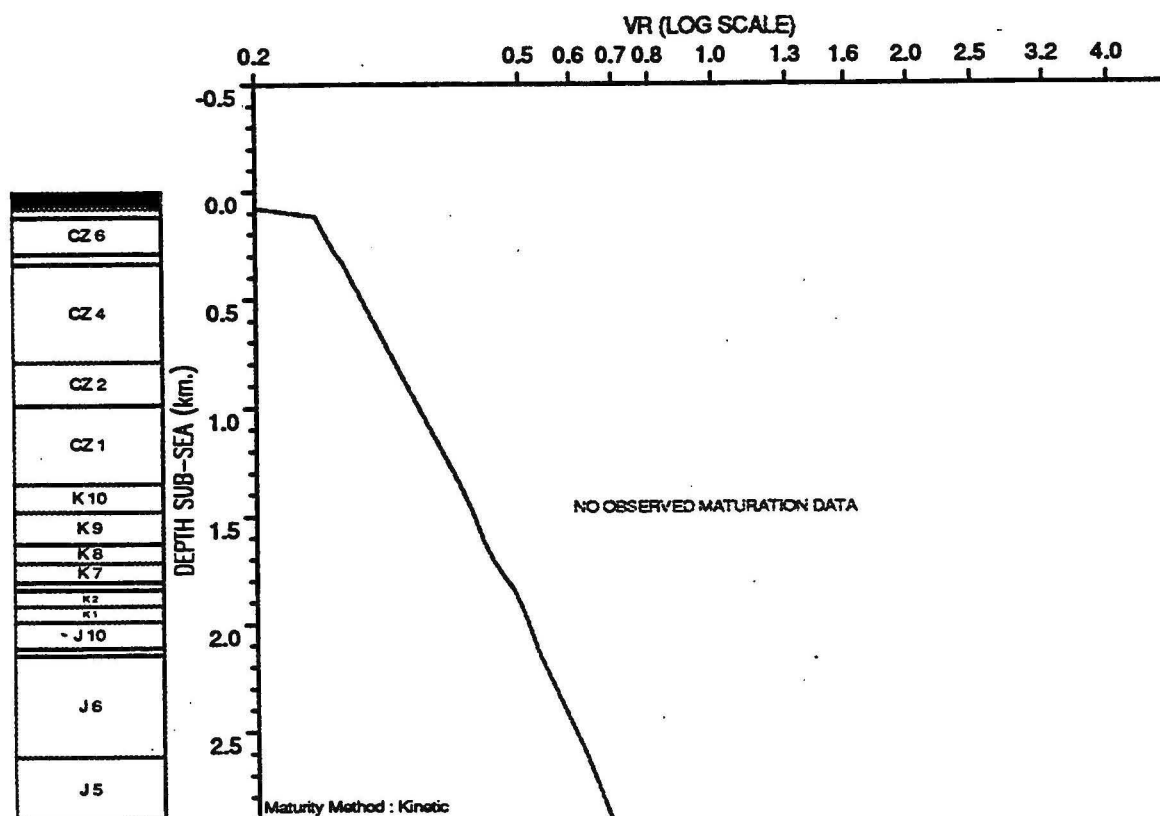
OBSERVED vs COMPUTED MATURITY PLOT : Talisman 1
