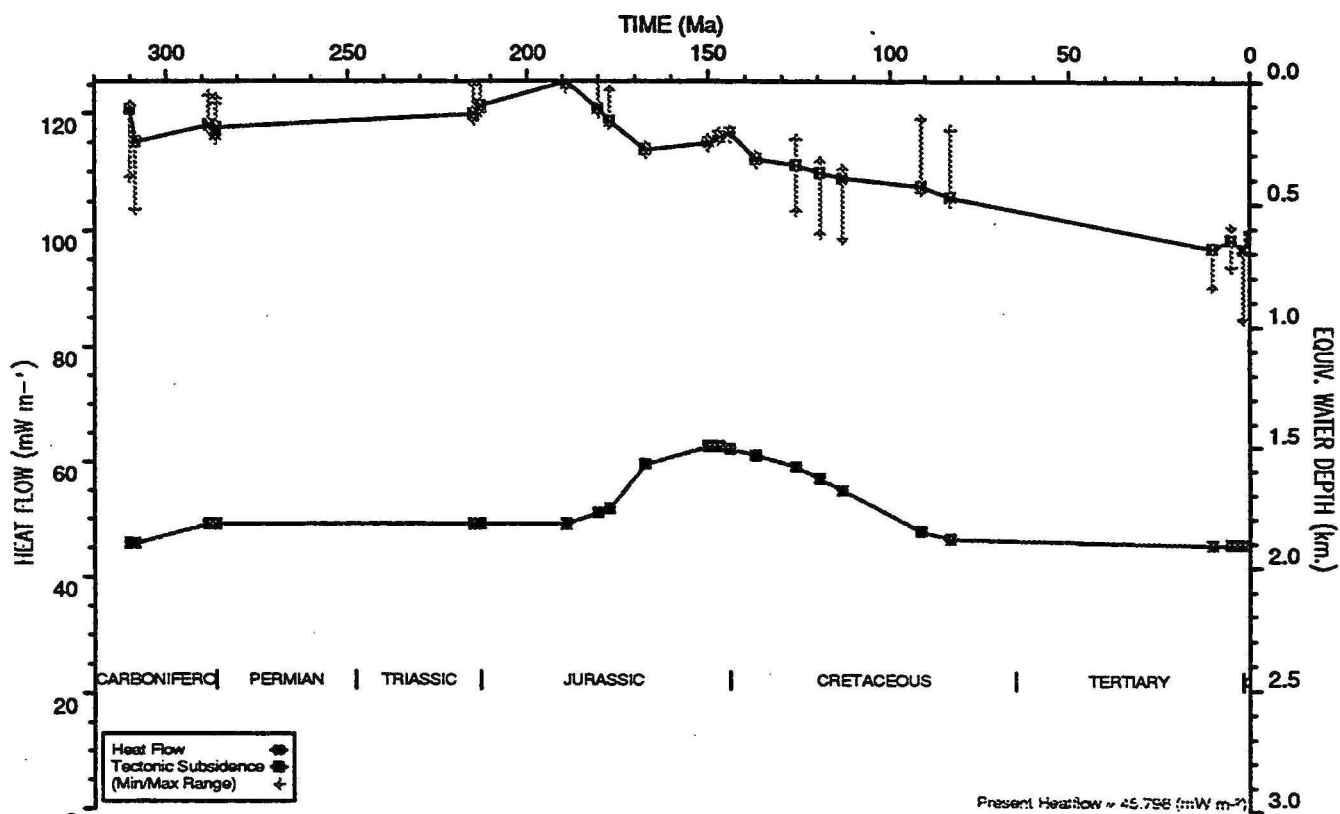
HEATFLOW AND TECTONIC SUBSIDENCE PLOT : Lapeche 1A
