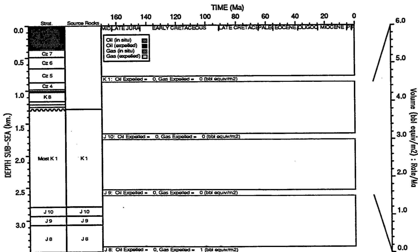
HYDROCARBON GENERATION PLOT : Novara 1
