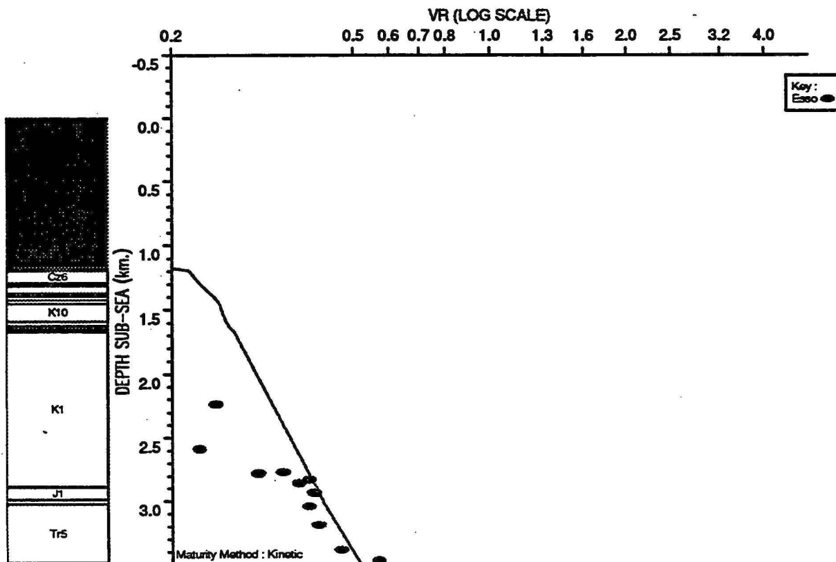
OBSERVED vs COMPUTED MATURITY PLOT : Sirius 1
