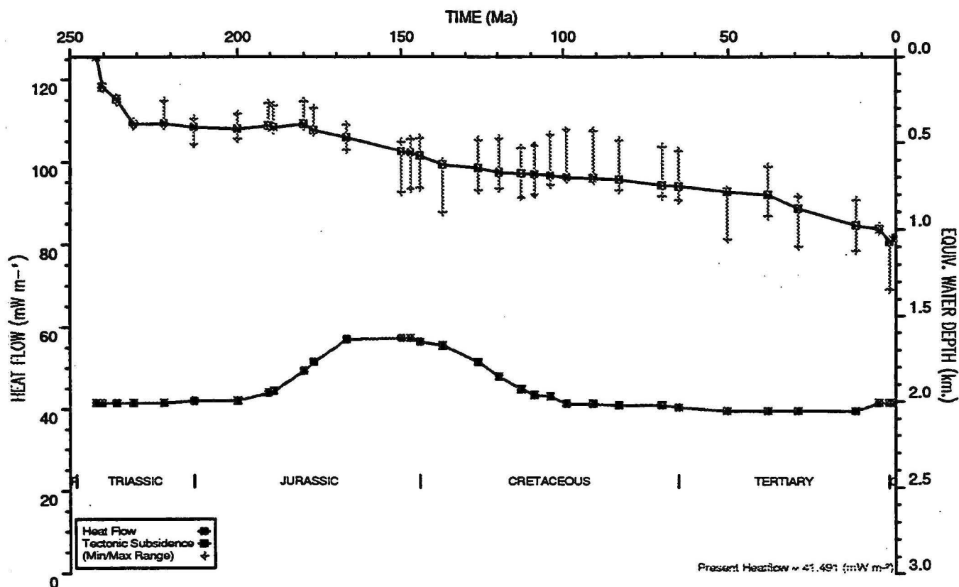
HEATFLOW AND TECTONIC SUBSIDENCE PLOT : Keraudren 1
