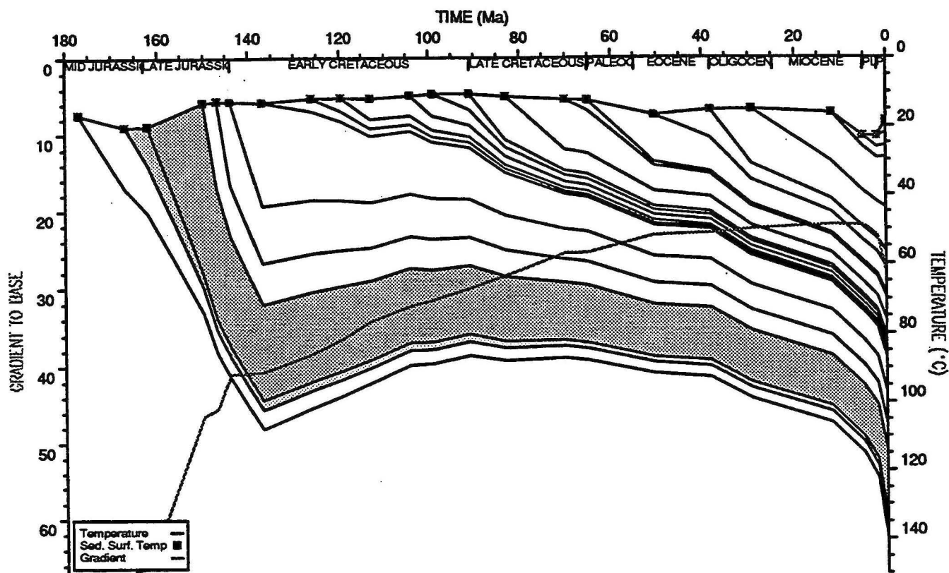
BED TEMPERATURE PLOT : Madeleine 1
