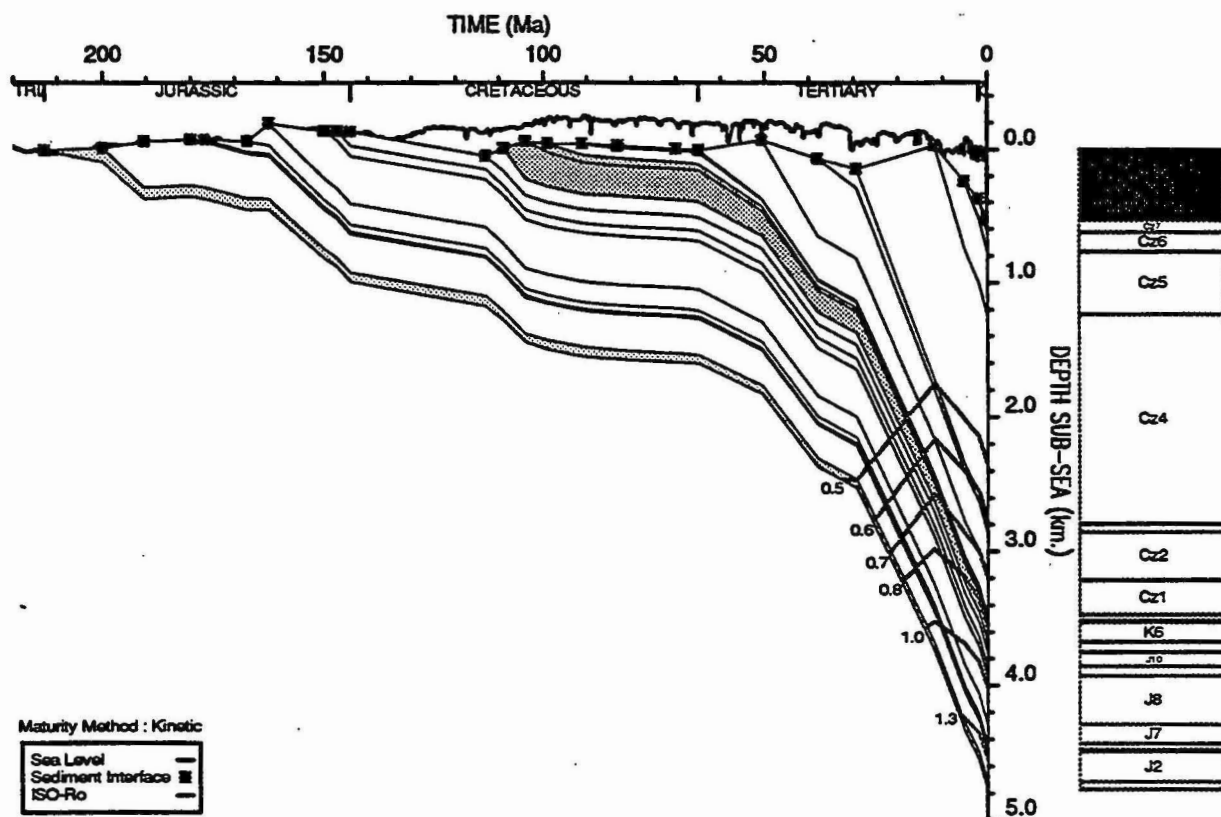
GEOHISTORY PLOT : Buffon 1
