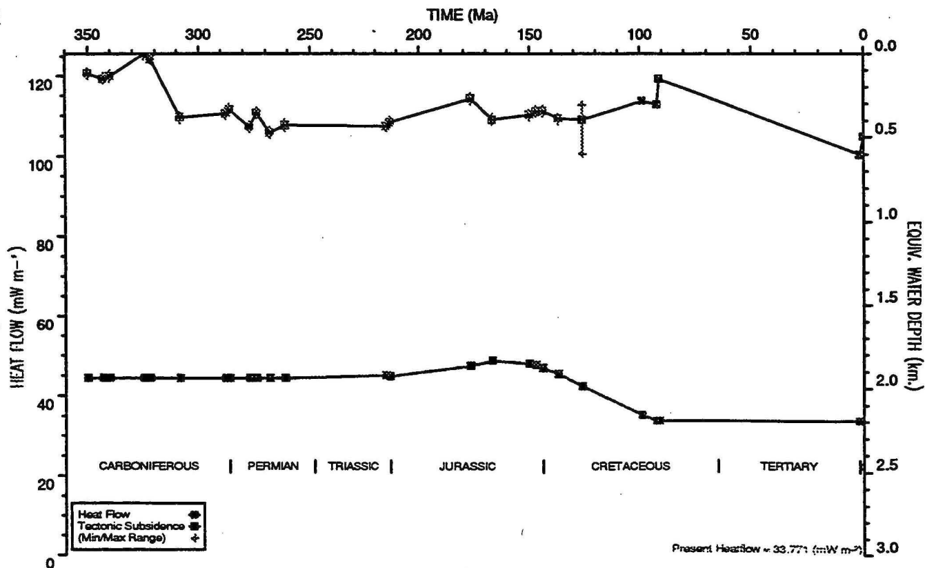
HEATFLOW AND TECTONIC SUBSIDENCE PLOT : Pearl 1
