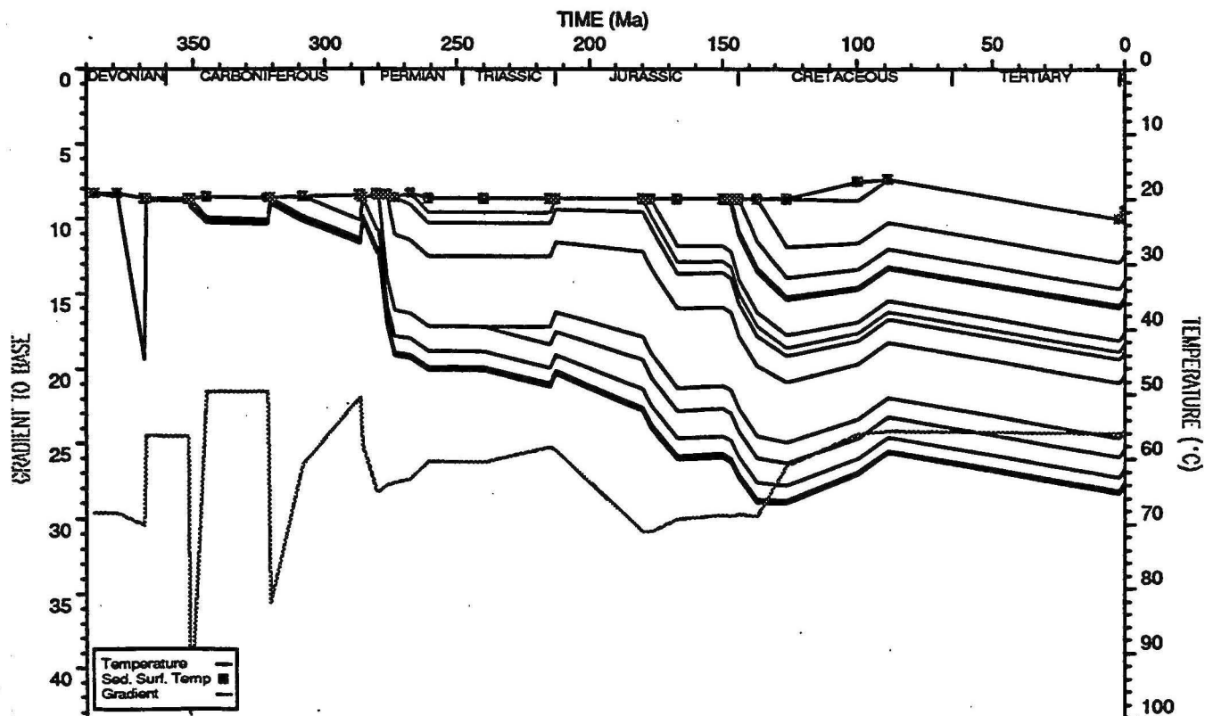
BED TEMPERATURE PLOT : Perindi 1
