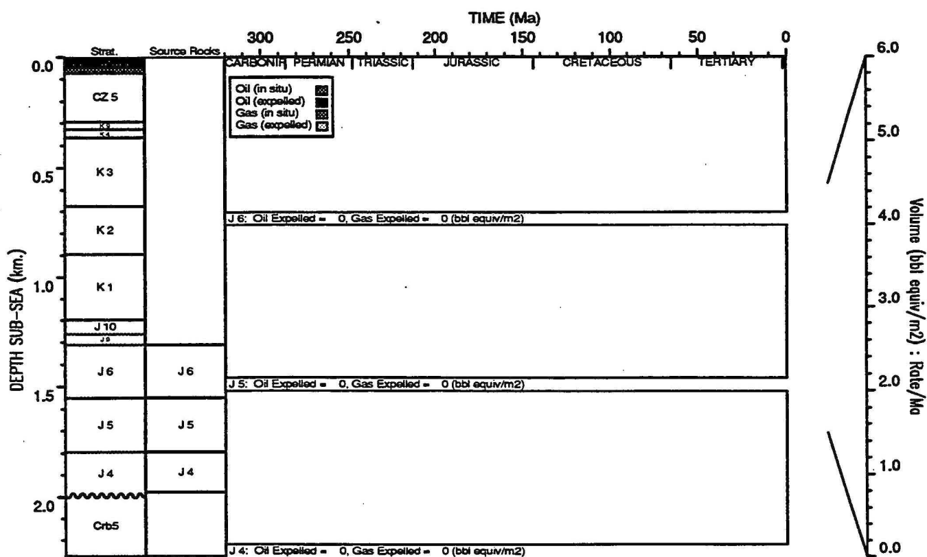
HYDROCARBON GENERATION PLOT : Lacedpede 1A
