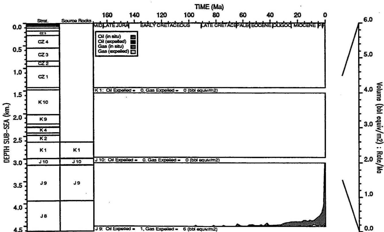
HYDROCARBON GENERATION PLOT : Withnell 1
