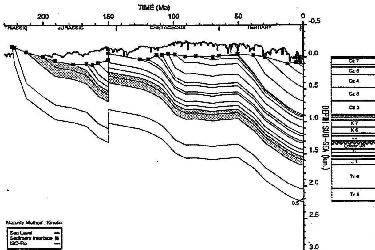
GEOHISTORY PLOT : Leatherback 1
