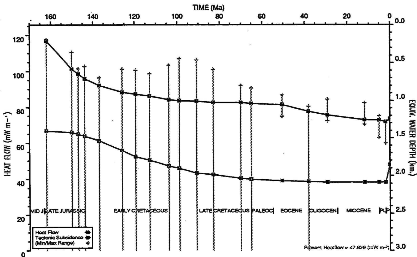
HEATFLOW AND TECTONIC SUBSIDENCE PLOT : Withnell 1
