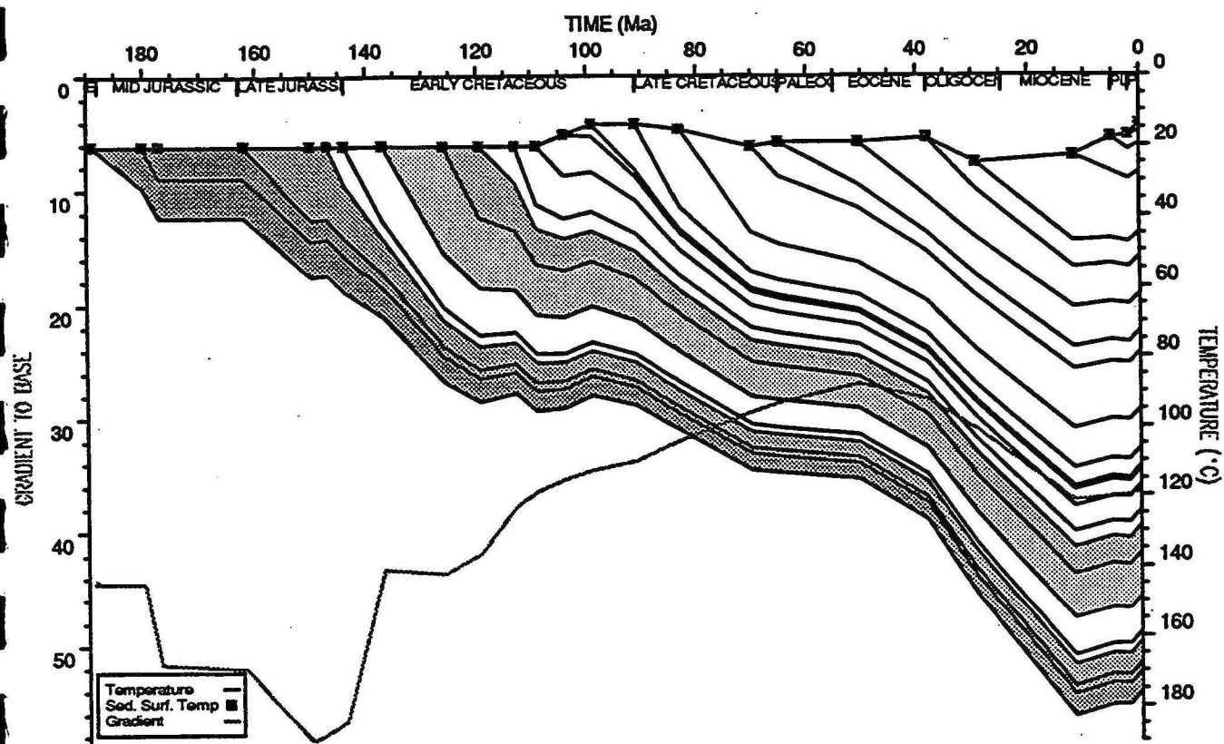
BED TEMPERATURE PLOT : Brewster 1A
