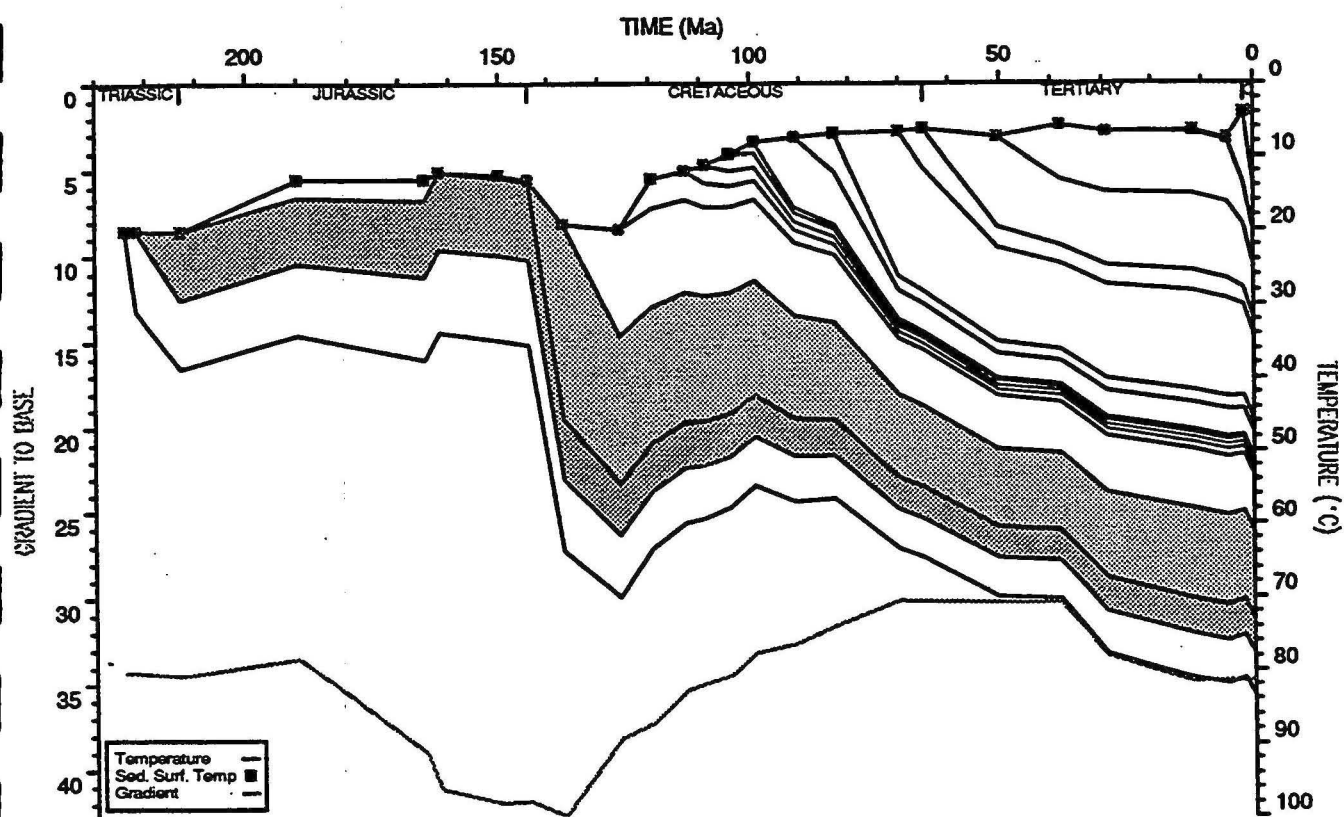
BED TEMPERATURE PLOT : Zeewulf 1
