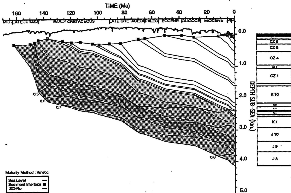
GEOHISTORY PLOT : Dampier 1
