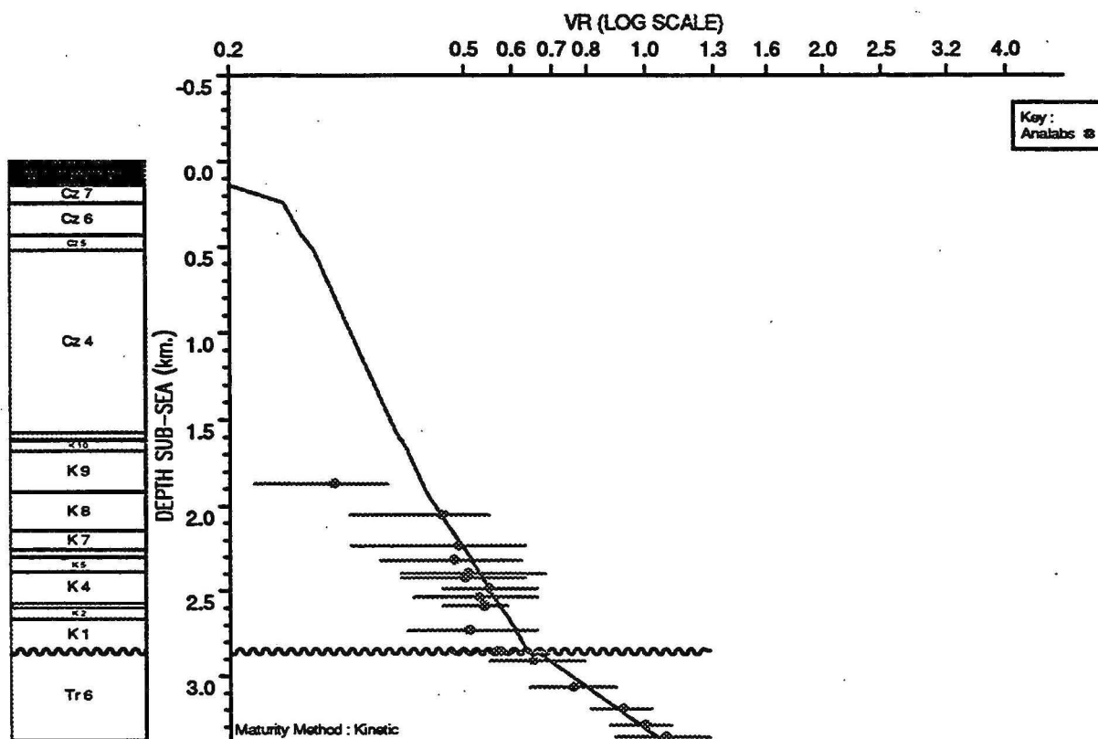
OBSERVED vs COMPUTED MATURITY PLOT : Griffin 1
