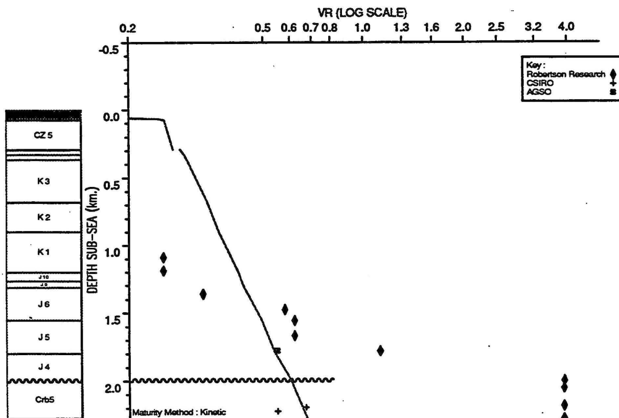
OBSERVED vs COMPUTED MATURITY PLOT : Lacedpede 1A
