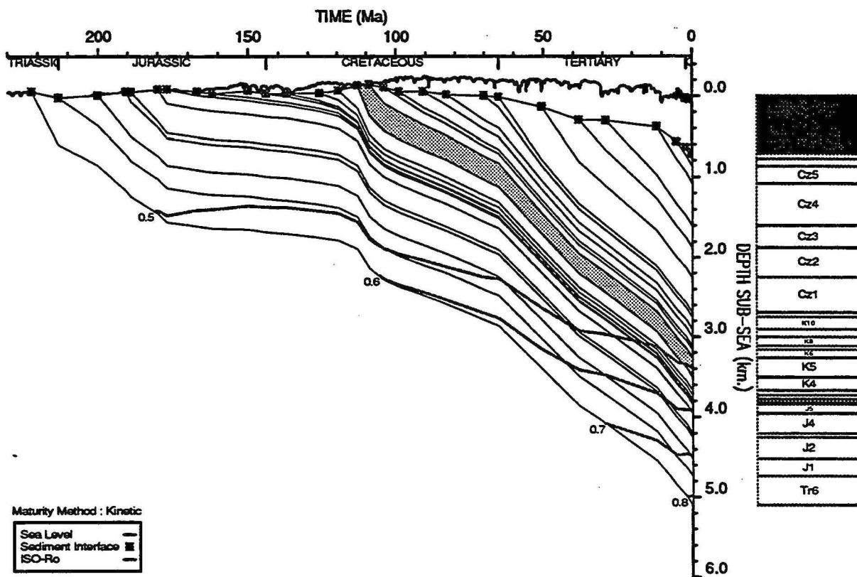
GEOHISTORY PLOT : Barcoo 1
