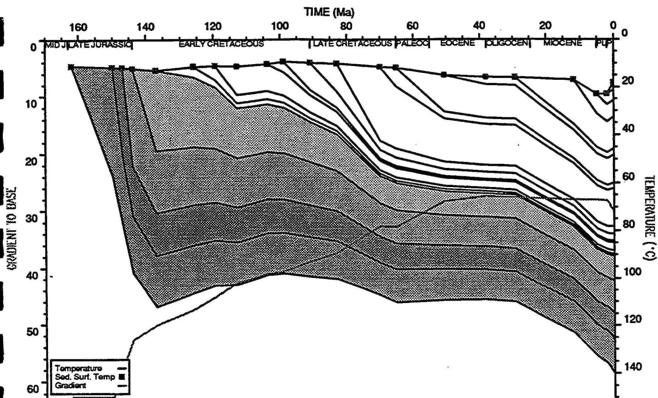
BED TEMPERATURE PLOT : Dampier 1
