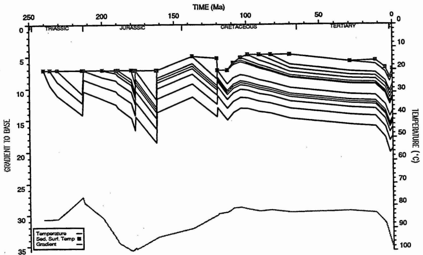
BED TEMPERATURE PLOT : Strickland 1
