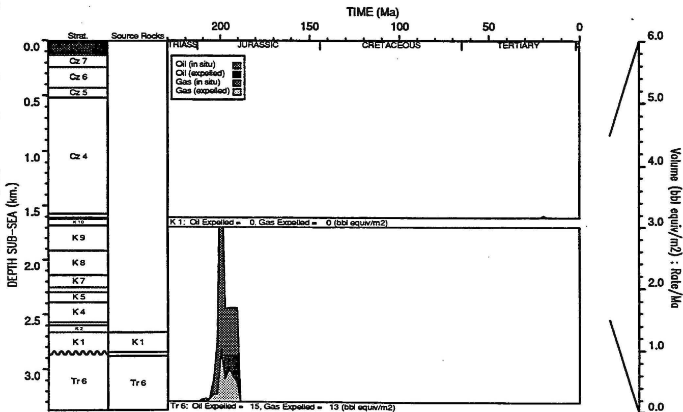
HYDROCARBON GENERATION PLOT : Griffin 1
