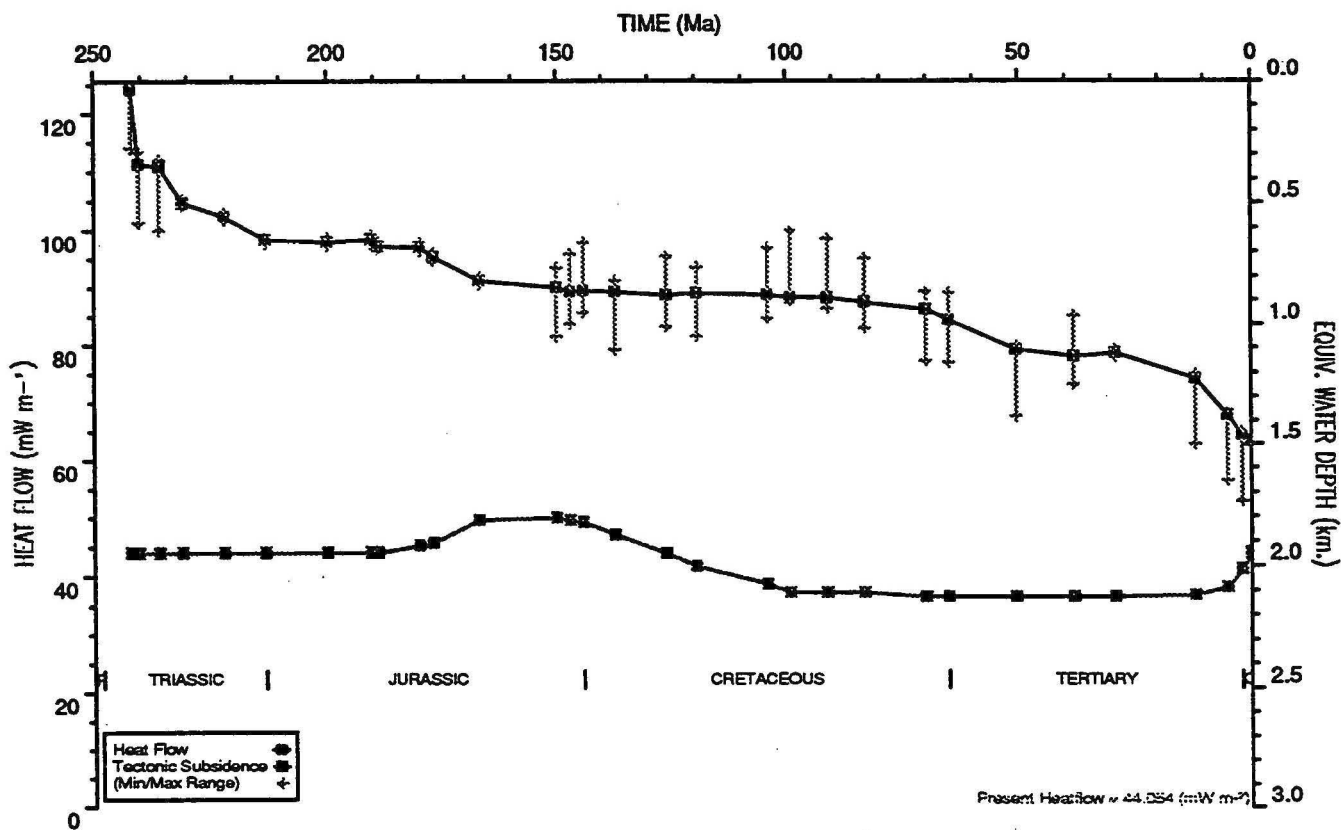
HEATFLOW AND TECTONIC SUBSIDENCE PLOT : Phoenix 1
