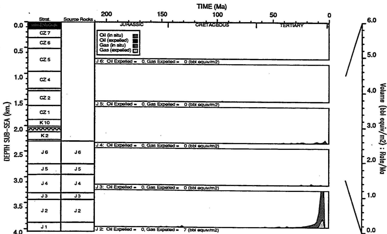
HYDROCARBON GENERATION PLOT : Picard 1
