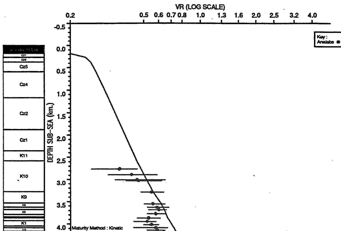
OBSERVED vs COMPUTED MATURITY PLOT : Discorbis 1
