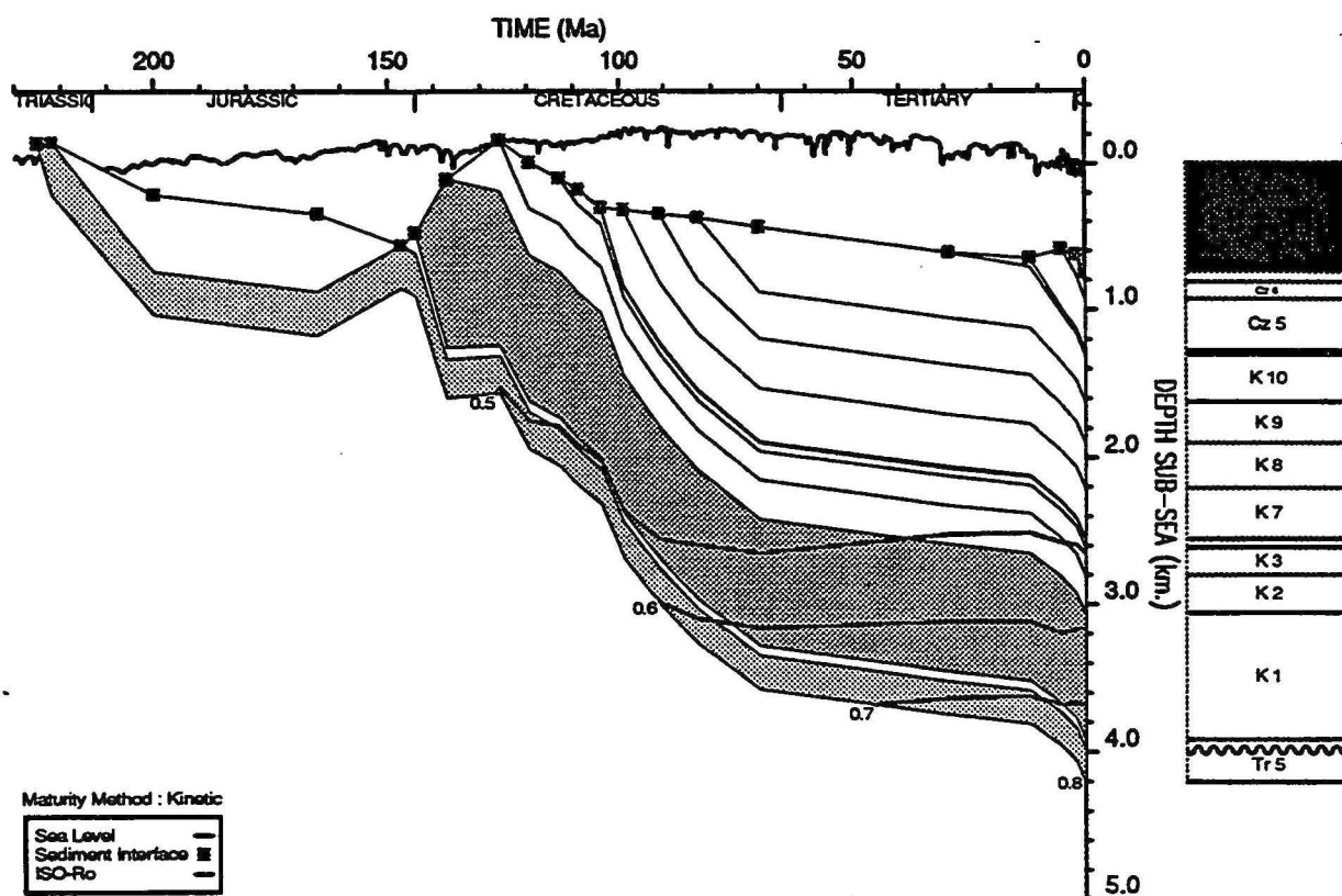
GEOHISTORY PLOT : Zeepaard 1
