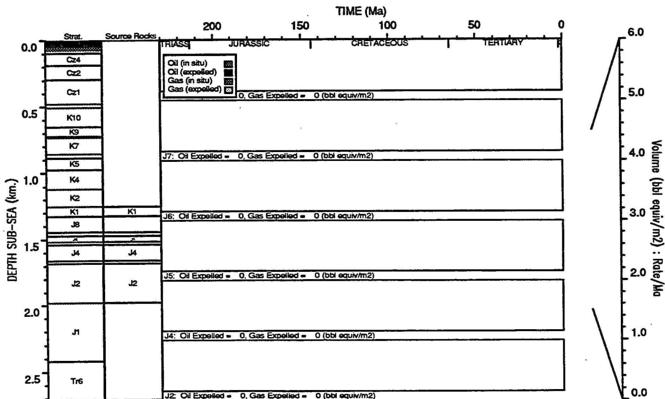
HYDROCARBON GENERATION PLOT : Lynher 1
