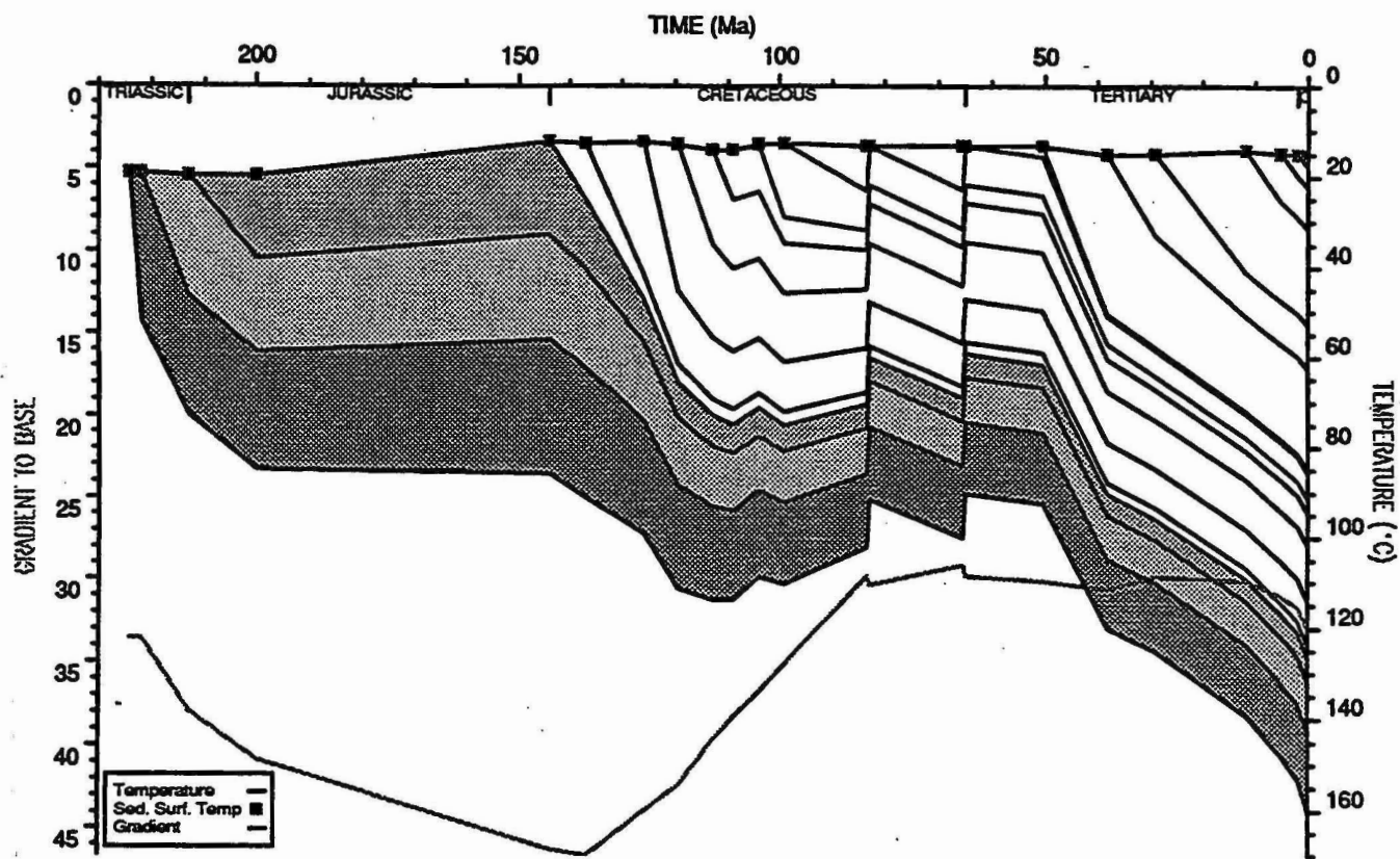
BED TEMPERATURE PLOT : Bluebell 1
