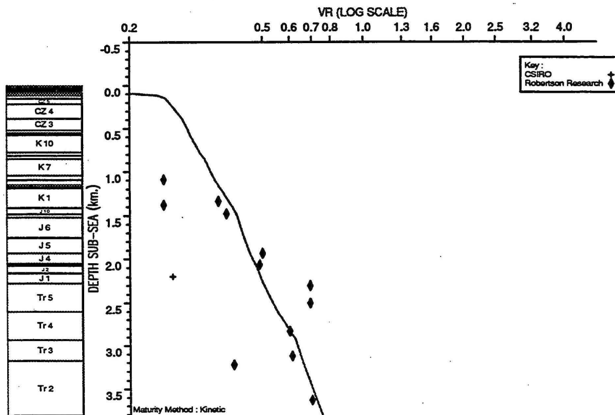
OBSERVED vs COMPUTED MATURITY PLOT : Keraudren 1
