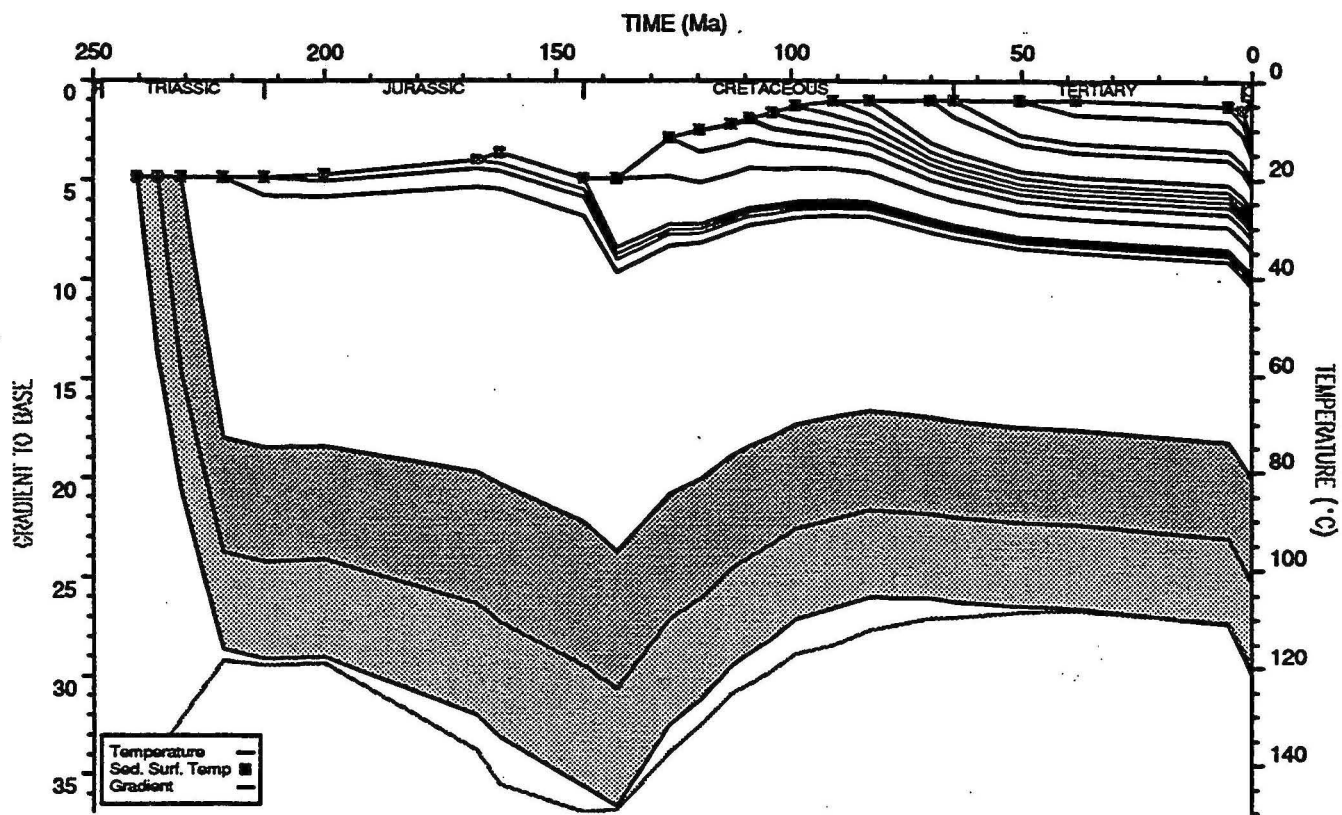
BED TEMPERATURE PLOT : Jupiter 1
