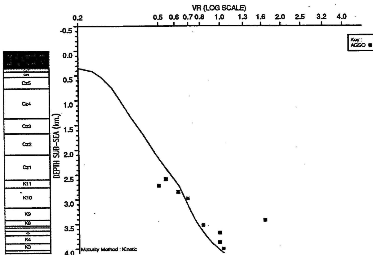
OBSERVED vs COMPUTED MATURITY PLOT : Caswell 1
