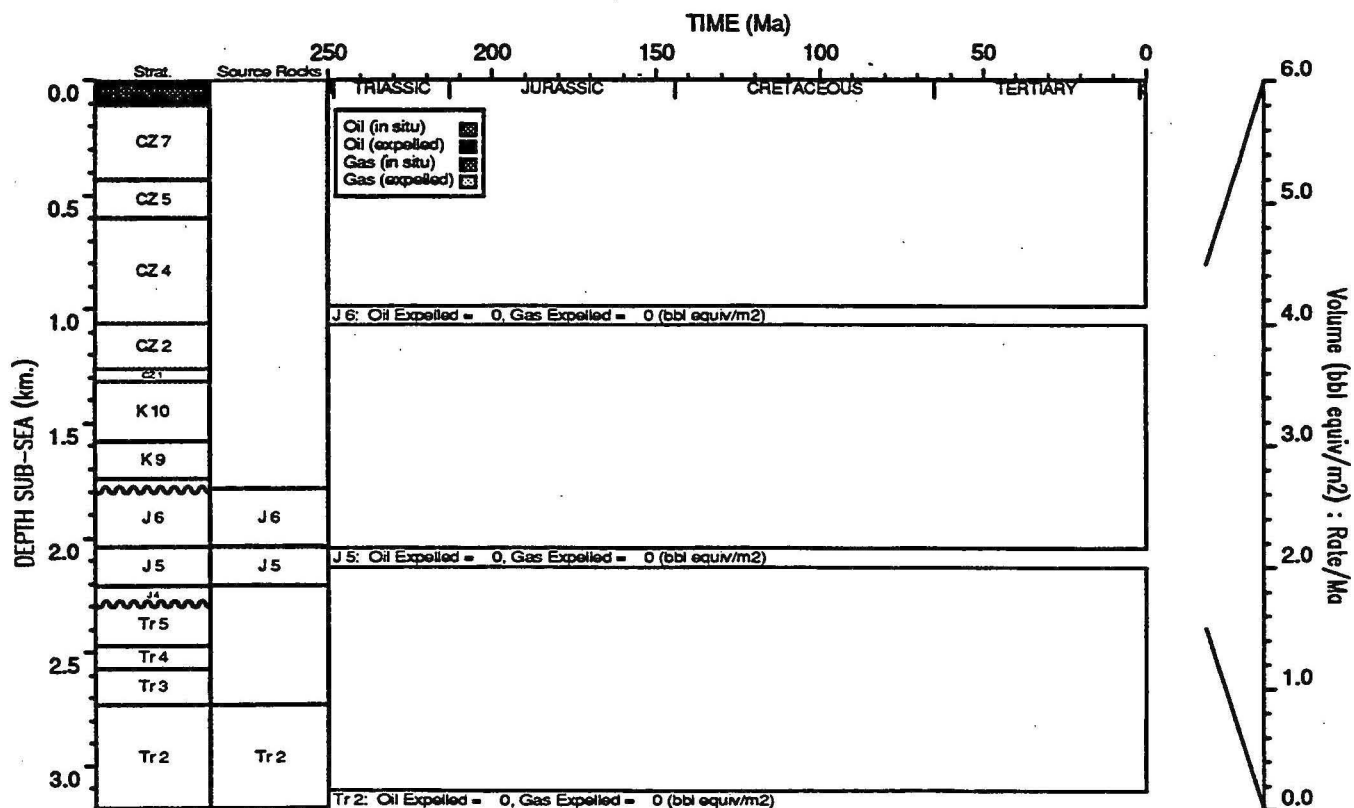
HYDROCARBON GENERATION PLOT : Cossigny 1
