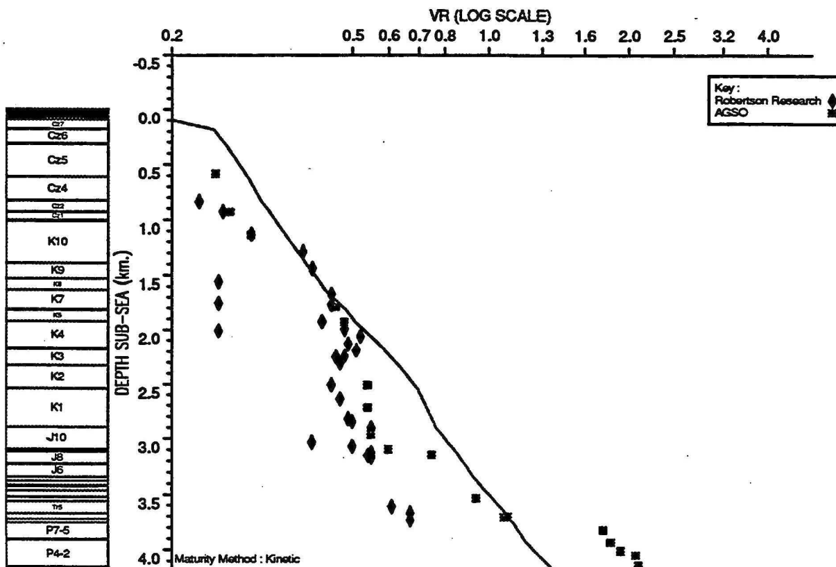
OBSERVED vs COMPUTED MATURITY PLOT : Yampi 1
