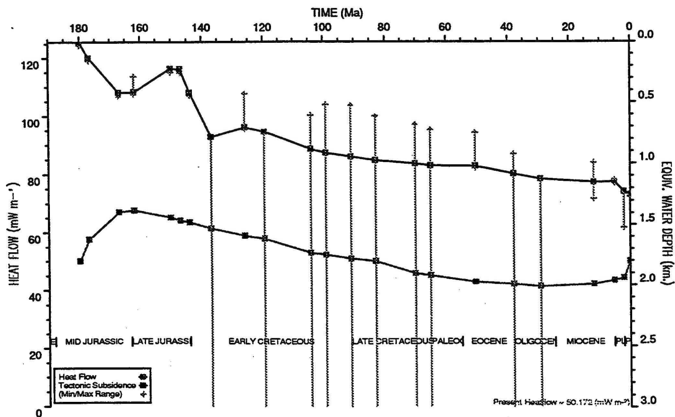
HEATFLOW AND TECTONIC SUBSIDENCE PLOT : Angel 2
