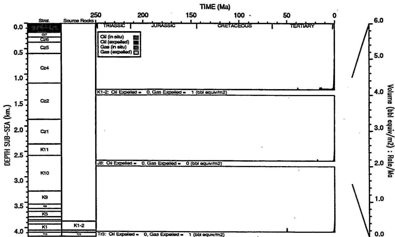
HYDROCARBON GENERATION PLOT : Discorbis 1
