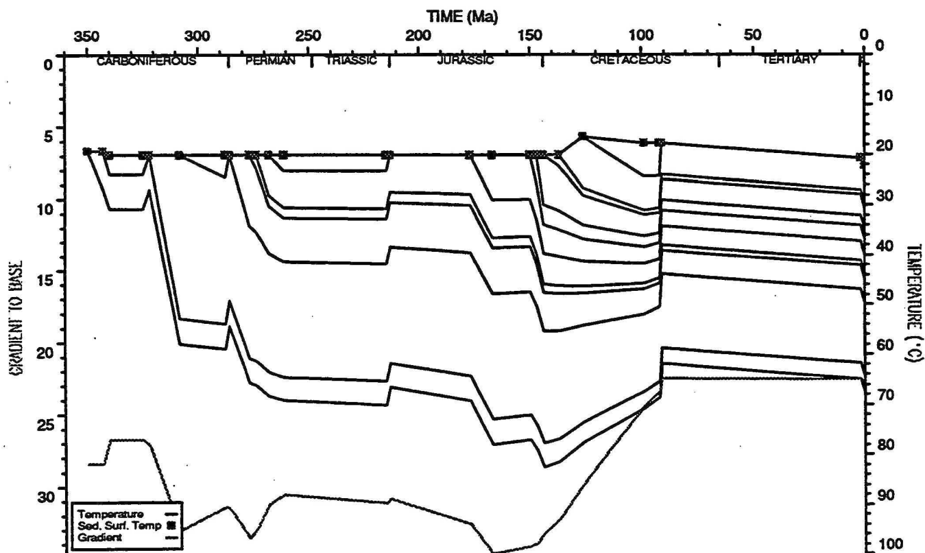
BED TEMPERATURE PLOT : Pearl 1
