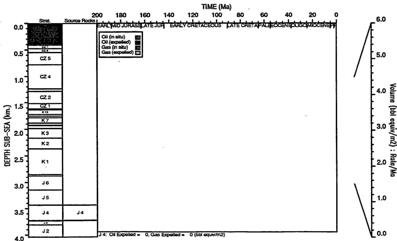
HYDROCARBON GENERATION PLOT : East Mermaid 1
