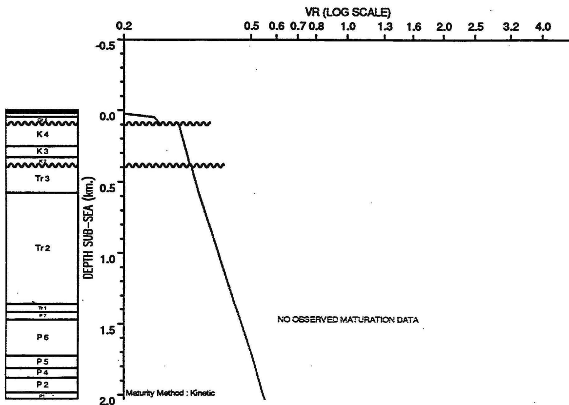
OBSERVED vs COMPUTED MATURITY PLOT : Candace 1
