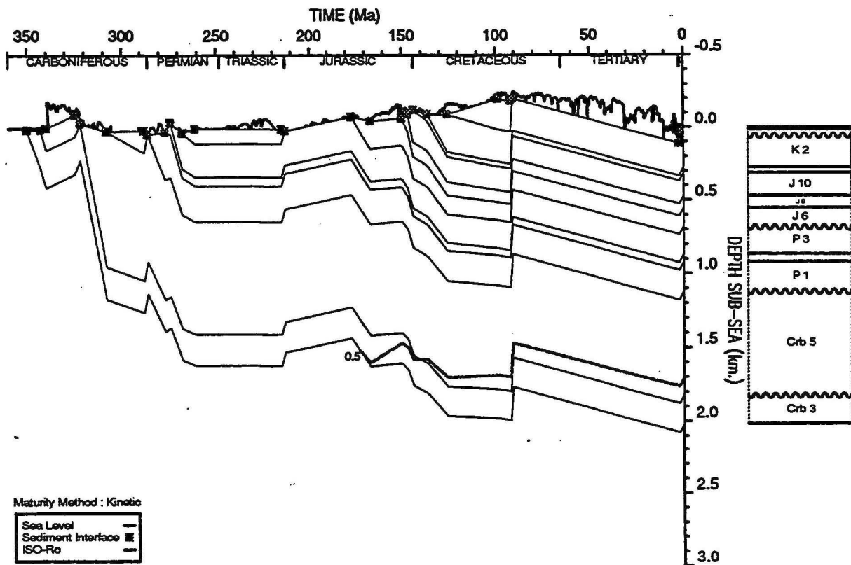
GEOHISTORY PLOT : Pearl 1
