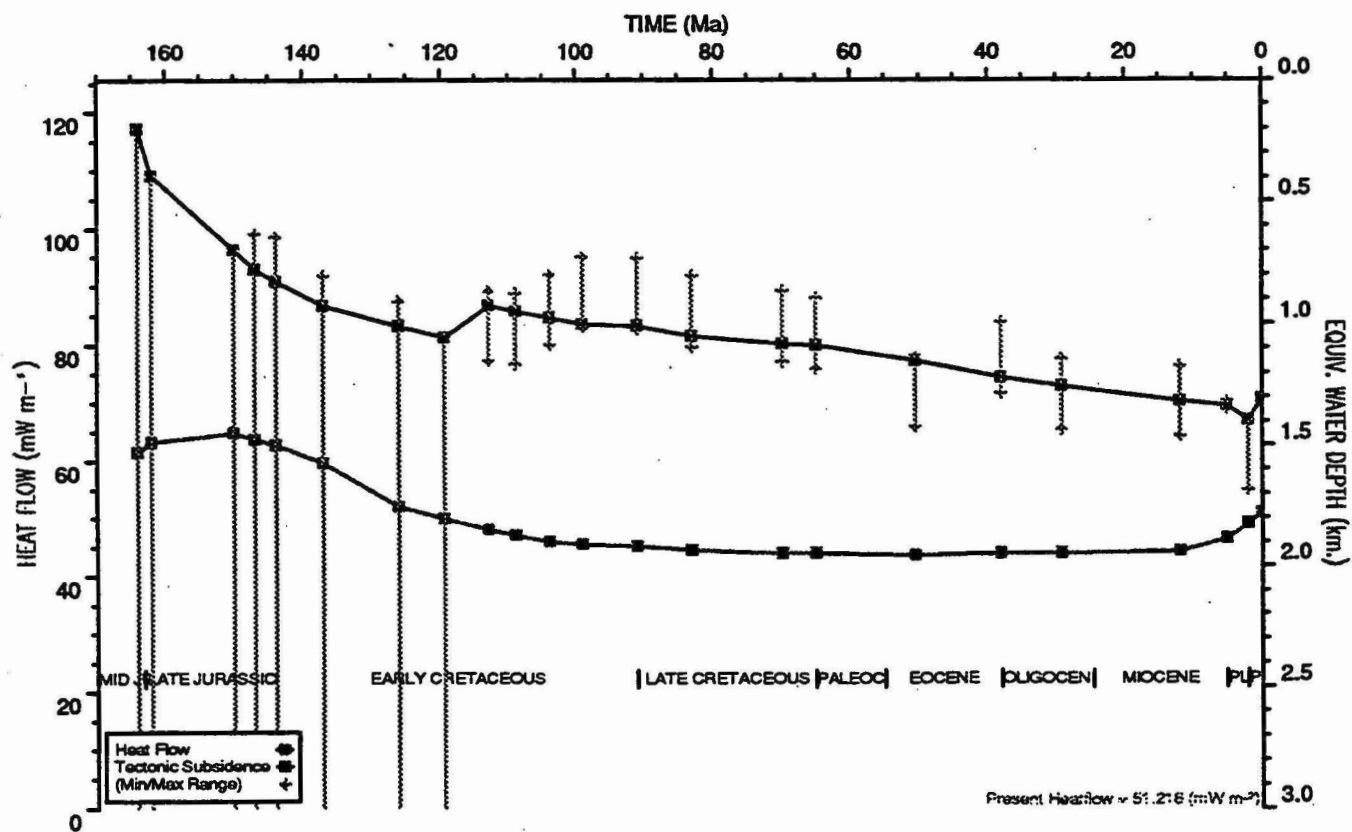
HEATFLOW AND TECTONIC SUBSIDENCE PLOT : Bambra 2
