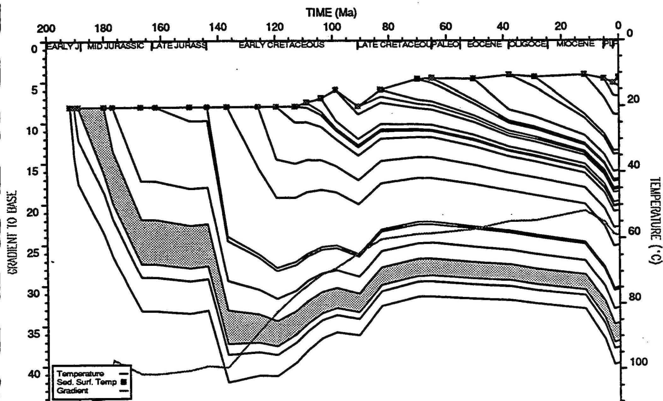
BED TEMPERATURE PLOT : East Mermaid 1
