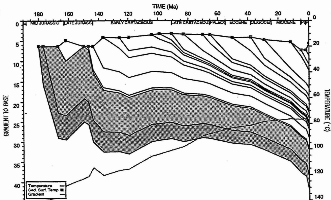
BED TEMPERATURE PLOT : Angel 2
