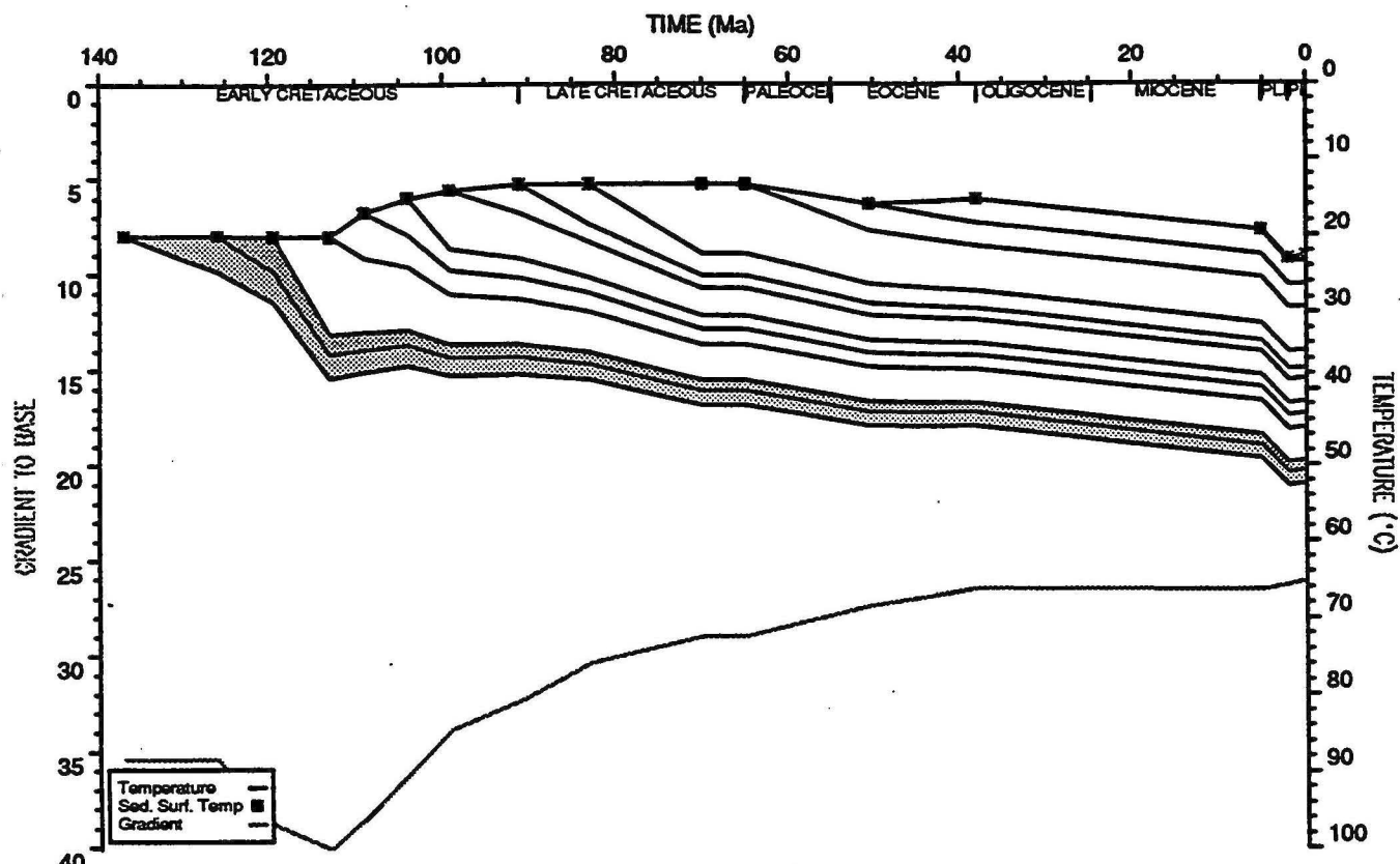
BED TEMPERATURE PLOT : Cowle 1
