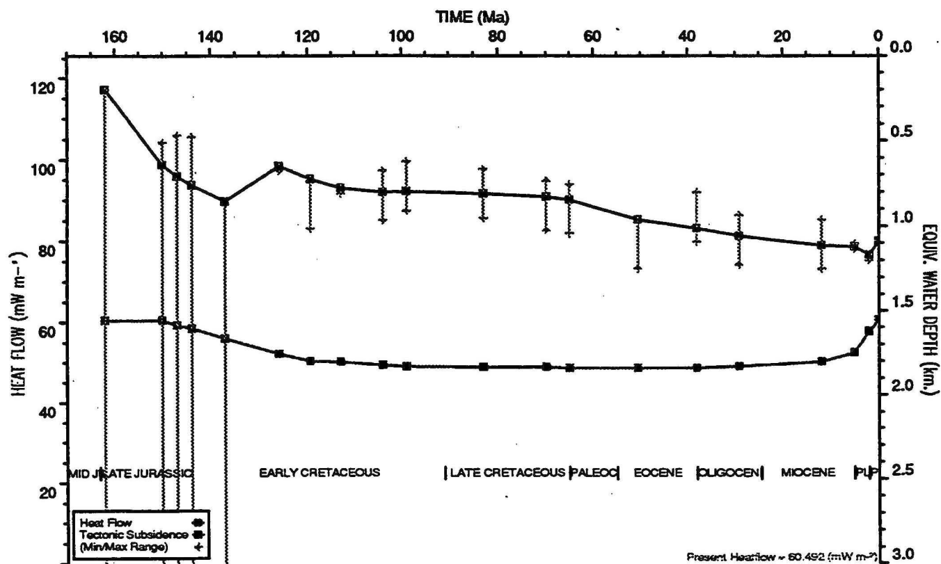
HEATFLOW AND TECTONIC SUBSIDENCE PLOT : South Pepper 1
