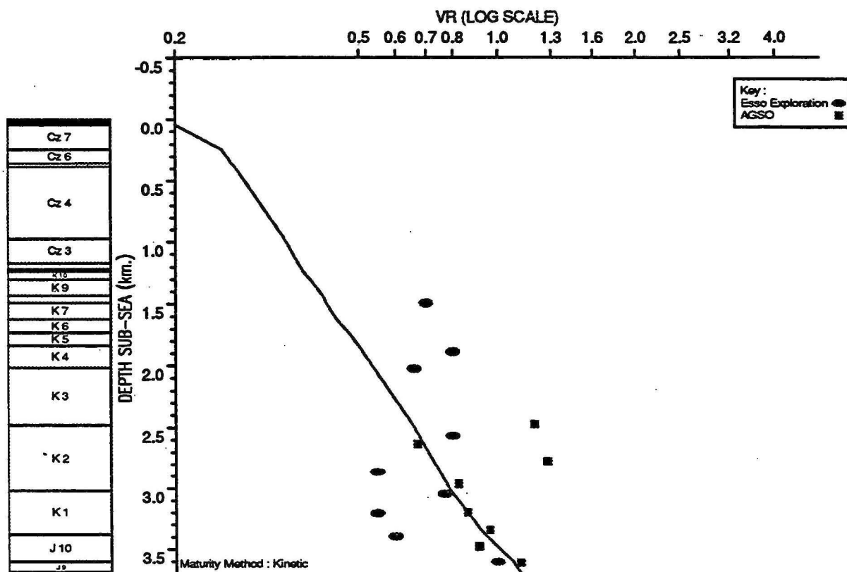
OBSERVED vs COMPUTED MATURITY PLOT : Tryal Rocks 1
