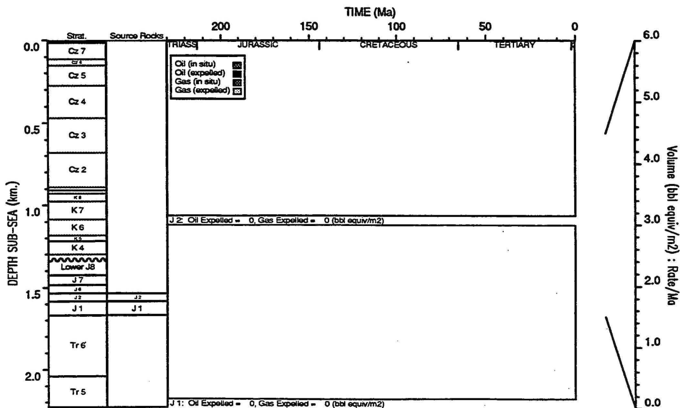
HYDROCARBON GENERATION PLOT : Leatherback 1
