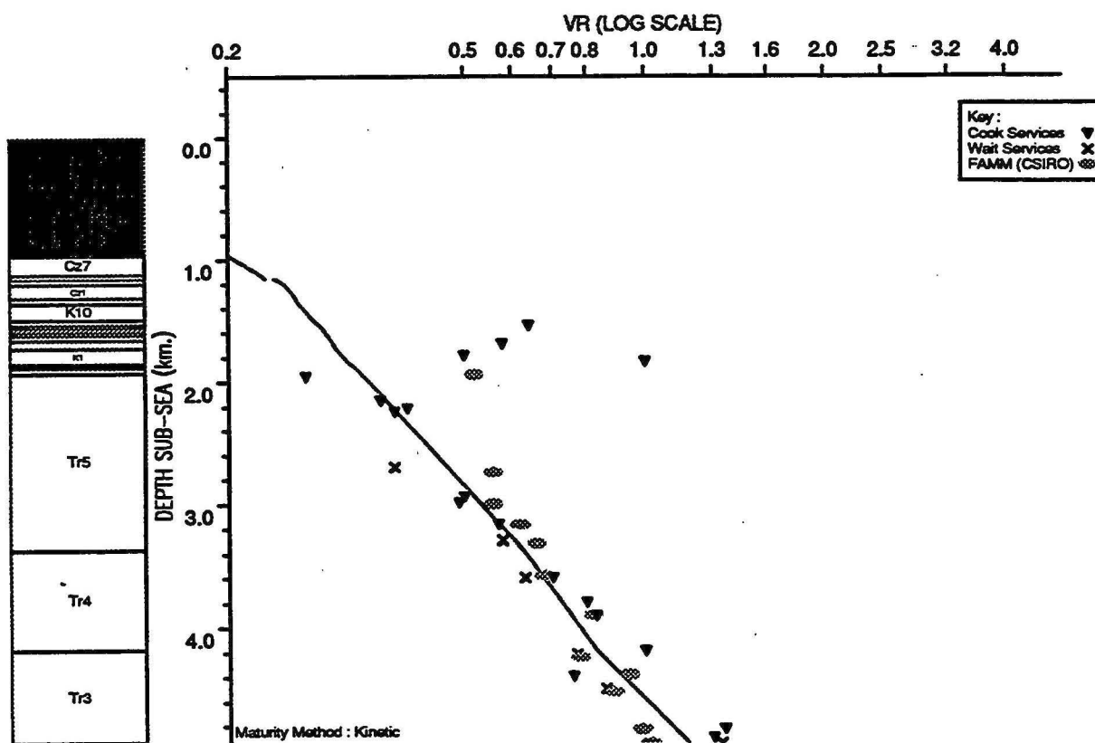
OBSERVED vs COMPUTED MATURITY PLOT : Jupiter 1
