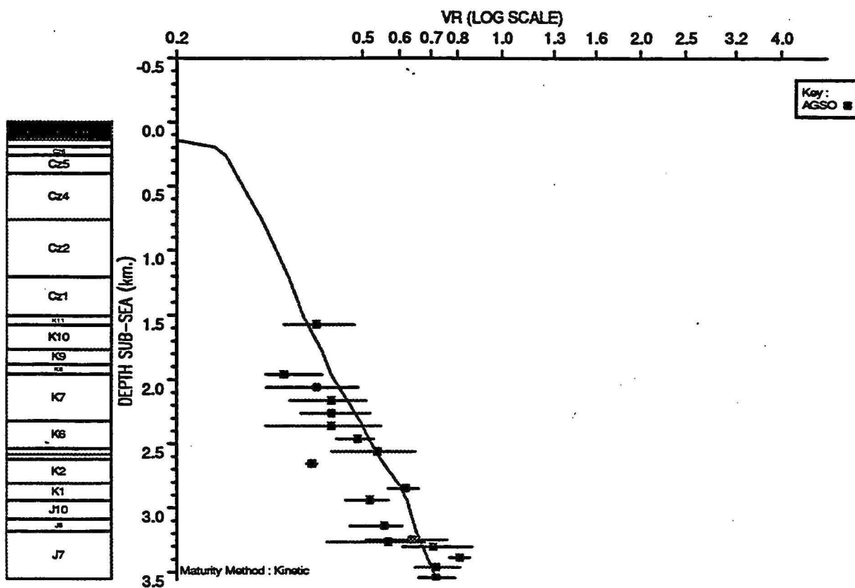
OBSERVED vs COMPUTED MATURITY PLOT : Buccaneer 1
