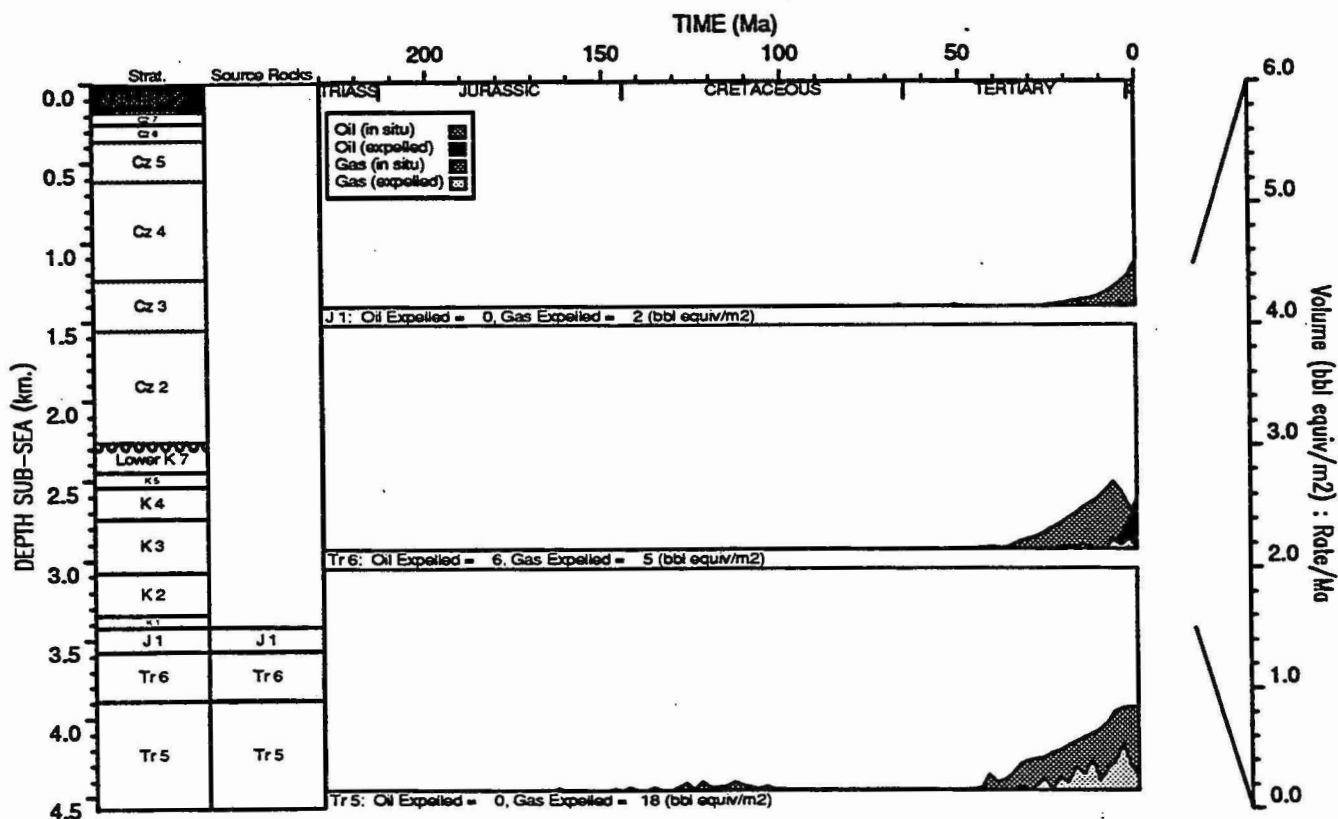
HYDROCARBON GENERATION PLOT : Bluebell 1
