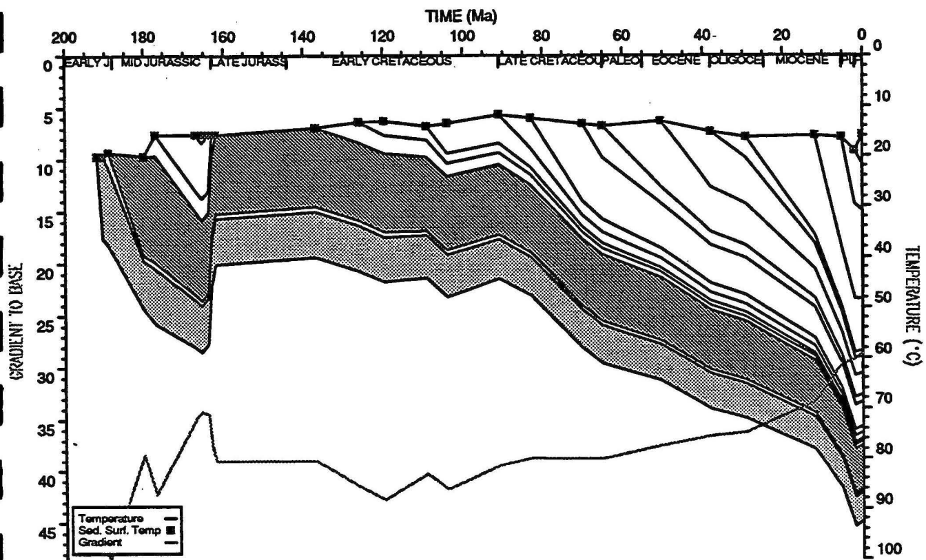
BED TEMPERATURE PLOT : Ronsard 1
