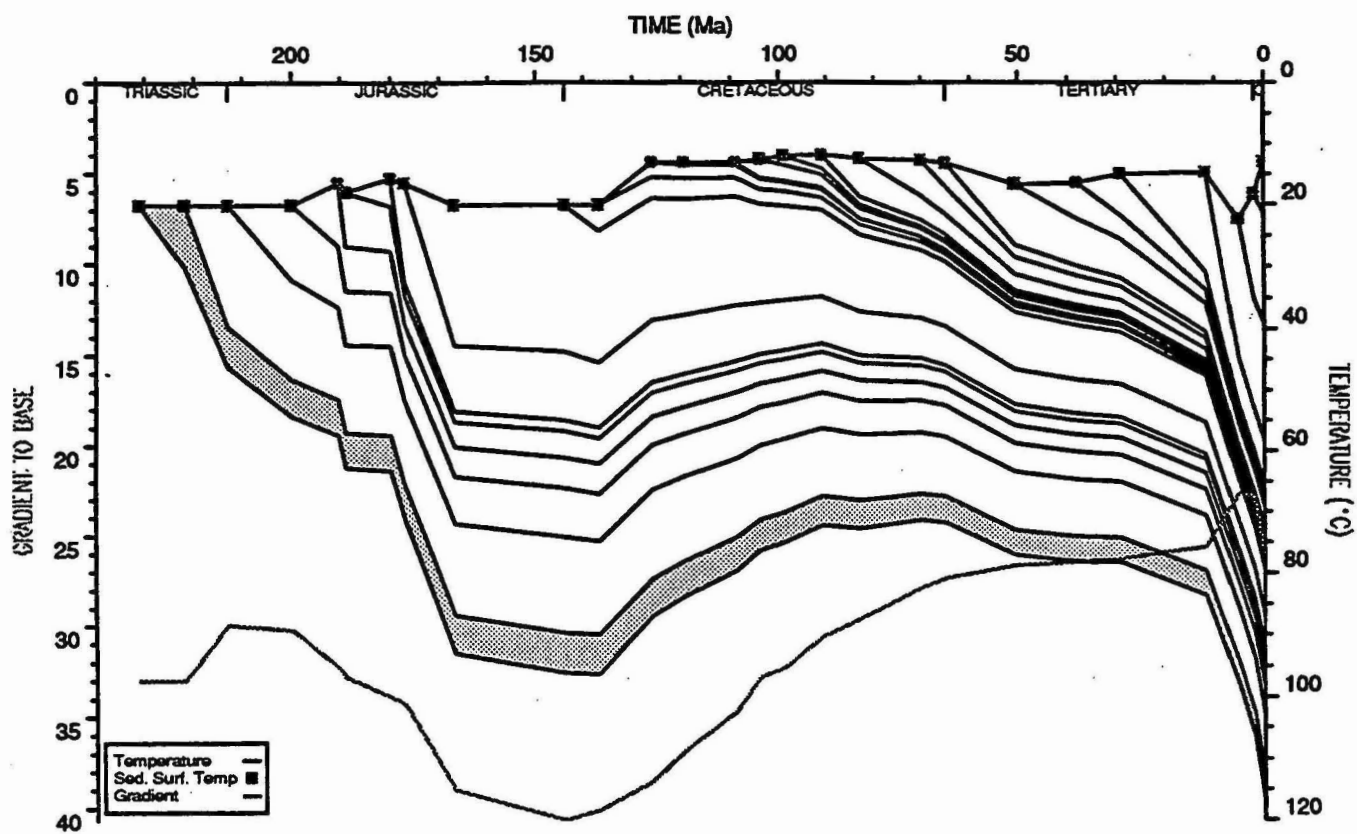
BED TEMPERATURE PLOT : Brigadier 1
