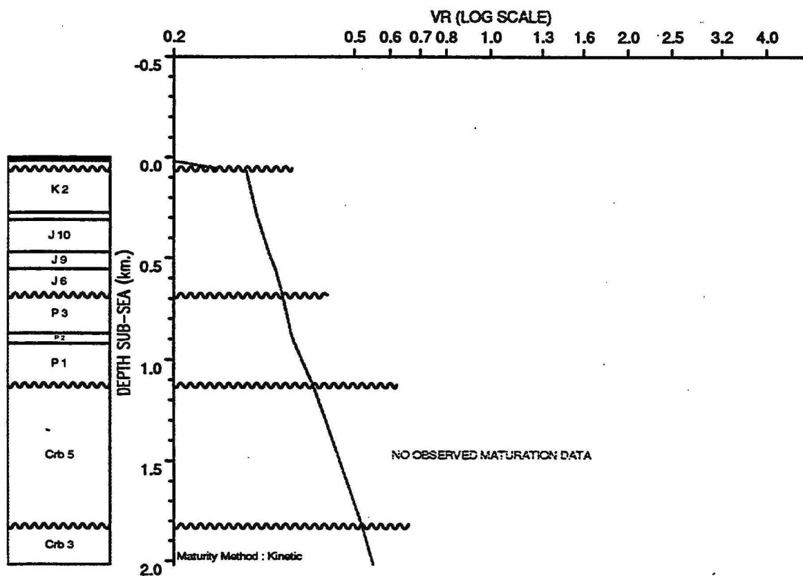
OBSERVED vs COMPUTED MATURITY PLOT : Pearl 1
