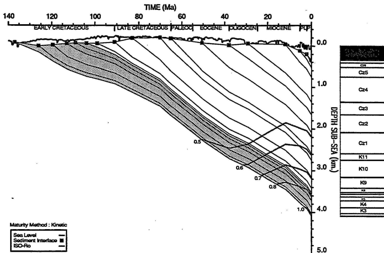
GEOHISTORY PLOT : Caswell 1
