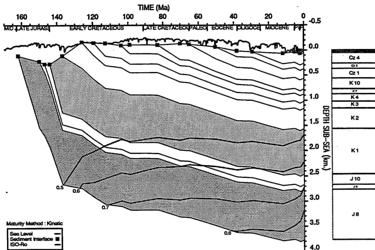
GEOHISTORY PLOT : South Pepper 1
