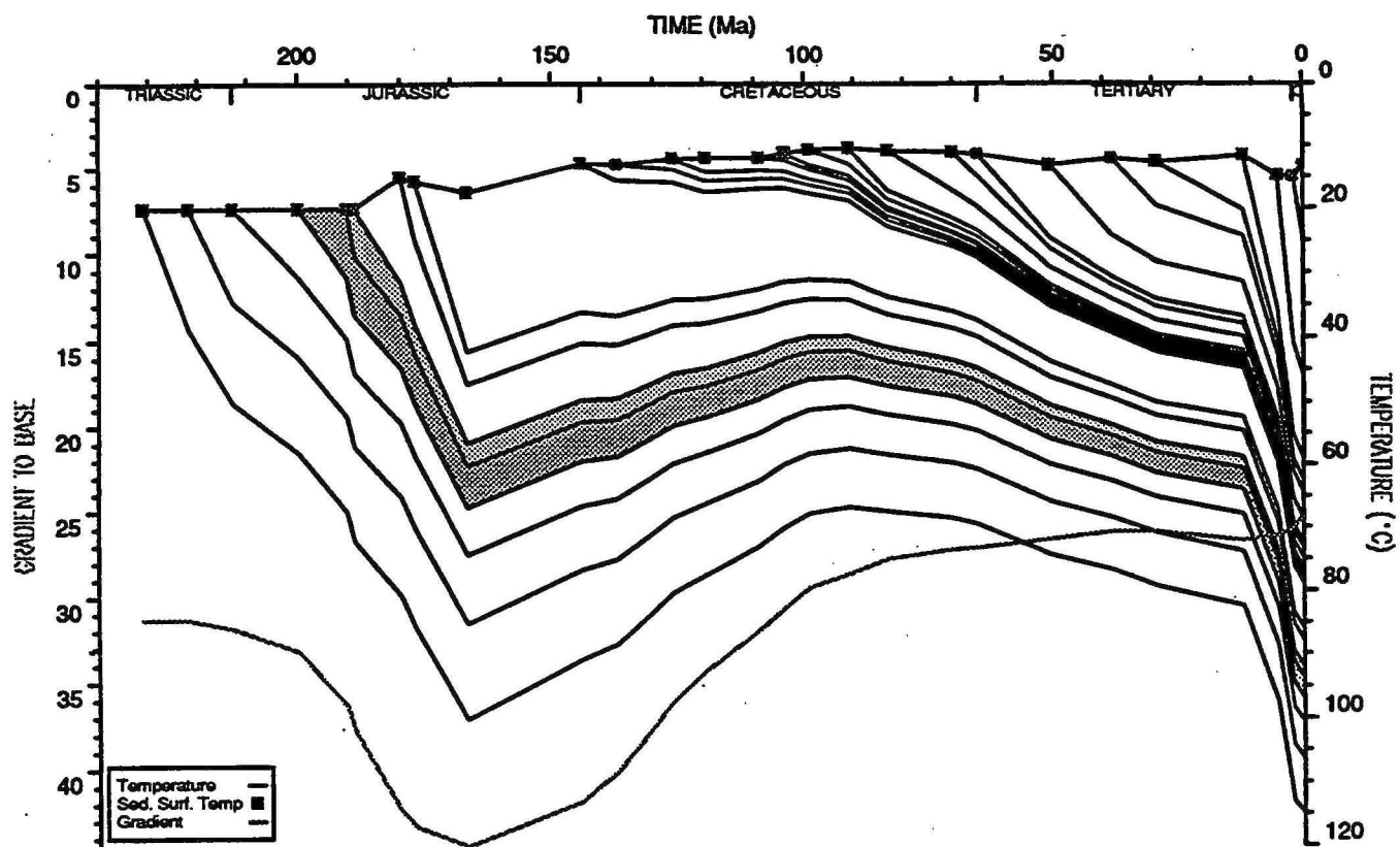
BED TEMPERATURE PLOT : Gandara 1
