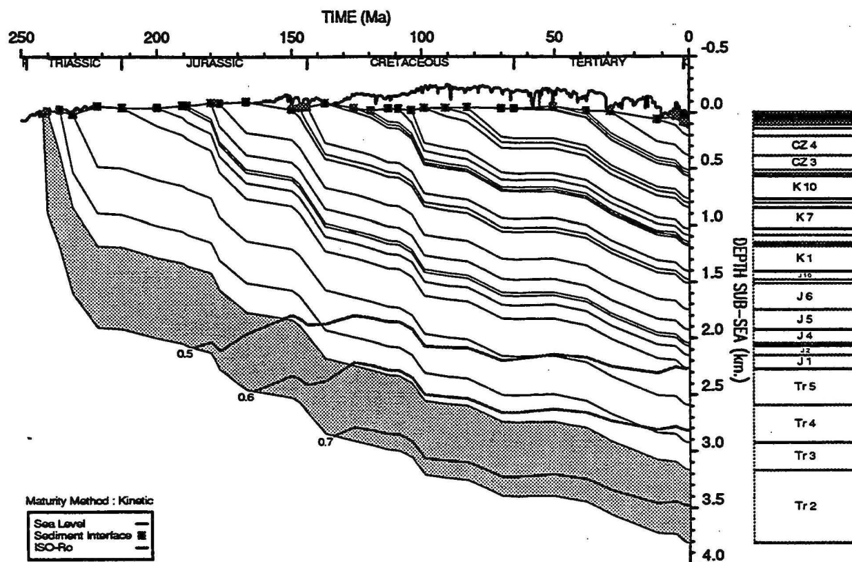
GEOHISTORY PLOT : Keraudren 1
