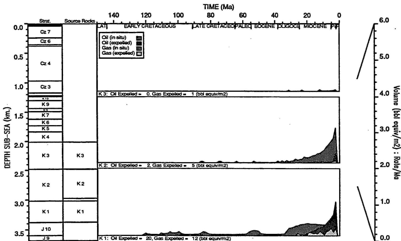
HYDROCARBON GENERATION PLOT : Tryal Rocks 1
