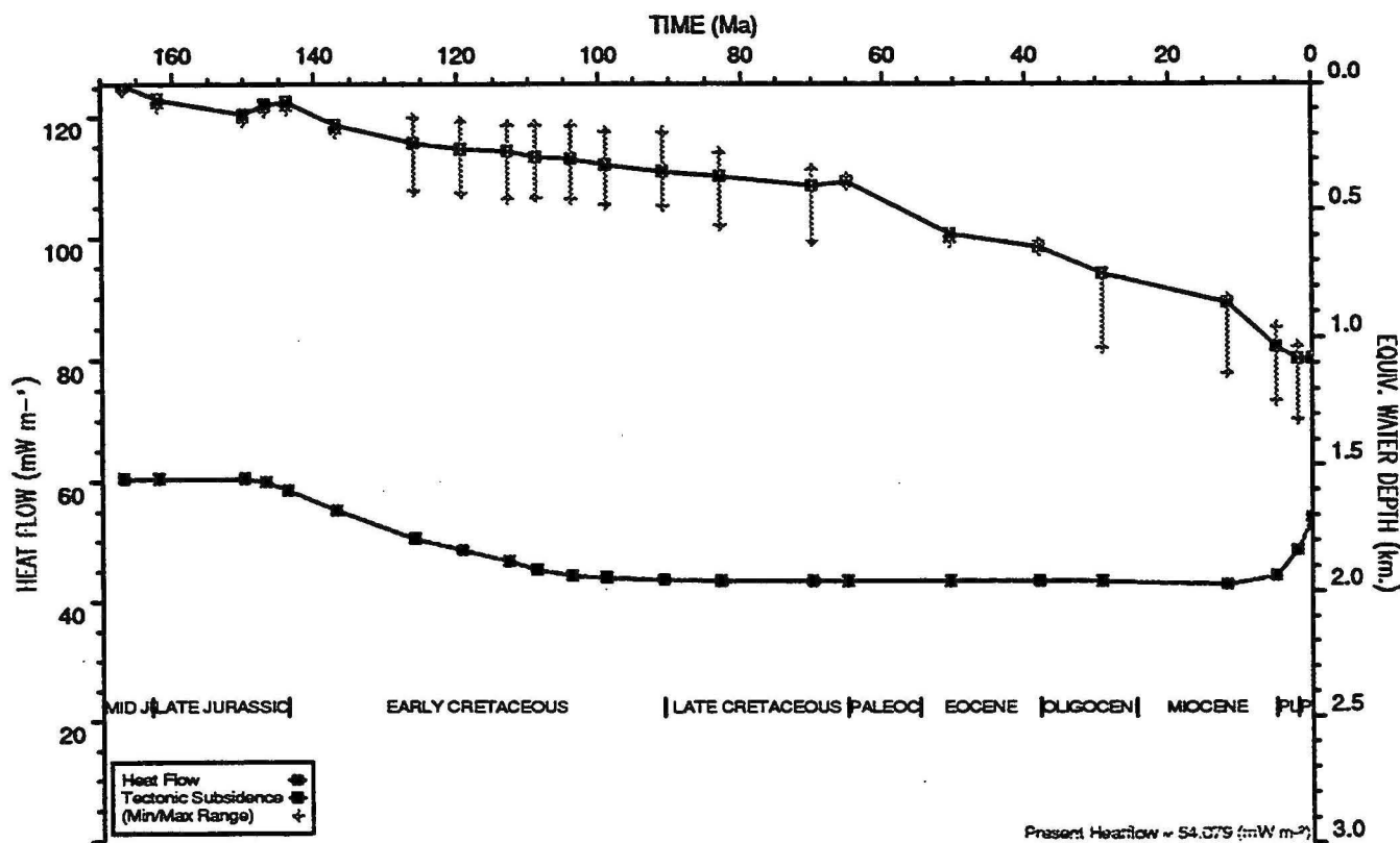
HEATFLOW AND TECTONIC SUBSIDENCE PLOT : Buccaneer 1
