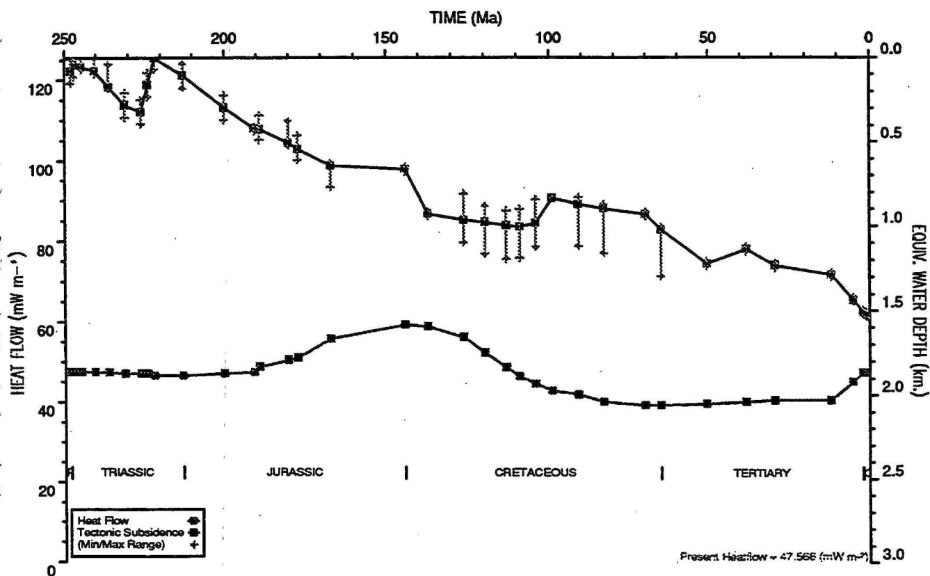
HEATFLOW AND TECTONIC SUBSIDENCE PLOT : Bedout 1
