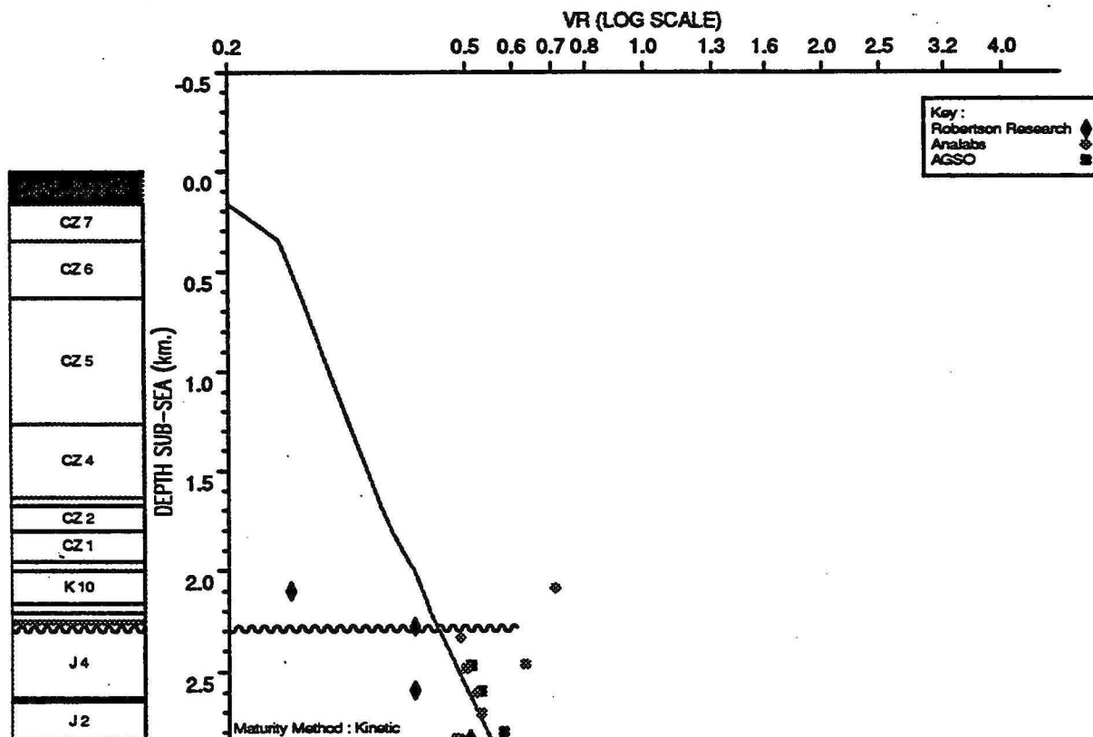
OBSERVED vs COMPUTED MATURITY PLOT : Ronsard 1
