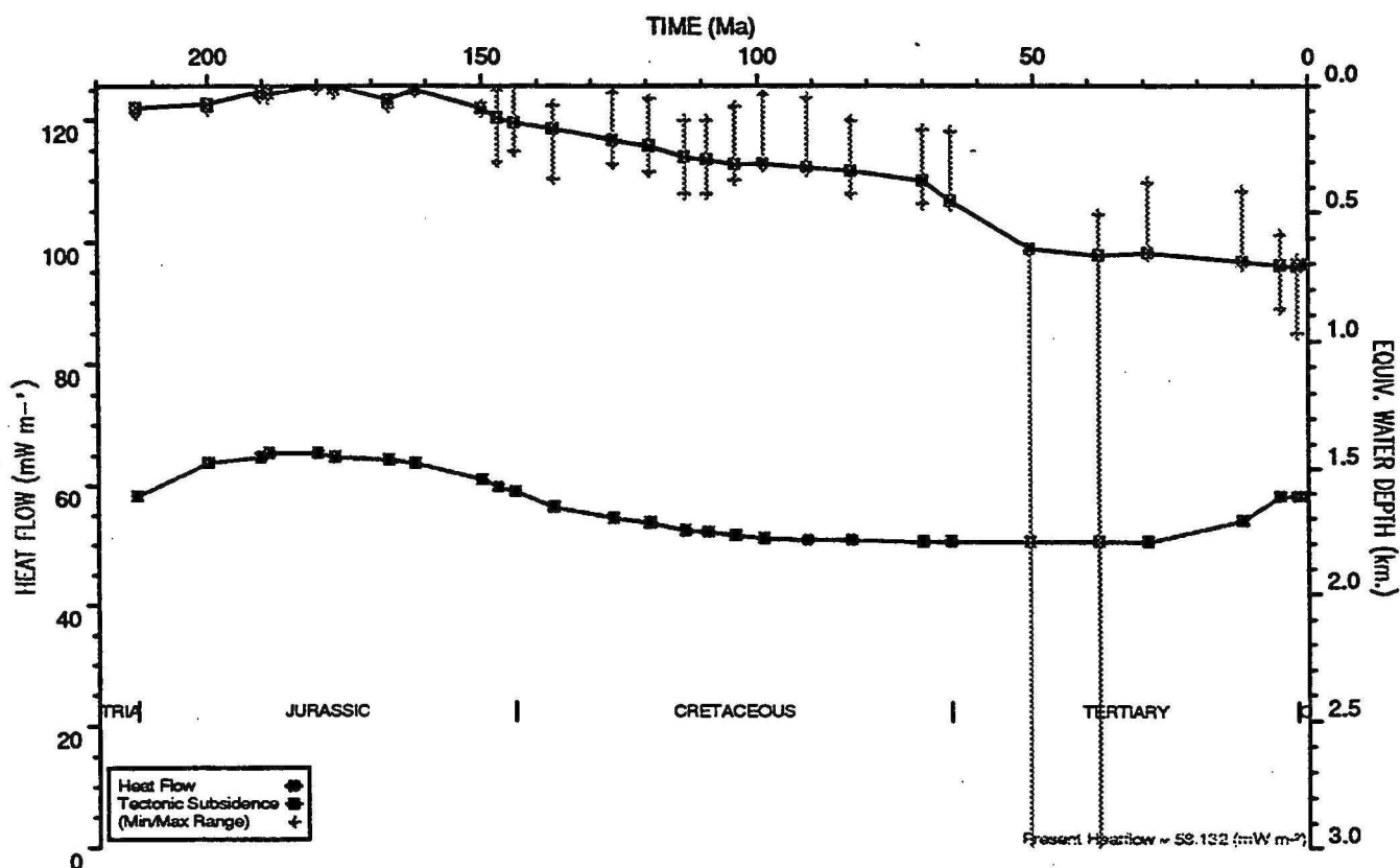
HEATFLOW AND TECTONIC SUBSIDENCE PLOT : Lombardina 1
