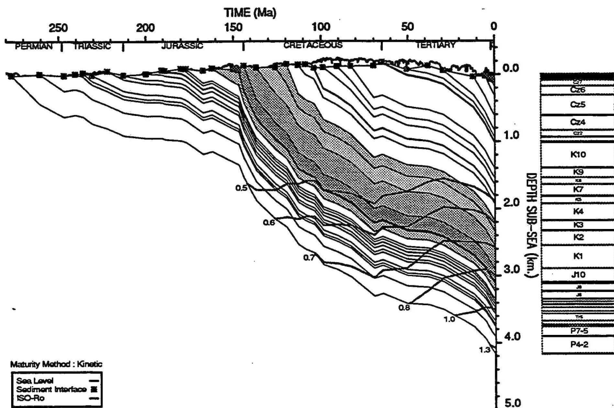
GEOHISTORY PLOT : Yampi 1
