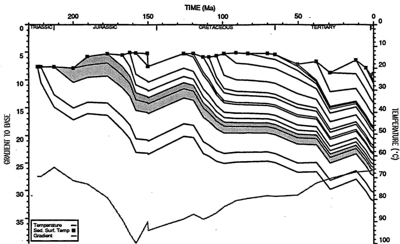
BED TEMPERATURE PLOT : Leatherback 1
