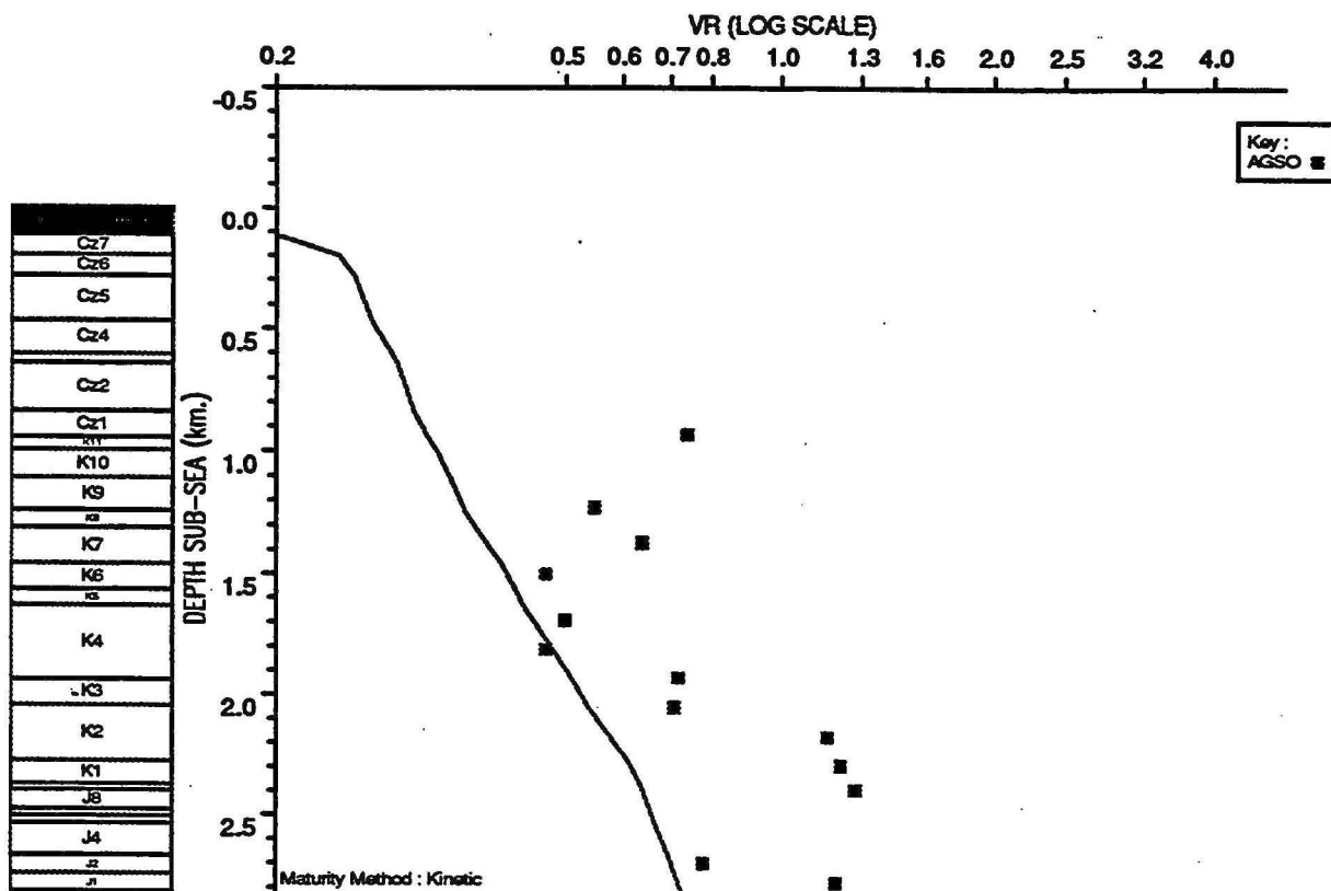
OBSERVED vs COMPUTED MATURITY PLOT : Lombardina 1
