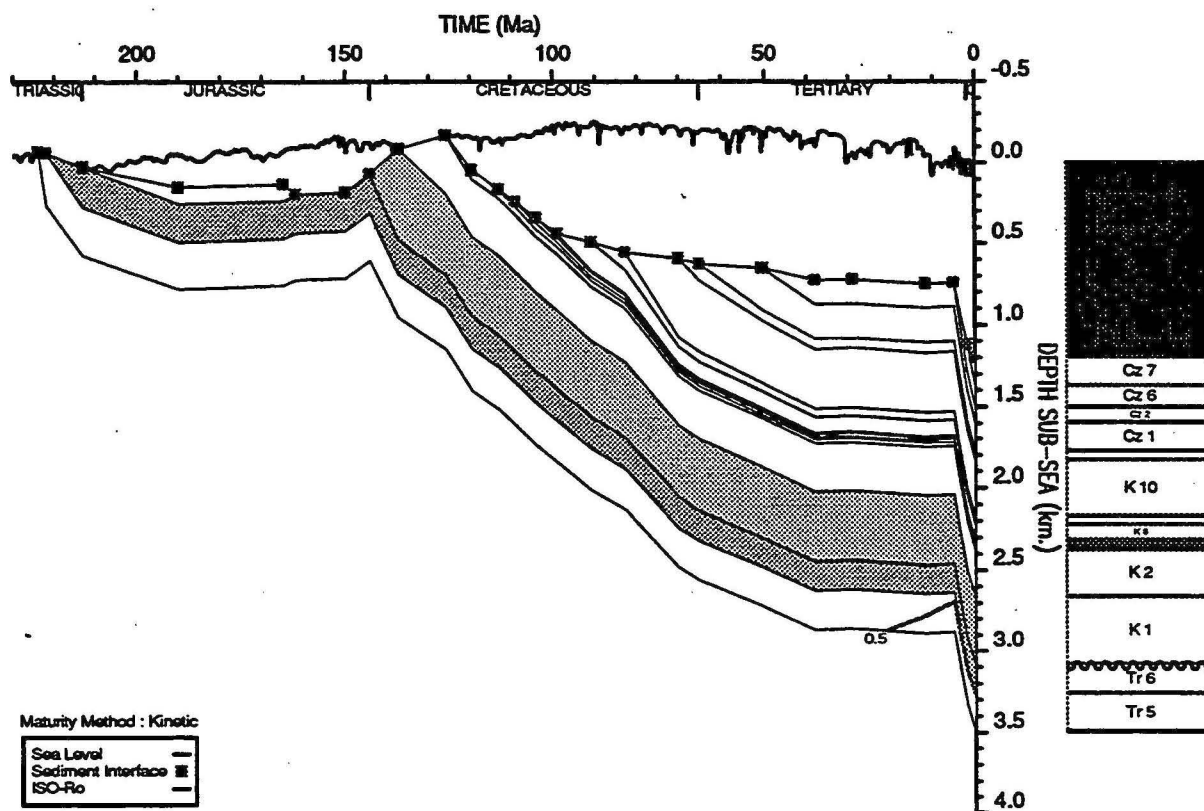
GEOHISTORY PLOT : Zeewulf 1
