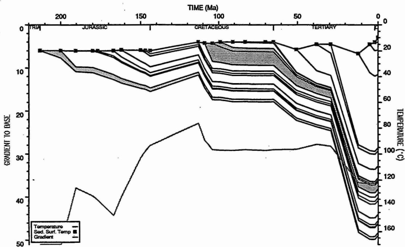
BED TEMPERATURE PLOT : Buffon 1
