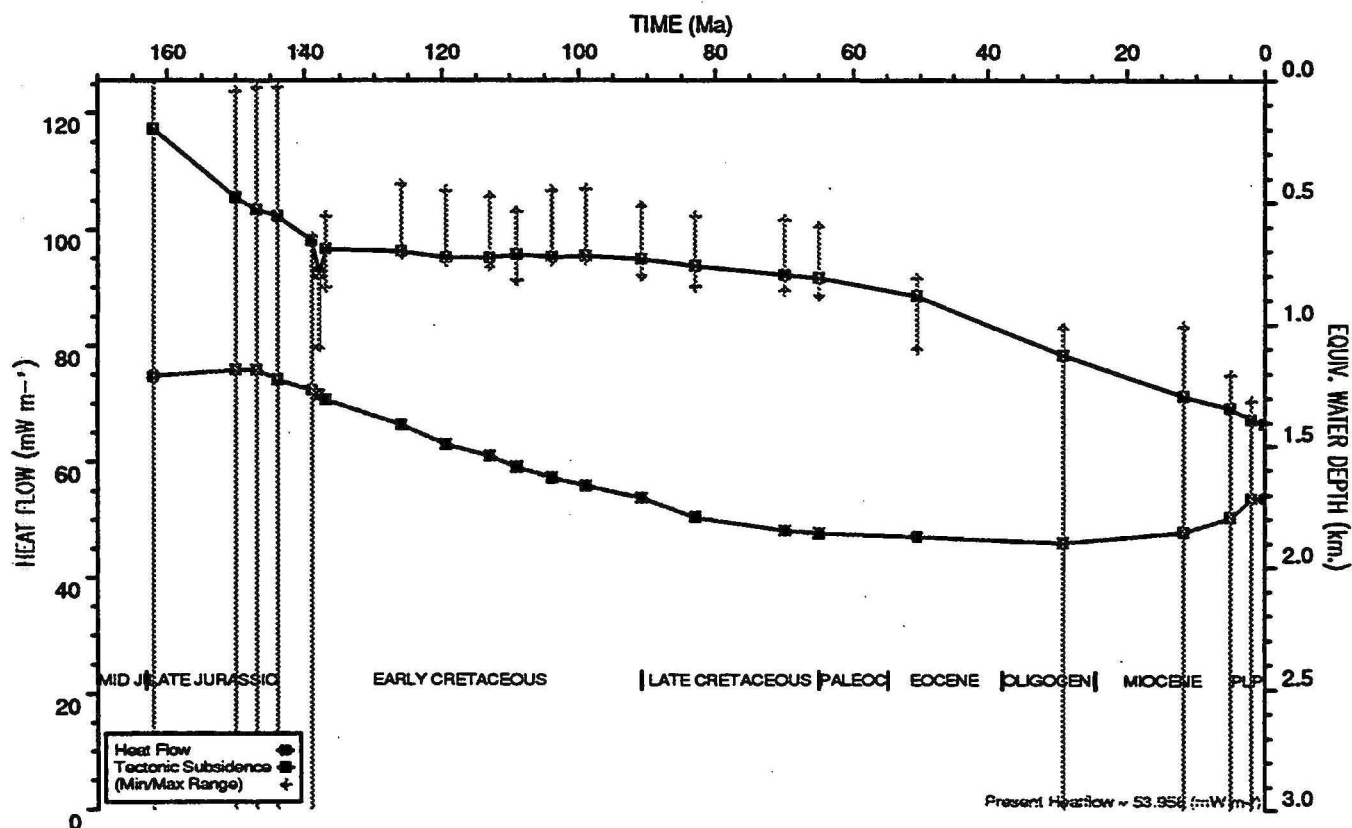
HEATFLOW AND TECTONIC SUBSIDENCE PLOT : Novara 1
