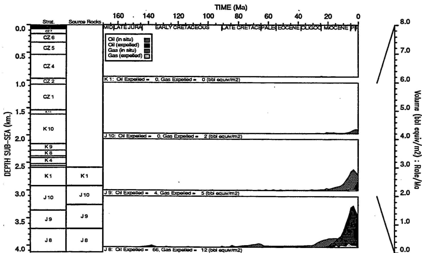
HYDROCARBON GENERATION PLOT : Dampier 1
