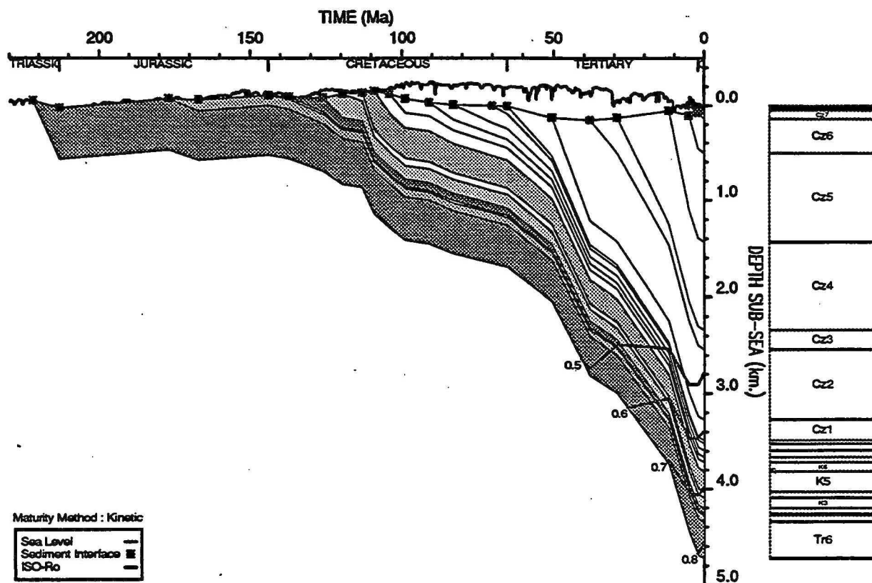
GEOHISTORY PLOT : Scott Reef 1
