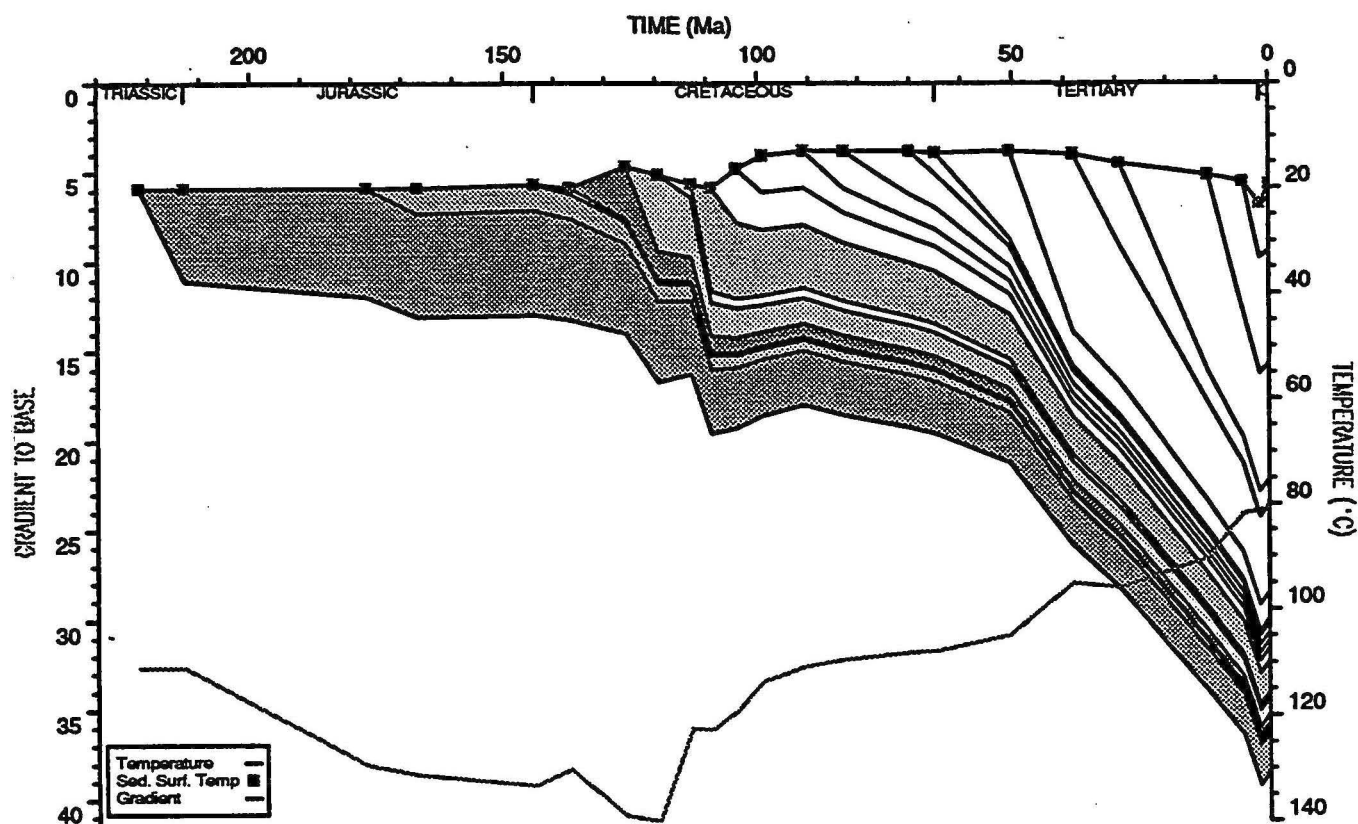
BED TEMPERATURE PLOT : Scott Reef 1
