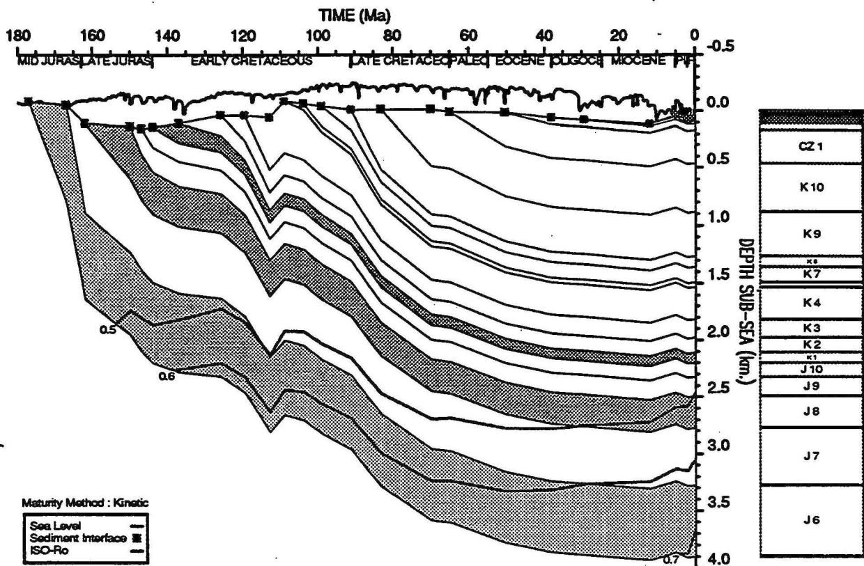
GEOHISTORY PLOT : Rosemary 1
