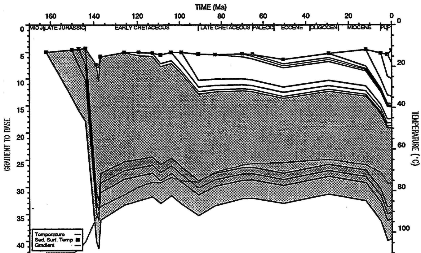
BED TEMPERATURE PLOT : Novara 1
