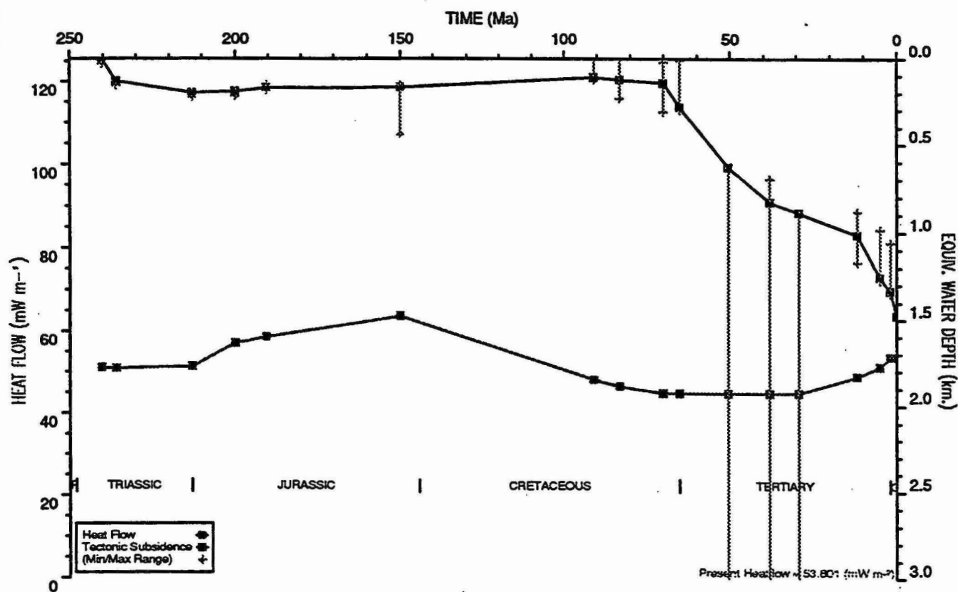
HEATFLOW AND TECTONIC SUBSIDENCE PLOT : North Scott Reef 1
