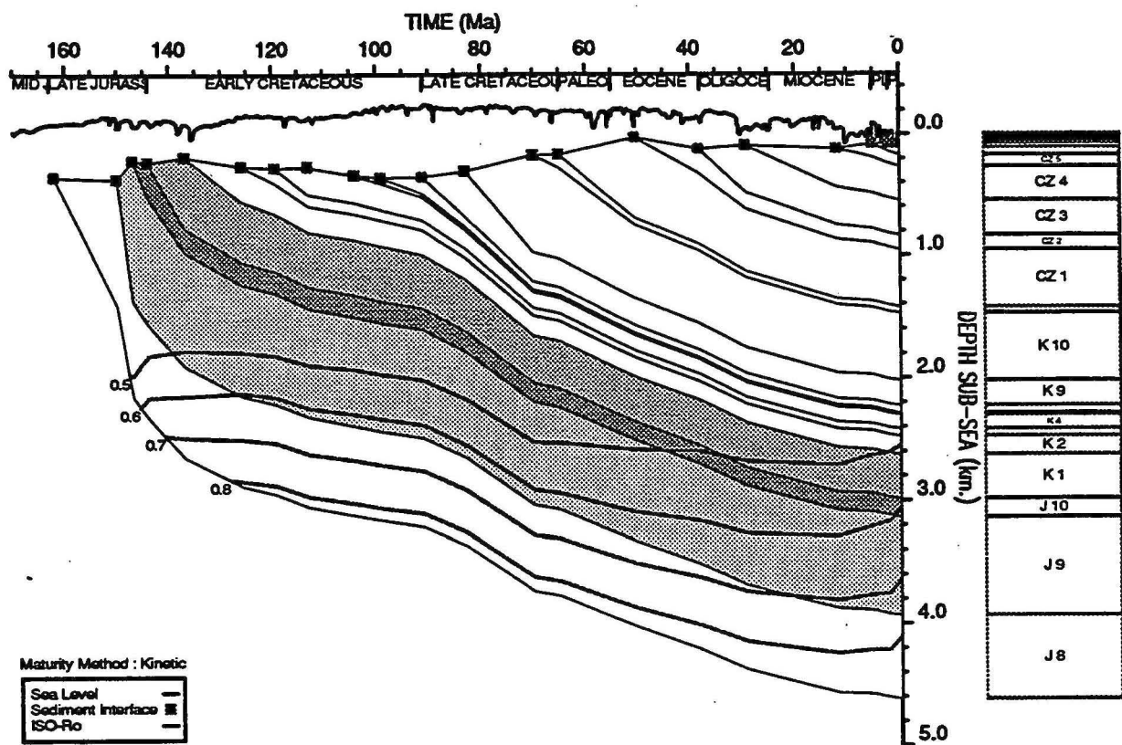
GEOHISTORY PLOT : Withnell 1
