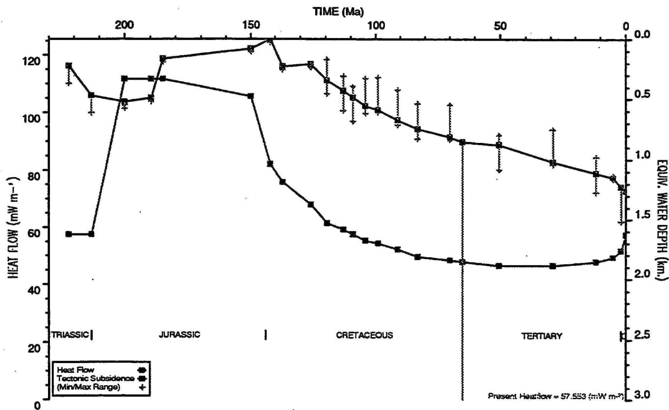
HEATFLOW AND TECTONIC SUBSIDENCE PLOT : Griffin 1
