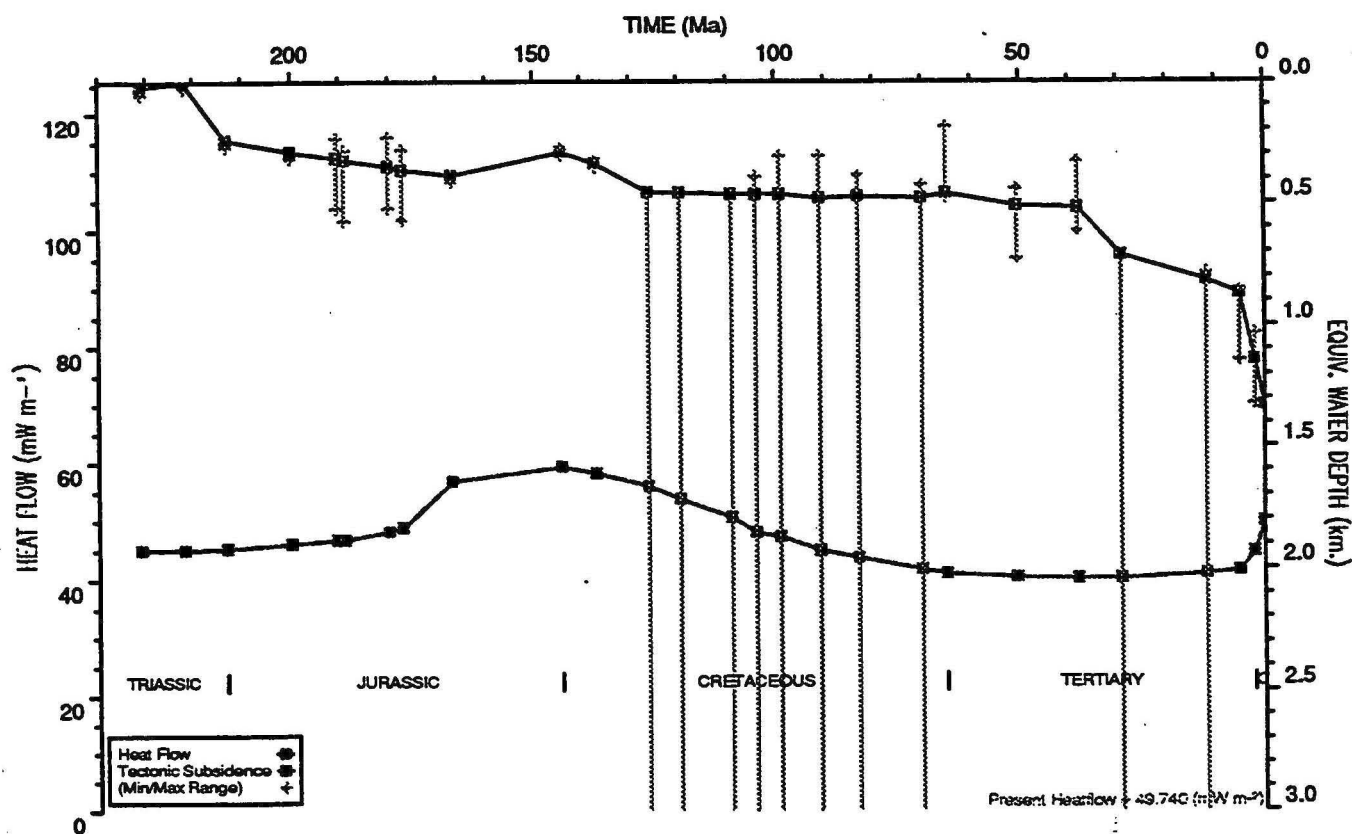
HEATFLOW AND TECTONIC SUBSIDENCE PLOT : Brigadier 1
