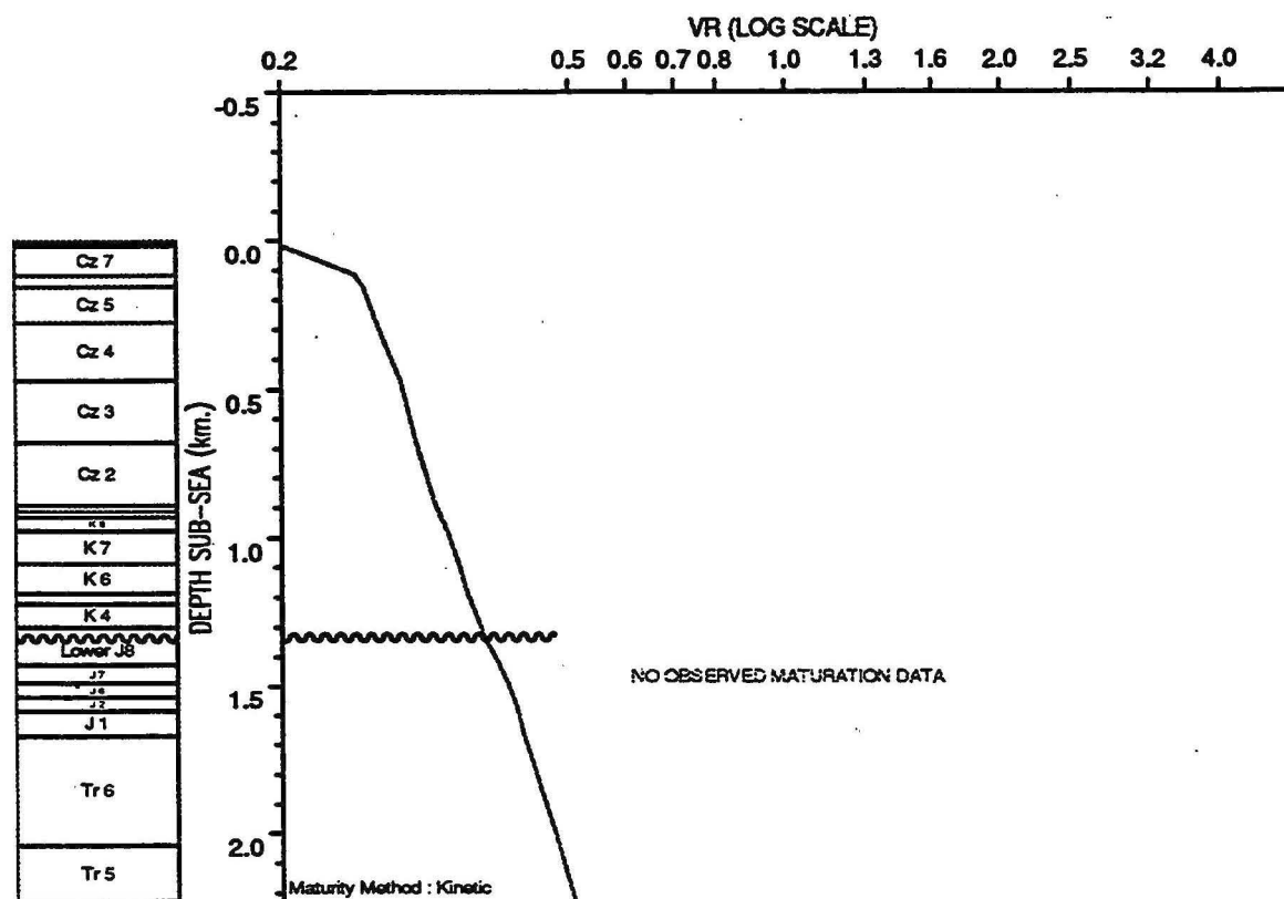
OBSERVED vs COMPUTED MATURITY PLOT : Leatherback 1
