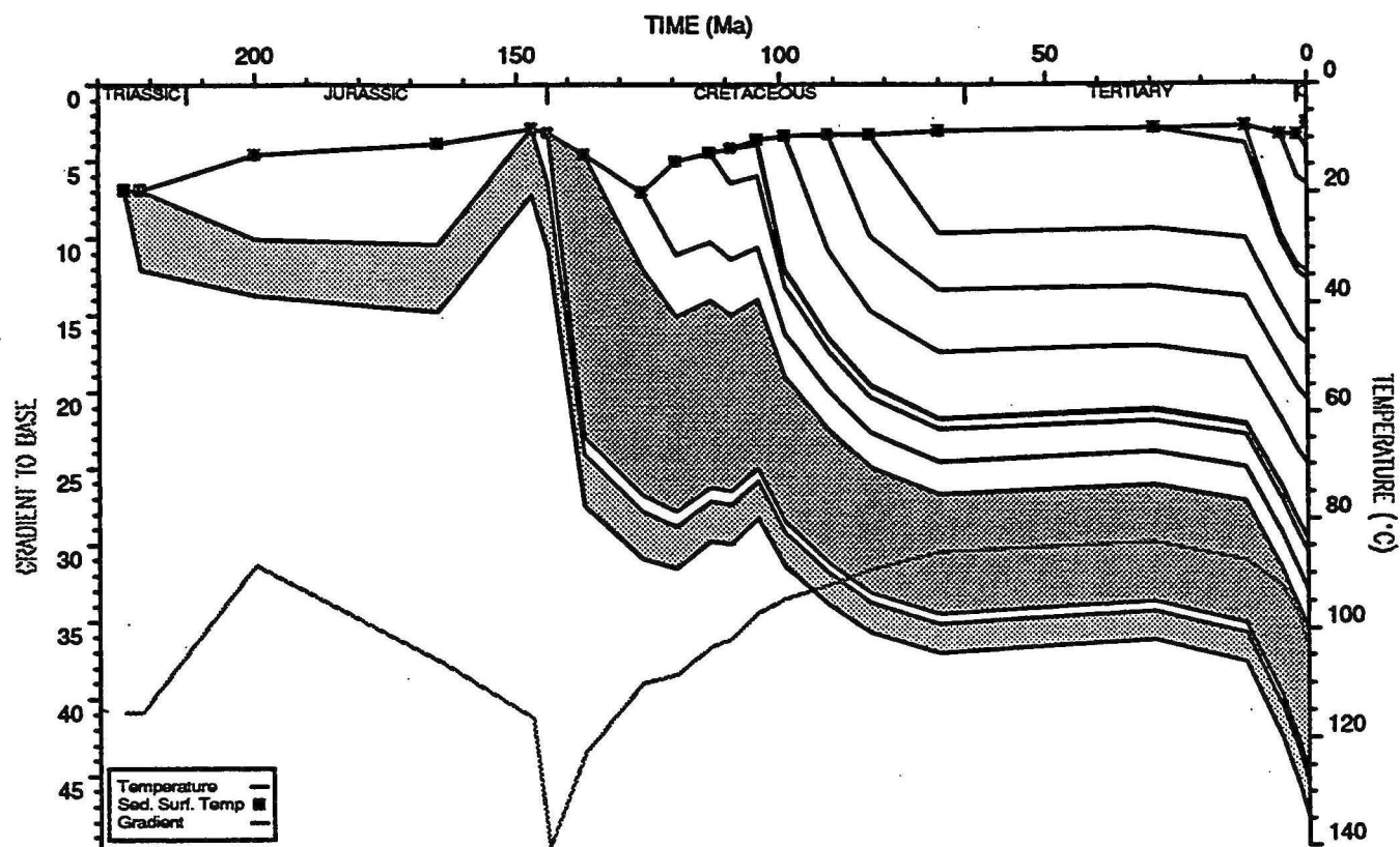
BED TEMPERATURE PLOT : Zeepaard 1
