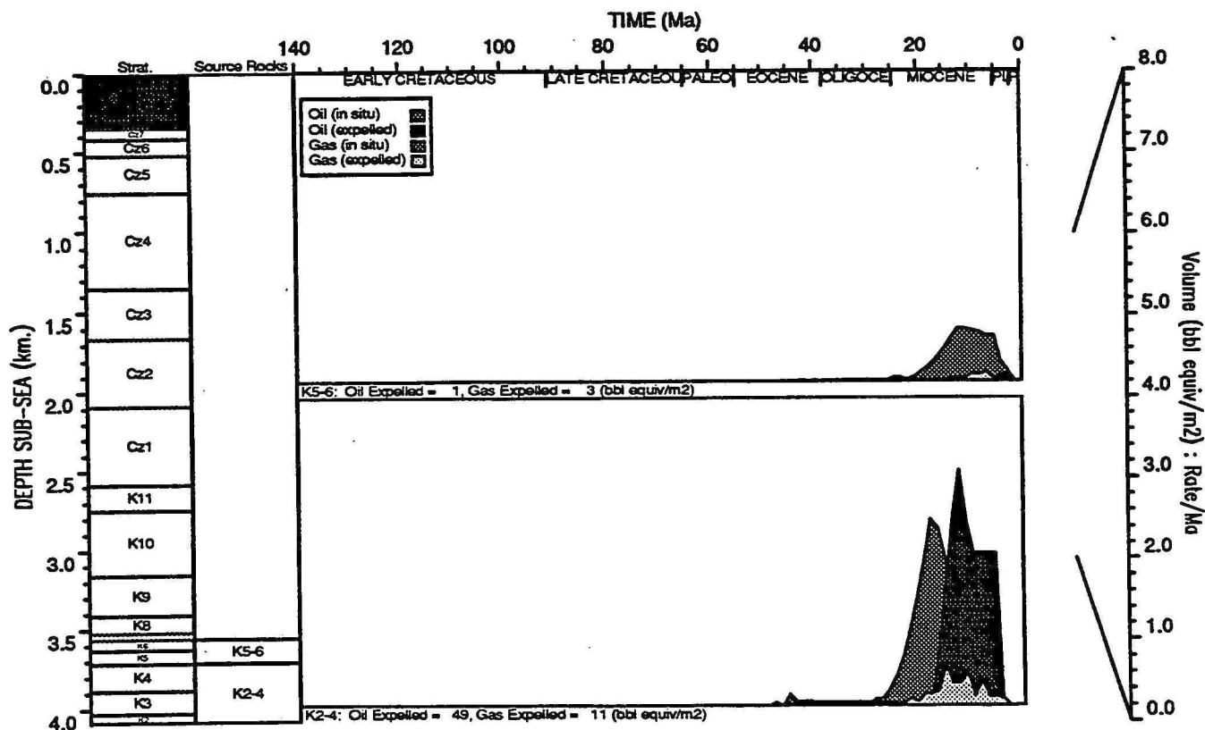
HYDROCARBON GENERATION PLOT : Caswell 1
