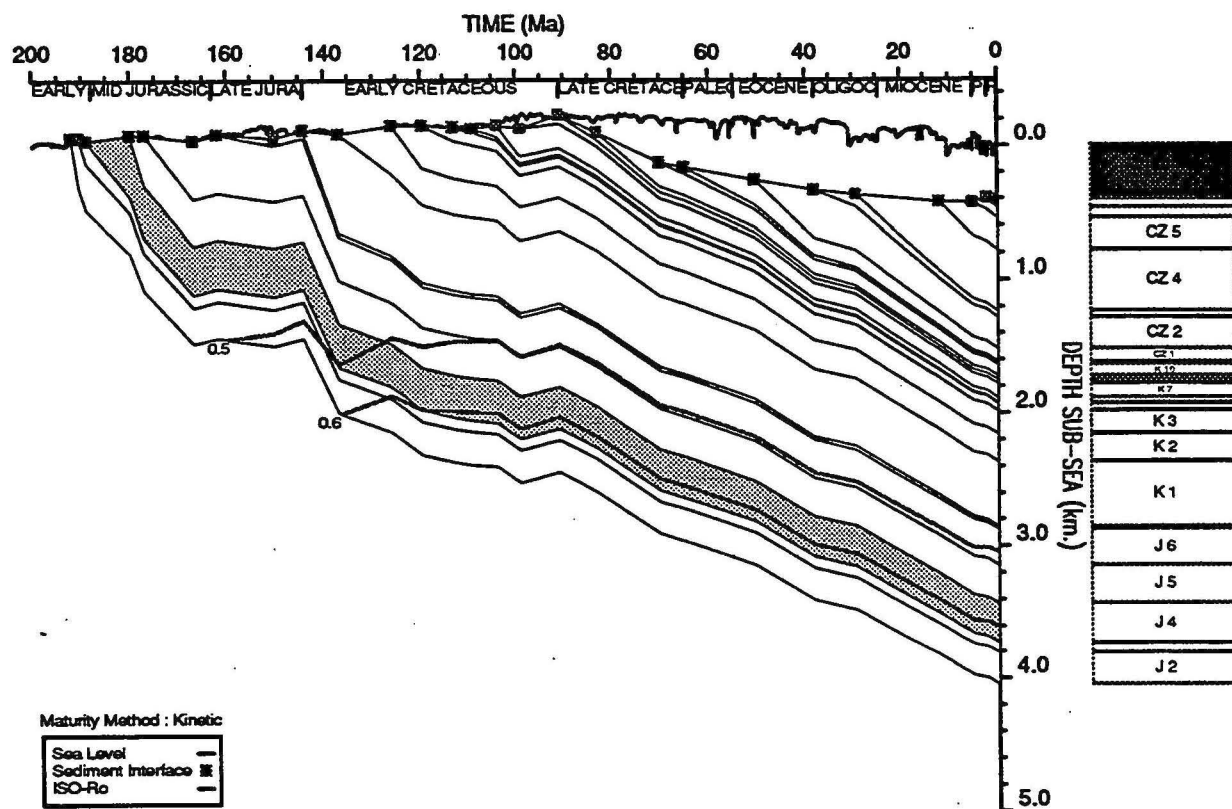
GEOHISTORY PLOT : East Mermaid 1
