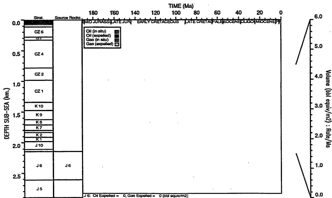
HYDROCARBON GENERATION PLOT : Talisman 1
