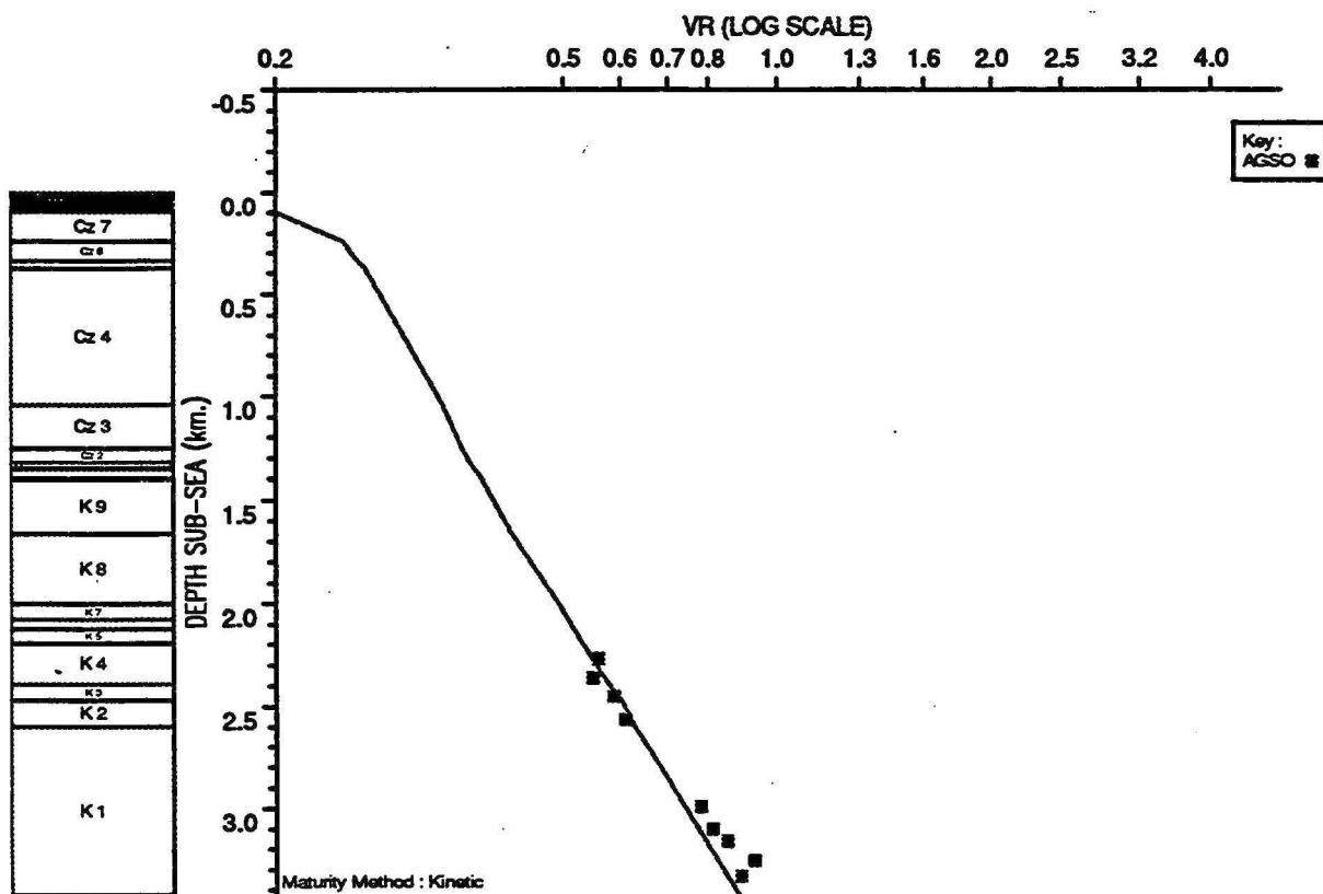
OBSERVED vs COMPUTED MATURITY PLOT : West Barrow 2
