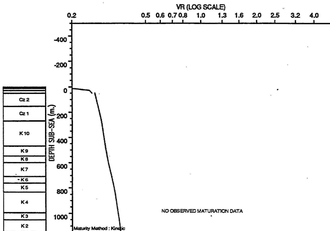
OBSERVED vs COMPUTED MATURITY PLOT : Cowle 1
