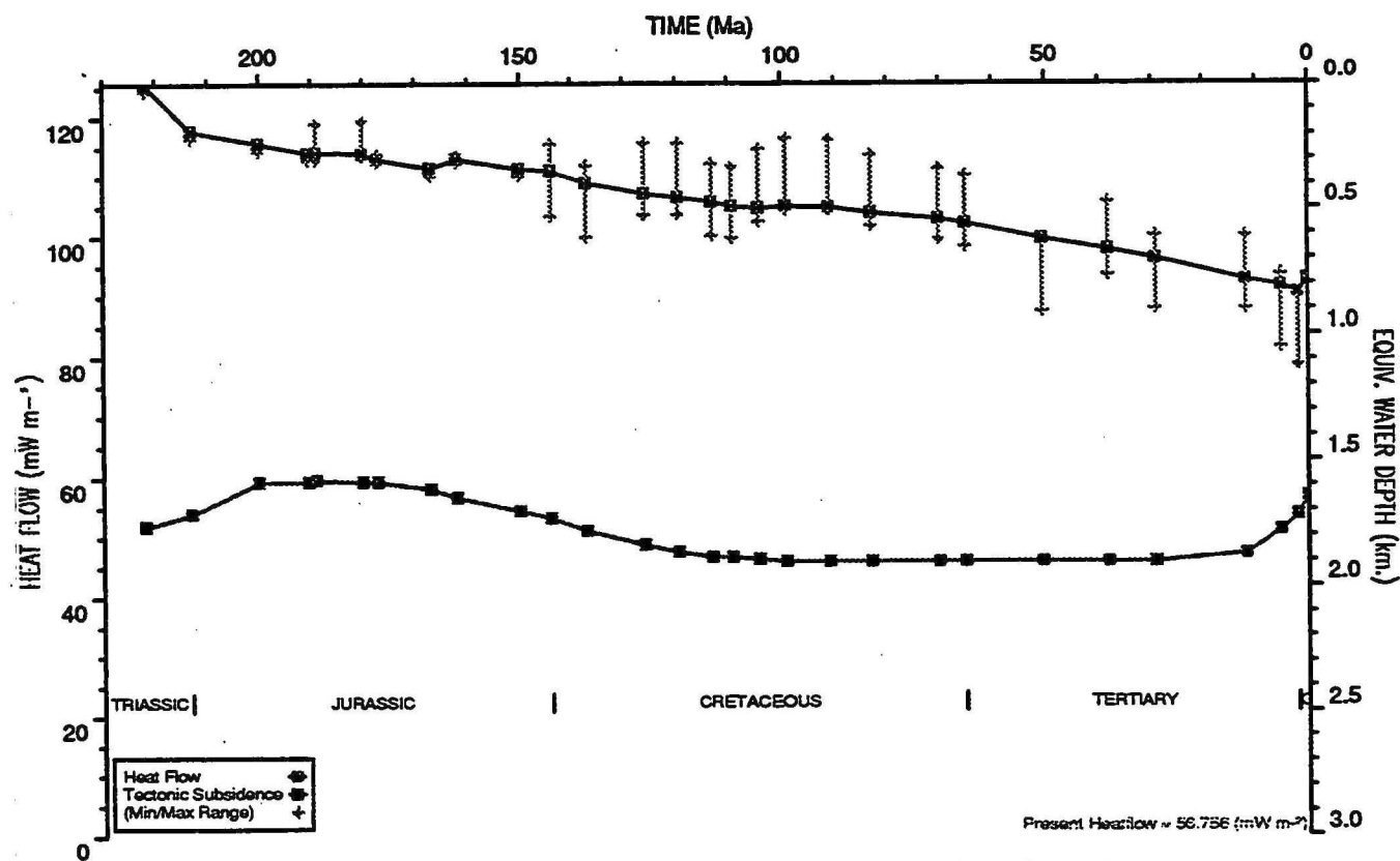
HEATFLOW AND TECTONIC SUBSIDENCE PLOT : Lynher 1
