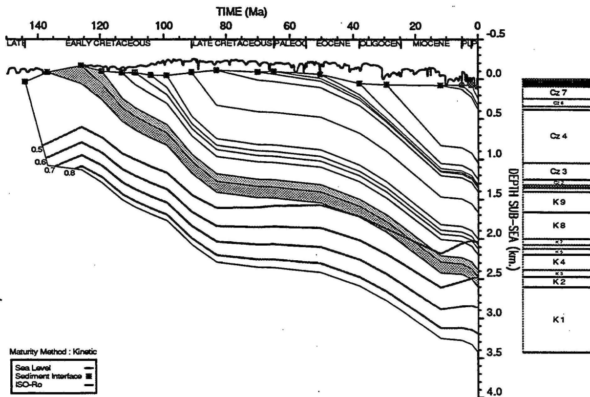
GEOHISTORY PLOT : West Barrow 2
