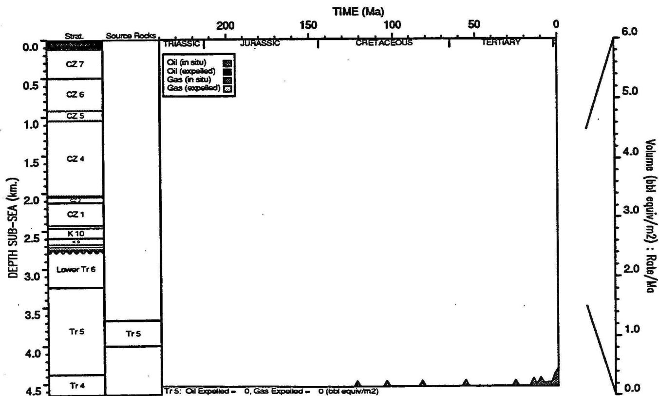
HYDROCARBON GENERATION PLOT : Goodwyn 6
