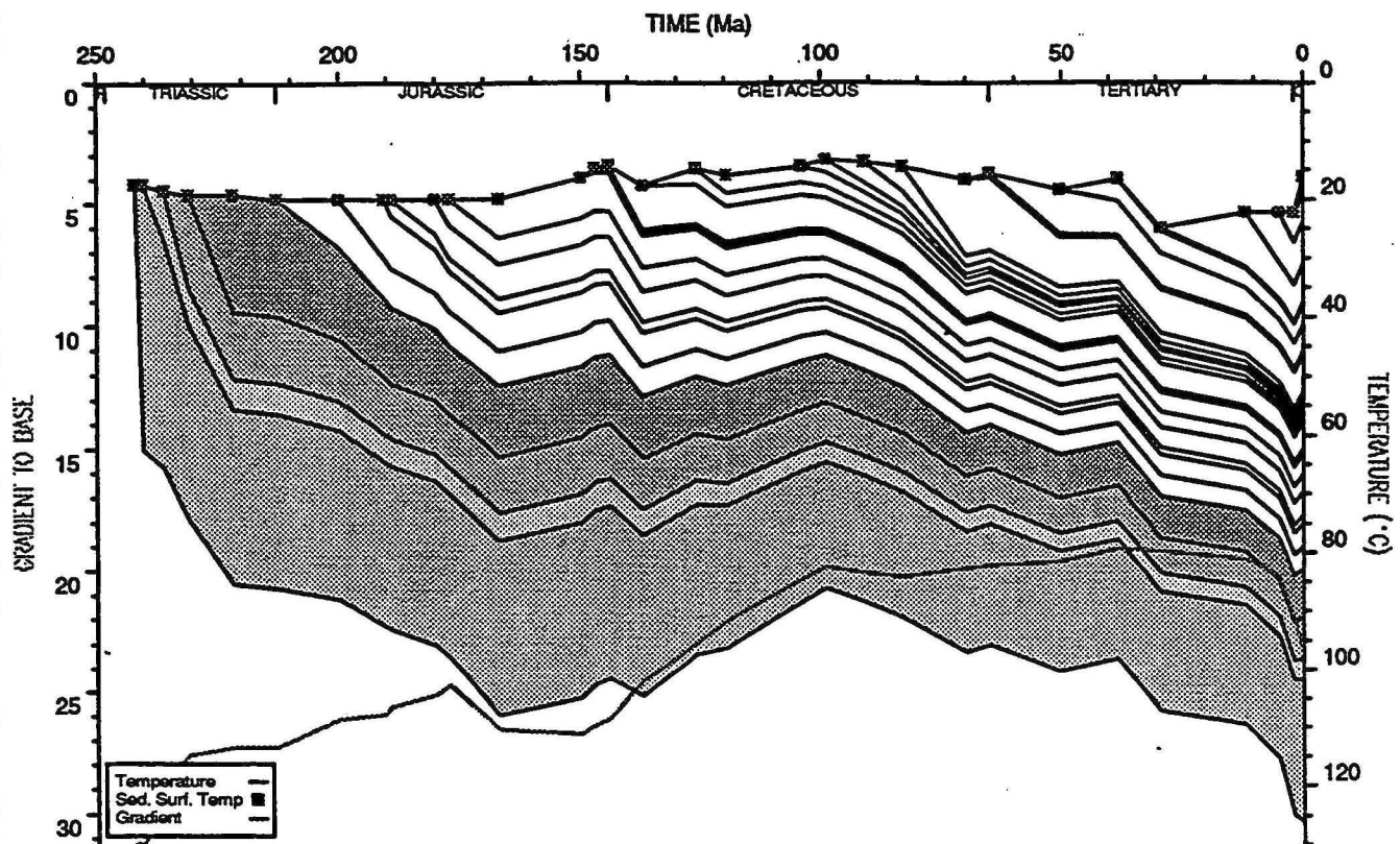
BED TEMPERATURE PLOT : Phoenix 1
