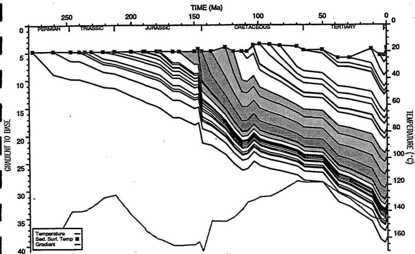
BED TEMPERATURE PLOT : Yampi 1
