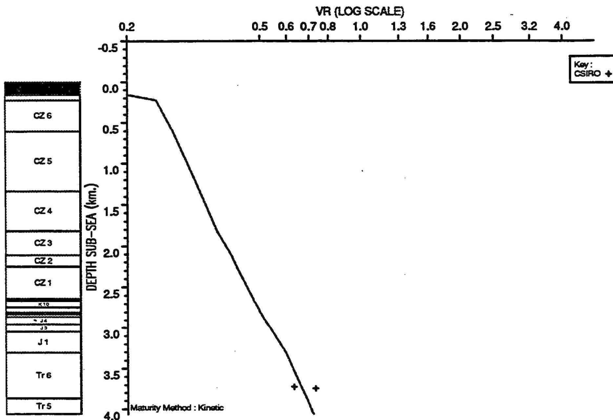
OBSERVED vs COMPUTED MATURITY PLOT : North Rankin 3
