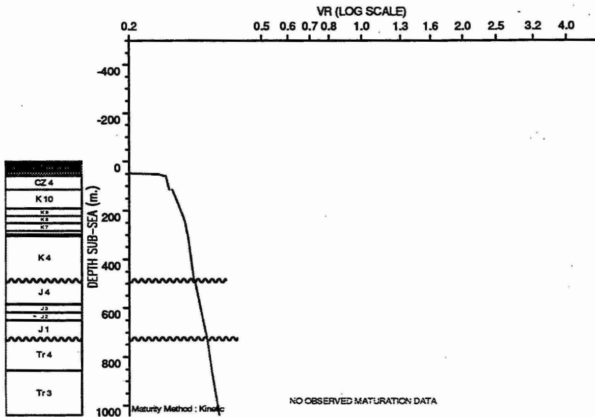
OBSERVED vs COMPUTED MATURITY PLOT : Strickland 1
