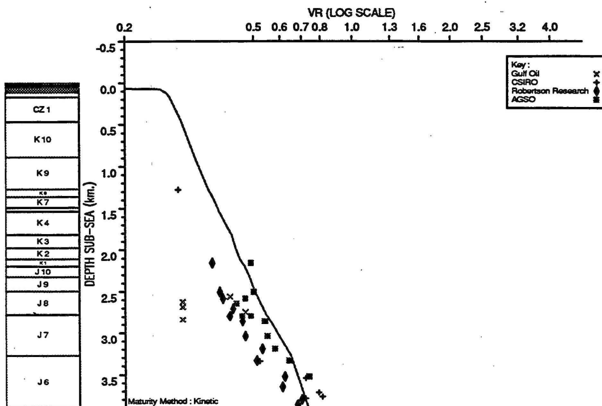
OBSERVED vs COMPUTED MATURITY PLOT : Rosemary 1
