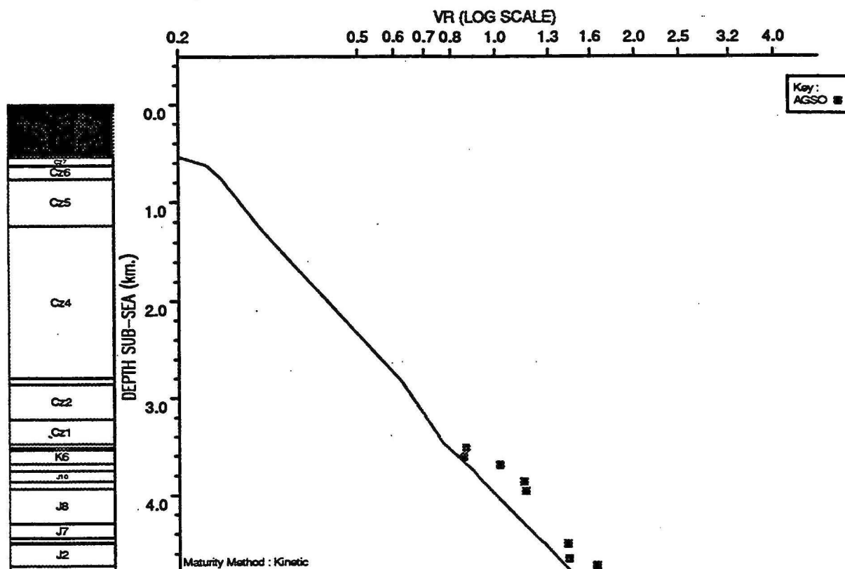
OBSERVED vs COMPUTED MATURITY PLOT : Buffon 1
