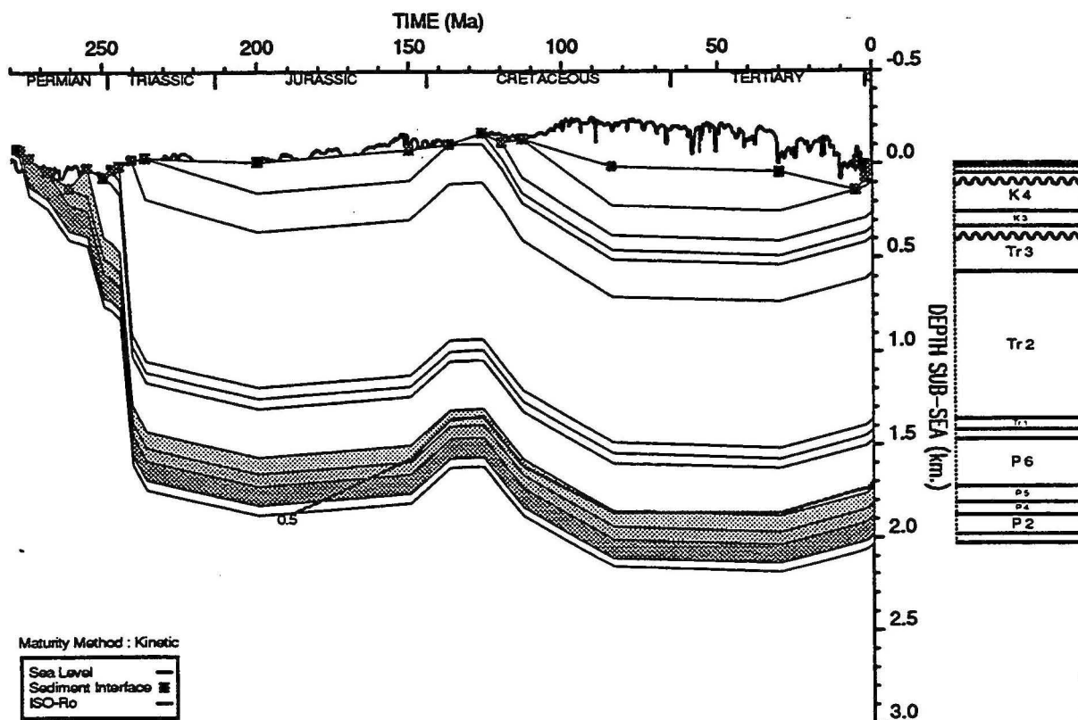
GEOHISTORY PLOT : Candace 1
