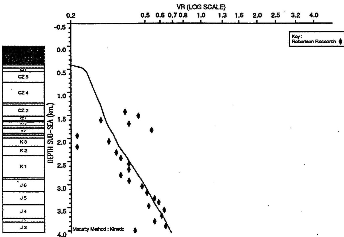
OBSERVED vs COMPUTED MATURITY PLOT : East Mermaid 1
