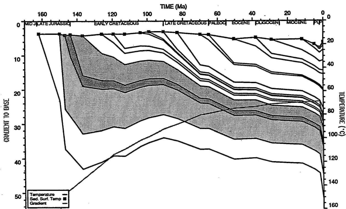
BED TEMPERATURE PLOT : Withnell 1
