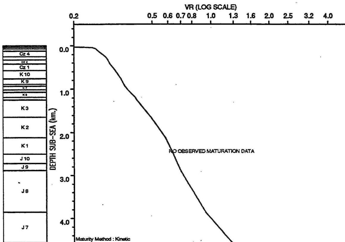
OBSERVED vs COMPUTED MATURITY PLOT : Bambra 2
