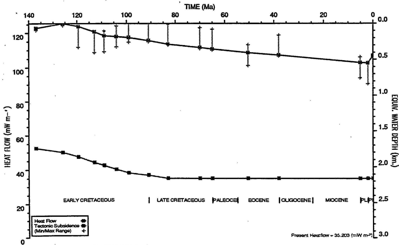
HEATFLOW AND TECTONIC SUBSIDENCE PLOT : Cowle 1
