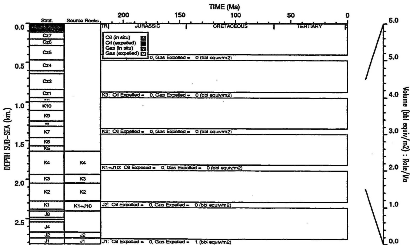
HYDROCARBON GENERATION PLOT : Lombardina 1
