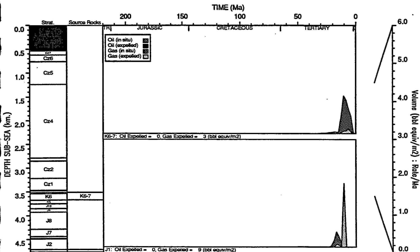
HYDROCARBON GENERATION PLOT : Buffon 1
