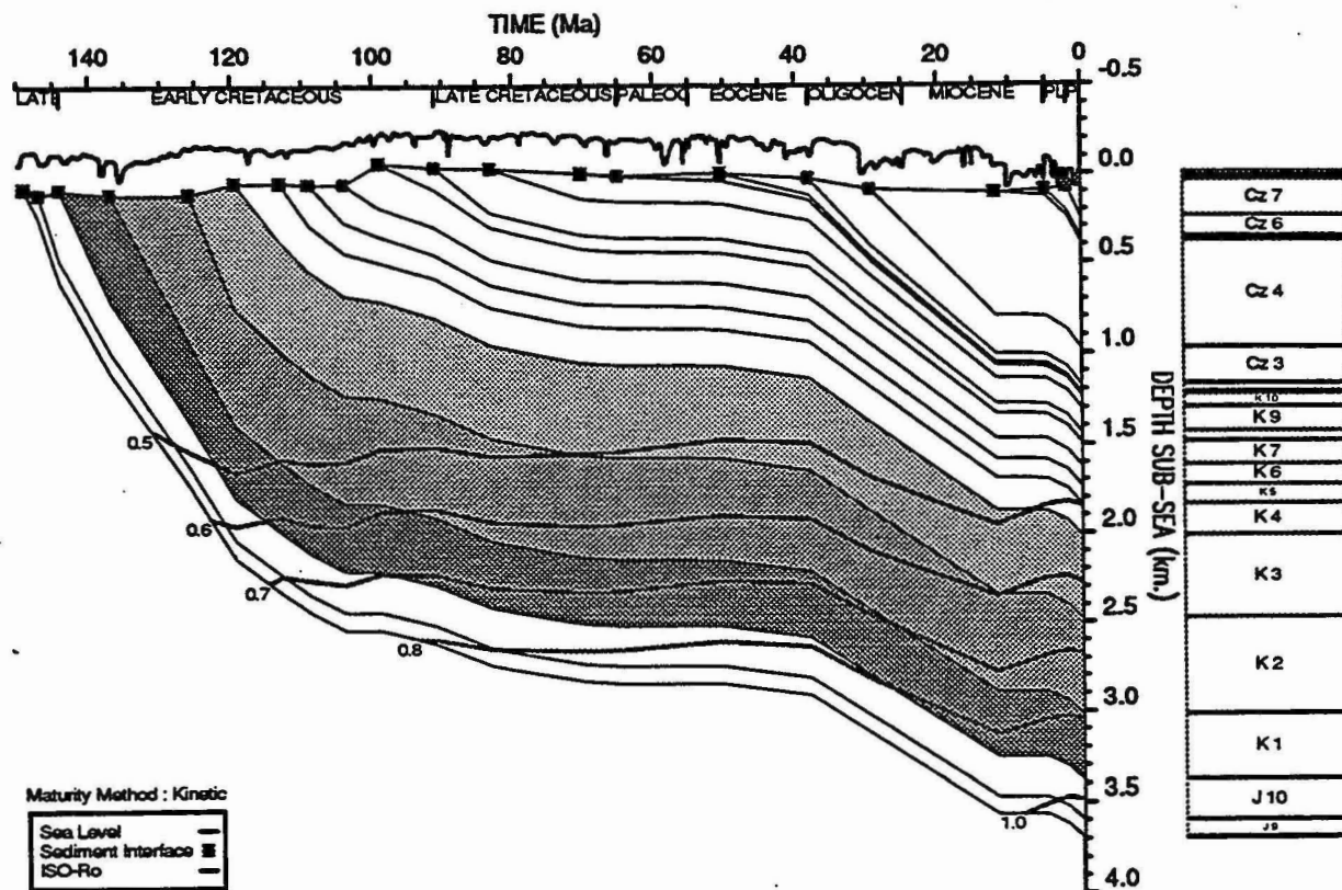
GEOHISTORY PLOT : Tryal Rocks 1
