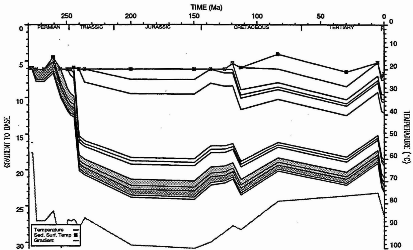
BED TEMPERATURE PLOT : Candace 1
