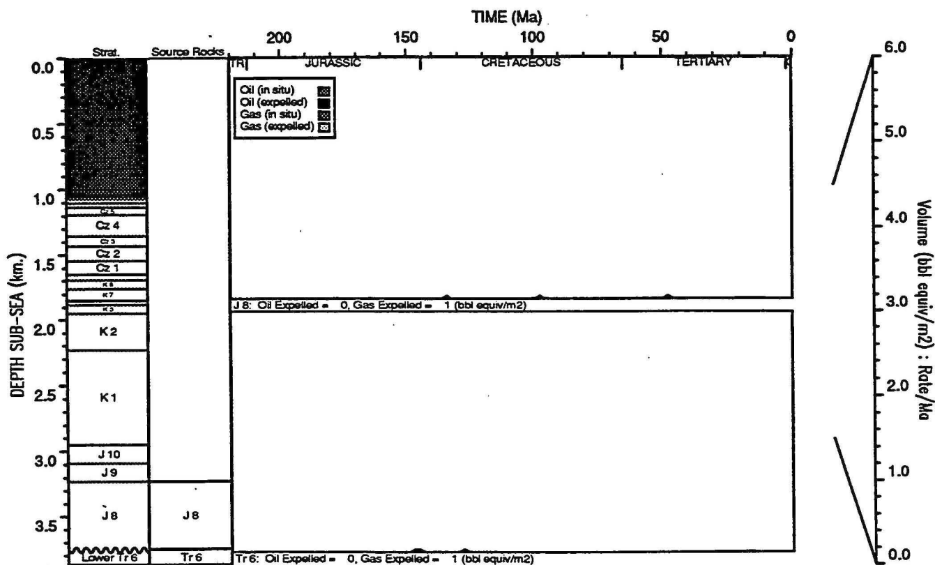
HYDROCARBON GENERATION PLOT : Resolution 1
