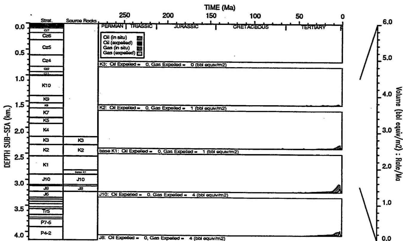
HYDROCARBON GENERATION PLOT : Yampi 1
