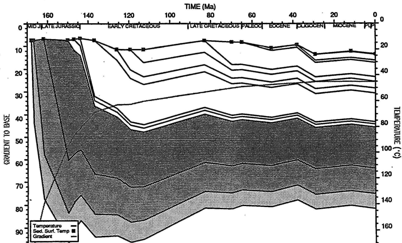
BED TEMPERATURE PLOT : Barrow Deep 1
