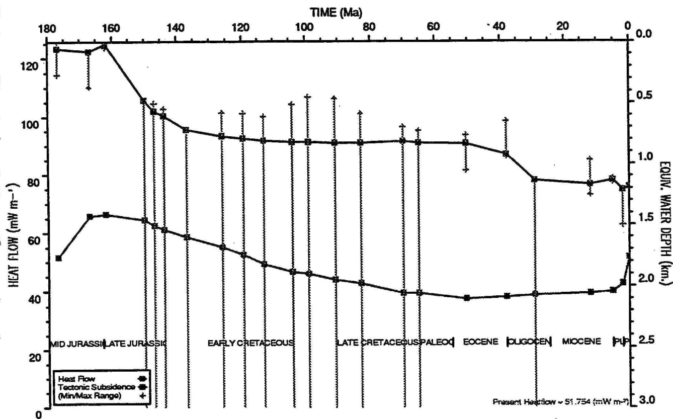
HEATFLOW AND TECTONIC SUBSIDENCE PLOT : Madeleine 1
