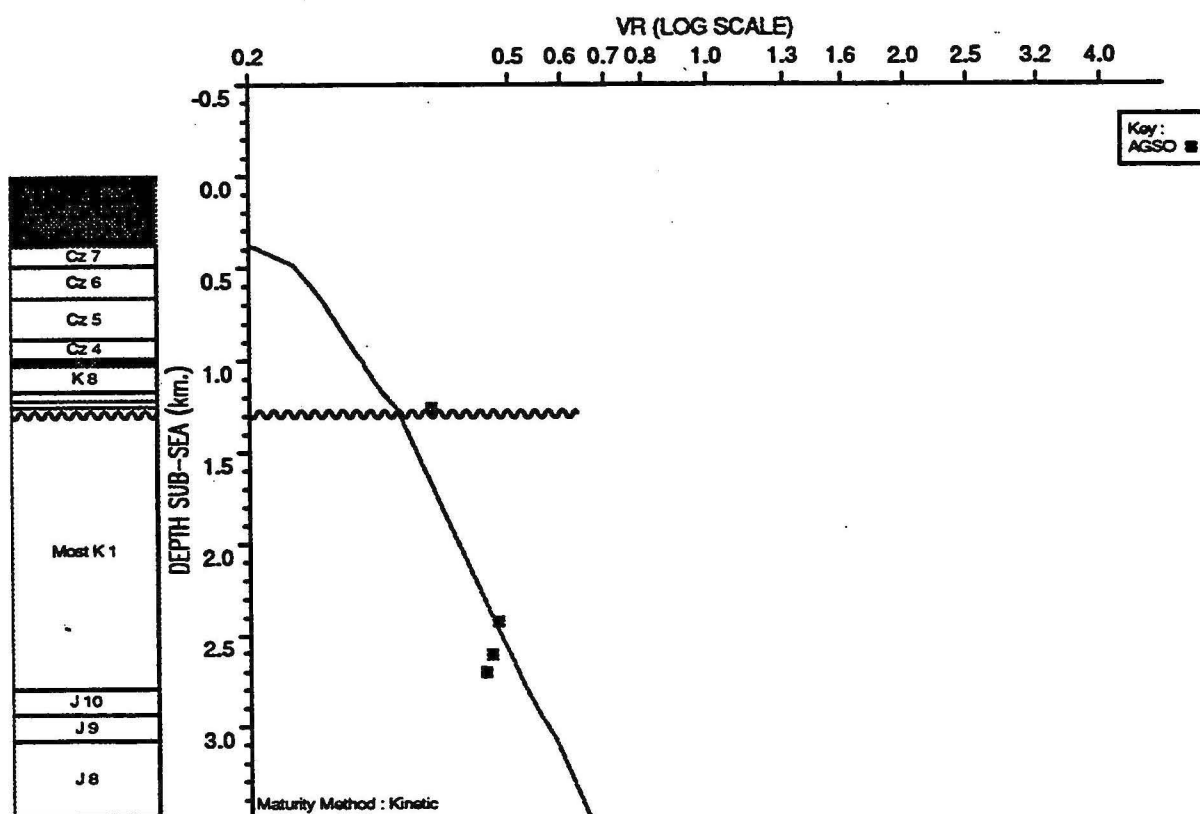
OBSERVED vs COMPUTED MATURITY PLOT : Novara 1
