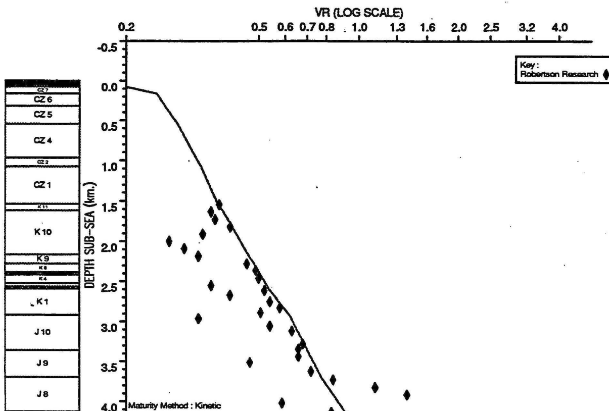
OBSERVED vs COMPUTED MATURITY PLOT : Dampier 1
