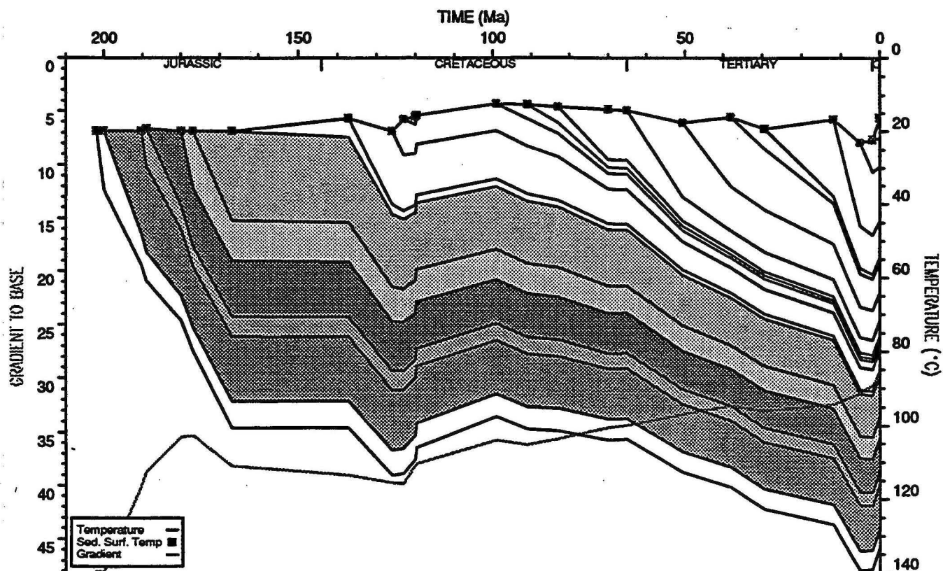
BED TEMPERATURE PLOT : Picard 1
