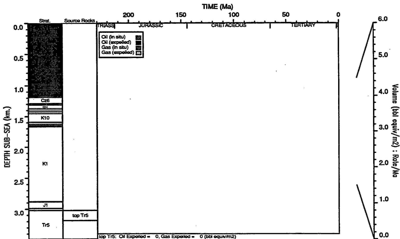
HYDROCARBON GENERATION PLOT : Sirius 1
