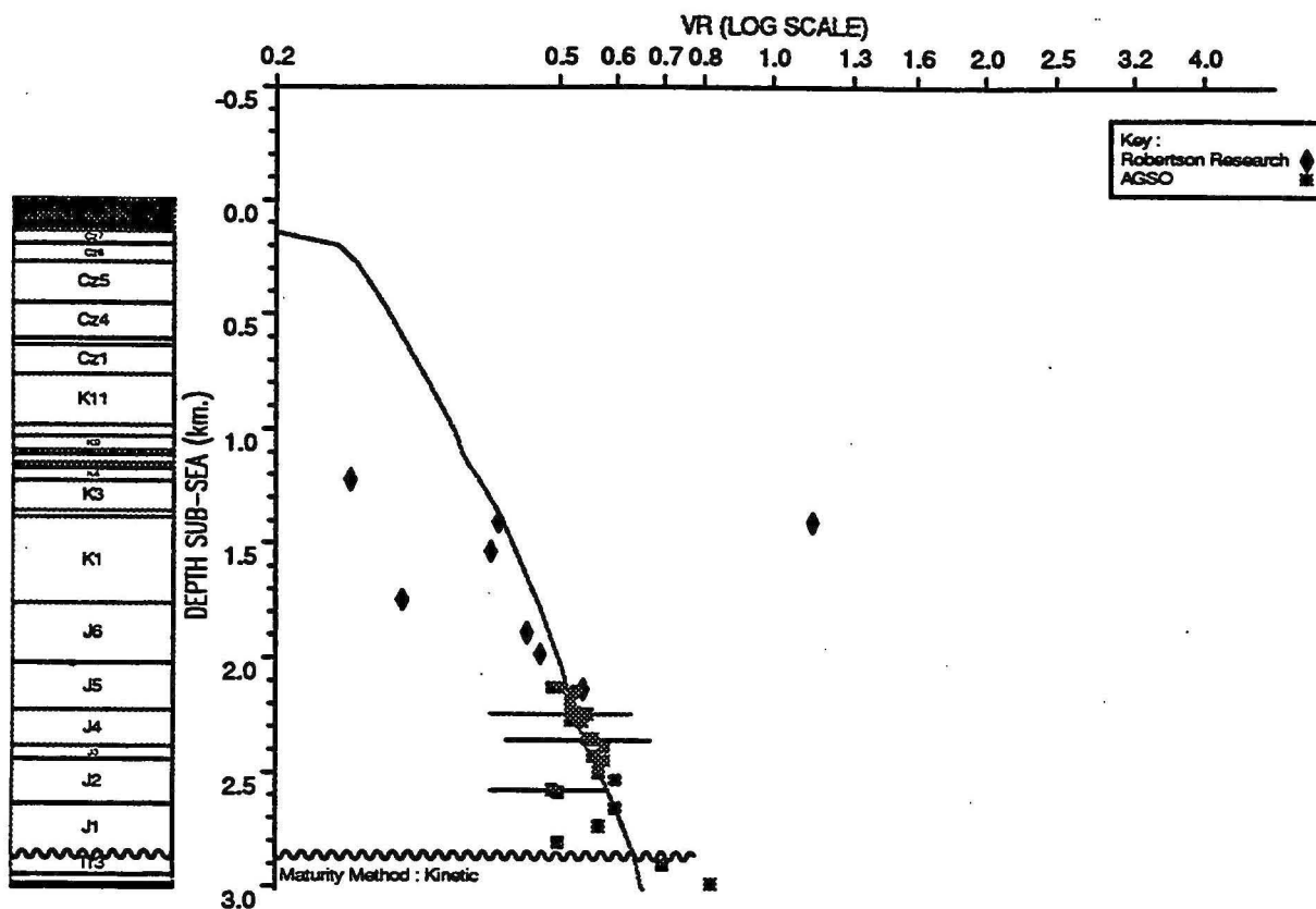
OBSERVED vs COMPUTED MATURITY PLOT : Bedout 1
