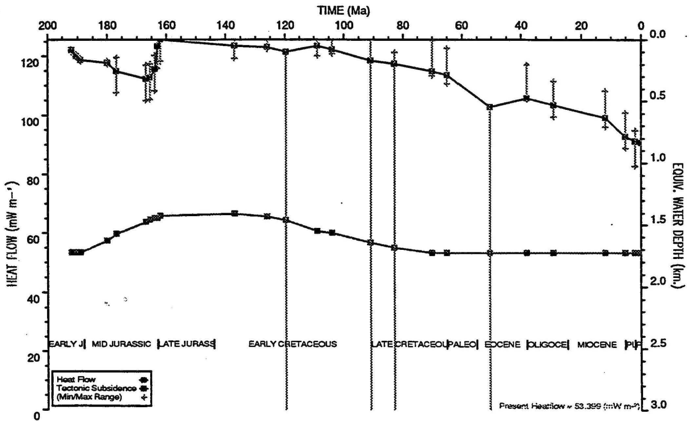
HEATFLOW AND TECTONIC SUBSIDENCE PLOT : Ronsard 1
