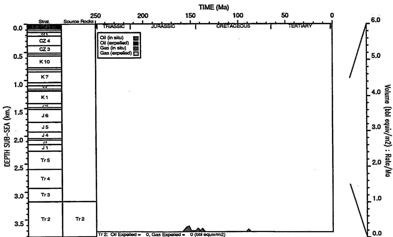
HYDROCARBON GENERATION PLOT : Keraudren 1
