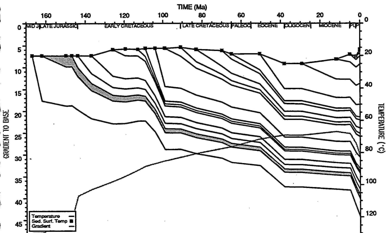
BED TEMPERATURE PLOT : Buccaneer 1
