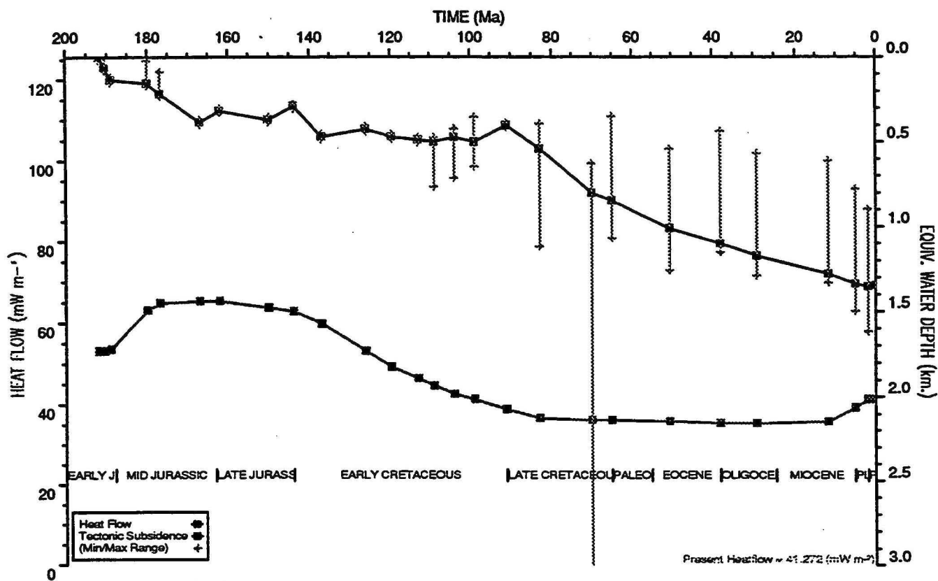
HEATFLOW AND TECTONIC SUBSIDENCE PLOT : East Mermaid 1
