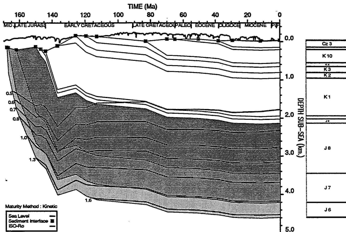
GEOHISTORY PLOT : Barrow Deep 1
