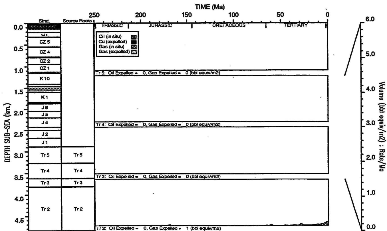
HYDROCARBON GENERATION PLOT : Phoenix 1
