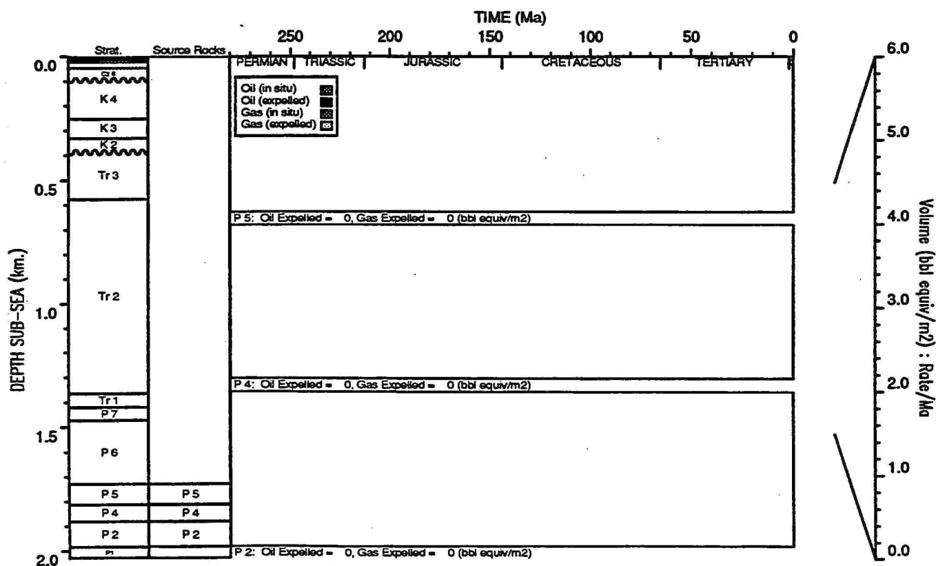
HYDROCARBON GENERATION PLOT : Candace 1
