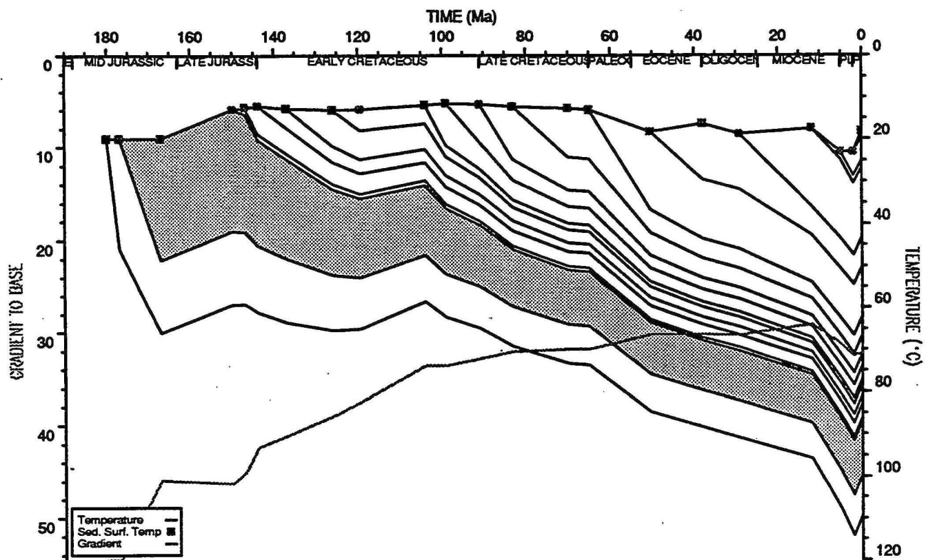
BED TEMPERATURE PLOT : Talisman 1
