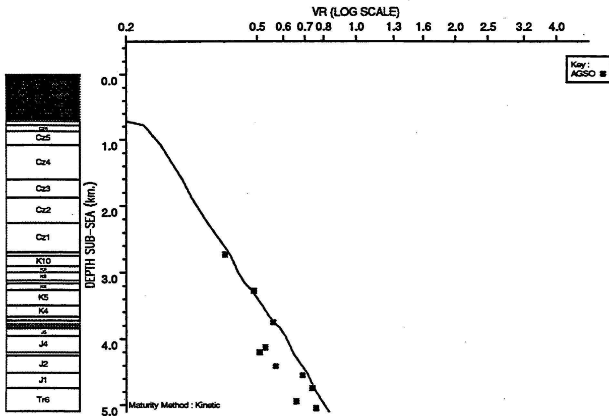
OBSERVED vs COMPUTED MATURITY PLOT : Barcoo 1
