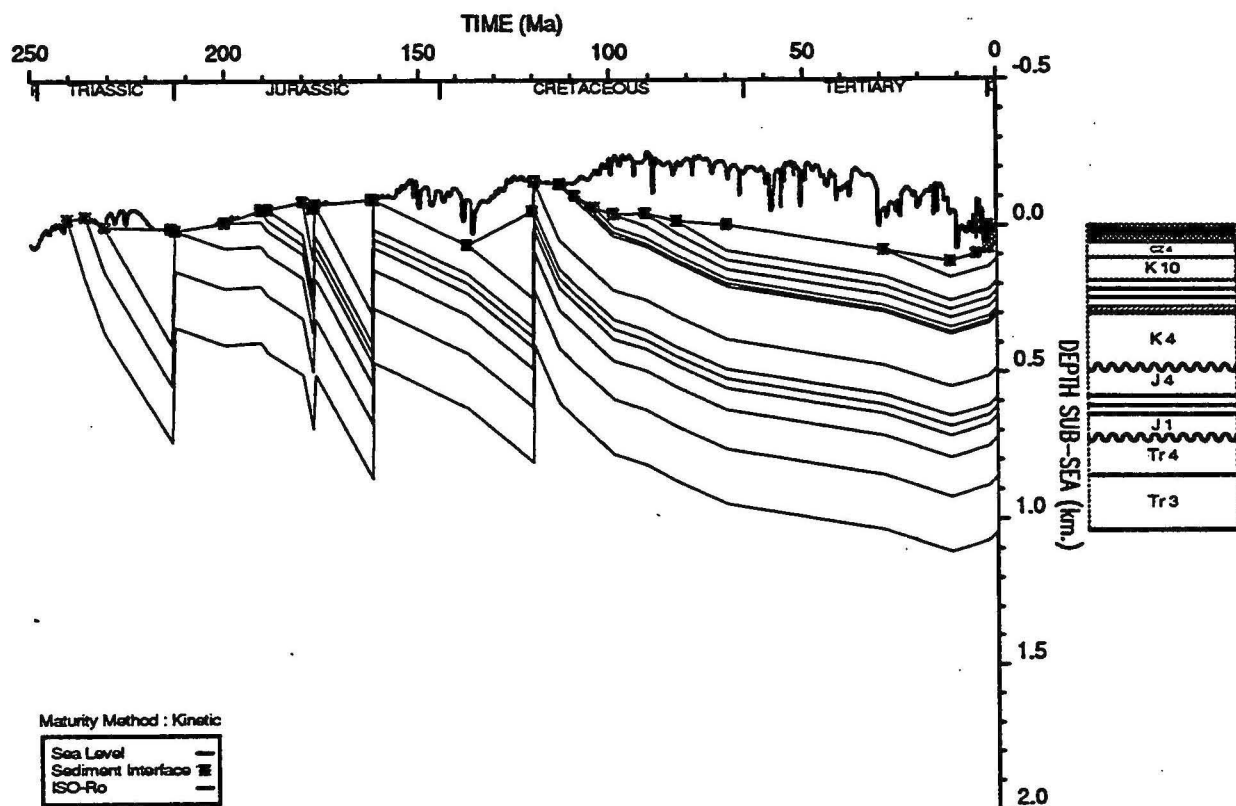
GEOHISTORY PLOT : Strickland 1
