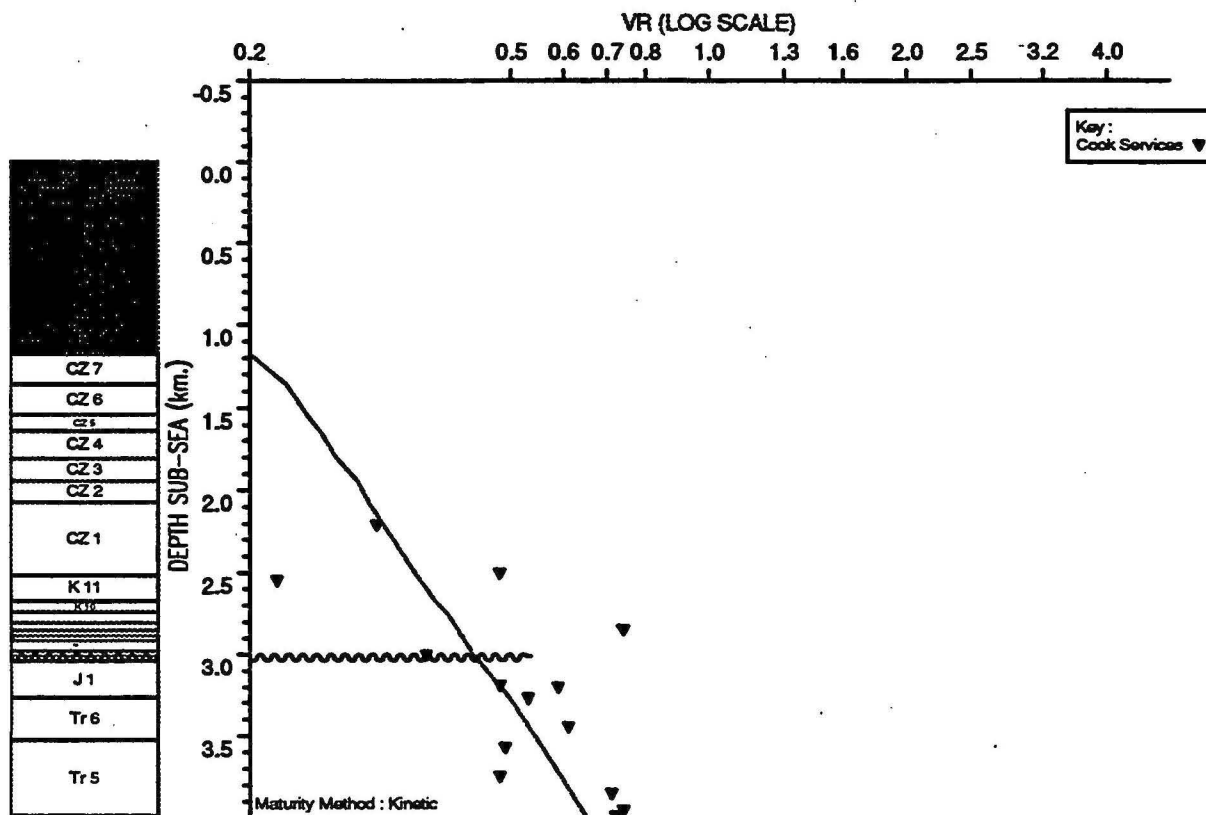
OBSERVED vs COMPUTED MATURITY PLOT : Saturn 1
