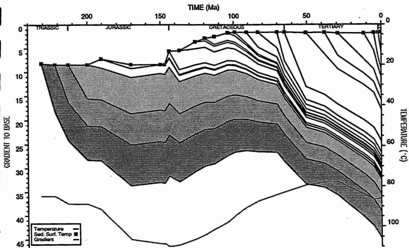
BED TEMPERATURE PLOT : Saturn 1
