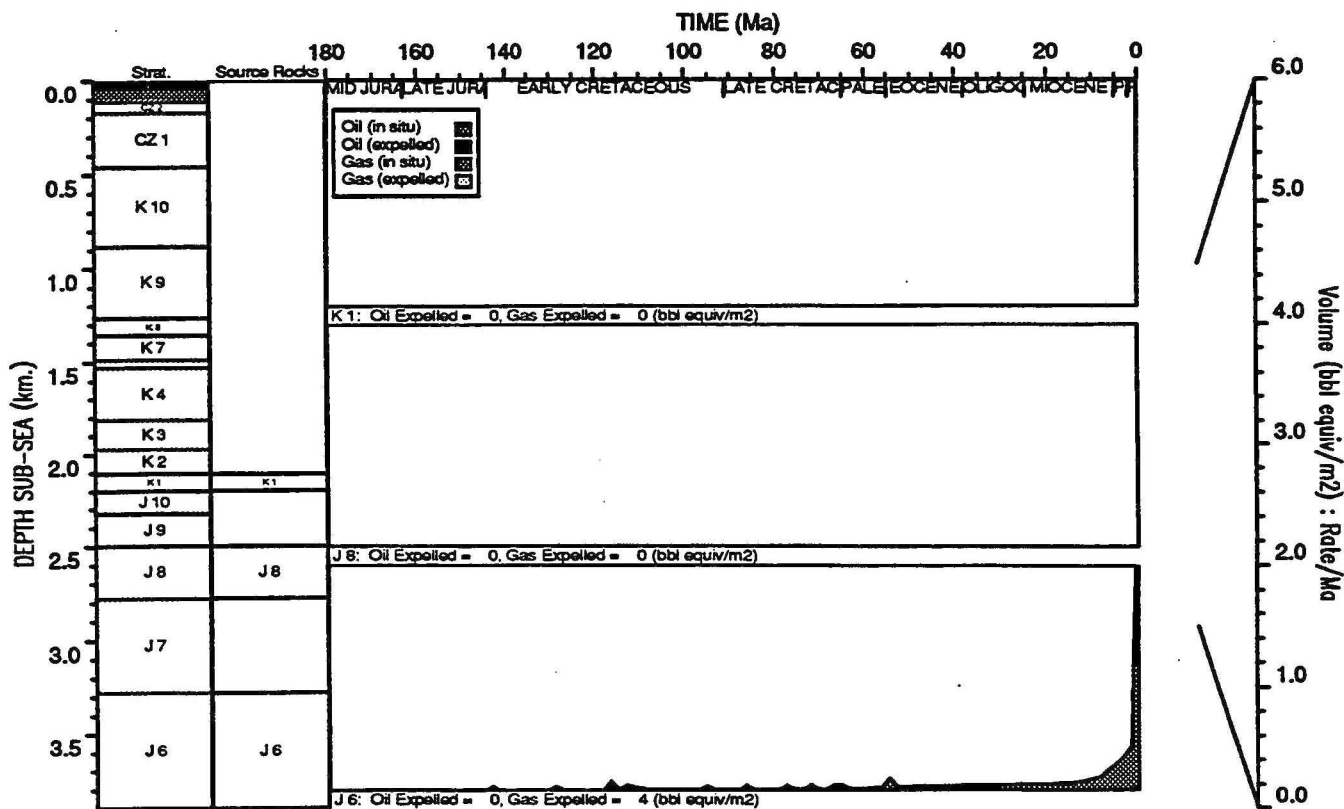
HYDROCARBON GENERATION PLOT : Rosemary 1
