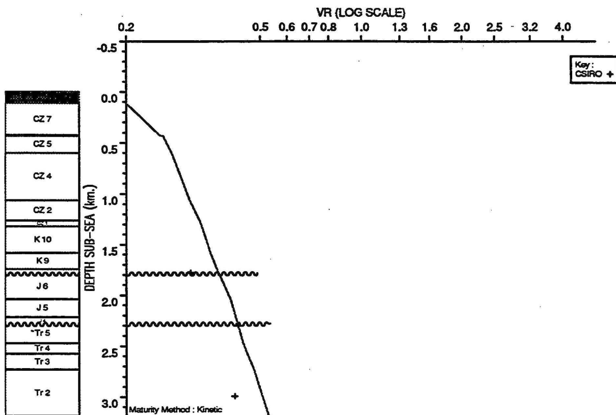
OBSERVED vs COMPUTED MATURITY PLOT : Cossigny 1
