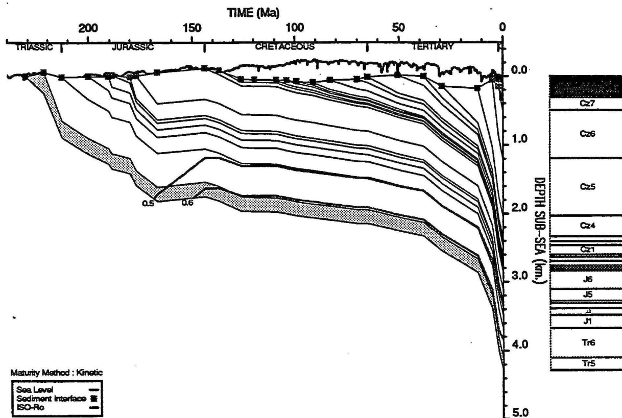
GEOHISTORY PLOT : Brigadier 1
