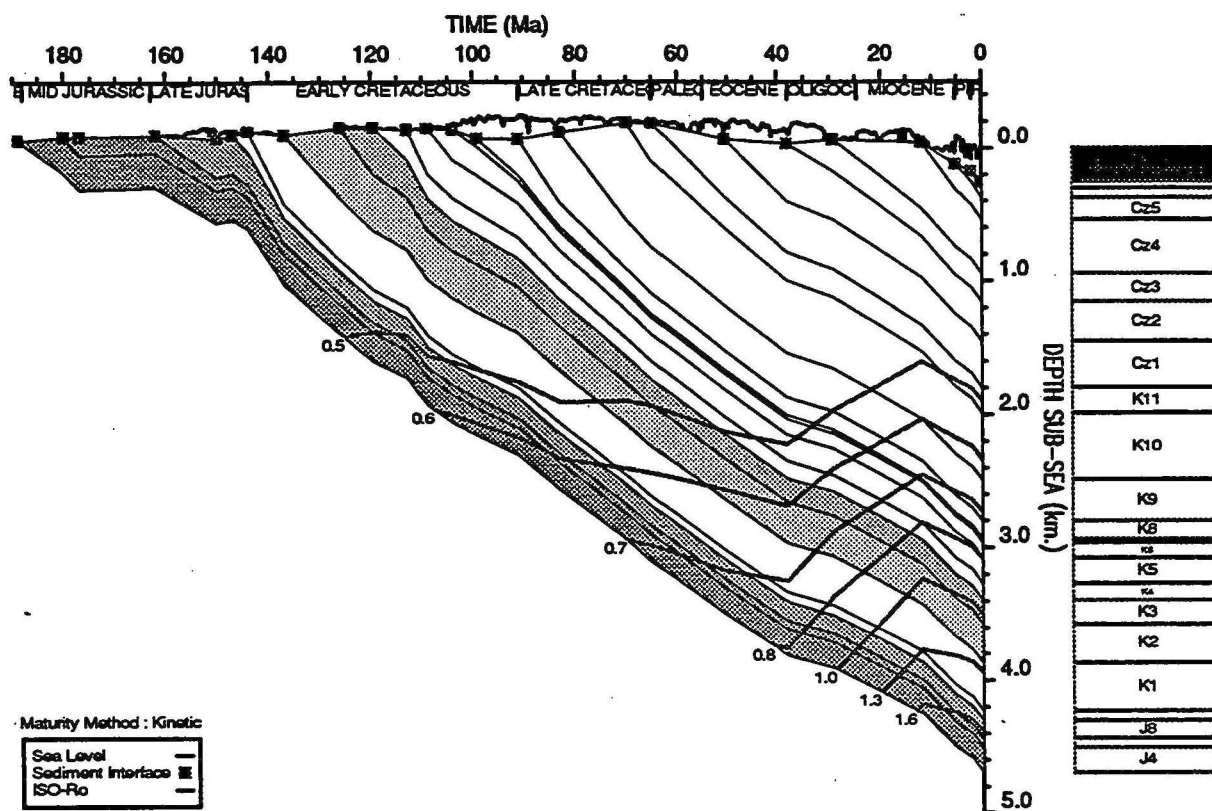
GEOHISTORY PLOT : Brewster 1A
