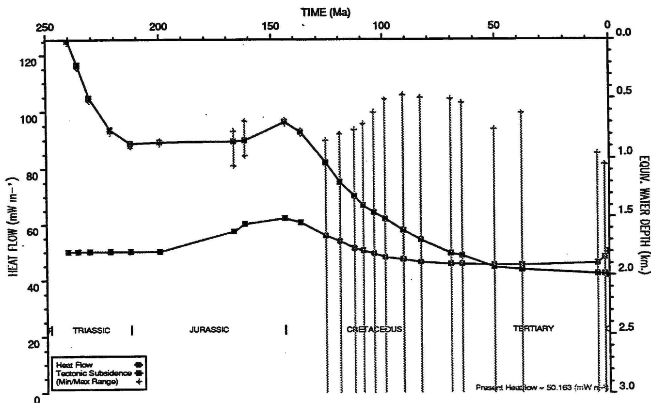
HEATFLOW AND TECTONIC SUBSIDENCE PLOT : Jupiter 1
