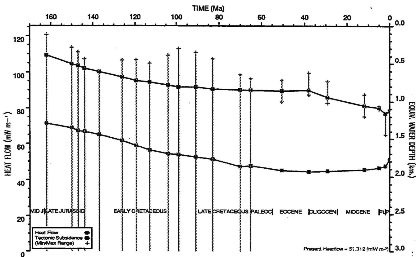
HEATFLOW AND TECTONIC SUBSIDENCE PLOT : Dampier 1
