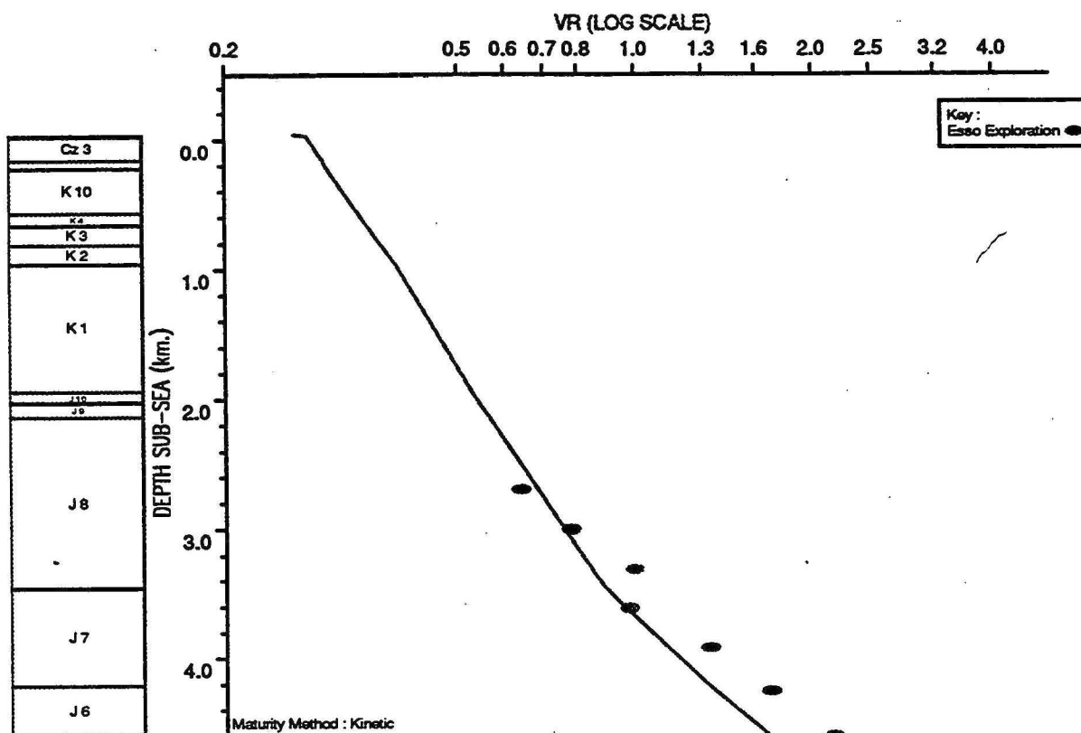
OBSERVED vs COMPUTED MATURITY PLOT : Barrow Deep 1
