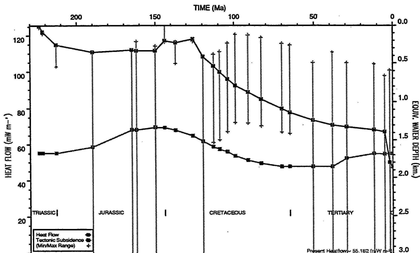
HEATFLOW AND TECTONIC SUBSIDENCE PLOT : Zeewulf 1
