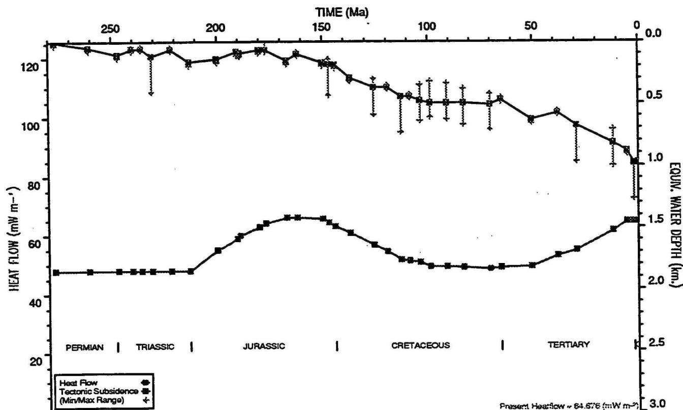
HEATFLOW AND TECTONIC SUBSIDENCE PLOT : Yampi 1
