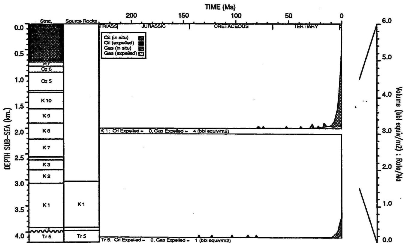
HYDROCARBON GENERATION PLOT : Zeepaard 1
