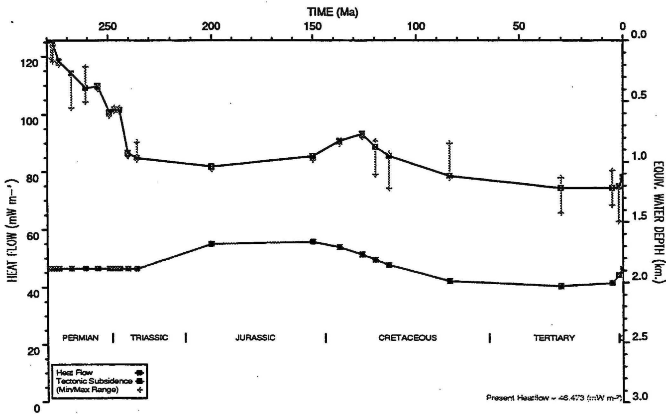
HEATFLOW AND TECTONIC SUBSIDENCE PLOT : Candace 1
