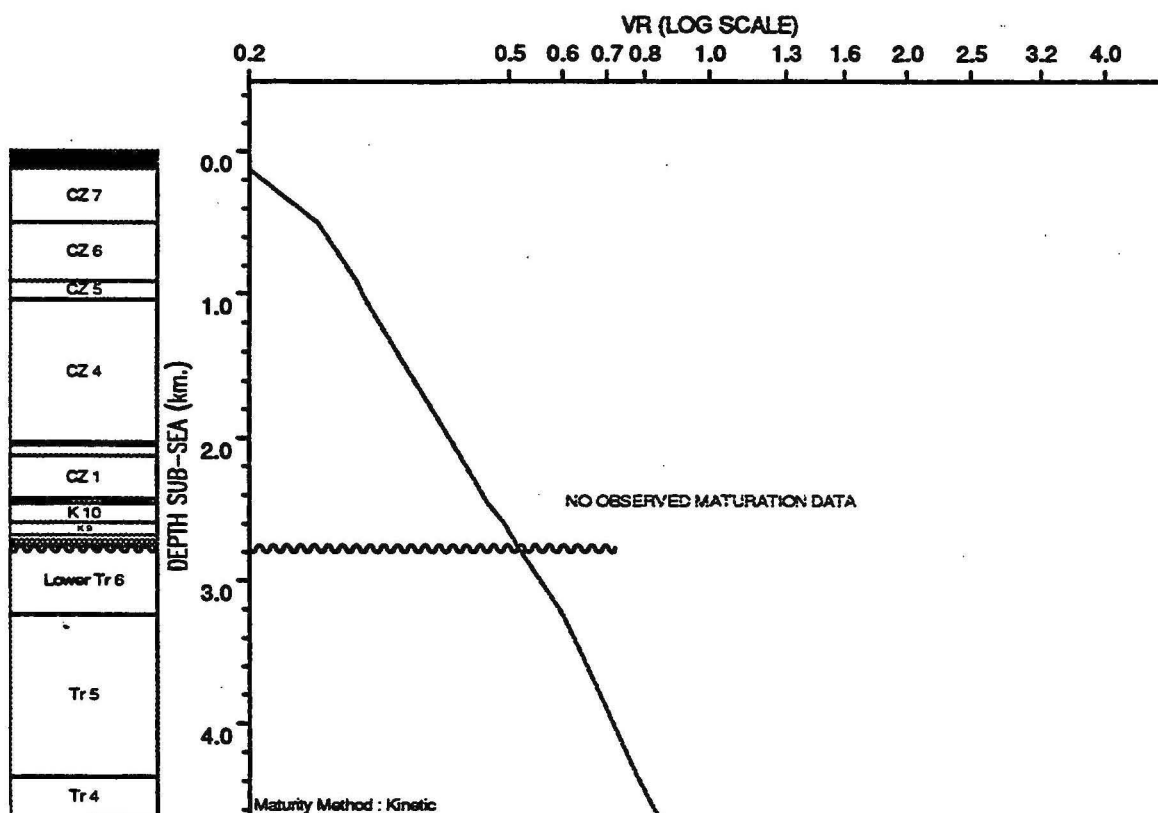
OBSERVED vs COMPUTED MATURITY PLOT : Goodwyn 6
