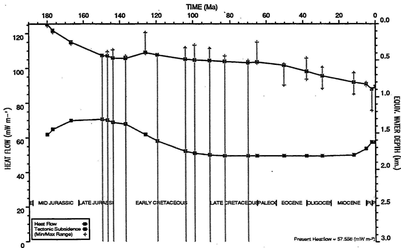
HEATFLOW AND TECTONIC SUBSIDENCE PLOT : Talisman 1
