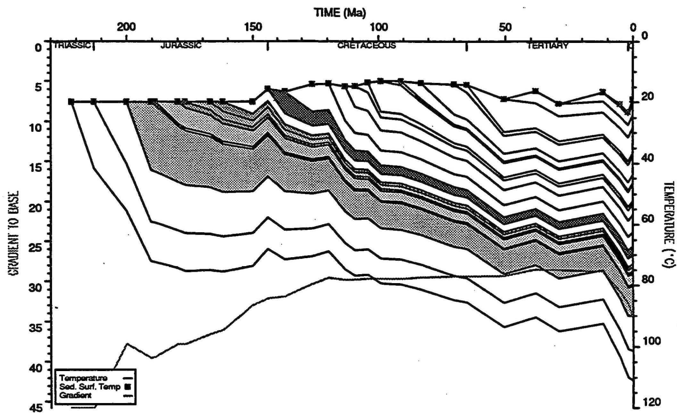
BED TEMPERATURE PLOT : Lynher 1
