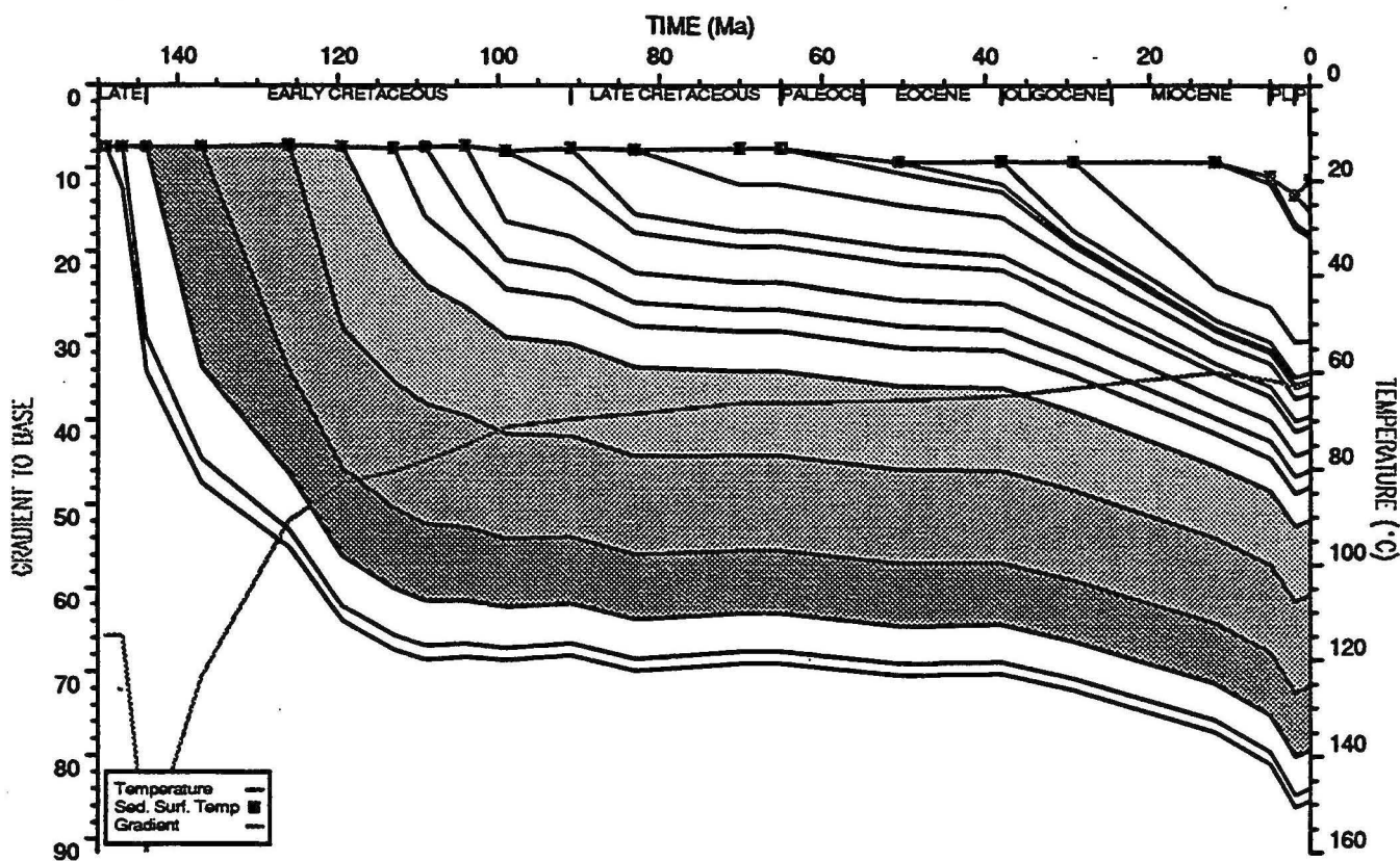
BED TEMPERATURE PLOT : Tryal Rocks 1
