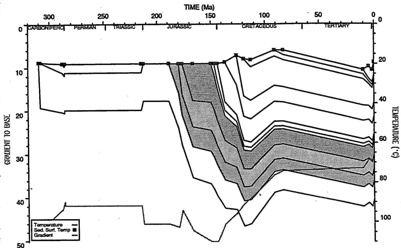
BED TEMPERATURE PLOT : Lacepede 1A
