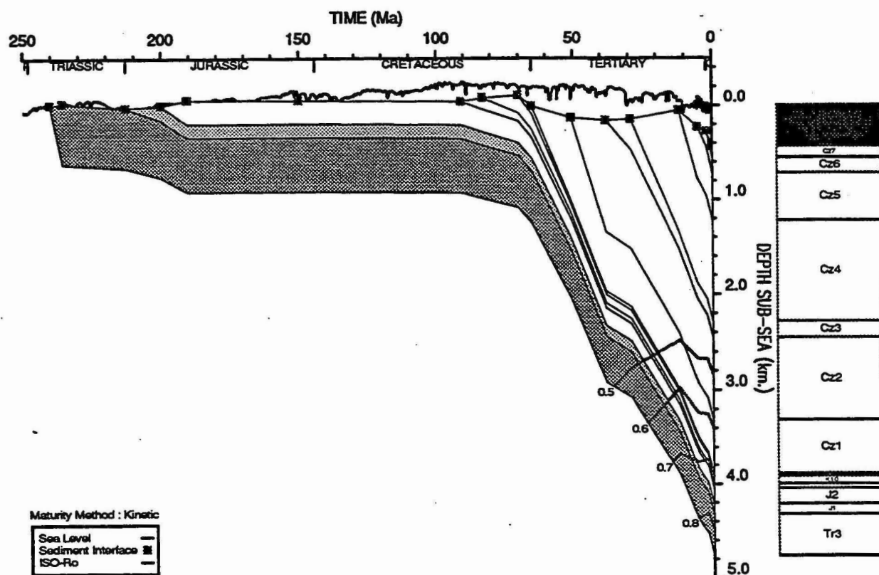
GEOHISTORY PLOT : North Scott Reef 1
