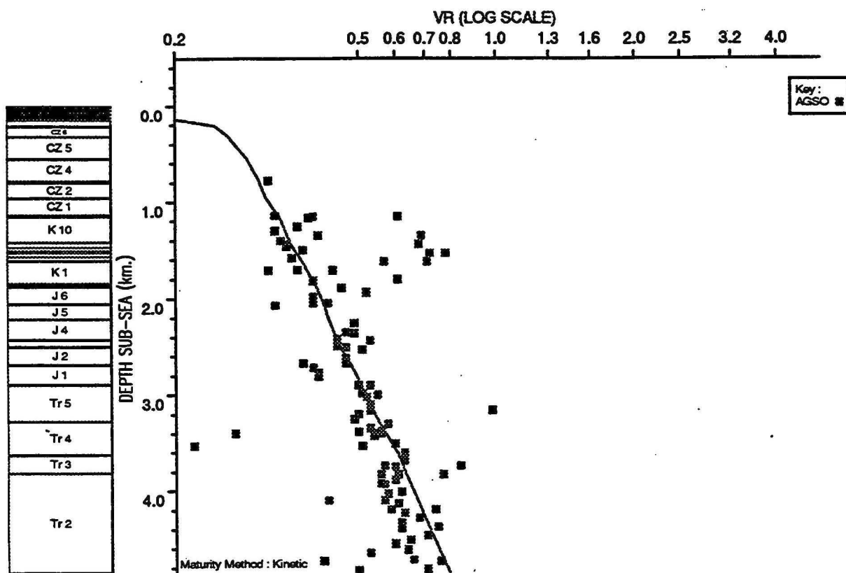
OBSERVED vs COMPUTED MATURITY PLOT : Phoenix 1
