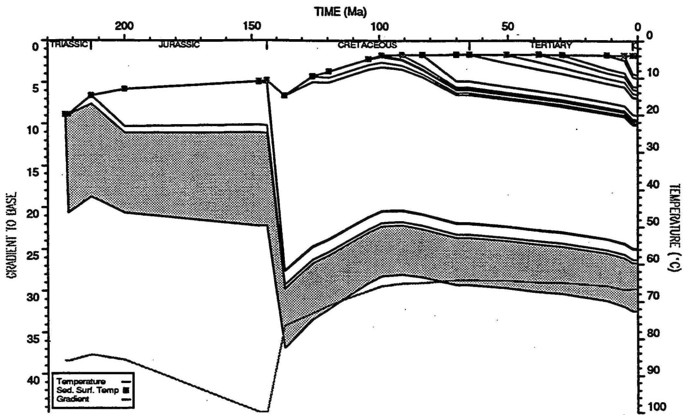
BED TEMPERATURE PLOT : Sirius 1
