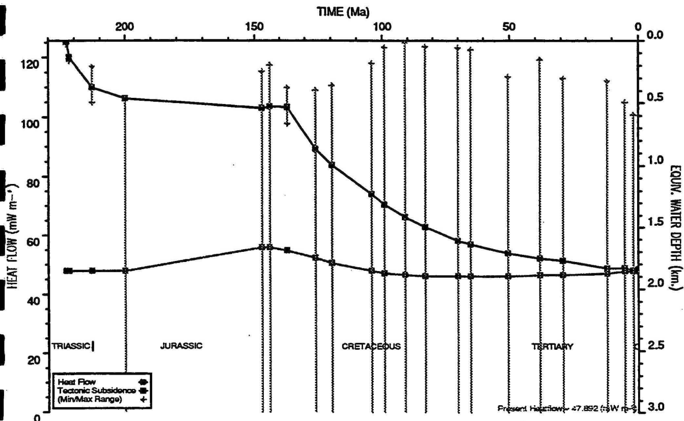
HEATFLOW AND TECTONIC SUBSIDENCE PLOT : Sirius 1
