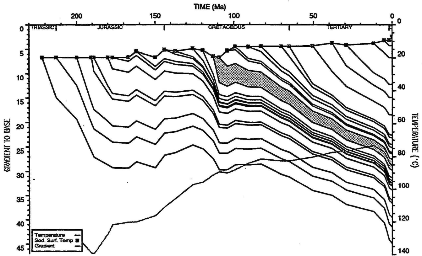
BED TEMPERATURE PLOT : Barcoo 1
