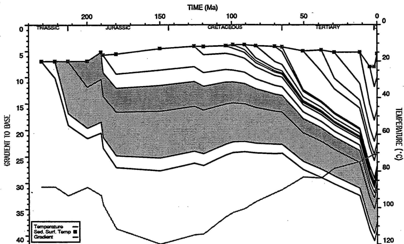
BED TEMPERATURE PLOT : North Rankin 3
