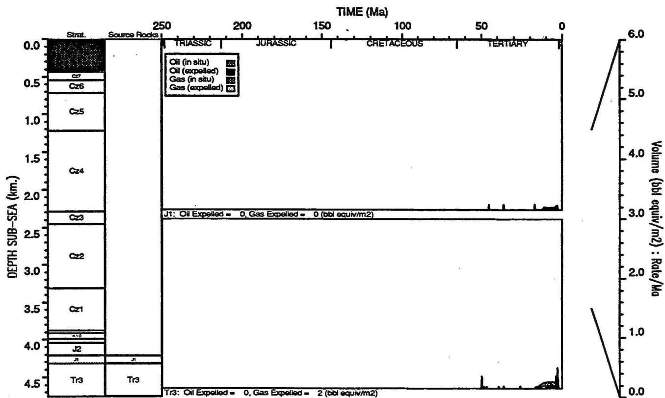
HYDROCARBON GENERATION PLOT : North Scott Reef 1
