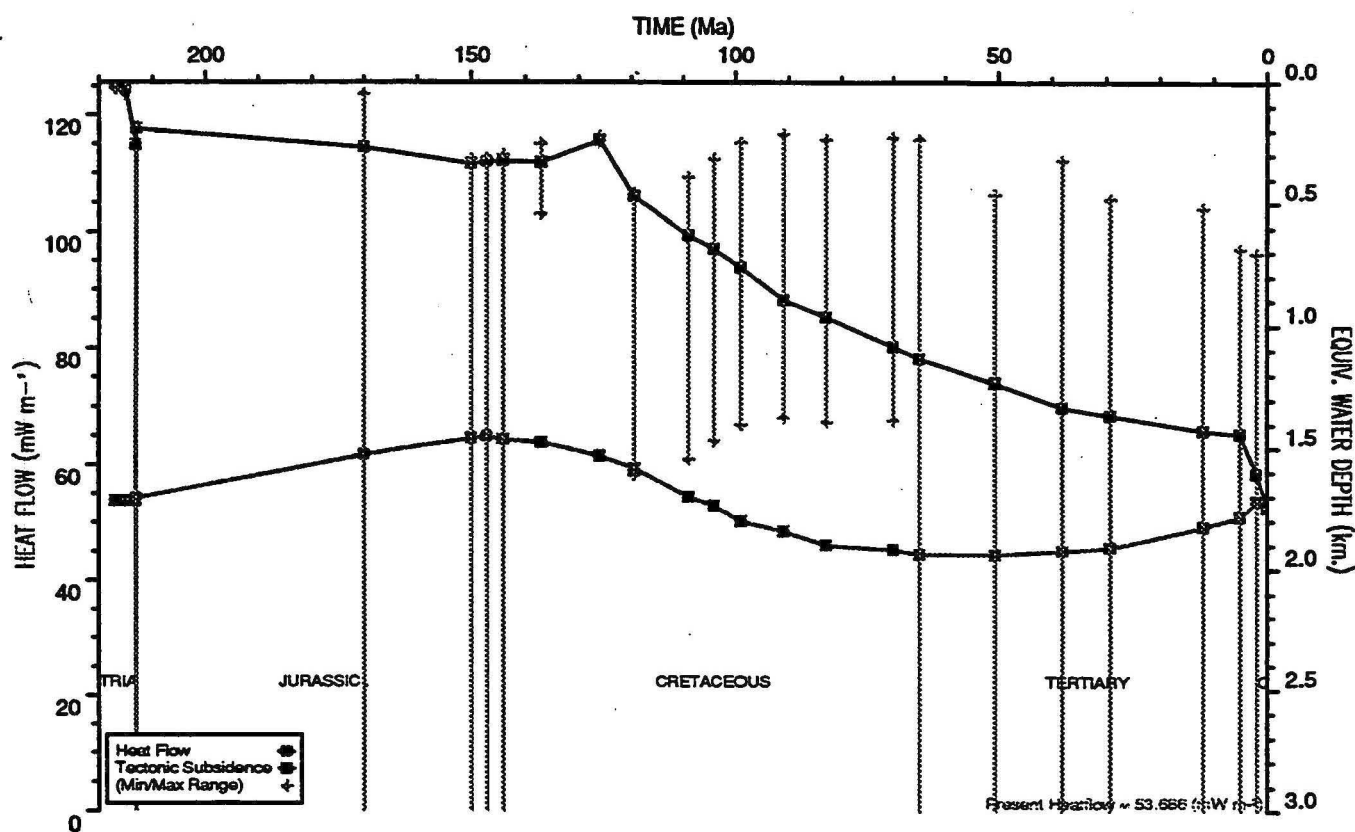
HEATFLOW AND TECTONIC SUBSIDENCE PLOT : Resolution 1
