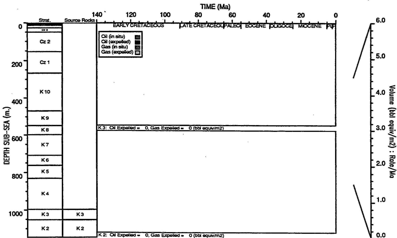
HYDROCARBON GENERATION PLOT : Cowle 1
