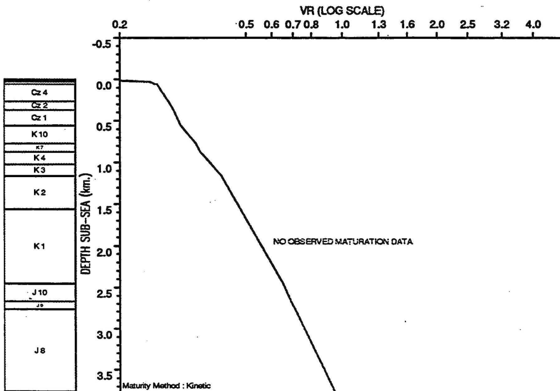
OBSERVED vs COMPUTED MATURITY PLOT : South Pepper 1
