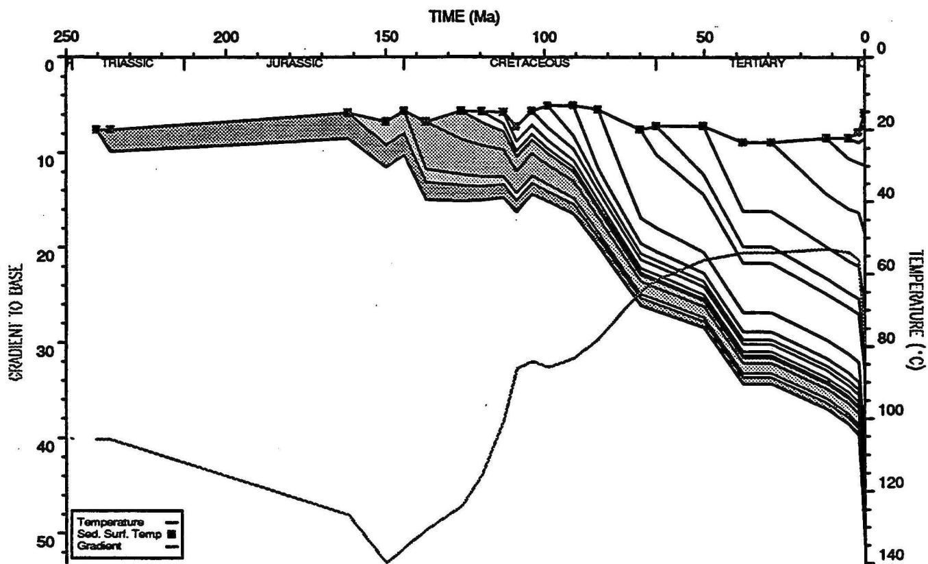
BED TEMPERATURE PLOT : Discorbis 1
