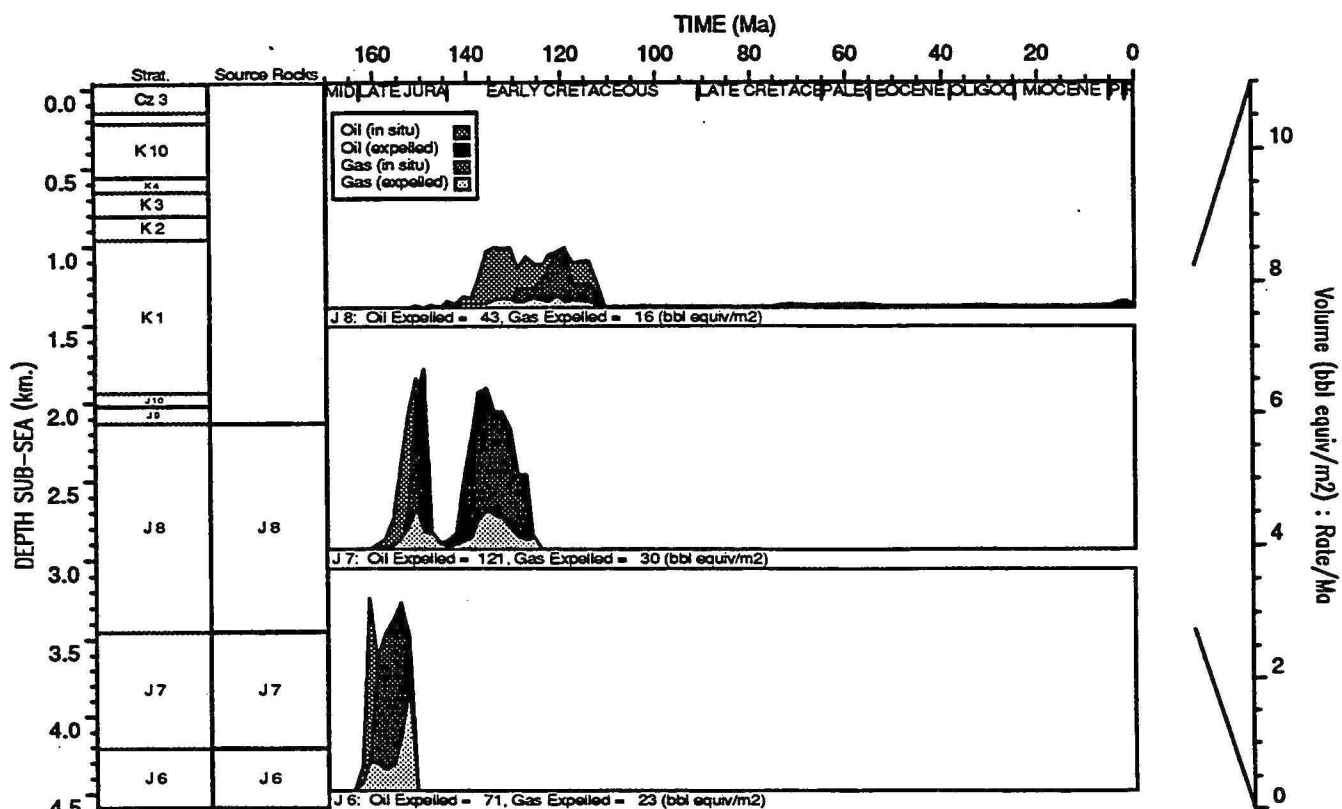
HYDROCARBON GENERATION PLOT : Barrow Deep 1
