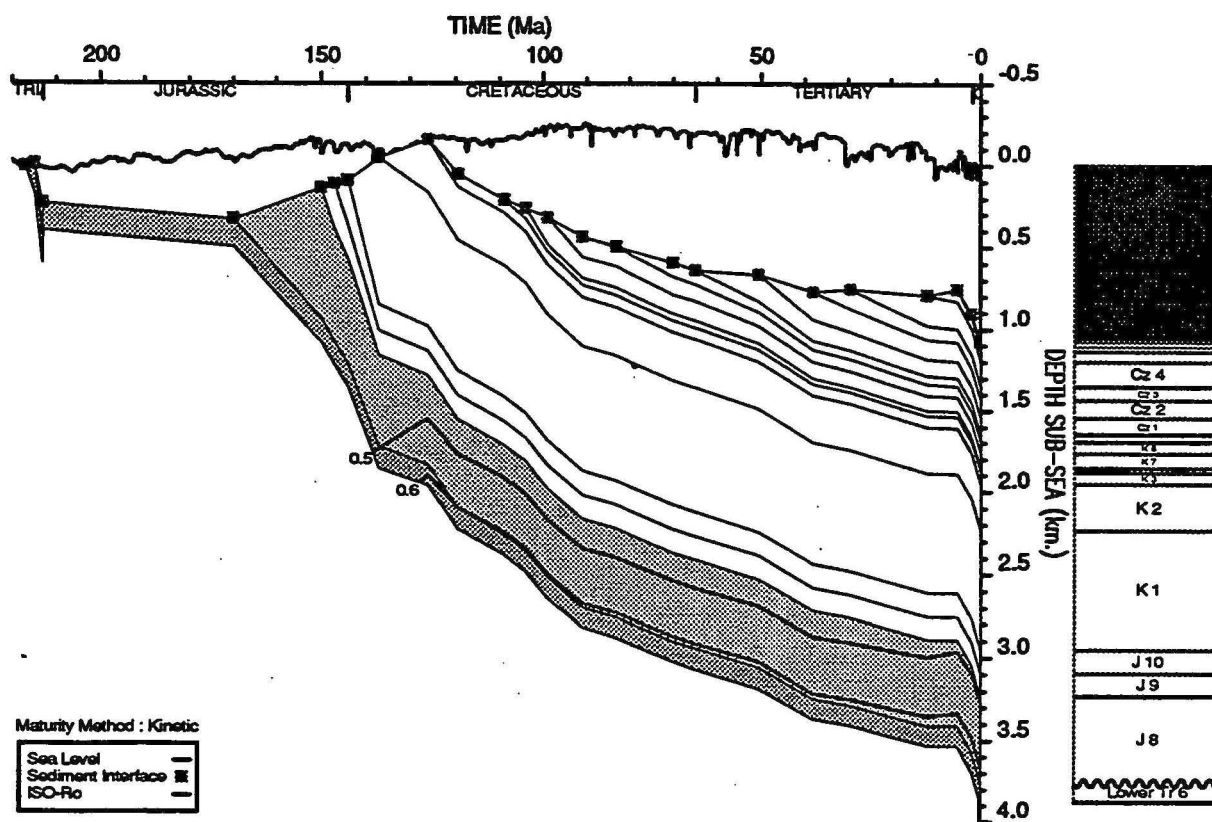
GEOHISTORY PLOT : Resolution 1
