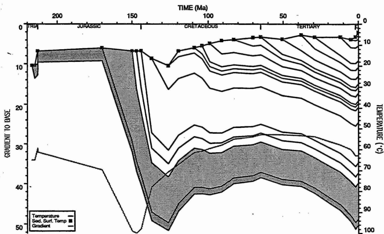
BED TEMPERATURE PLOT : Resolution 1
