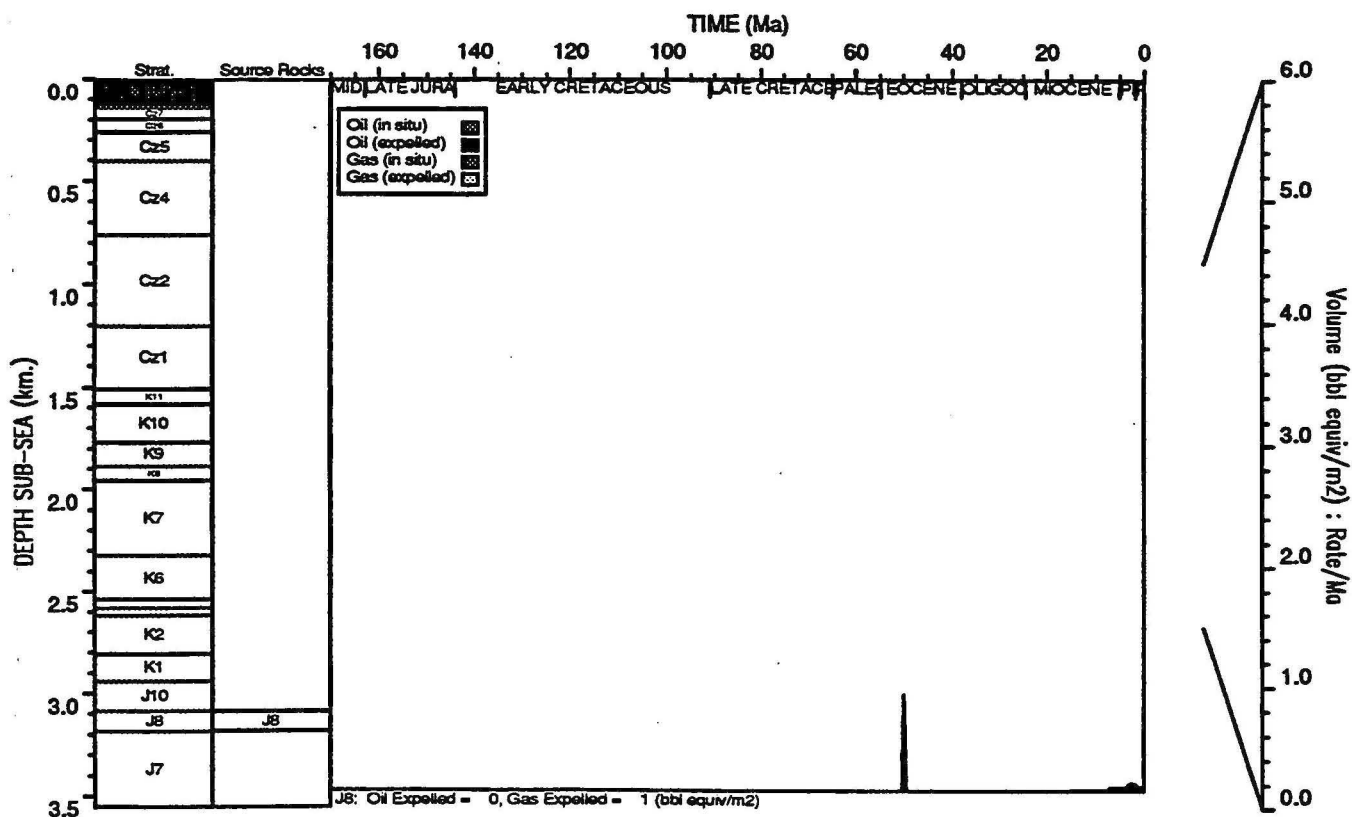
HYDROCARBON GENERATION PLOT : Buccaneer 1
