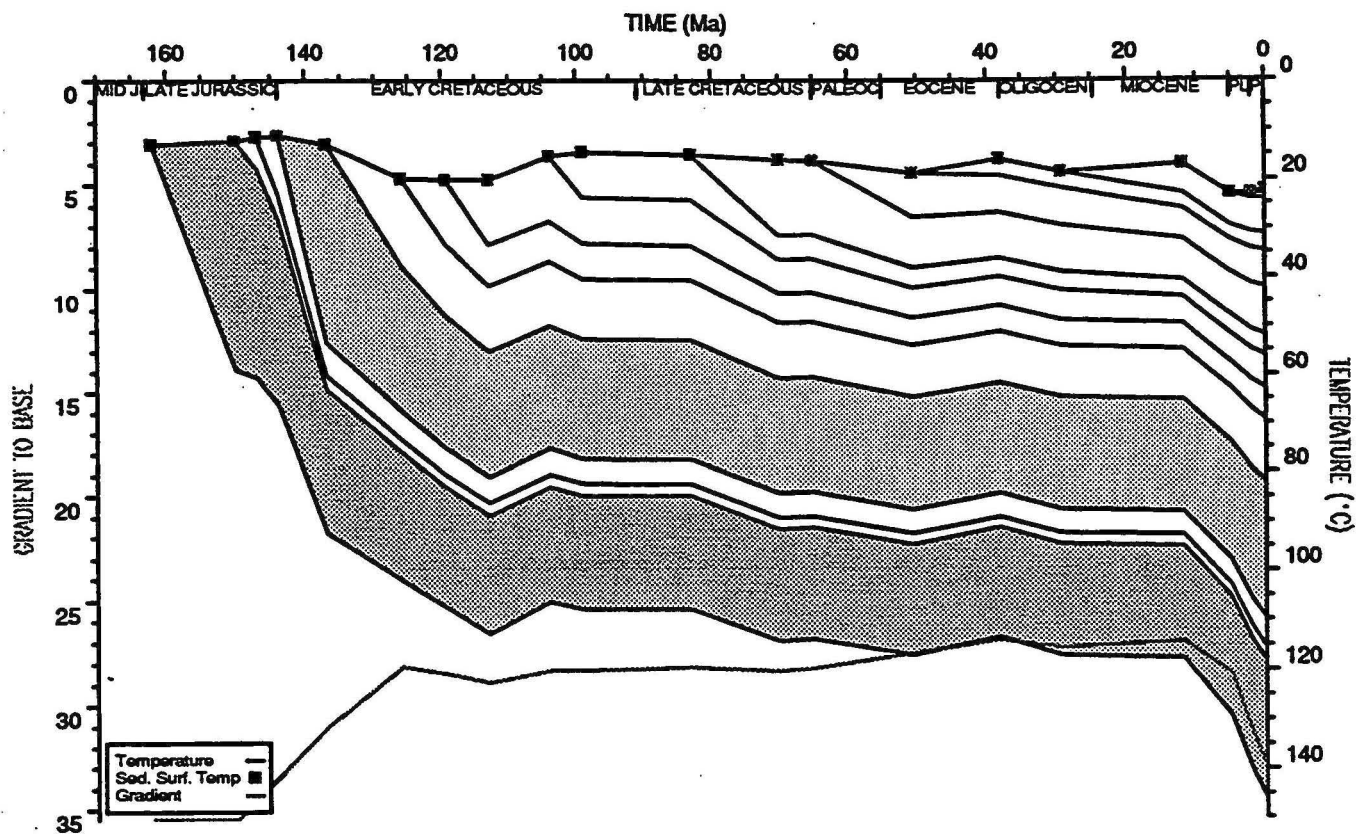
BED TEMPERATURE PLOT : South Pepper 1
