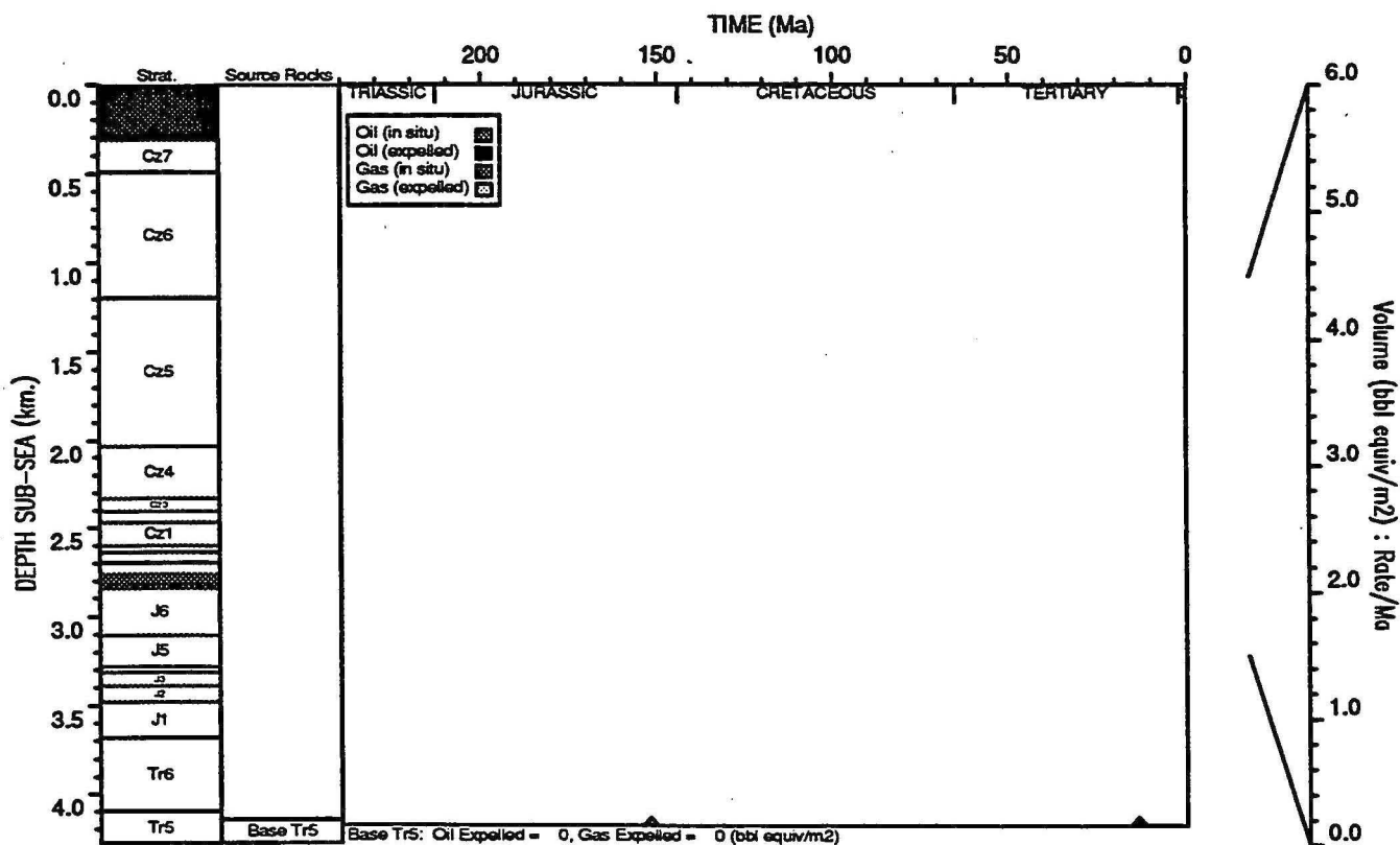
HYDROCARBON GENERATION PLOT : Brigadier 1
