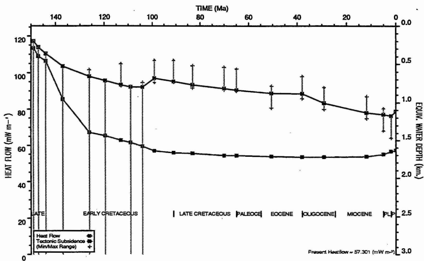
HEATFLOW AND TECTONIC SUBSIDENCE PLOT : Tryal Rocks 1
