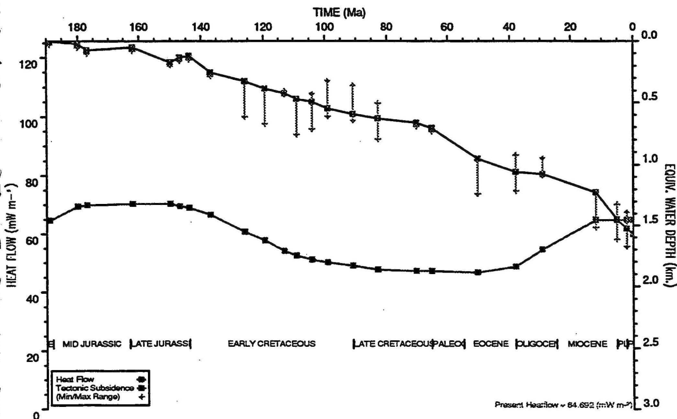
HEATFLOW AND TECTONIC SUBSIDENCE PLOT : Brewster 1A
