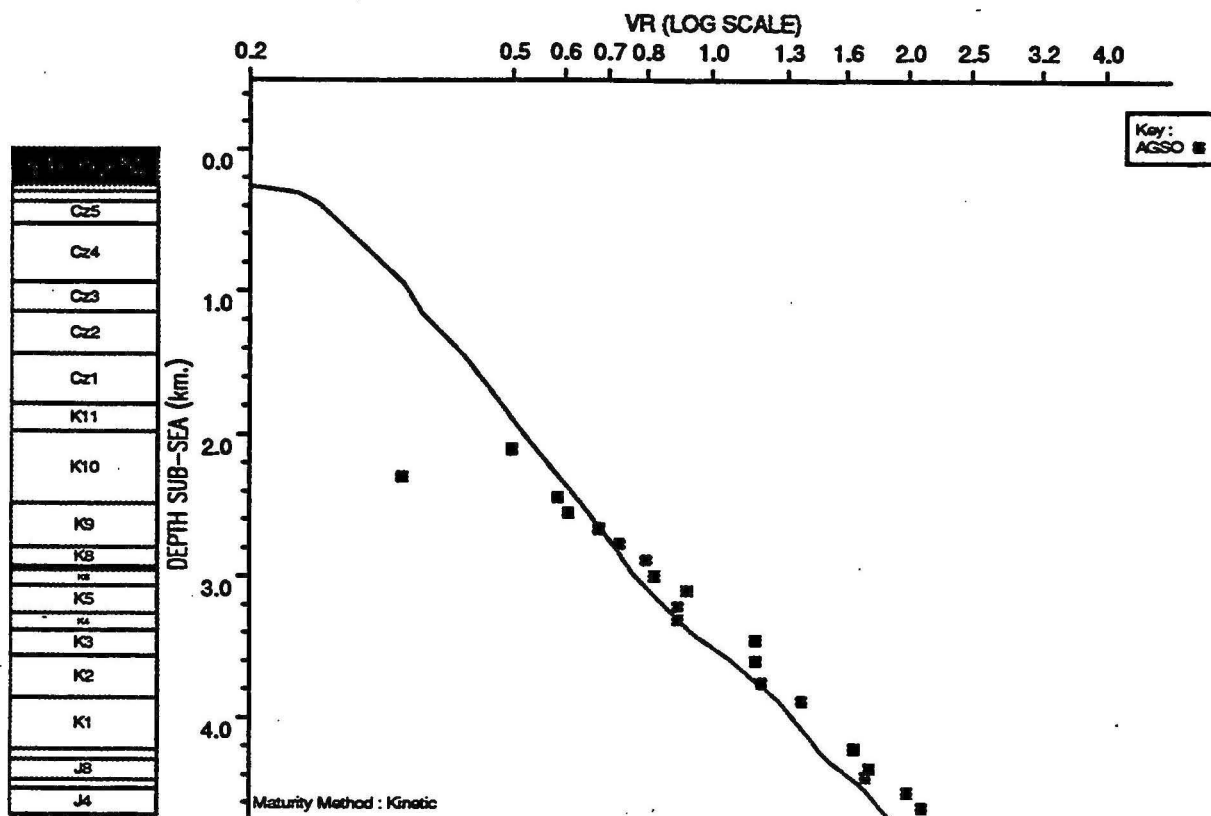
OBSERVED vs COMPUTED MATURITY PLOT : Brewster 1A
