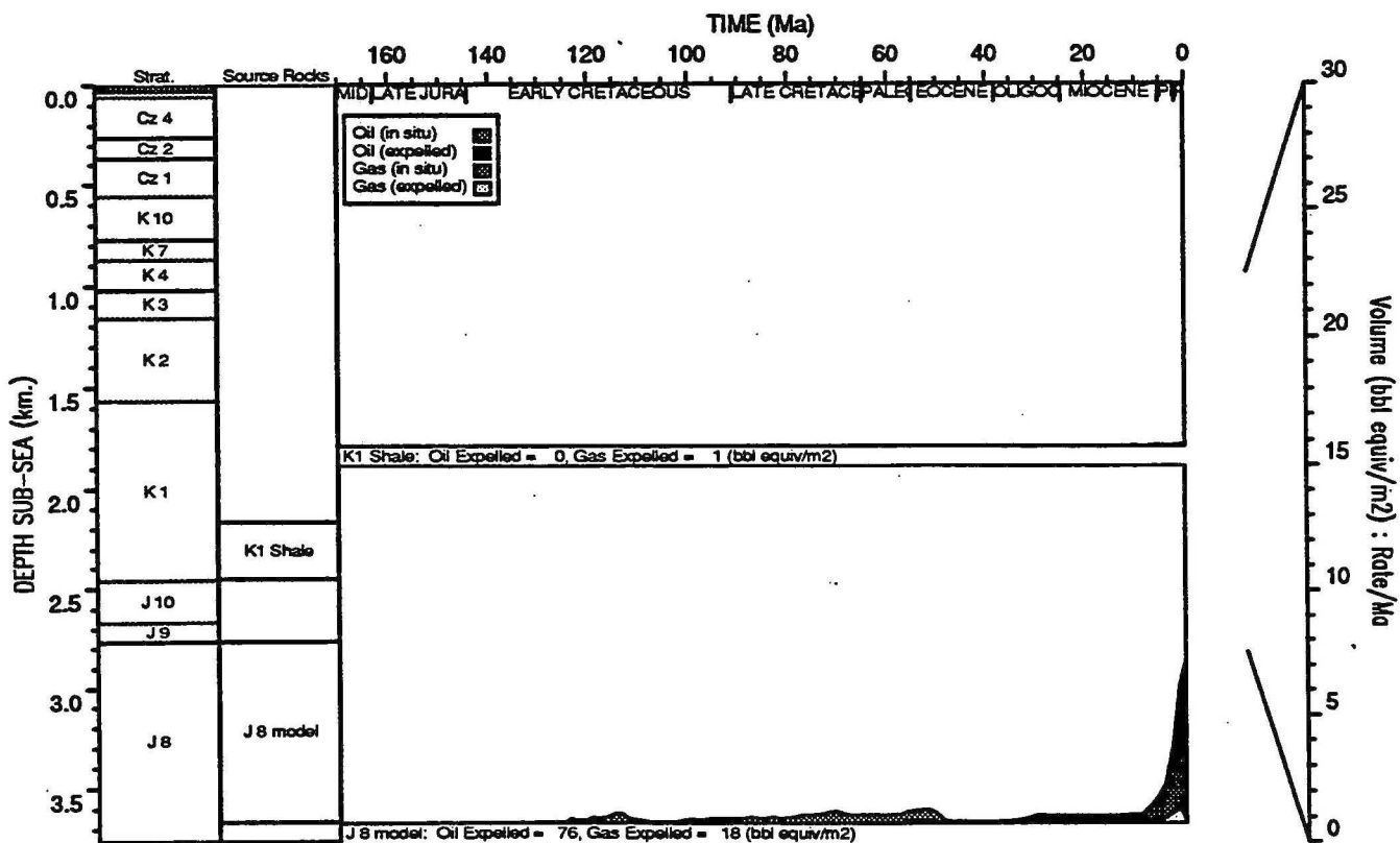
HYDROCARBON GENERATION PLOT : South Pepper 1
