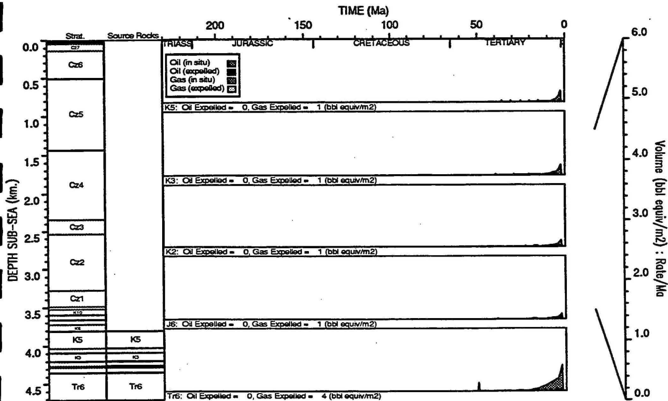
HYDROCARBON GENERATION PLOT : Scott Reef 1
