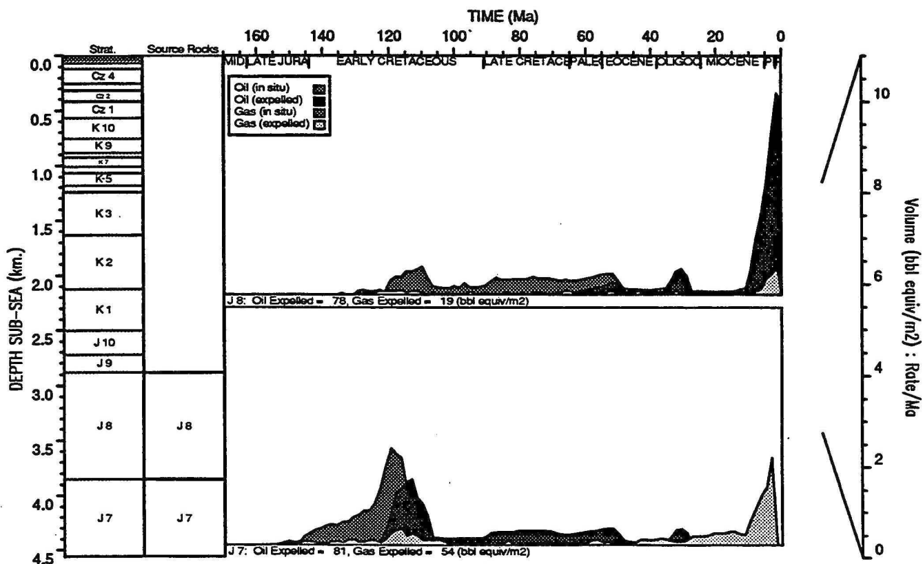
HYDROCARBON GENERATION PLOT : Bambra 2
