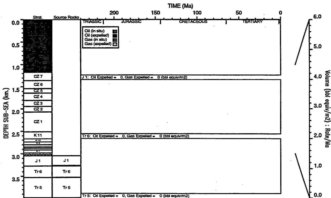
HYDROCARBON GENERATION PLOT : Saturn 1
