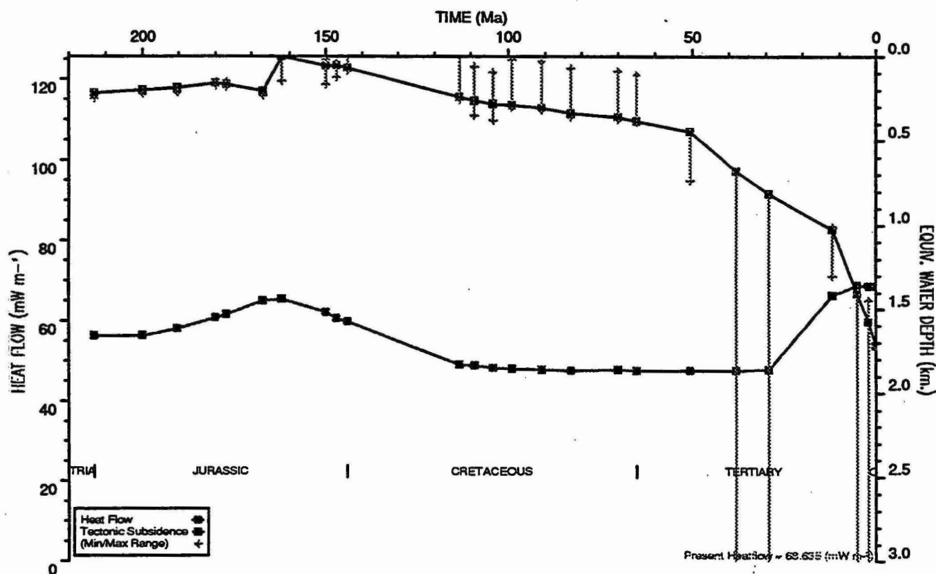
HEATFLOW AND TECTONIC SUBSIDENCE PLOT : Buffon 1
