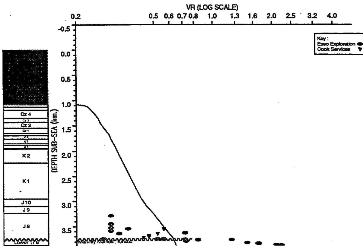
OBSERVED vs COMPUTED MATURITY PLOT : Resolution 1
