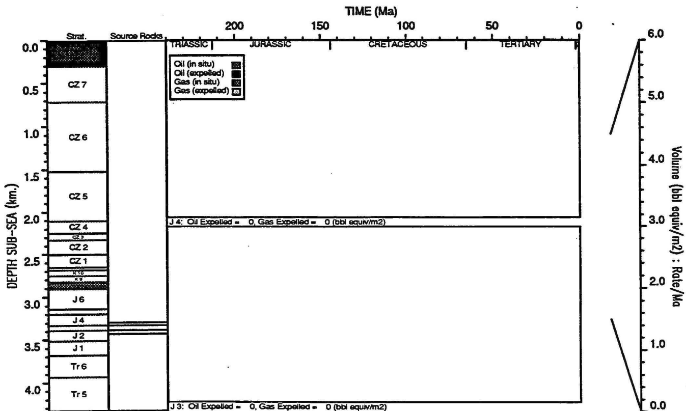
HYDROCARBON GENERATION PLOT : Gandara 1
