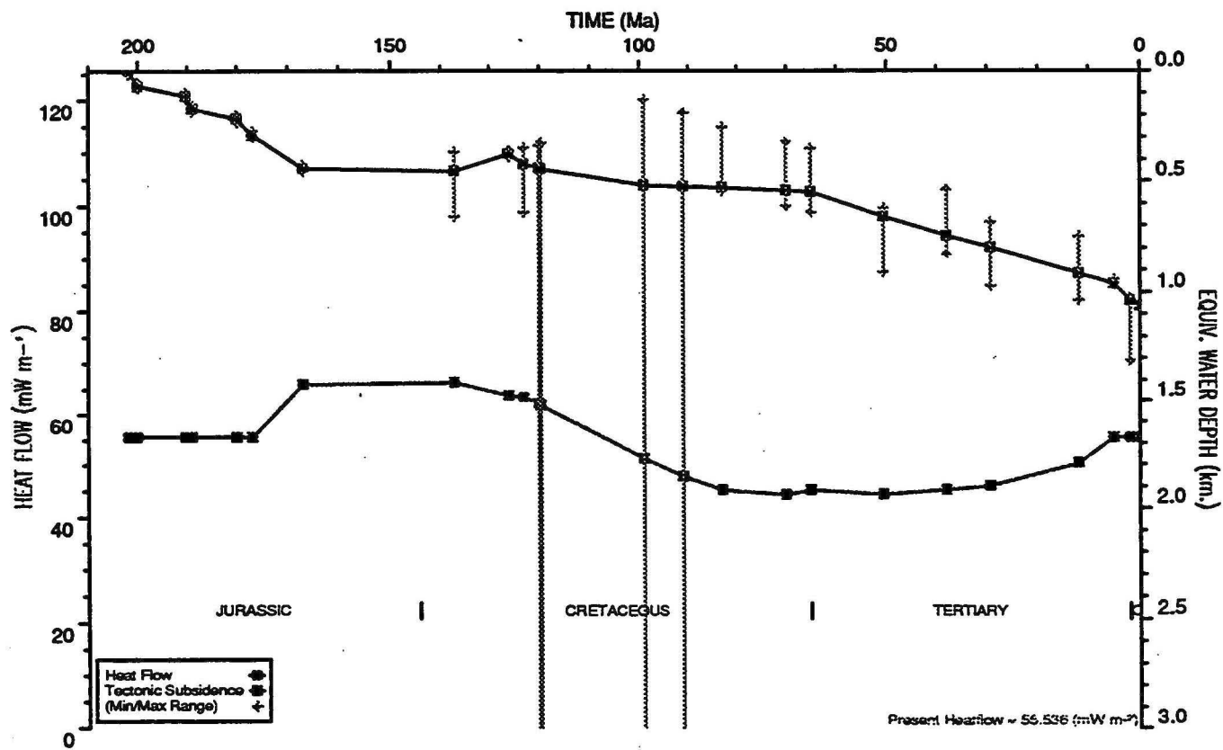
HEATFLOW AND TECTONIC SUBSIDENCE PLOT : Picard 1
