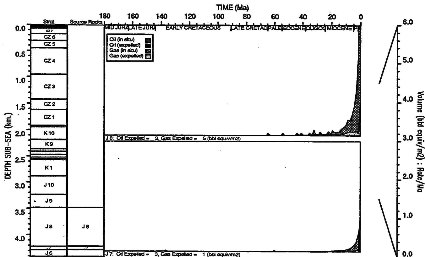
HYDROCARBON GENERATION PLOT : Madeleine 1
