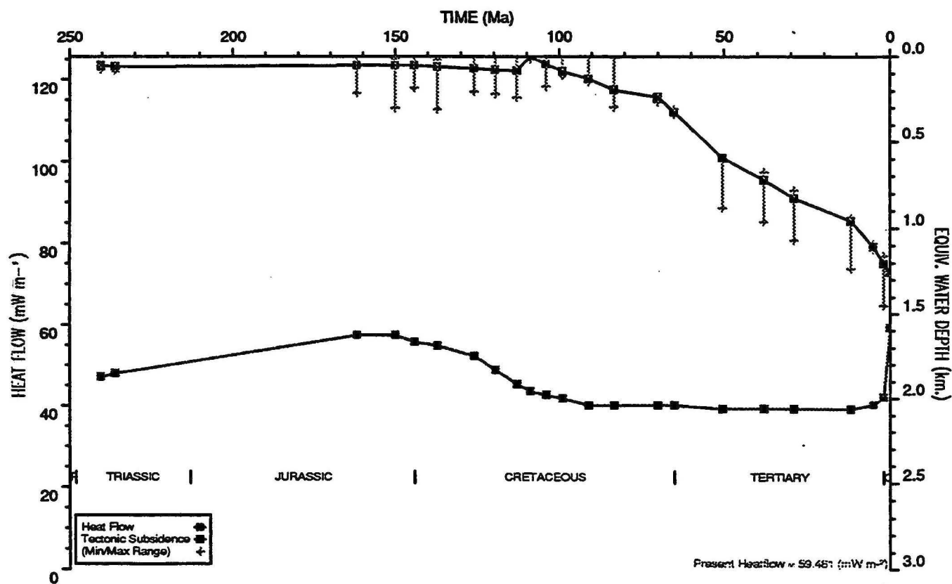
HEATFLOW AND TECTONIC SUBSIDENCE PLOT : Discorbis 1
