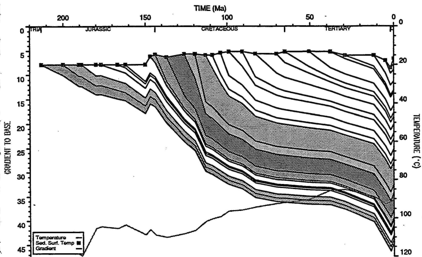
BED TEMPERATURE PLOT : Lombardina 1
