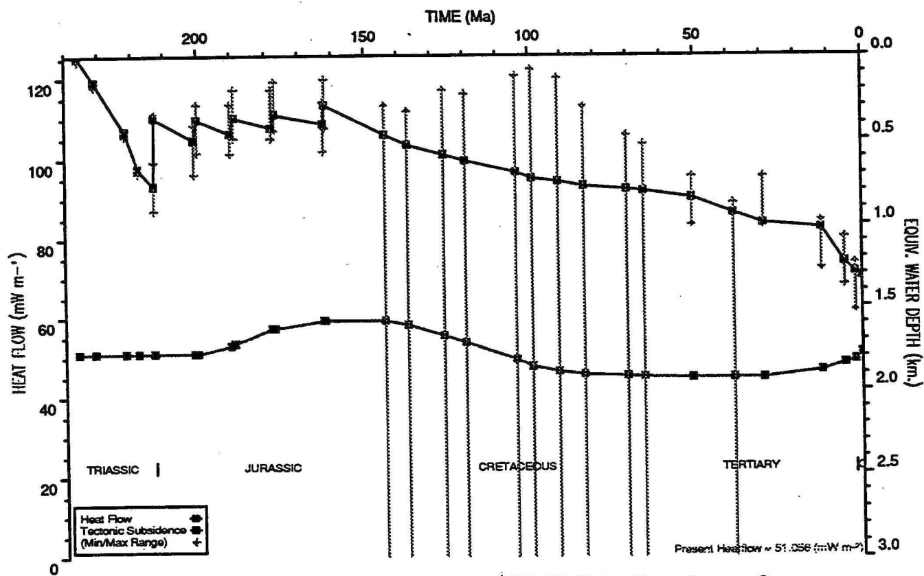
HEATFLOW AND TECTONIC SUBSIDENCE PLOT : Goodwyn 6
