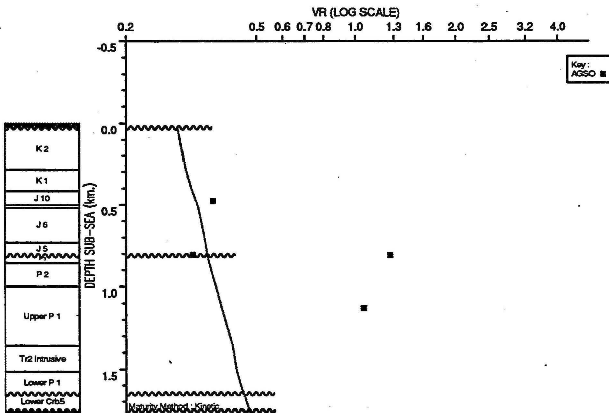
OBSERVED vs COMPUTED MATURITY PLOT : Perindi 1
