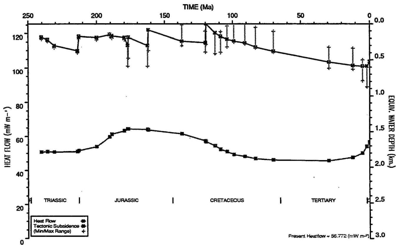
HEATFLOW AND TECTONIC SUBSIDENCE PLOT : Strickland 1
