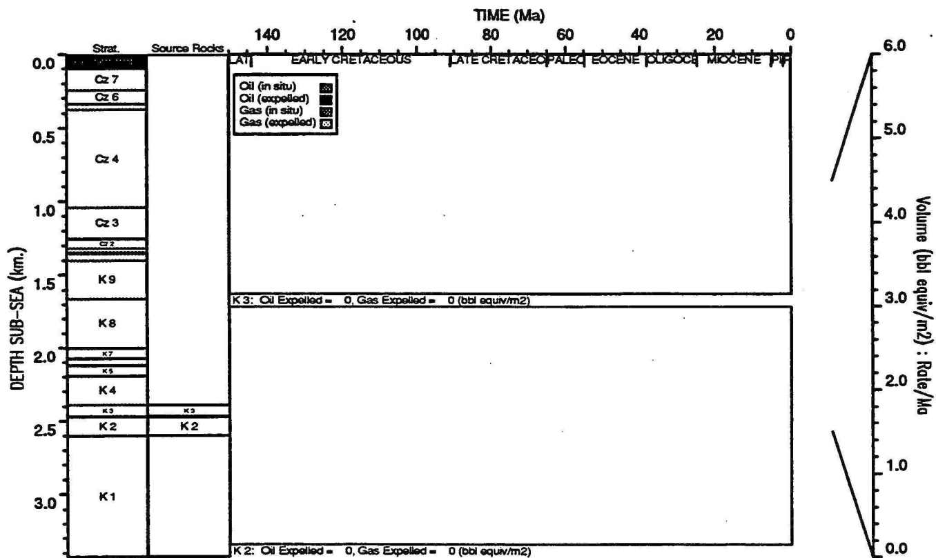
HYDROCARBON GENERATION PLOT : West Barrow 2
