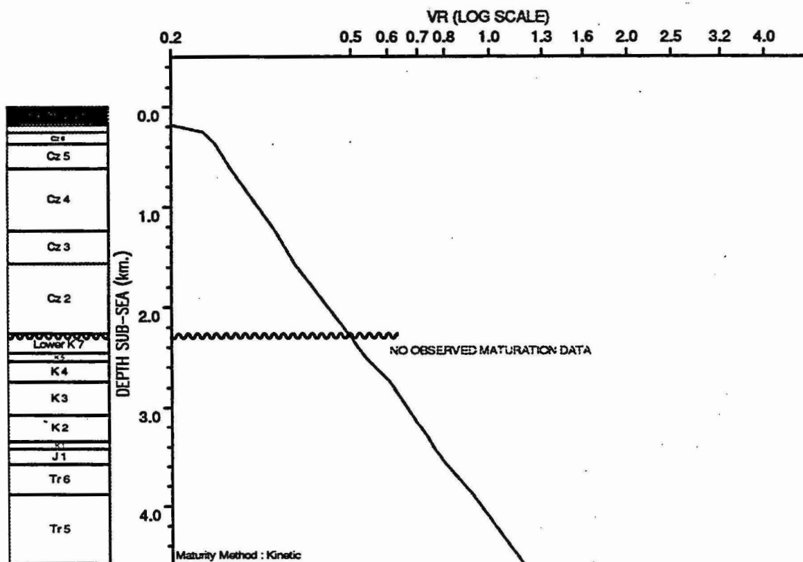
OBSERVED vs COMPUTED MATURITY PLOT : Bluebell 1
