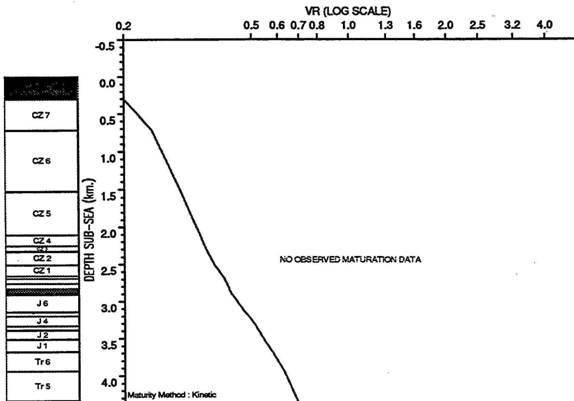
OBSERVED vs COMPUTED MATURITY PLOT : Gandara 1
