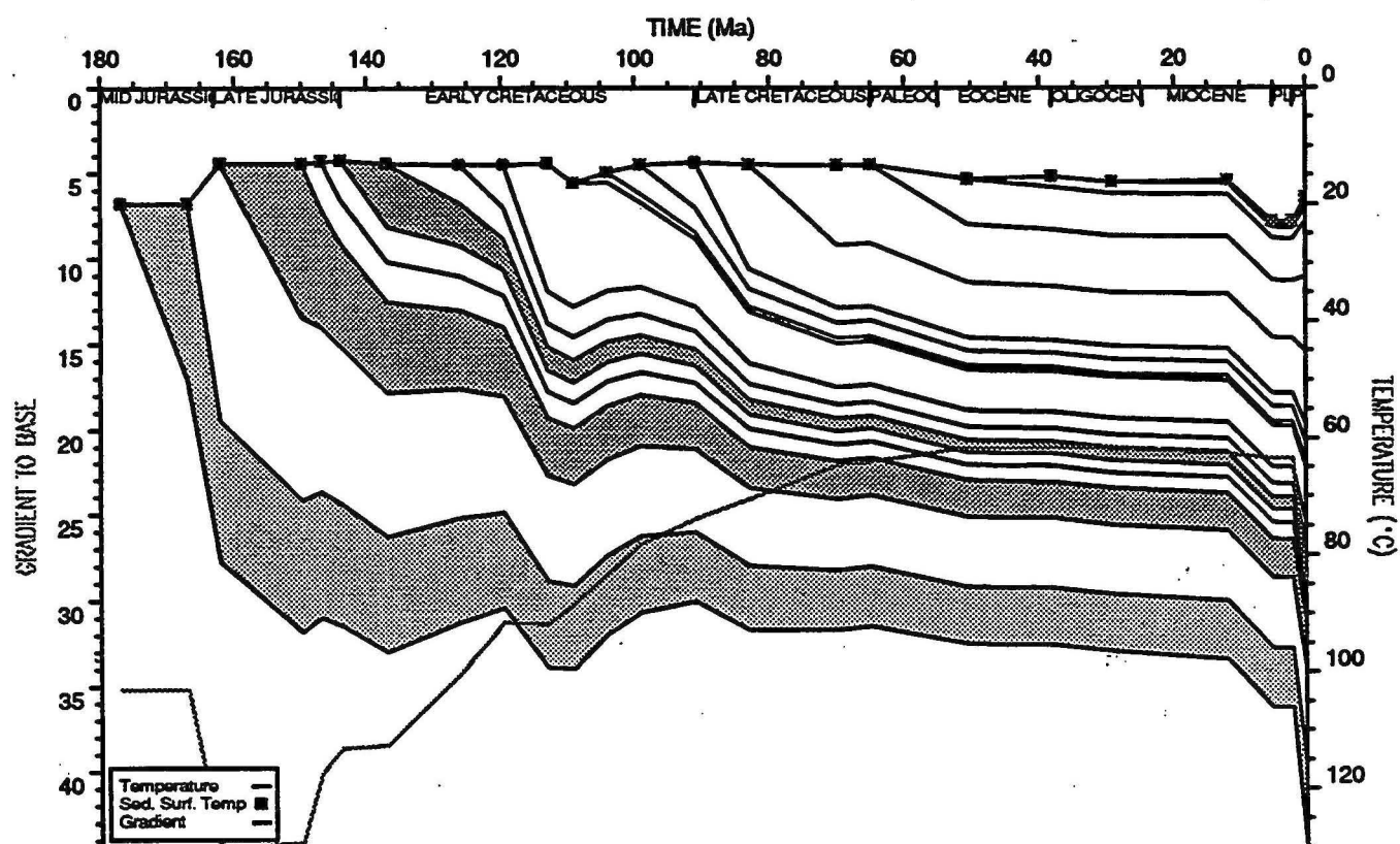
BED TEMPERATURE PLOT : Rosemary 1
