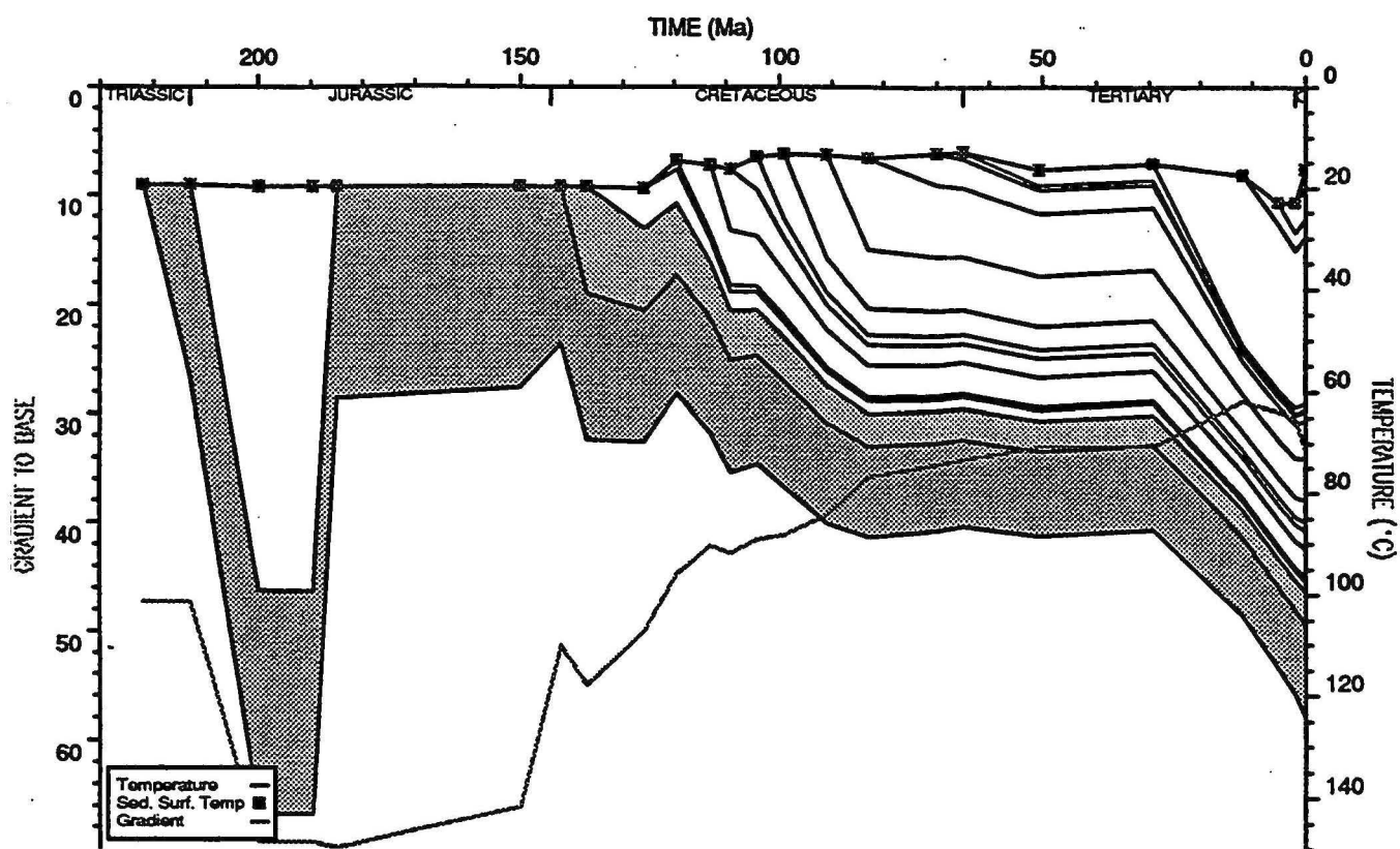
BED TEMPERATURE PLOT : Griffin 1
