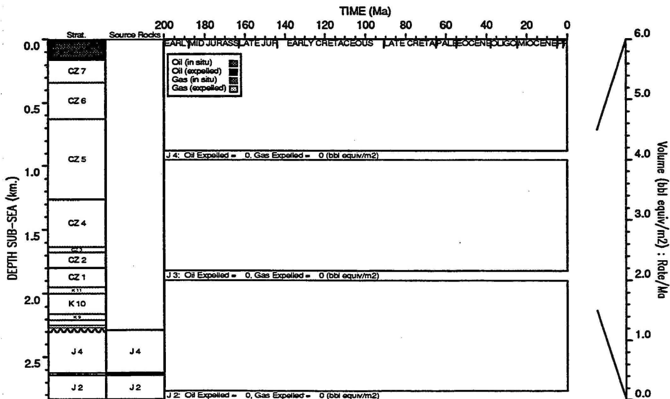
HYDROCARBON GENERATION PLOT : Ronsard 1
