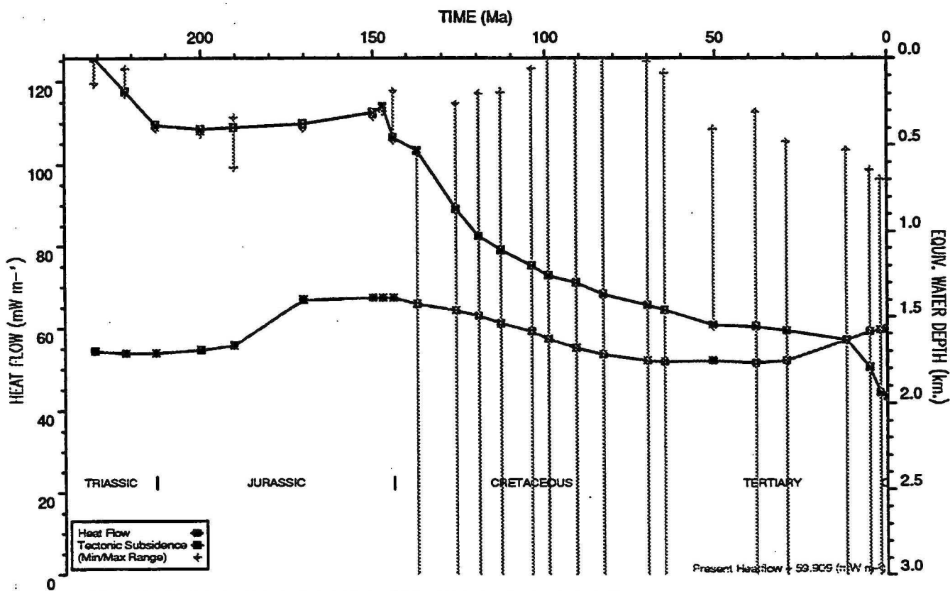
HEATFLOW AND TECTONIC SUBSIDENCE PLOT : Saturn 1
