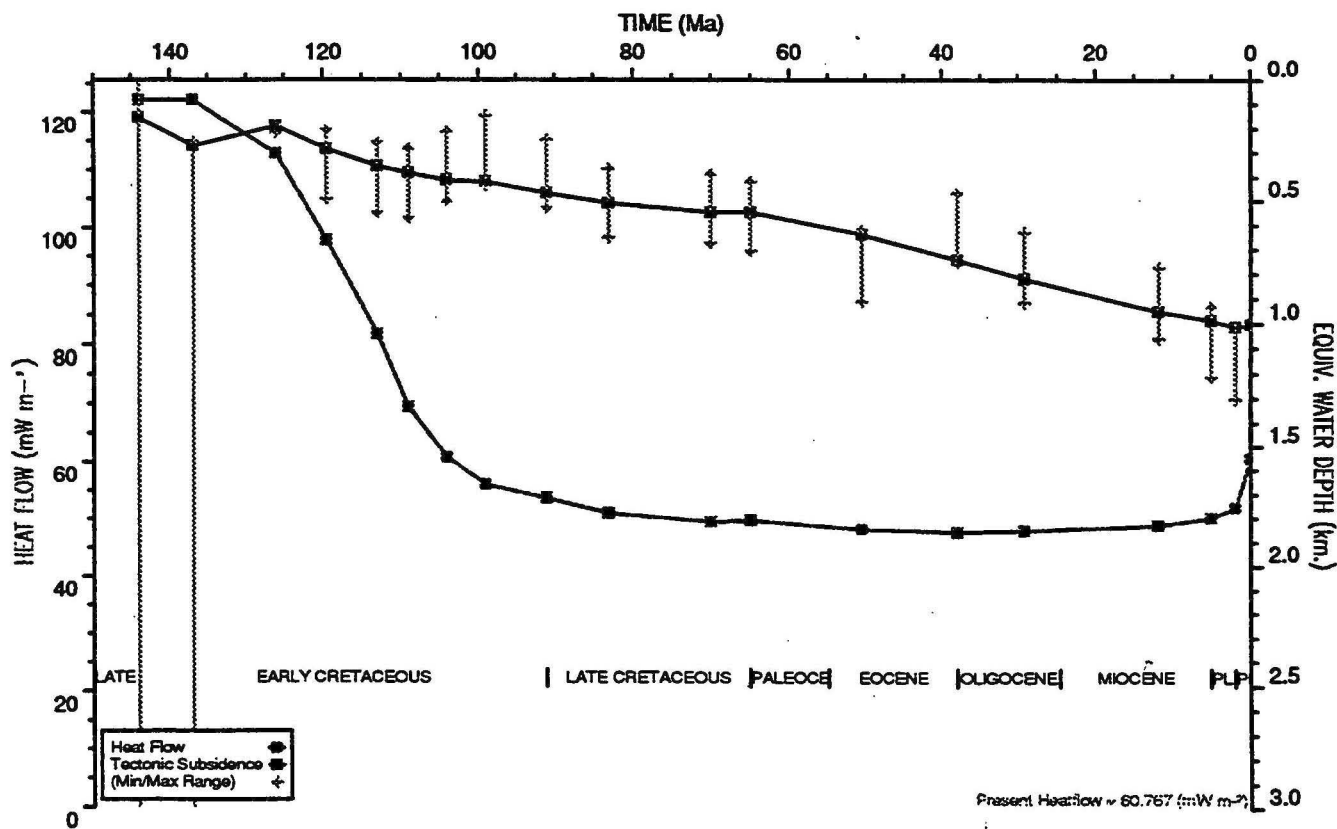
HEATFLOW AND TECTONIC SUBSIDENCE PLOT : West Barrow 2
