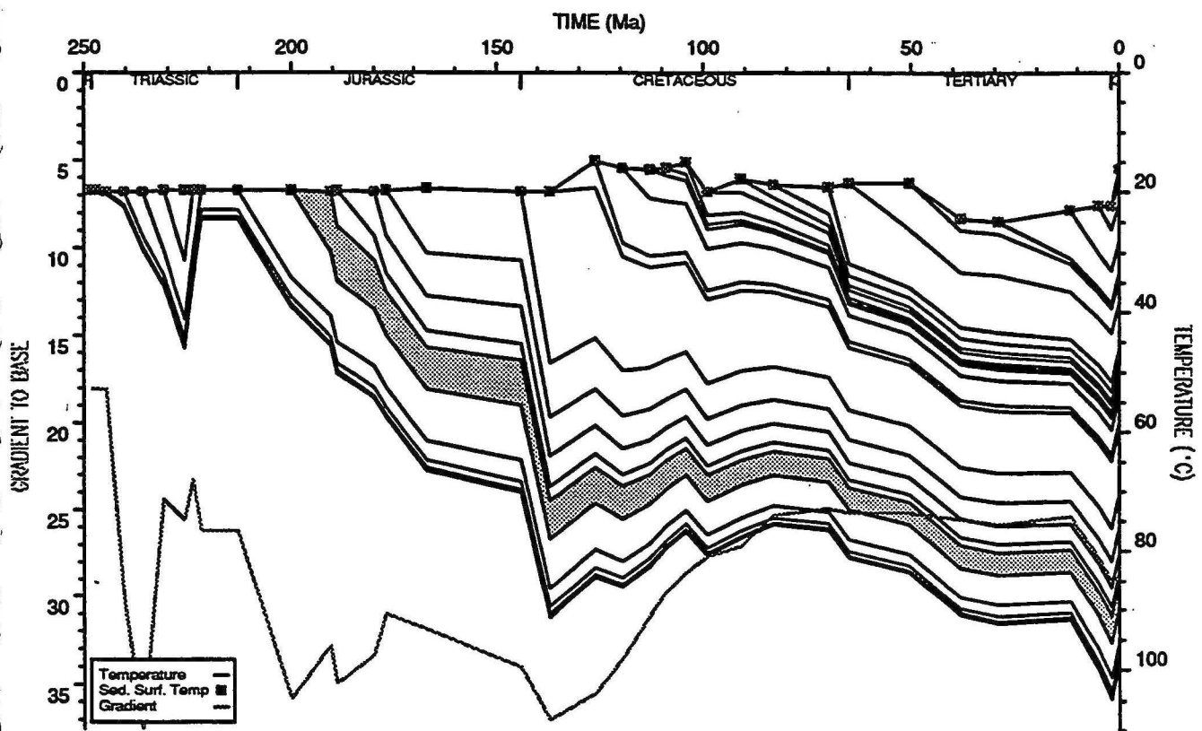
BED TEMPERATURE PLOT : Bedout 1
