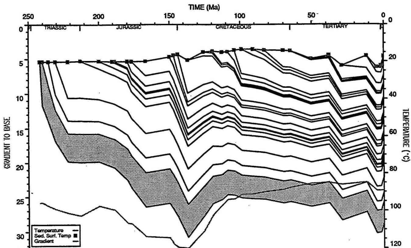
BED TEMPERATURE PLOT : Keraudren 1
