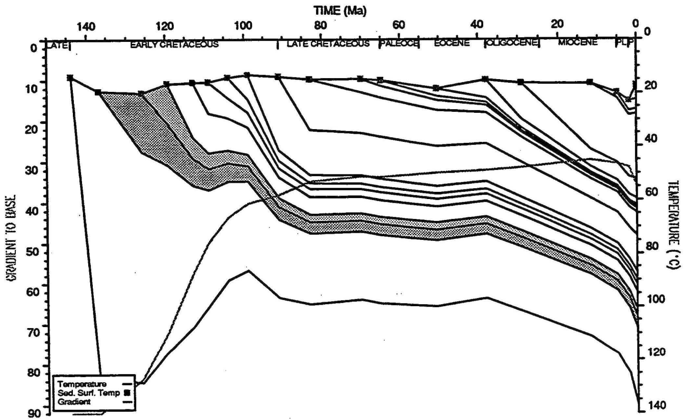
BED TEMPERATURE PLOT : West Barrow 2
