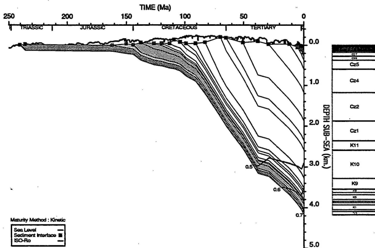
GEOHISTORY PLOT : Discorbis 1
