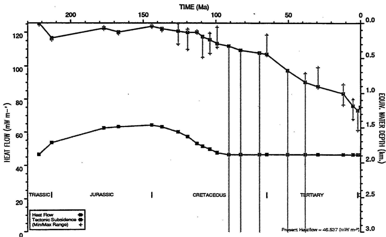
HEATFLOW AND TECTONIC SUBSIDENCE PLOT : Scott Reef 1
