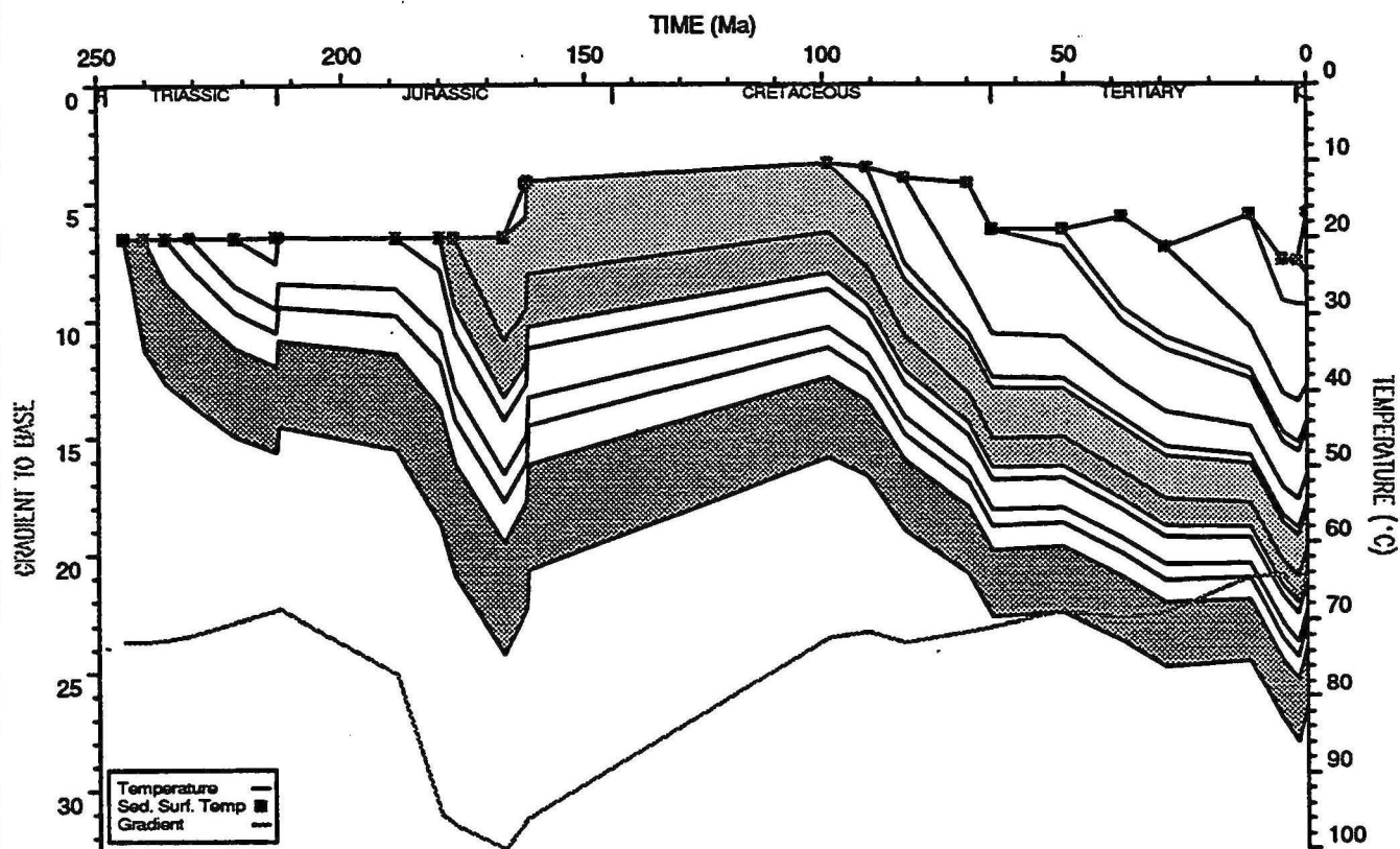
BED TEMPERATURE PLOT : Cossigny 1
