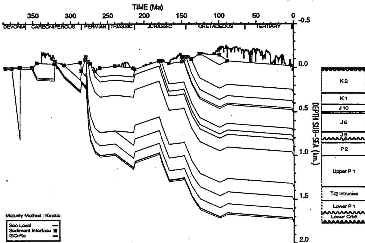
GEOHISTORY PLOT : Perindi 1
