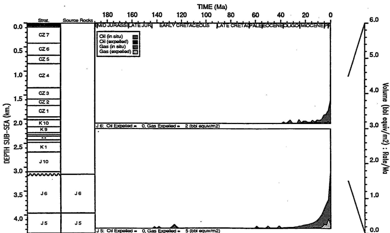
HYDROCARBON GENERATION PLOT : Angel 2
