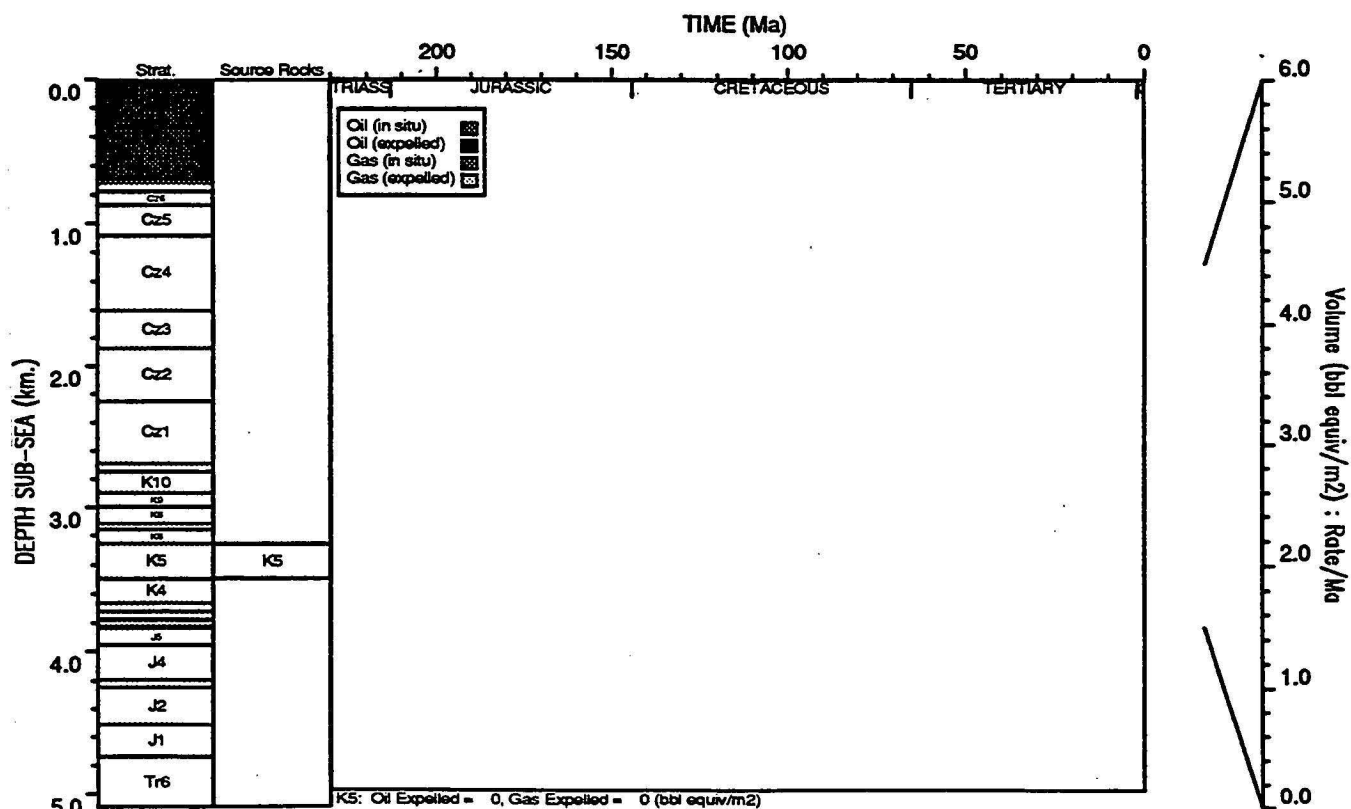
HYDROCARBON GENERATION PLOT : Barcoo 1
