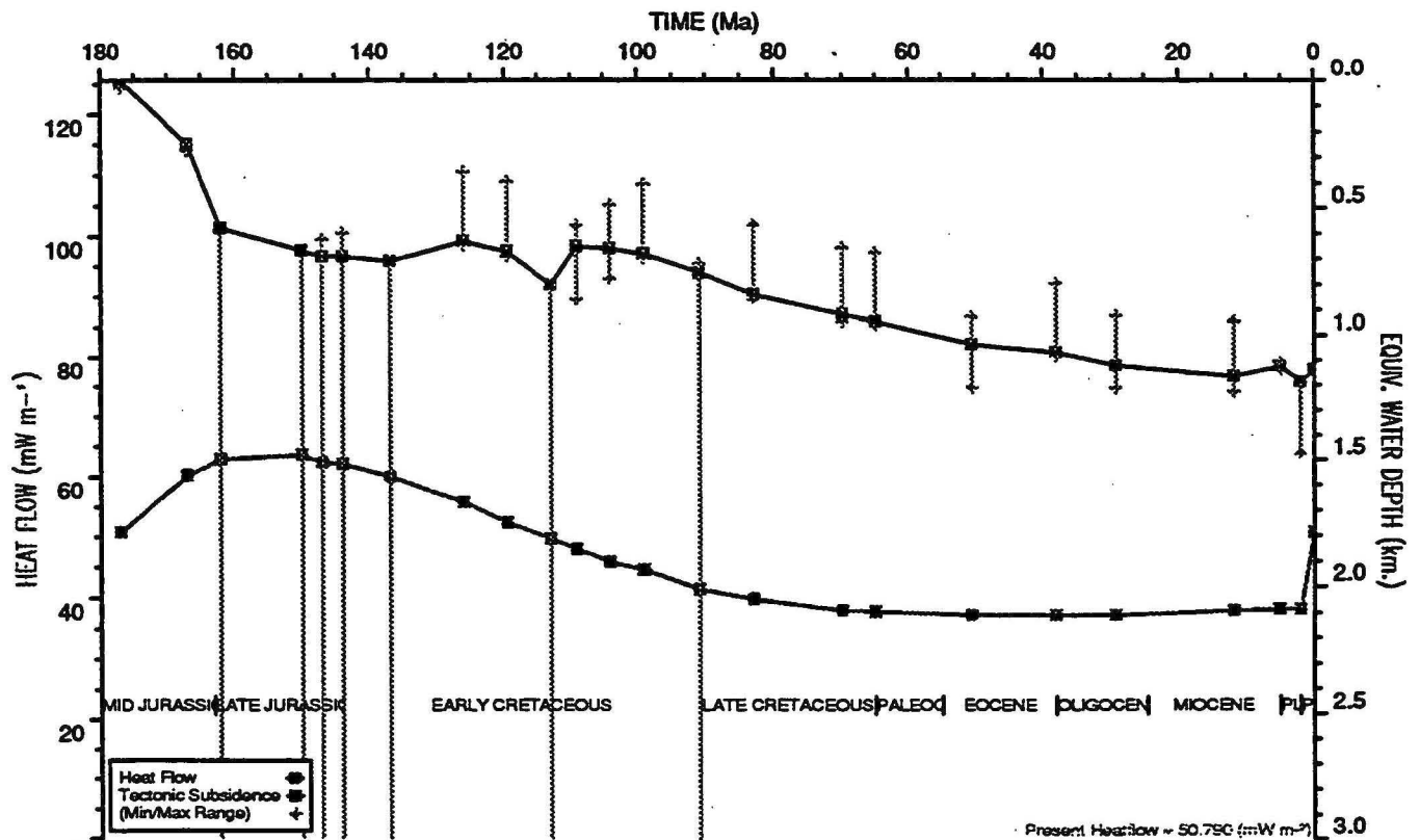
HEATFLOW AND TECTONIC SUBSIDENCE PLOT : Rosemary 1
