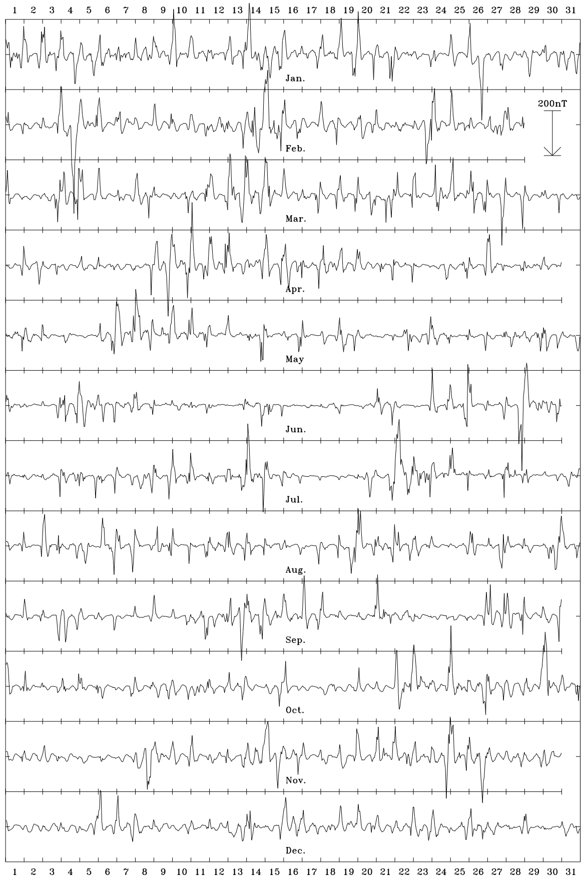
Mawson Stn. 2009 Vertical intensity (Z). Scale: 15.0 nT/mm. Mean: -45448 nT
