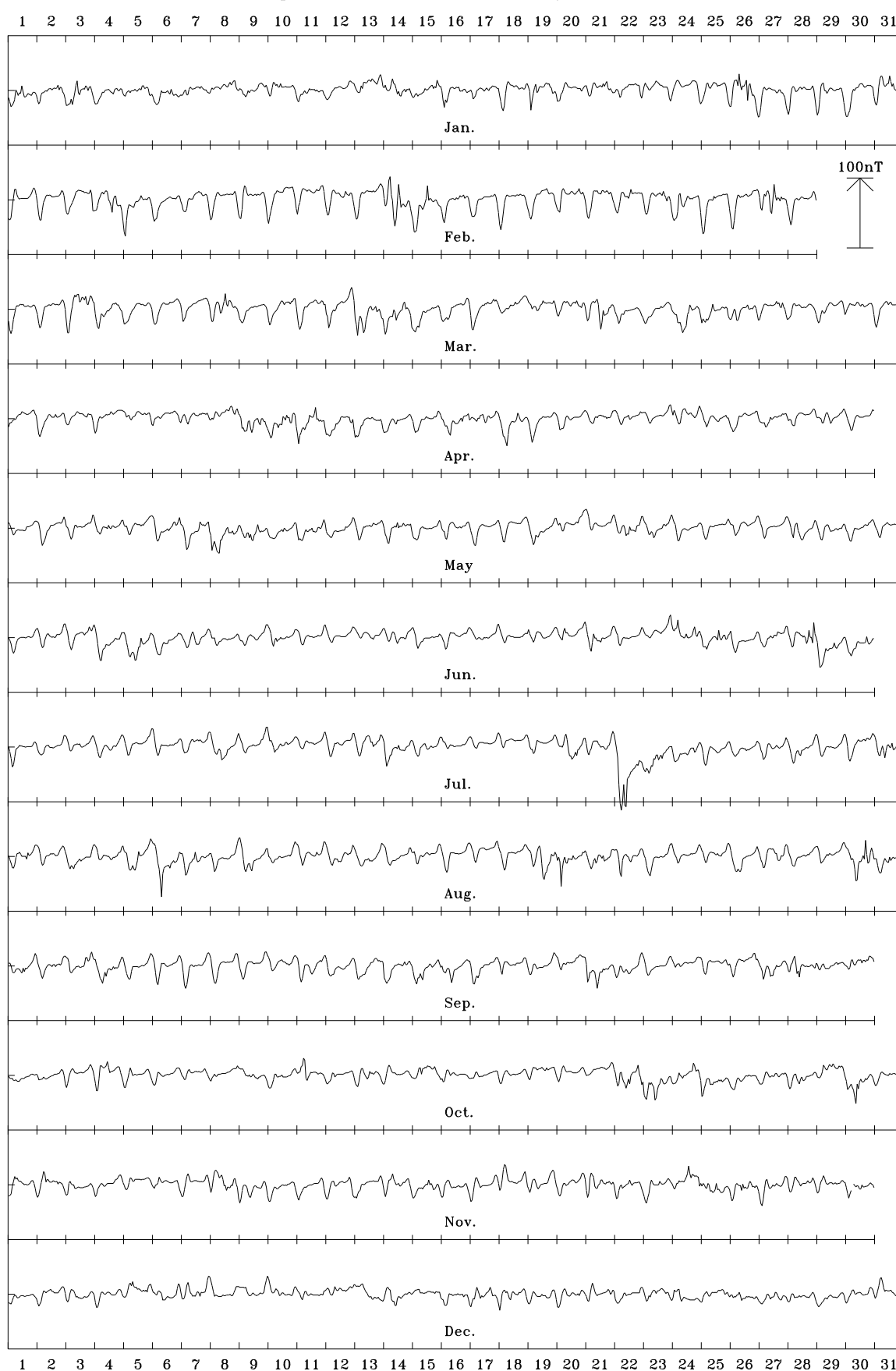
Canberra 2009 North component (X). Scale: 7.5 nT/mm. Mean: 23177 nT
