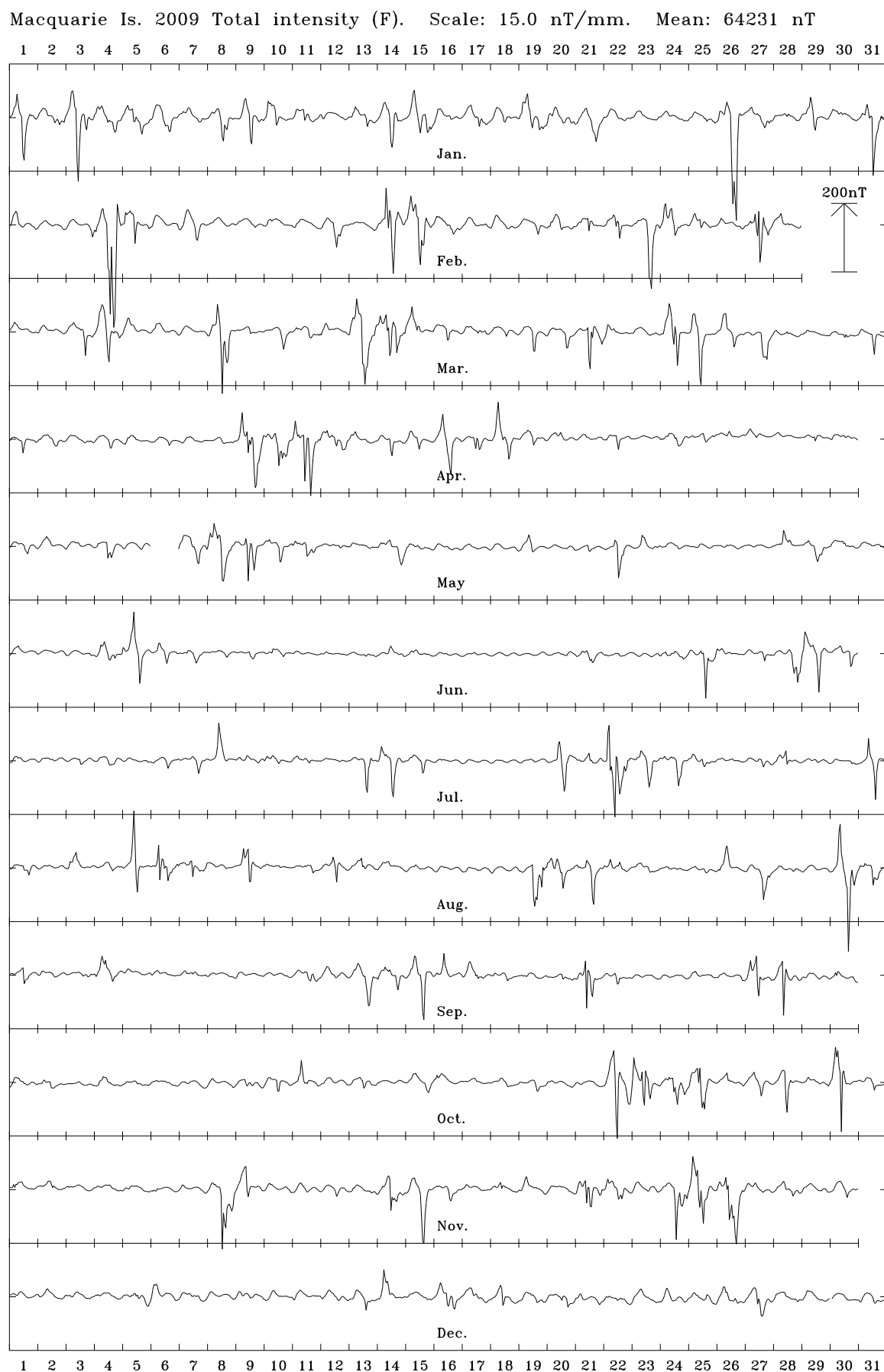
Figure 7.3. Macquarie Island 2009 hourly mean values in X, Y, Z and F.
