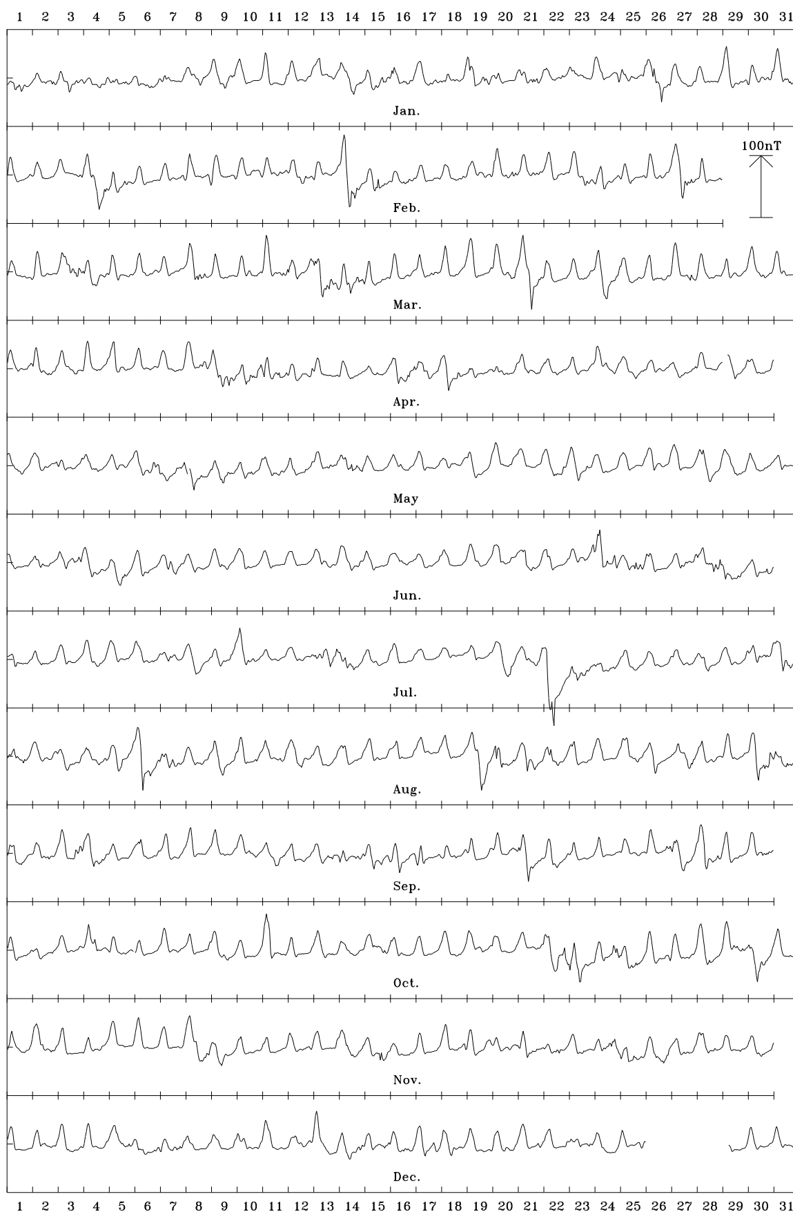
Kakadu, NT 2009 North component (X). Scale: 7.5 nT/mm. Mean: 35377 nT
