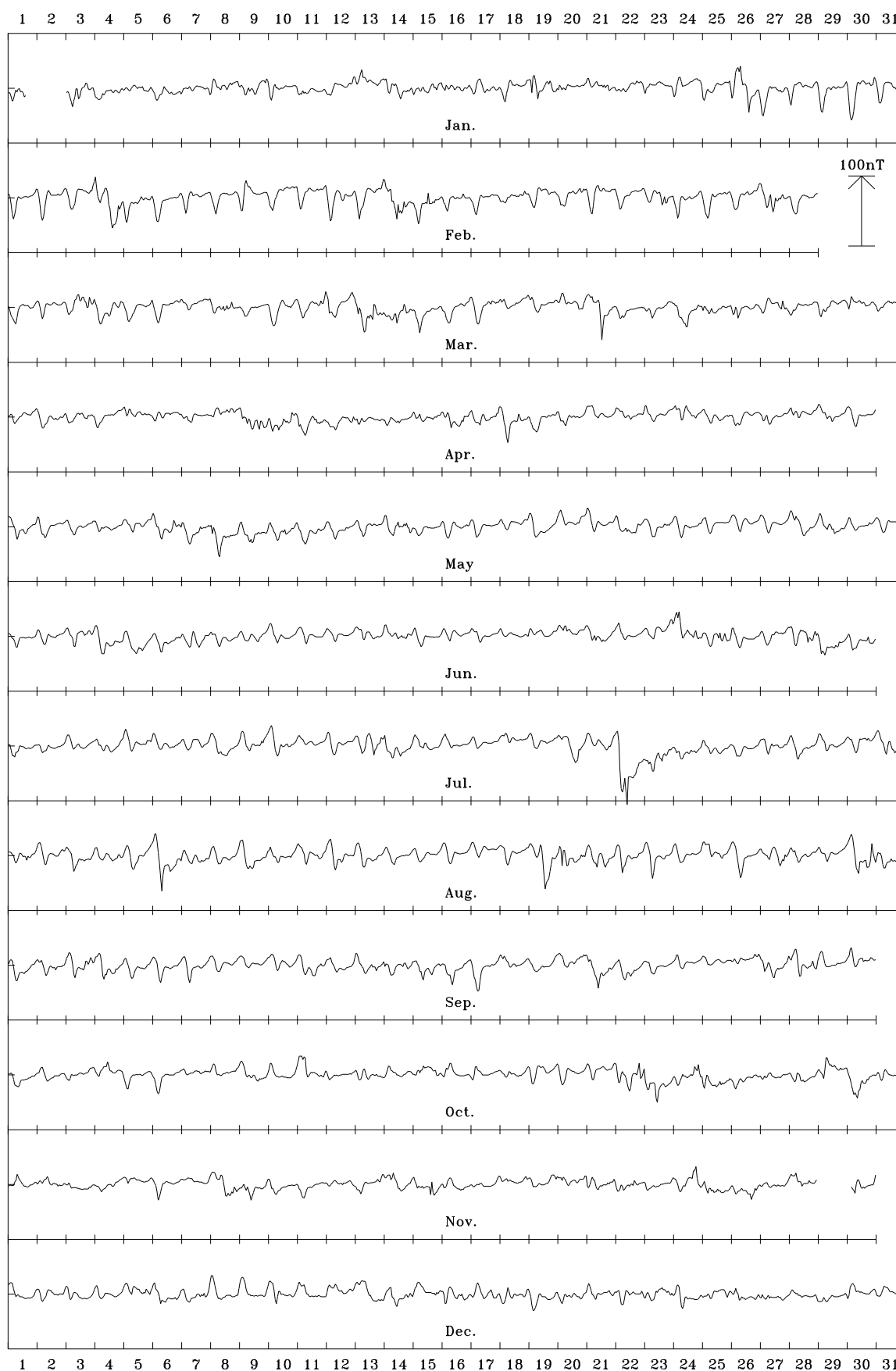
Gnangara 2009 North component (X). Scale: 7.5 nT/mm. Mean: 23398 nT
