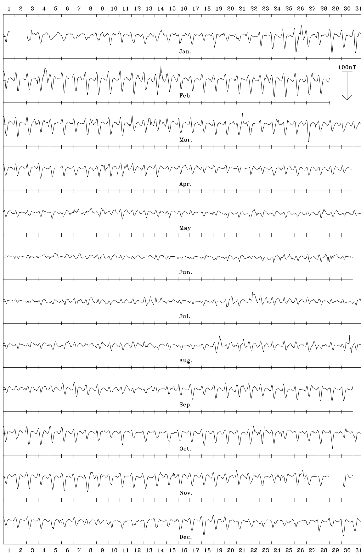
Gnangara 2009 Vertical intensity (Z). Scale: 7.5 nT/mm. Mean: -53307 nT
