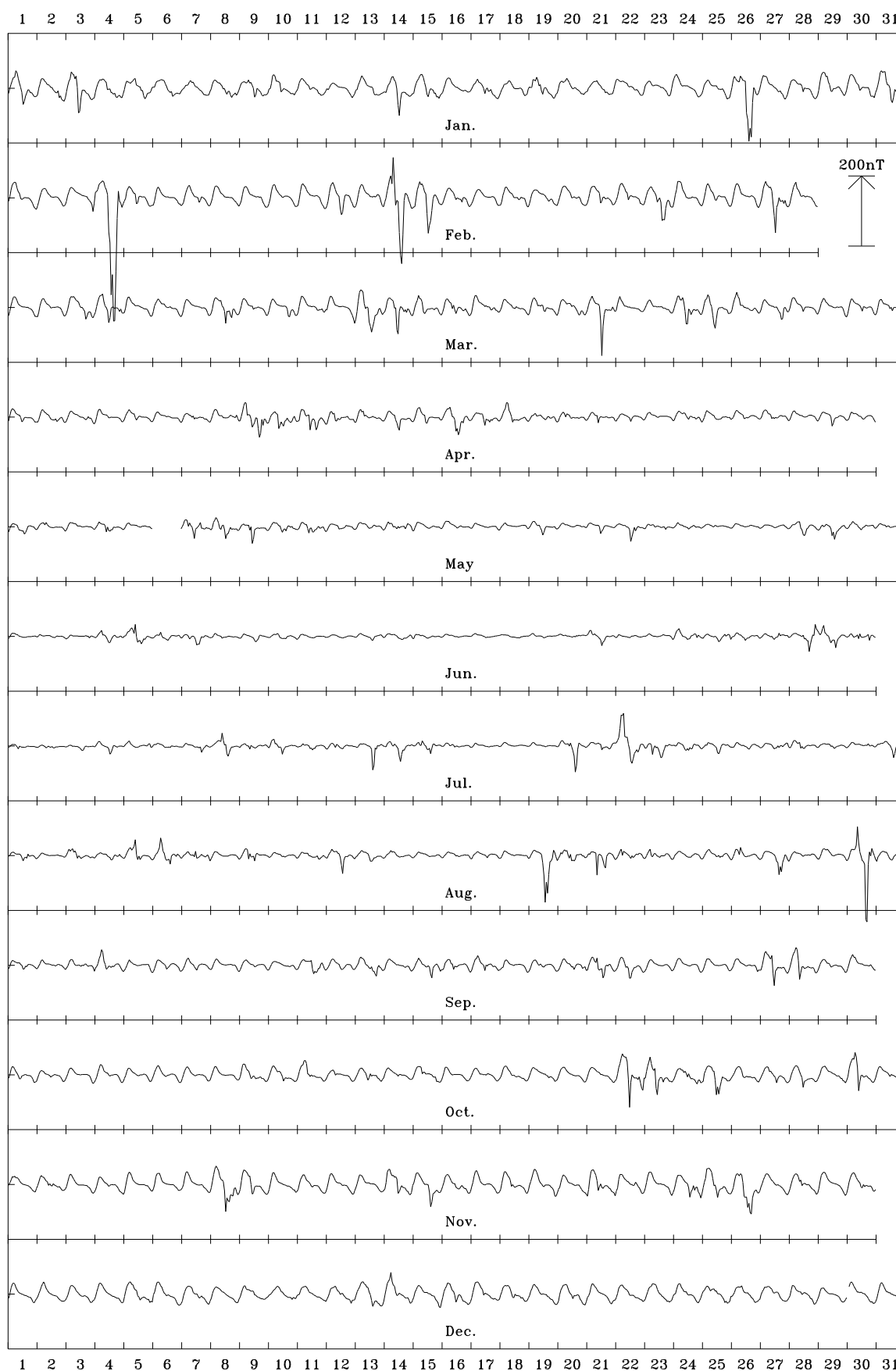
Macquarie Is. 2009 East component (Y). Scale: 15.0 nT/mm. Mean: 6556 nT
