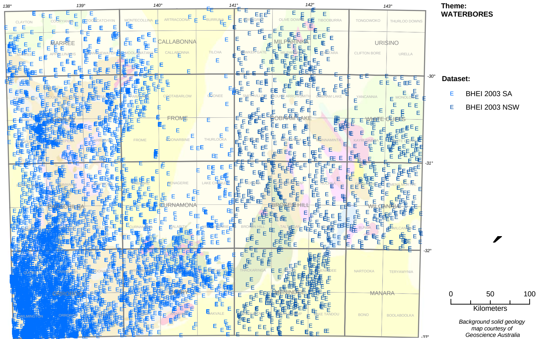
Map 8.2. All Water bore locations in the Curnamona Province
