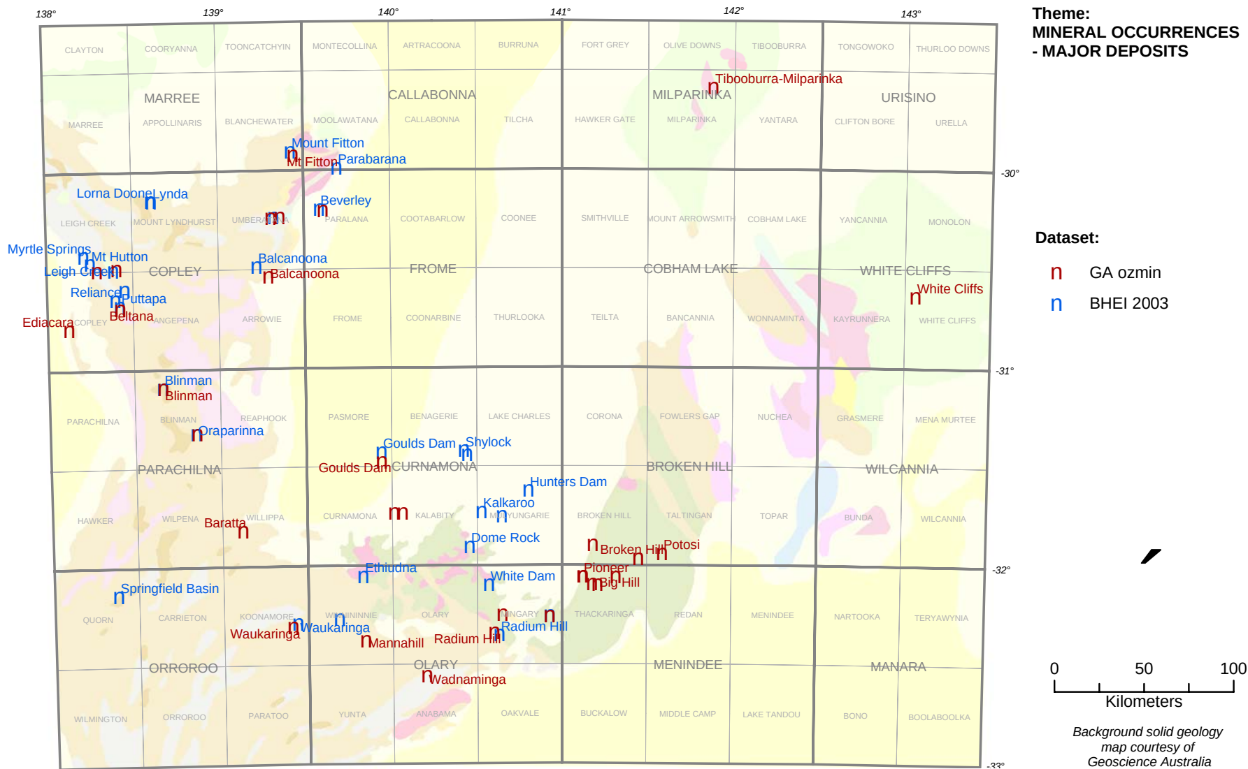
Map 7.3 Major Mineral Occurrences the Curnamona Province
