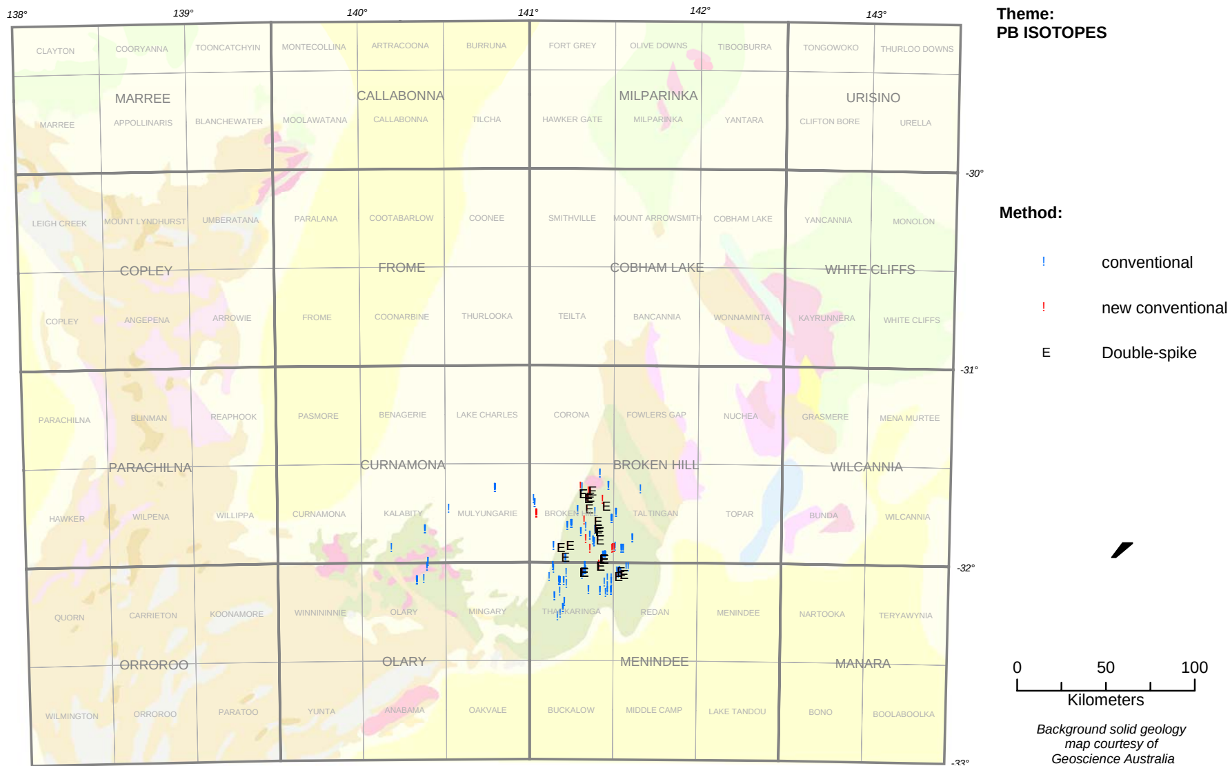
Map 8.4 Location of samples for lead isotope analysis in the Curnamona Province
