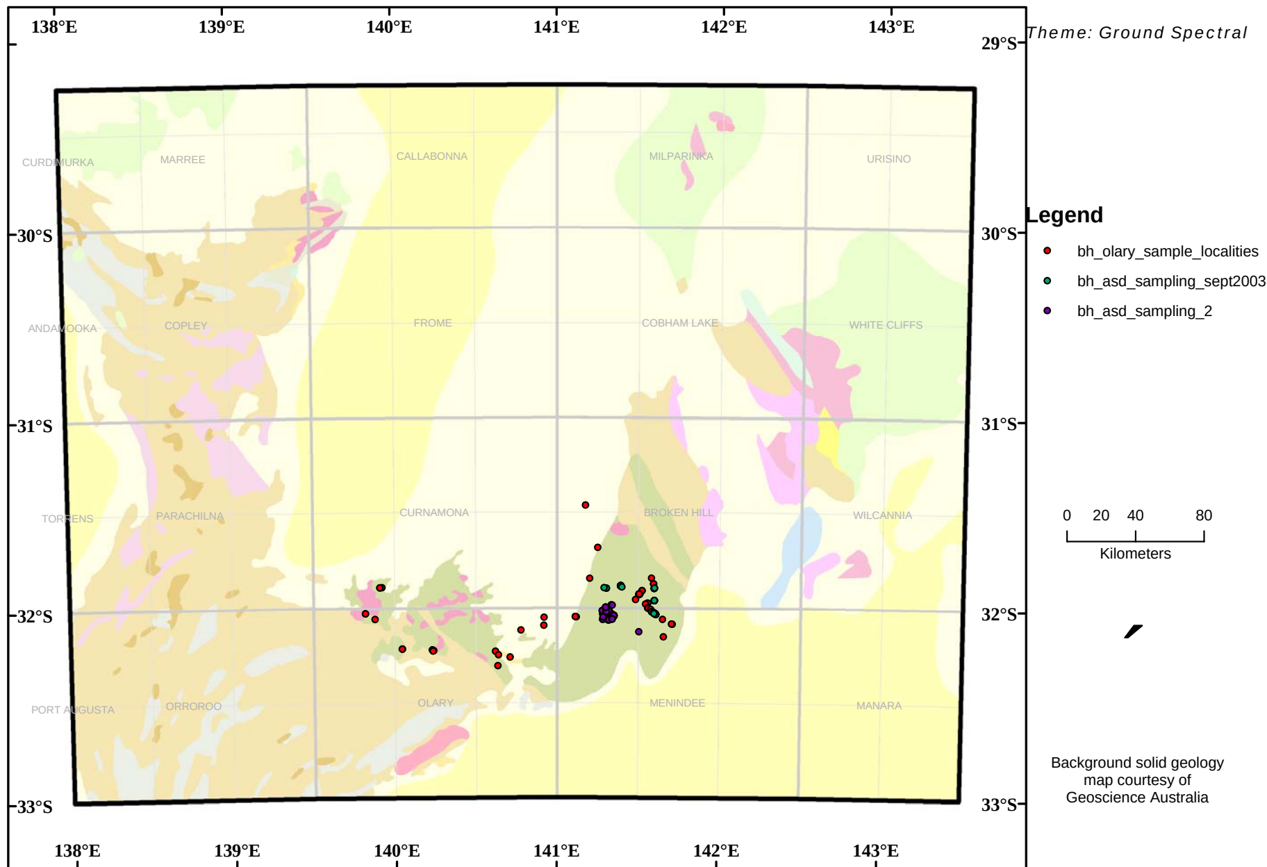
Map 11.7 Sample points for ground sampling for spectral analysis in the Curnamona Province
