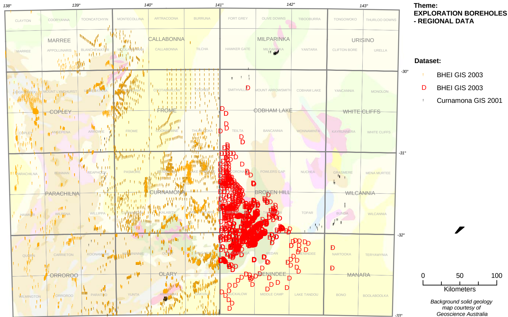
Map 8.1.1. Exploration borehole locations in the Curnamona Province
