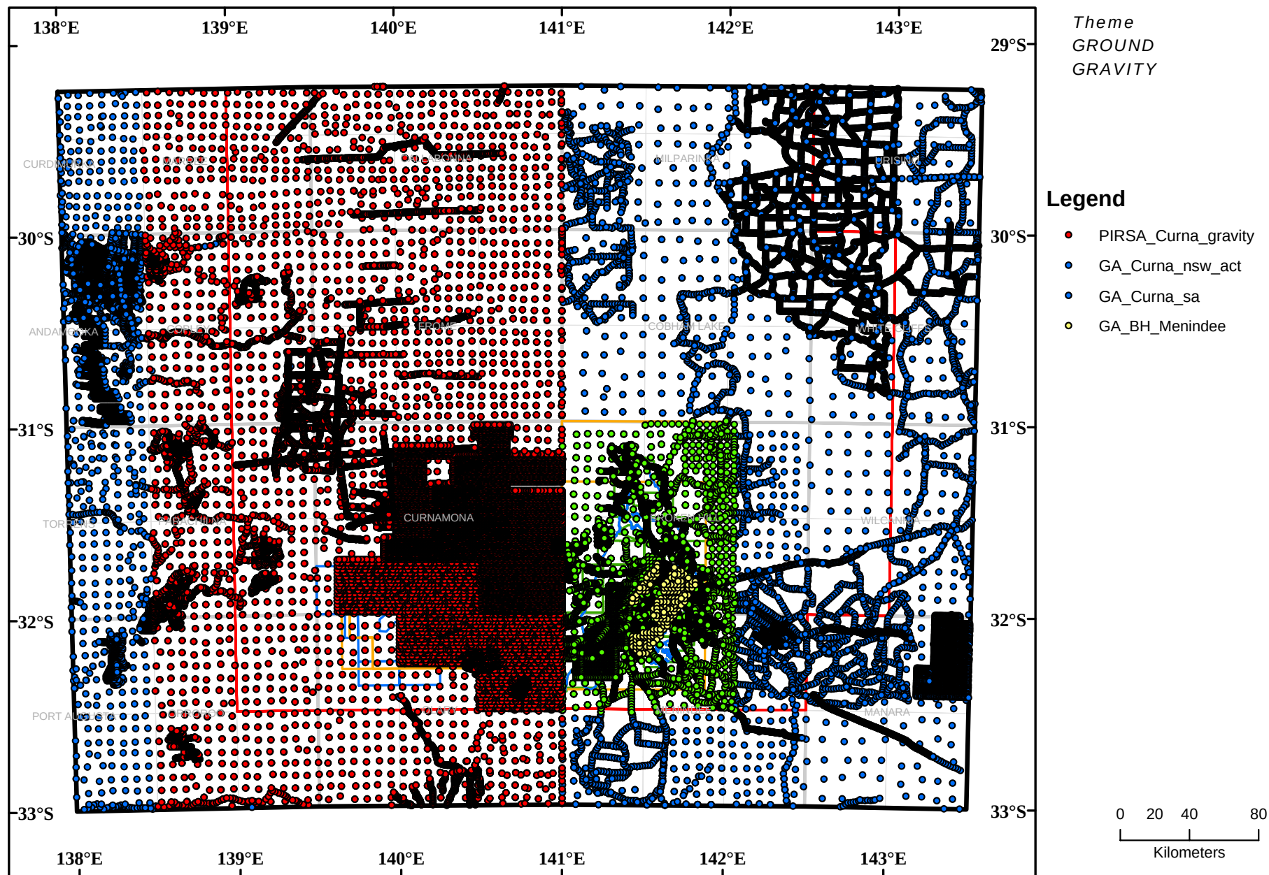
Map 9.4 Location of ground gravity stations in the Curnamona Province
