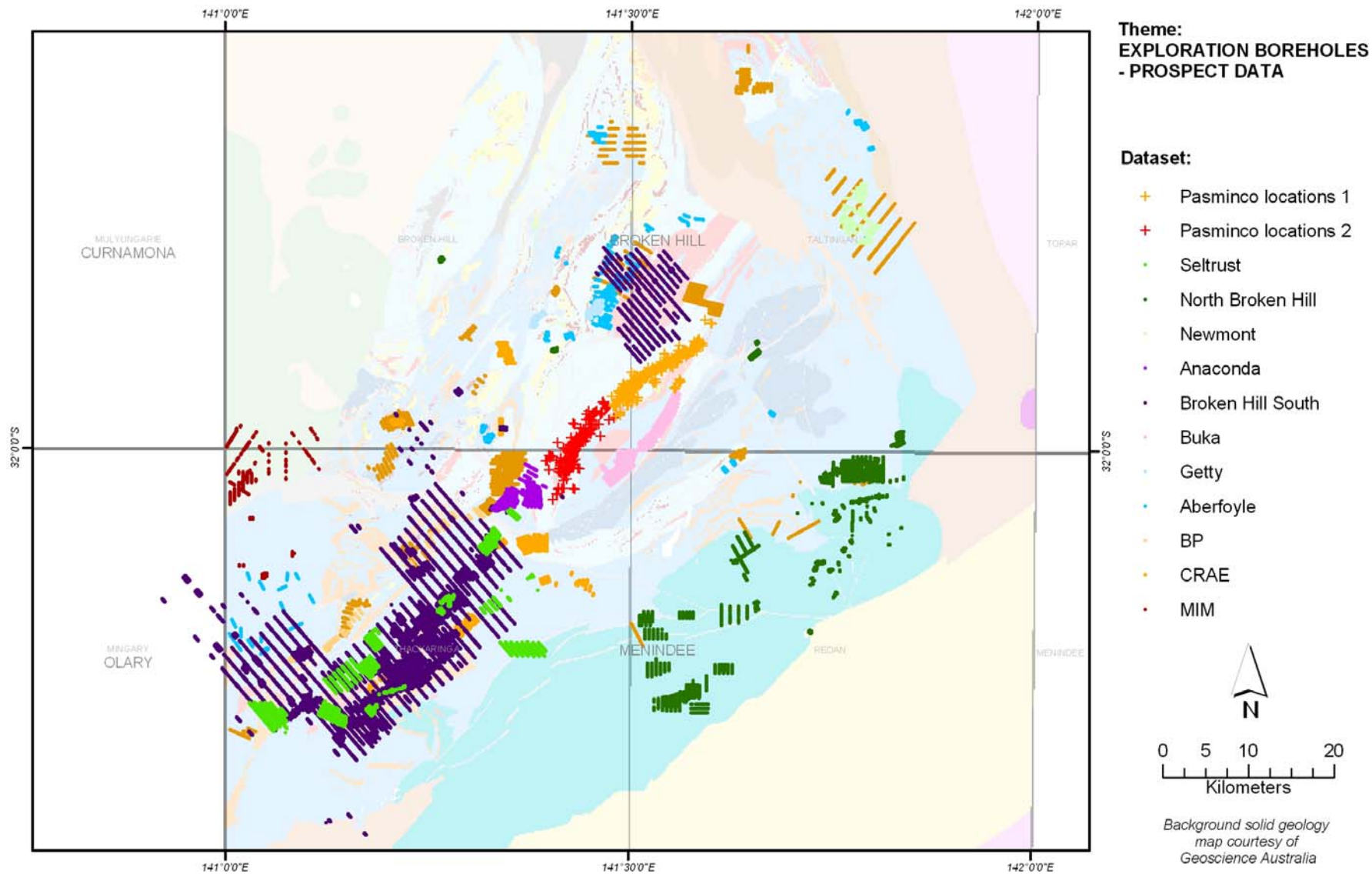
Map 8.1.2 Exploration Boreholes by company the Curnamona Province
