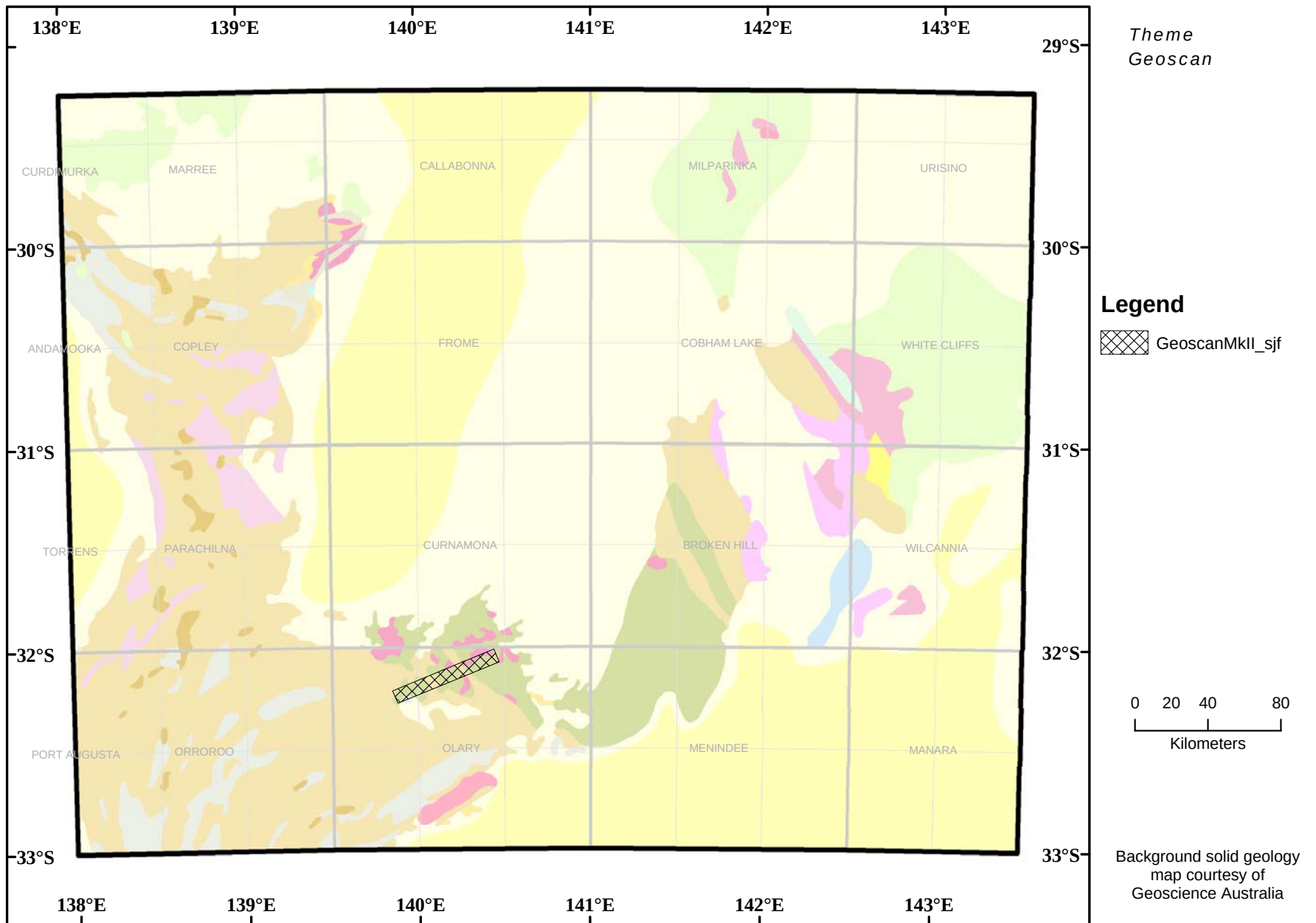
Map 11.3 Extent of GeoScan data acquisition over the Curnamona Province
