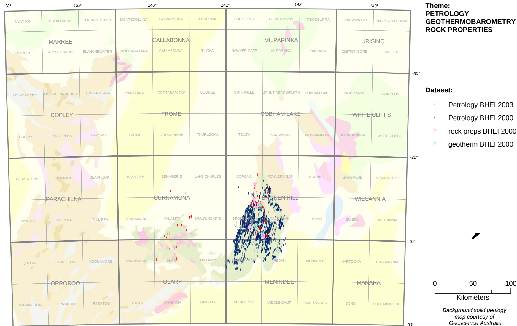
Map 7.5 Location of petrographic studies, geothermobarometric data points and samples for rock property analysis for the Curnamona Province
