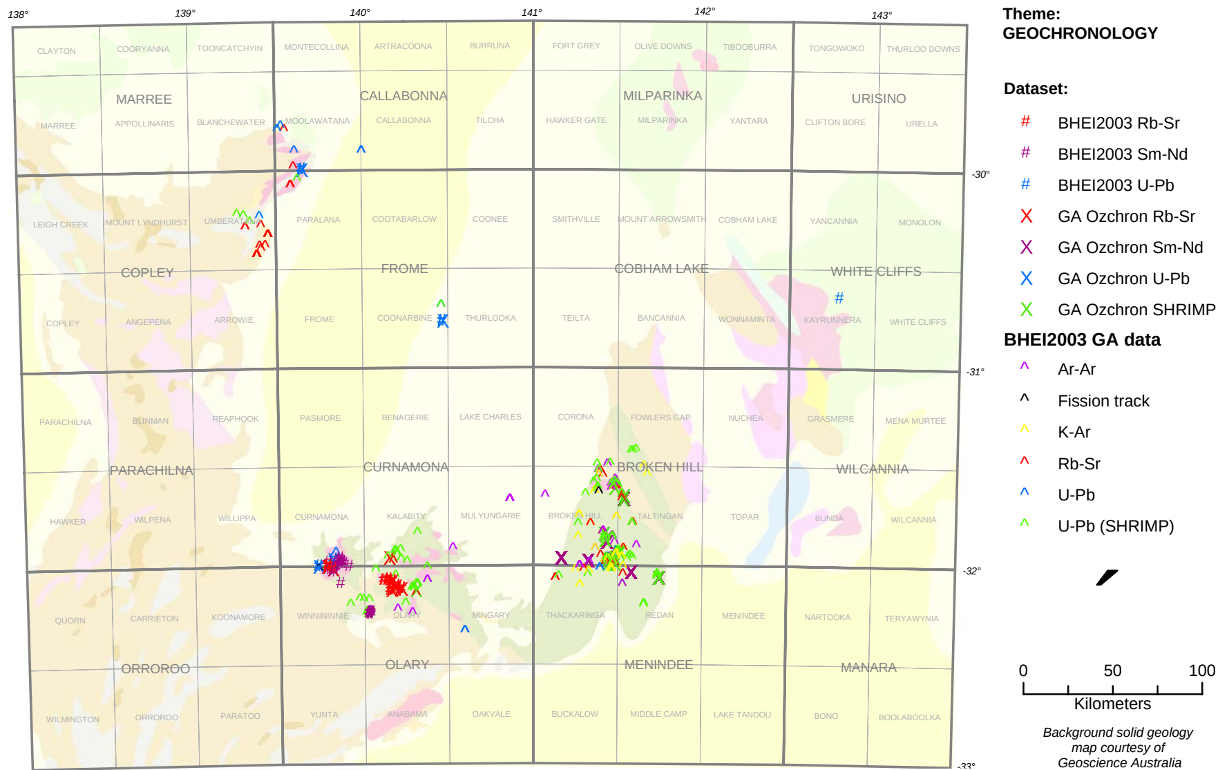
Map 8.3 Locations of samples for isotopic analysis in the Curnamona Province, including U-Pb geochronology
