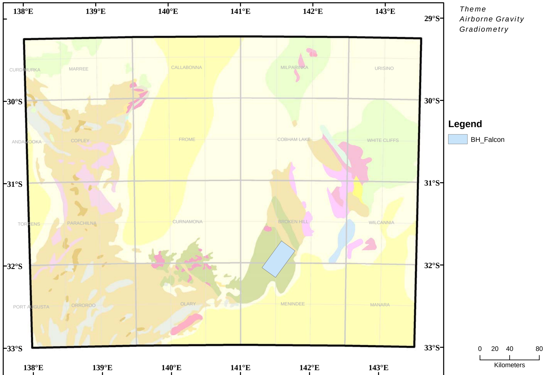
Map 9.5 Coverage of airborne gravity gradiometry surveys in the Curnamona Province
