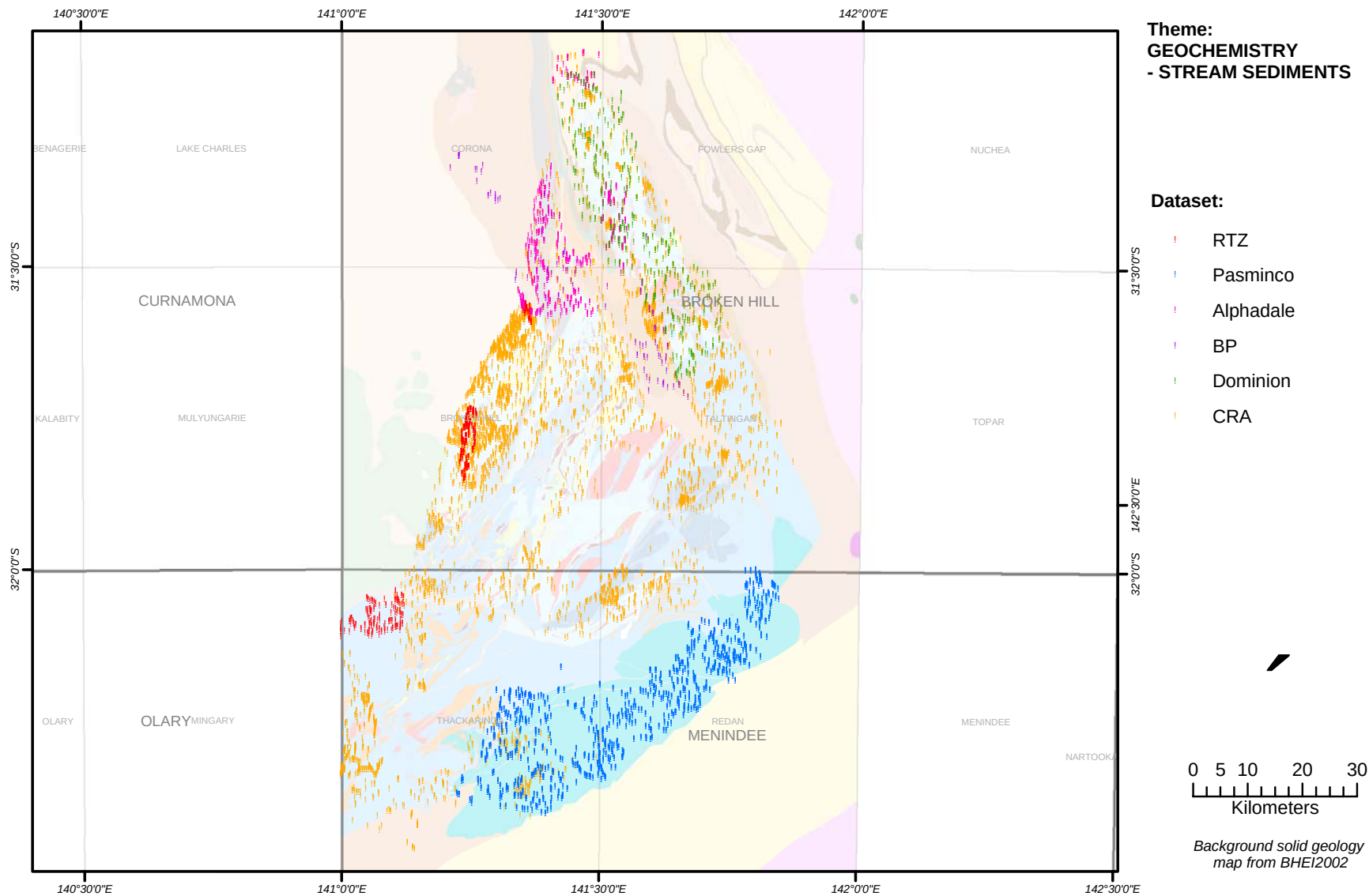
Map 8.1.4 Stream sediment geochemistry samples in the Curnamona Province
