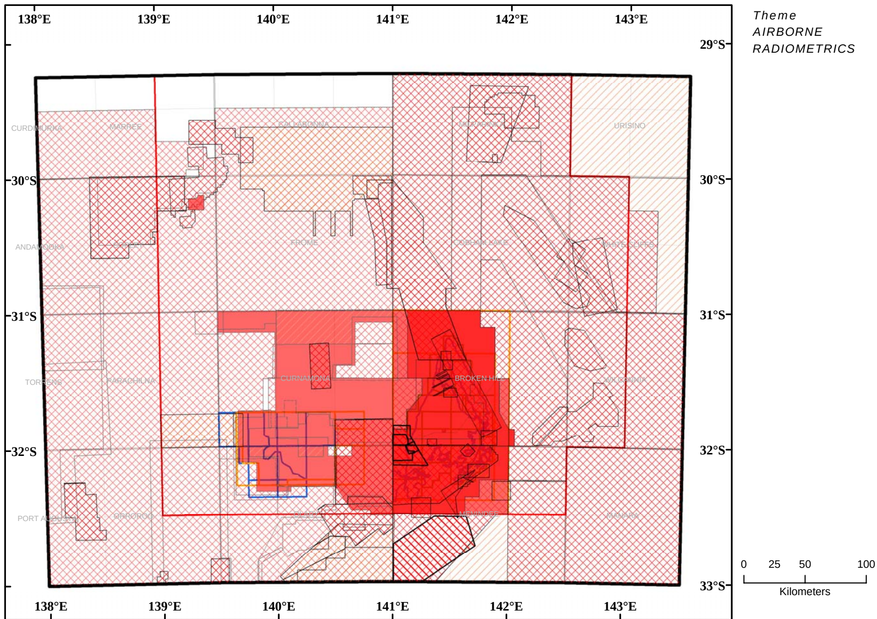
Map 9.3 Coverage of airborne radiometric surveys in the Curnamona Province
