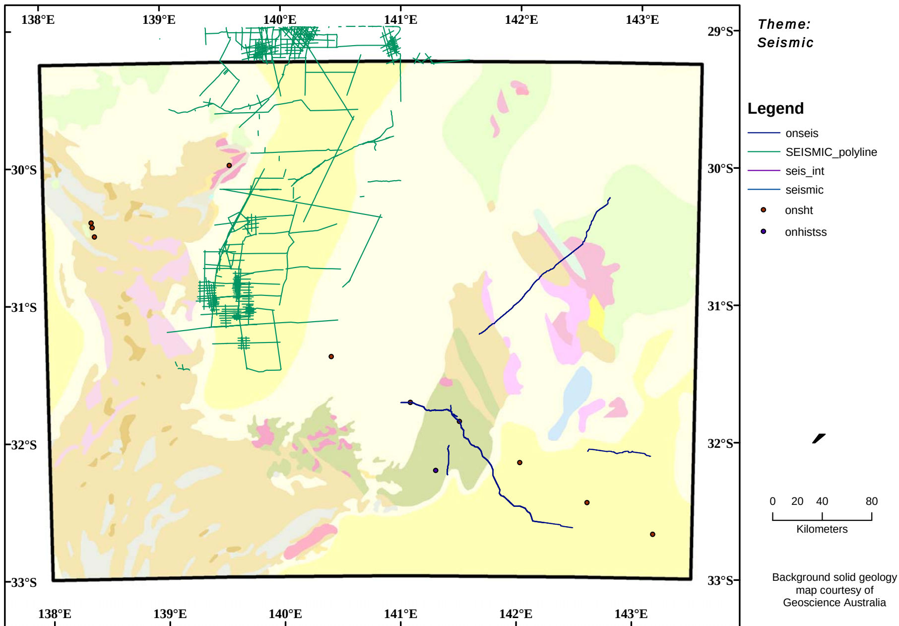
Map 9.6 Coverage of seismic surveys in the Curnamona Province
