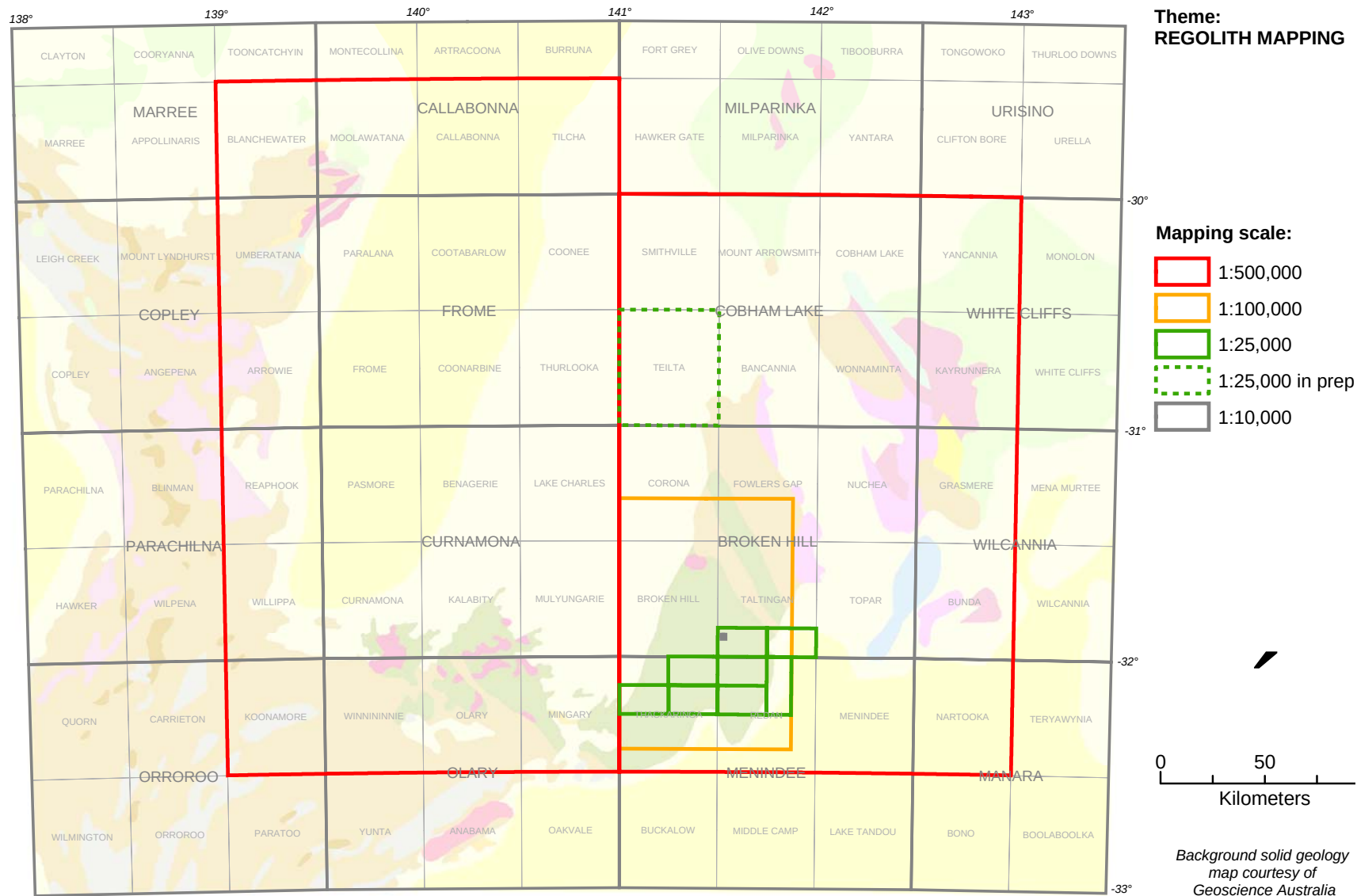
Map 7.2 Regolith Mapping coverage for the Curnamona Province
