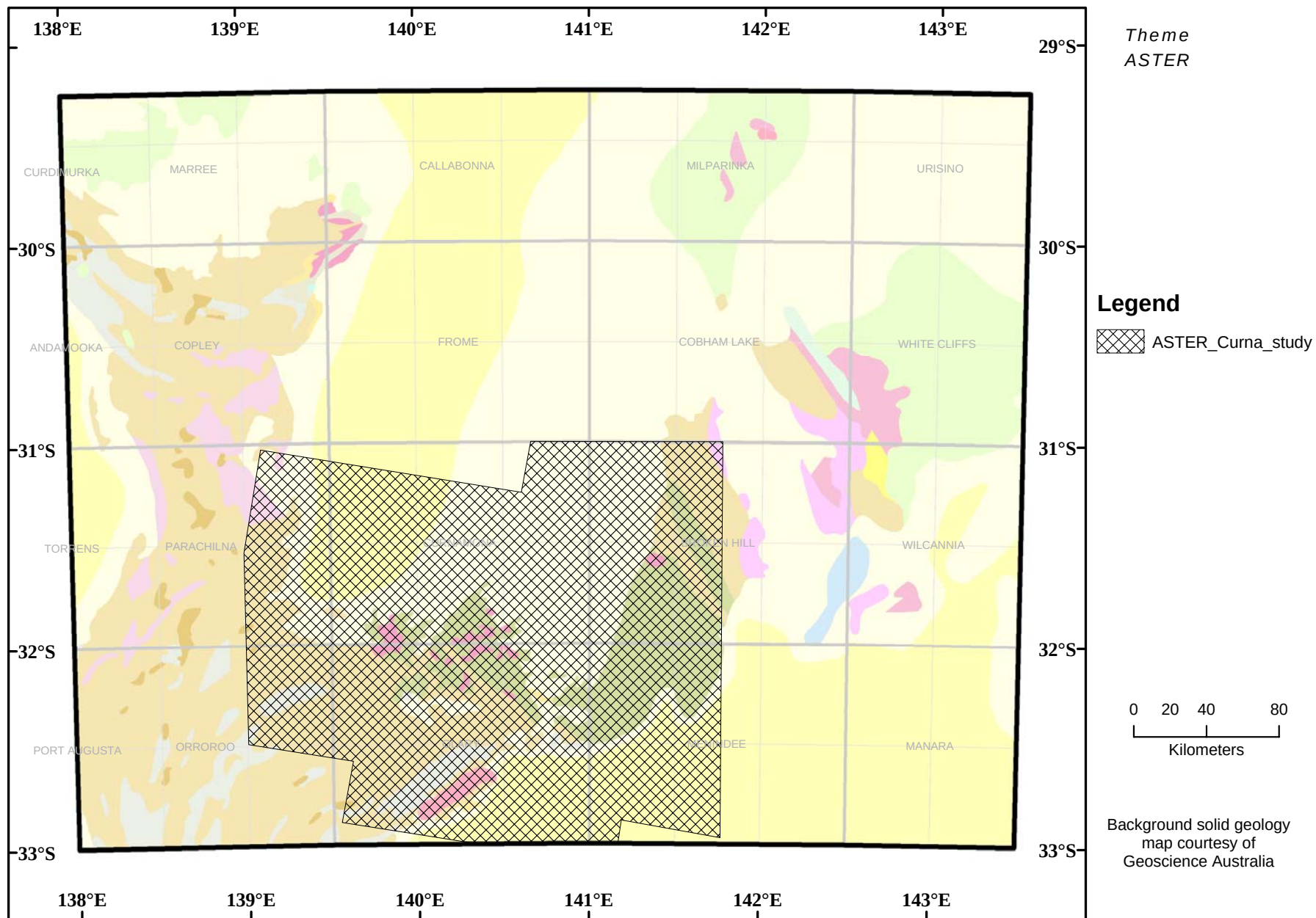
Map 11.1.1 Extent of ASTER data acquisition over the Curnamona Province
