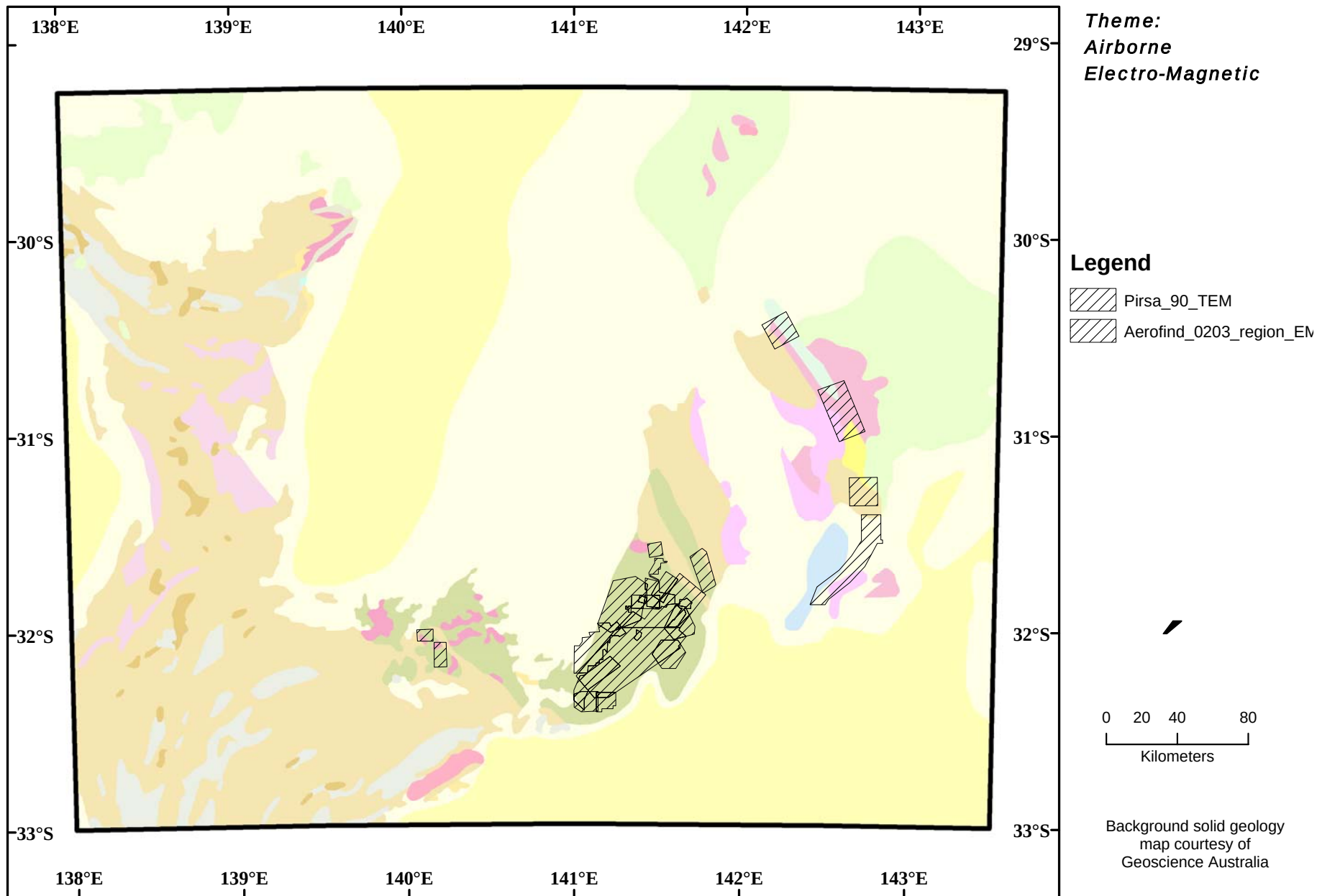
Map 9.1 Coverage of airborne electromagnetic surveys in the Curnamona Province
