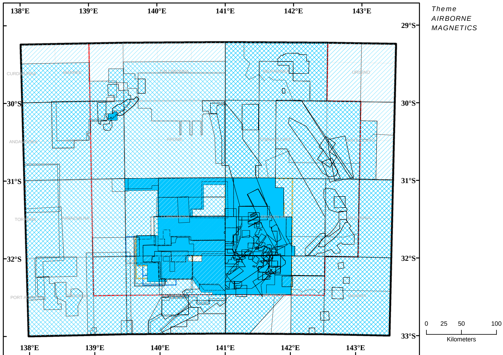
Map 9.2 Coverage of airborne magnetic surveys in the Curnamona Province
