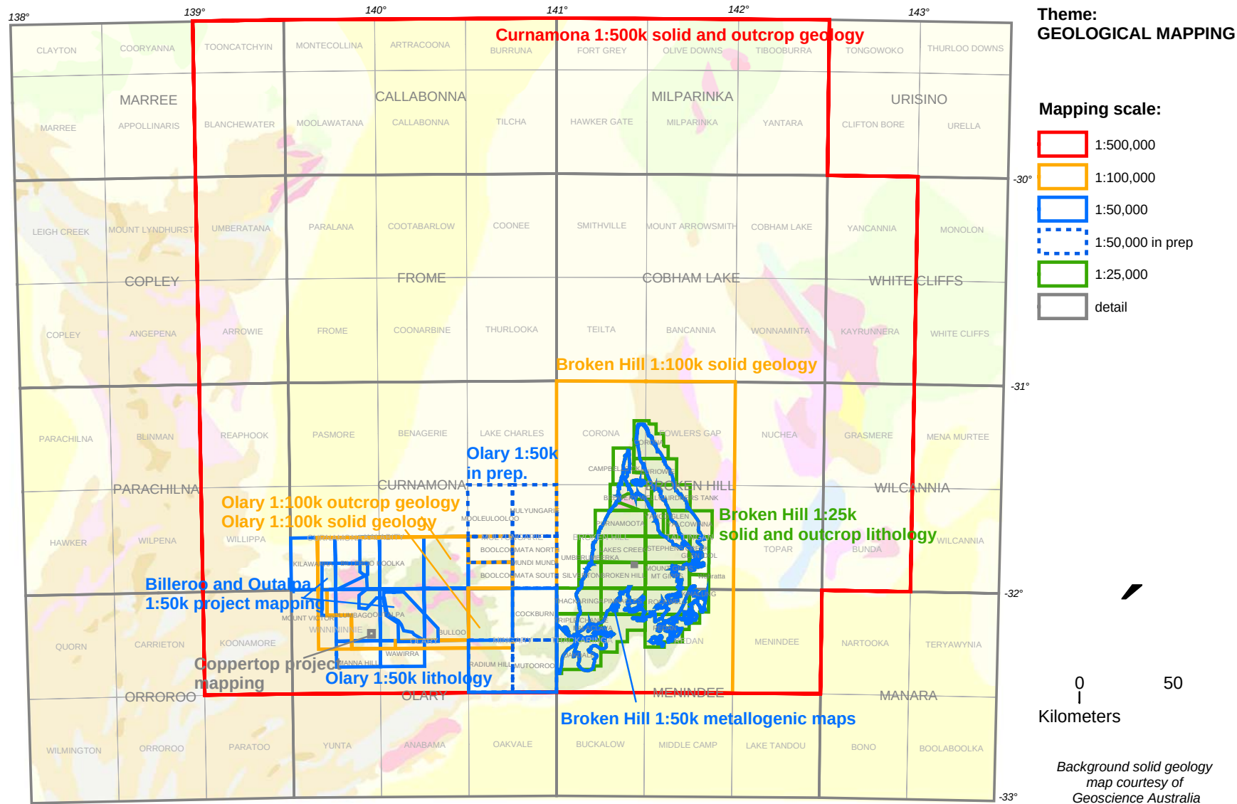
Map 7.1 Geological Mapping coverage for the Curnamona Province
