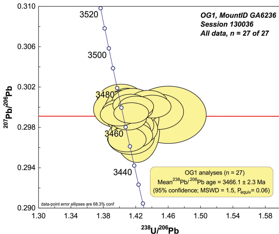
Appendix Figure A.2 Tera-Wasserburg concordia diagram for OG1 data. Heavy red line denotes reference value for OG1 ( ^{207}\text{Pb} / ^{206}\text{Pb} = 0.29907 ).
