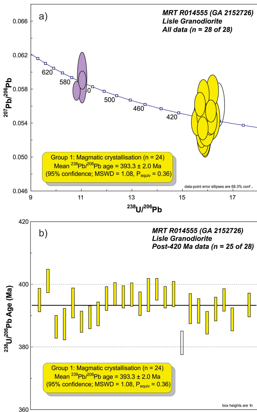
Figure 2.2 SHRIMP U–Pb data for zircons from the Lisle Granodiorite (MRT R014555, GA 2152726). (a) Tera-Wasserburg concordia diagram; (b) Post-420 Ma ^{238}\text{U}/^{206}\text{Pb} ages in order of acquisition. Yellow fill denotes Group 1 (magmatic crystallisation); purple fill denotes Group 2 (inheritance); white fill denotes Group 3 (analysis affected by loss of radiogenic Pb). Heavy black line: weighted mean ^{238}\text{U}/^{206}\text{Pb} age.
