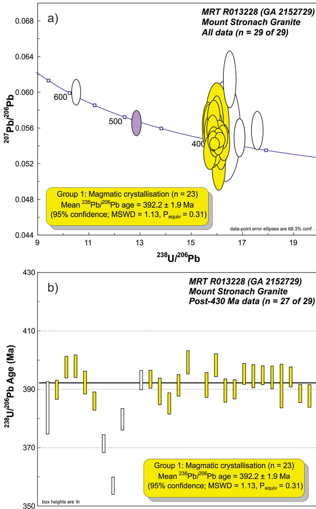
Figure 2.4 SHRIMP U–Pb data for zircons from the Mount Stronach Granite (MRT R013228, GA 2152729). (a) Tera-Wasserburg concordia diagram; (b) Post-430 Ma ^{238}\text{U}/^{206}\text{Pb} ages in order of acquisition. Yellow fill denotes Group 1 (magmatic crystallisation); purple fill denotes Group 2 (inheritance); white fill denotes relatively high common Pb ( ^{206}\text{Pb}_c > 0.9\% ). Heavy black line: weighted mean ^{238}\text{U}/^{206}\text{Pb} age.
