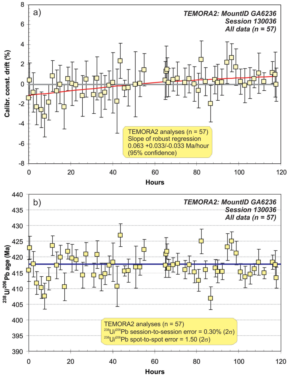
Appendix Figure A.1 (a) SHRIMP data for ^{238}\text{U}/^{206}\text{Pb} reference zircon TEMORA2 analysed during session 130036, illustrating the existence of measurable drift of the ^{238}\text{U}/^{206}\text{Pb} calibration as the session progressed; Heavy red line - robust regressions of individual ^{238}\text{U}/^{206}\text{Pb} ages against session duration. (b) SHRIMP data for ^{238}\text{U}/^{206}\text{Pb} reference zircon TEMORA2 independently corrected for secular drift. Heavy blue line denotes reference value for TEMORA2 ( ^{238}\text{U}/^{206}\text{Pb} age = 416.8 Ma).
