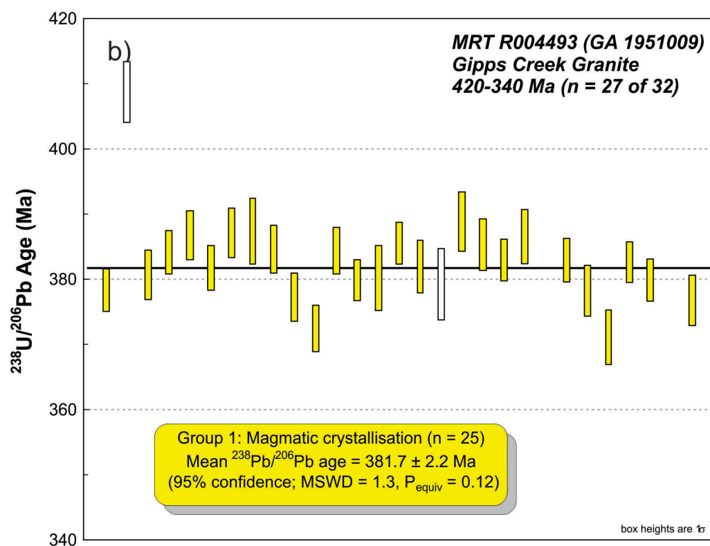
Figure 2.8 SHRIMP U–Pb data for zircons from the Gipps Creek Granite (MRT R004493, GA 1951009). (a) Tera-Wasserburg concordia diagram of pre-300 Ma data (analysis 24.1.1 not shown); (b) 420–340 Ma ^{238}\text{U}/^{206}\text{Pb} ages in order of acquisition. Yellow fill denotes Group 1 (magmatic crystallisation); purple fill denotes Group 2 (inheritance); white fill denotes relatively high common Pb ( ^{206}\text{Pb}_c > 3\% ). Heavy black line: weighted mean ^{238}\text{U}/^{206}\text{Pb} age.
