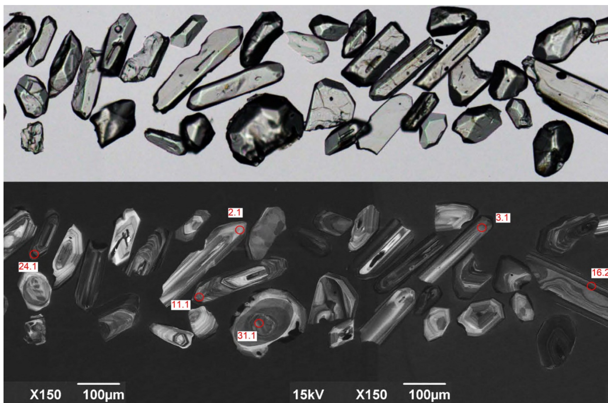
Figure 2.7 Representative zircons from the Gipps Creek Granite (MRT R004493, GA 1951009). Transmitted light image is shown in the upper half; cathodoluminescence image in the lower half. SHRIMP analysis sites are labelled.
