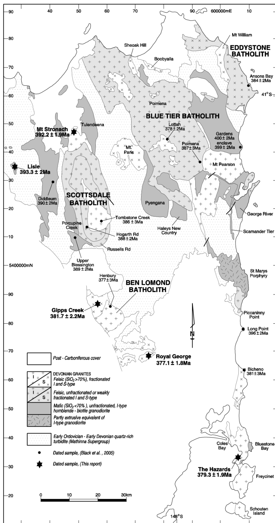
Figure 1.1 Map of northeast Tasmania showing granite plutons, sample locations and newly determined emplacement ages; other plutons mentioned in the text are also labelled (modified after Black et al., 2005).
