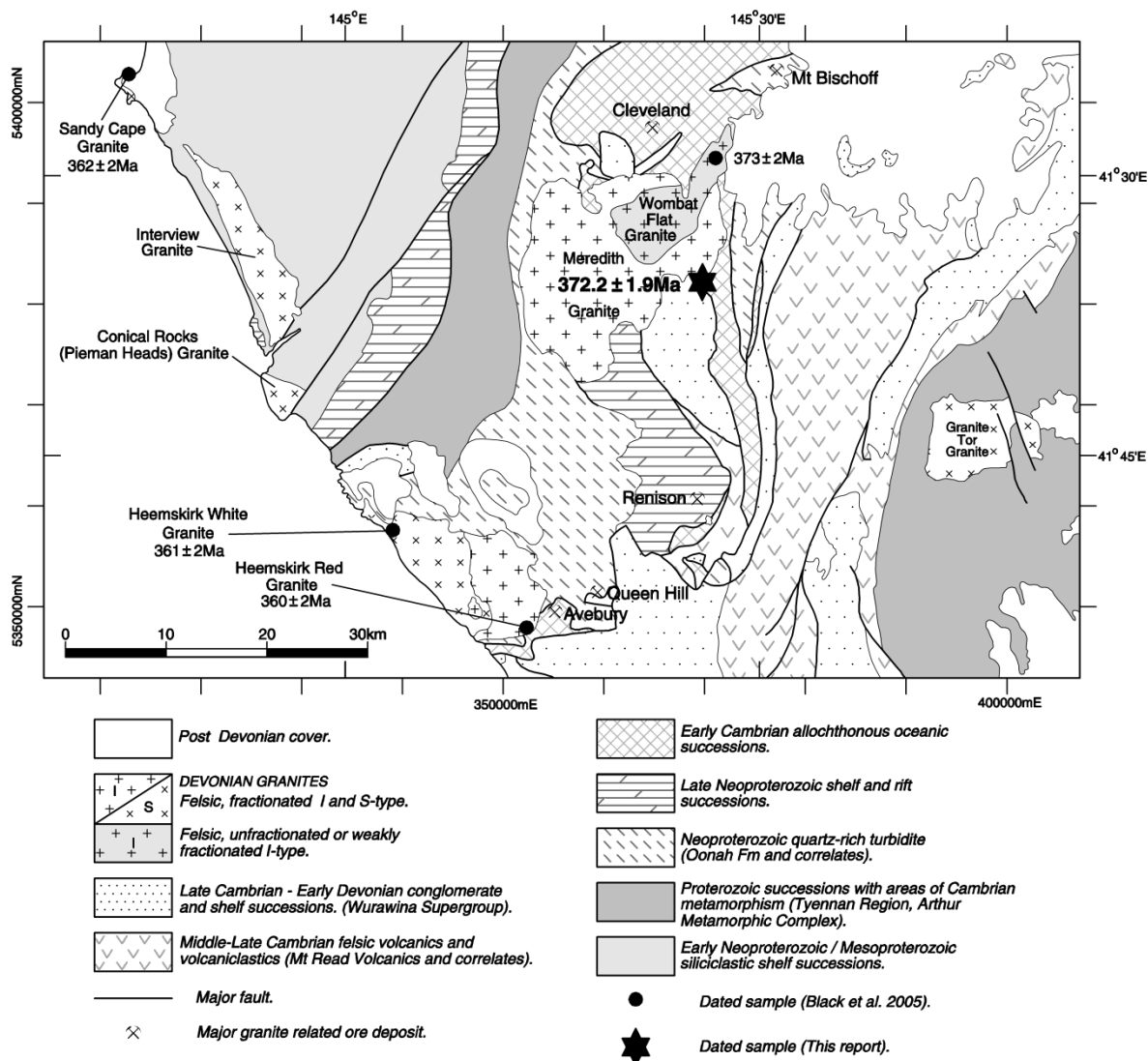
Figure 1.2 Map of northwest Tasmania showing granite plutons, sample locations and newly determined emplacement ages; other plutons mentioned in the text are also labelled.
