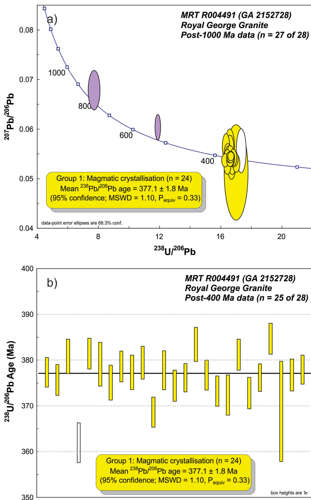
Figure 2.6 SHRIMP U–Pb data for zircons from the Royal George Granite (MRT R004491, GA 2152728). (a) Tera-Wasserburg concordia diagram of post-1000 Ma data (Group 3 inherited individual not shown); (b) Post-400 Ma ^{238}\text{U}/^{206}\text{Pb} ages in order of acquisition. Yellow fill denotes Group 1 (magmatic crystallisation); purple fill denotes Group 2 (inheritance); white fill denotes excluded analysis (instrumental instability). Heavy black line: weighted mean ^{238}\text{U}/^{206}\text{Pb} age.
