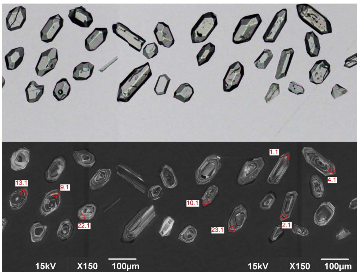
Figure 2.1 Representative zircons from the Lisle Granodiorite (MRT R014555, GA 2152726). Transmitted light image is shown in the upper half; cathodoluminescence image in the lower half. SHRIMP analysis sites are labelled.
