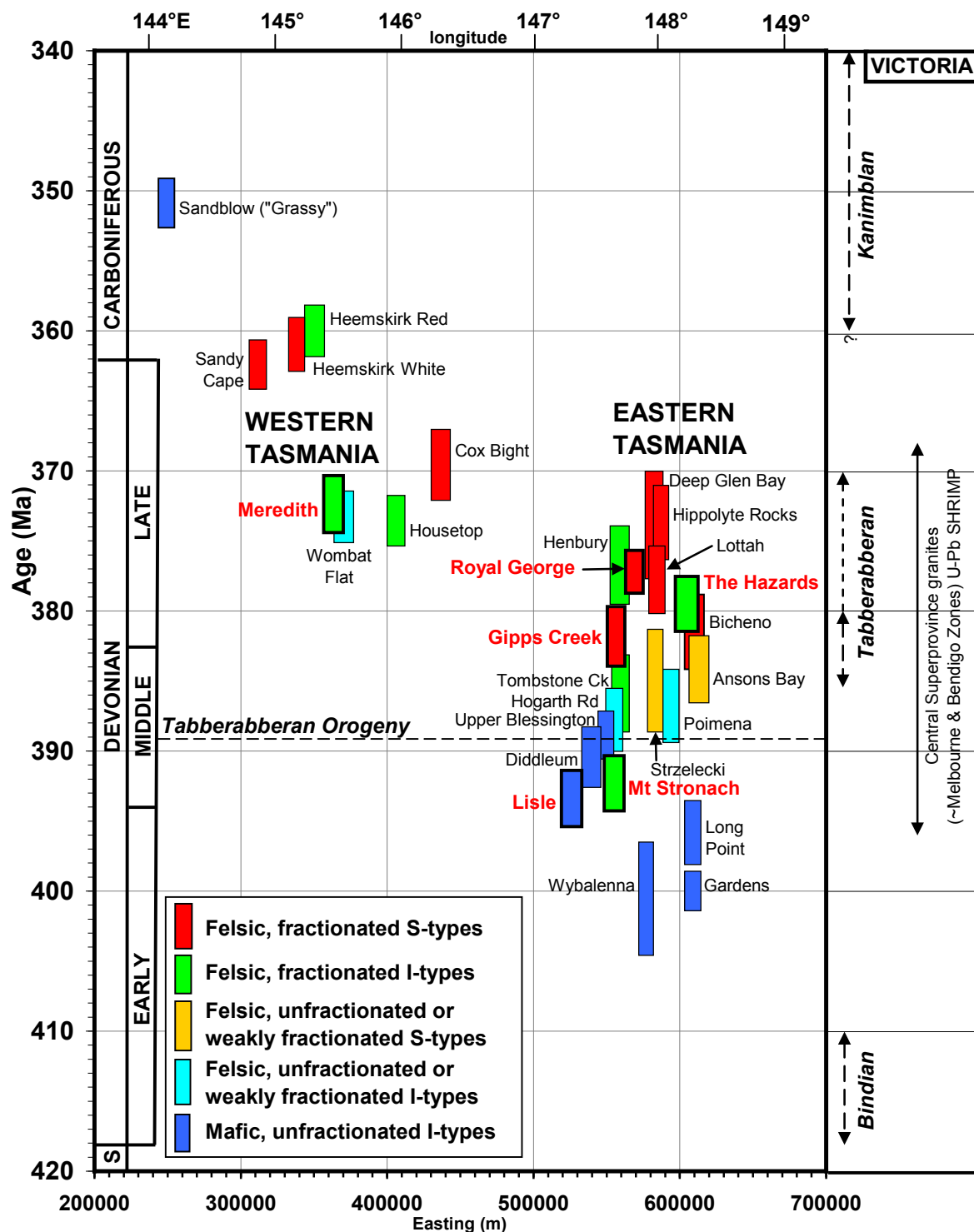
Figure 1.3 Summary time-space diagram (modified after Black et al., 2005, Figure 7) plotting emplacement age versus easting for Devonian–Carboniferous granites in Tasmania. New data presented in this record shown with heavy outline and red labels; the age uncertainties depicted include the additional component for session-specific calibration uncertainty. Time scale after Tucker et al. (1998), Victorian data after VandenBerg et al. (2000); see Black et al. (2005) for sources.
