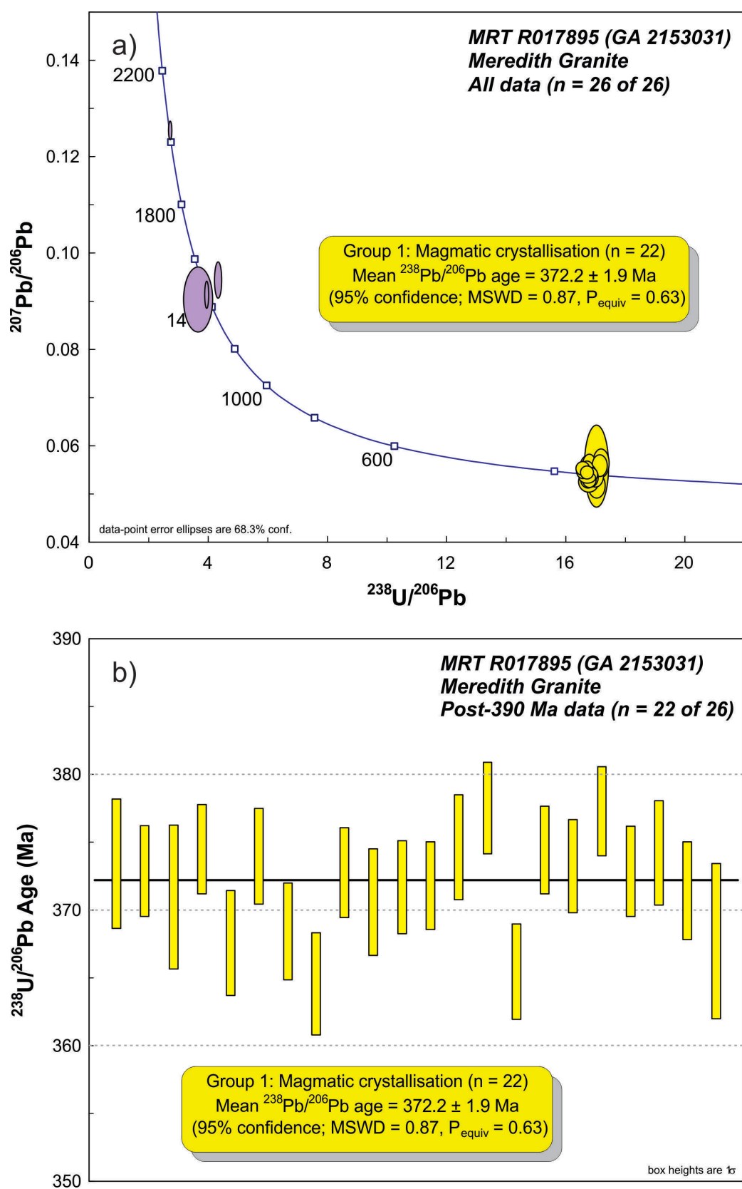
Figure 3.2 SHRIMP U–Pb data for zircons from the Meredith Granite (MRT R017895, GA 2153031). (a) Tera-Wasserburg concordia diagram; (b) Post-390 Ma ^{238}\text{U}/^{206}\text{Pb} ages in order of acquisition. Yellow fill denotes Group 1 (magmatic crystallisation); purple fill denotes Group 2 (inheritance). Heavy black line: weighted mean ^{238}\text{U}/^{206}\text{Pb} age.
