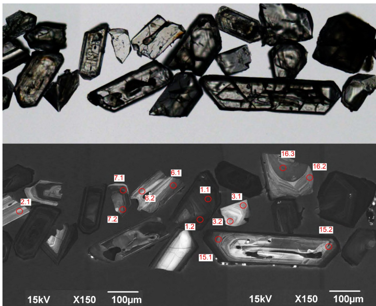
Figure 2.9 Representative zircons from The Hazards Granite (MRT R004499, GA 1950975). Transmitted light image is shown in the upper half; cathodoluminescence image in the lower half. SHRIMP analysis sites are labelled.
