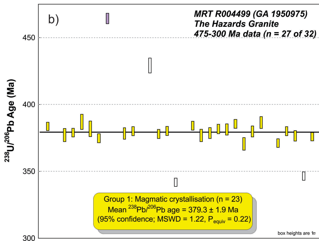
Figure 2.10 SHRIMP U–Pb data for zircons from The Hazards Granite (MRT R004499, GA 1950975). (a) Tera-Wasserburg concordia diagram for pre-230 Ma data (analysis 14.2.1 not shown); (b) ^{238}\text{U}/^{206}\text{Pb} ages in order of acquisition. Yellow fill denotes Group 1 (magmatic crystallisation); purple fill denotes Group 2 (inheritance); white fill denotes relatively high common Pb ( ^{206}\text{Pb}_c > 1.7\% ) and Group 3 analyses affected by loss of radiogenic Pb. Heavy black line: weighted mean ^{238}\text{U}/^{206}\text{Pb} age.
