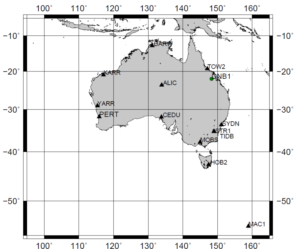
Figure 1: Station DNB1 (circle) at the BMA Daunia Mine in Queensland and AFN/ARGN/IGS (black triangles) stations used in GPS data processing.
