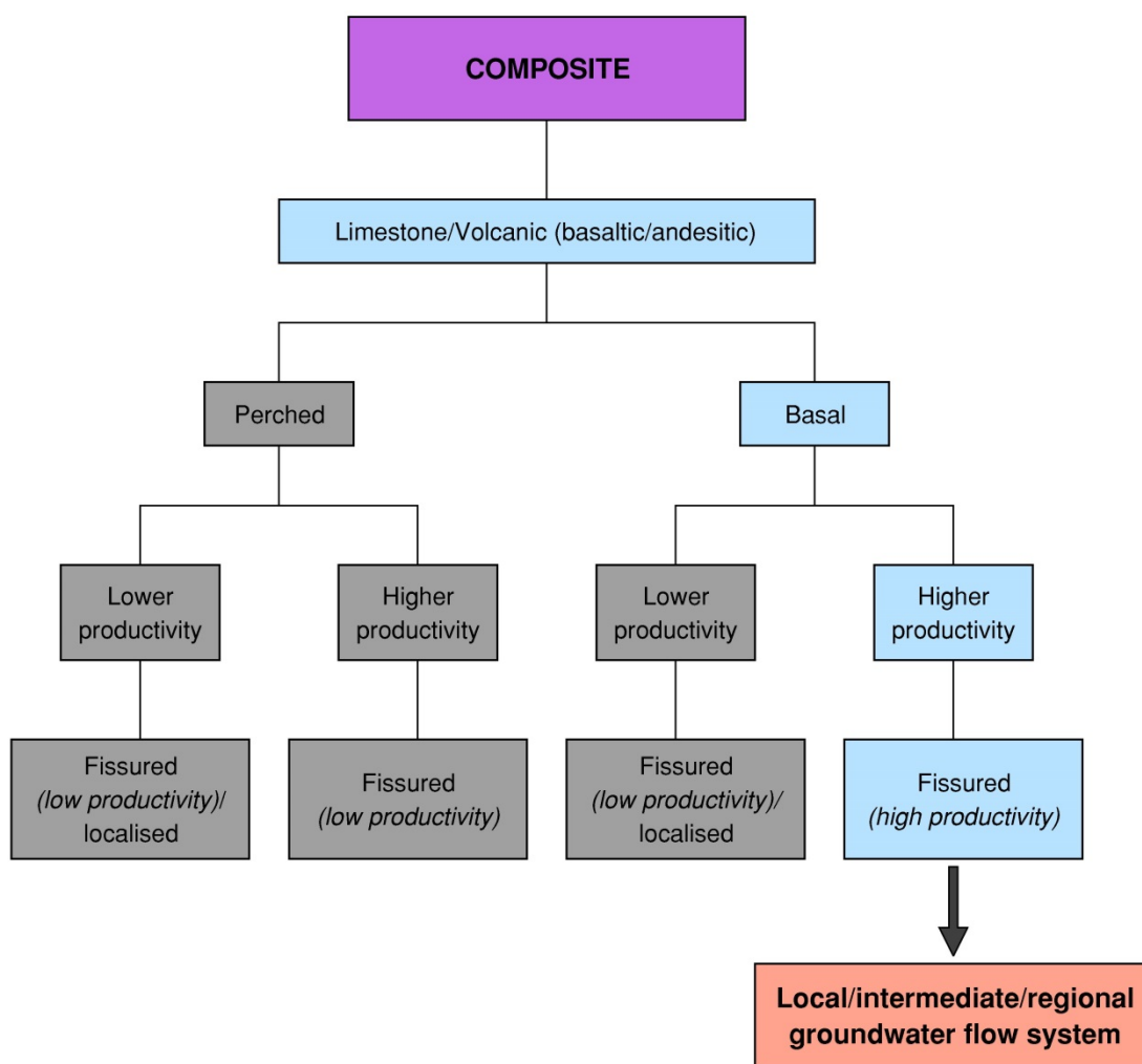
Figure 3.16 Typology for Composite islands. The purple box indicates the island type; the blue boxes highlight the characteristics of the assumed principal aquifer; the grey boxes indicate characteristics of other possible aquifers within the island type and the pink box highlights the GFS which has been assumed to be typical of the principal aquifer. Note that the most productive aquifer is assumed to occur in volcanic rock (fissured fractured aquifer type).
