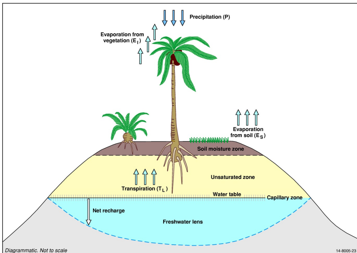
Appendix Figure F.2 Water balance model for the surface zone (comprising a soil moisture zone and an unsaturated zone) and freshwater lens on a small Low Carbonate island with no runoff (modified from Falkland 1993). Water balance terms are described in the text.
