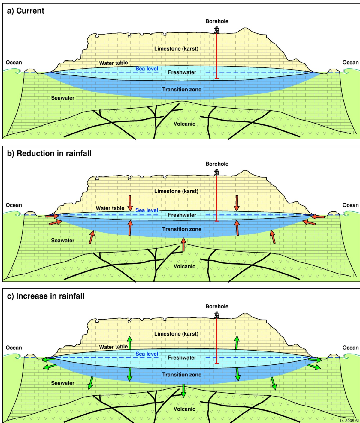
Appendix Figure E.2 Potential effect of b) reduction in rainfall or c) increase in rainfall on the freshwater lens of a Limestone island compared to the a) current situation (modified from Waterhouse 1984). Red arrows indicate a reduction in the size of the lens and green arrows indicate an increase in the size of the lens.
