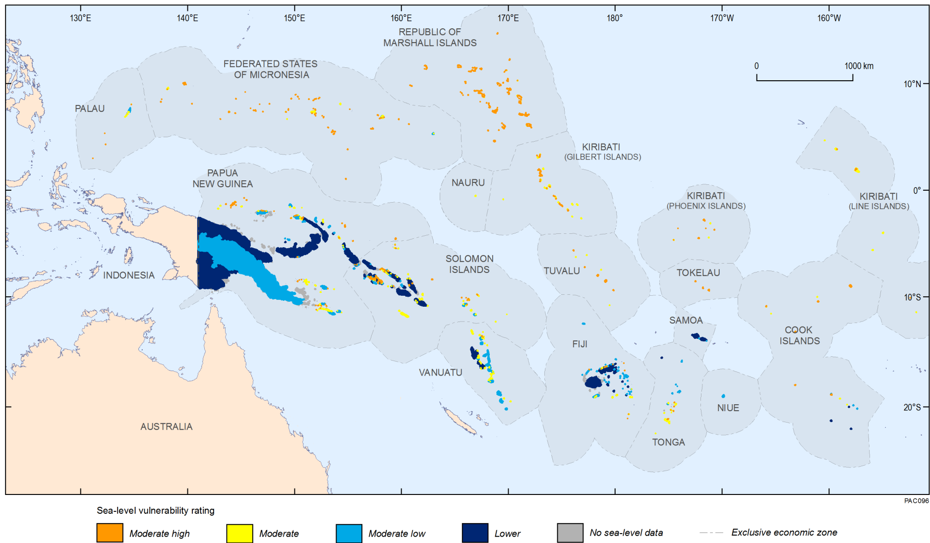
Figure 7.4 Regional map of relative potential vulnerability of groundwater systems on islands of the Pacific region to a rise in relative mean sea level in 2050.
