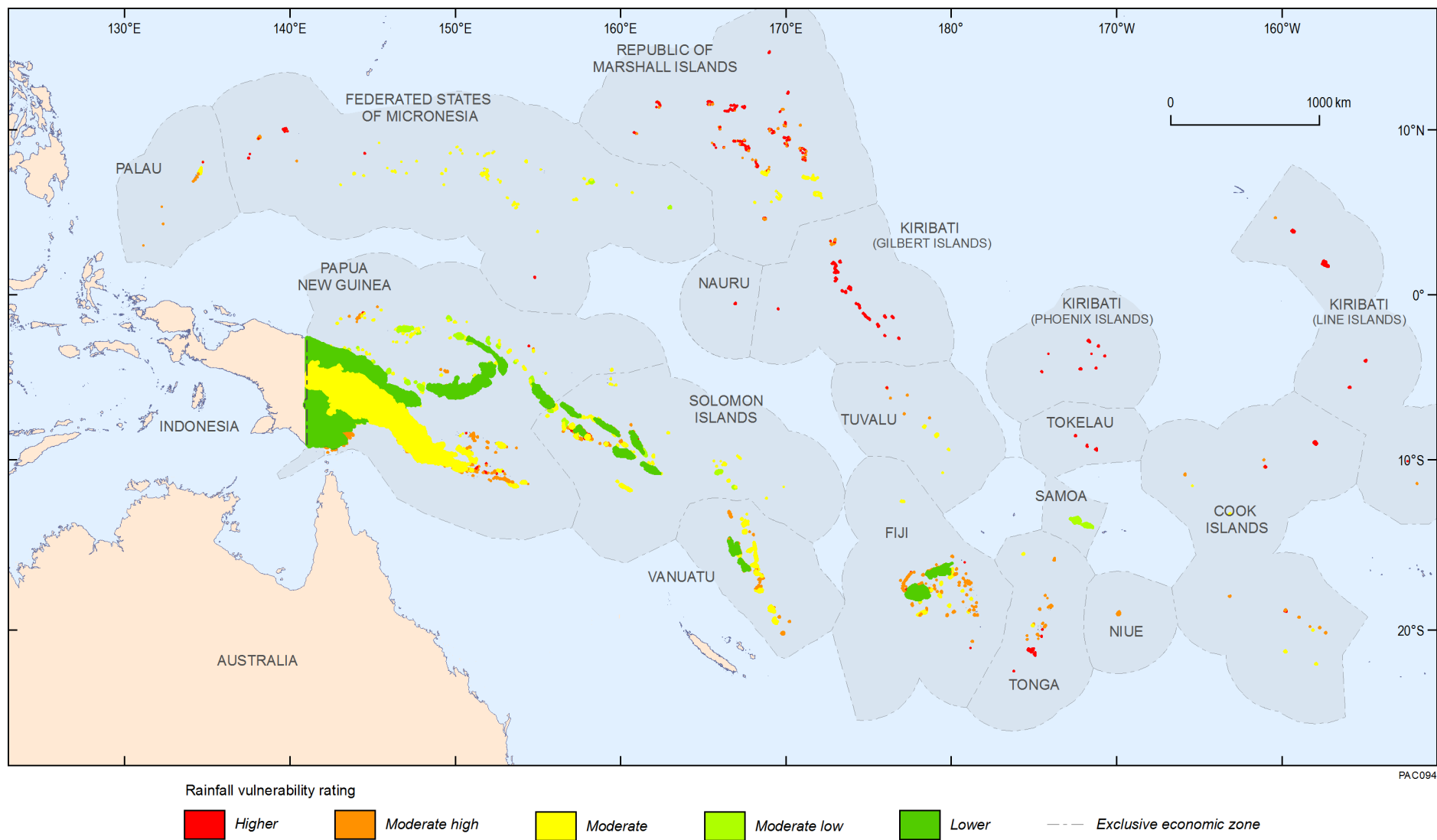
Figure 7.2 Regional map of potential vulnerability of groundwater systems on islands of the Pacific region to lowest mean annual rainfall in 2050.
