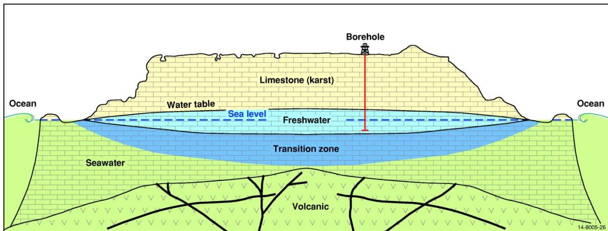
Figure 3.9 Main features of the aquifer system on a Limestone island (modified from Waterhouse 1984).
