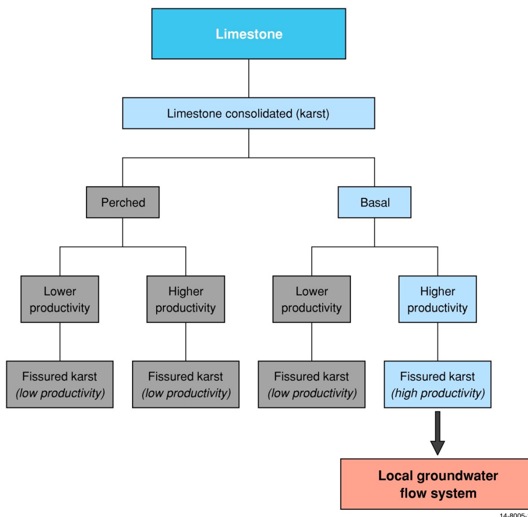
Figure 3.8 Typology for Limestone islands. The dark blue box indicates the island type; the blue boxes highlight the characteristics of the assumed principal aquifer; the grey boxes indicate characteristics of other possible aquifers within the island type and the pink box highlights the GFS which has been assumed to be typical of the principal aquifer.
