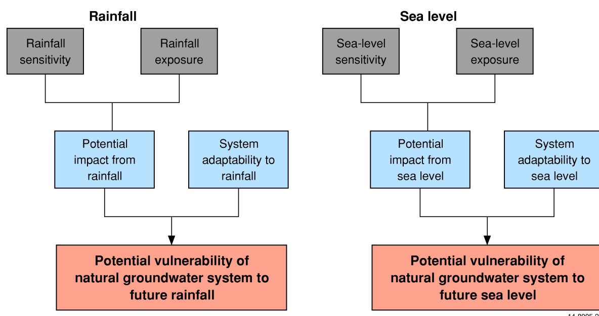
Figure 1.3 Functional vulnerability framework to assess the potential vulnerability of the natural groundwater system to projected future rainfall and sea level.
