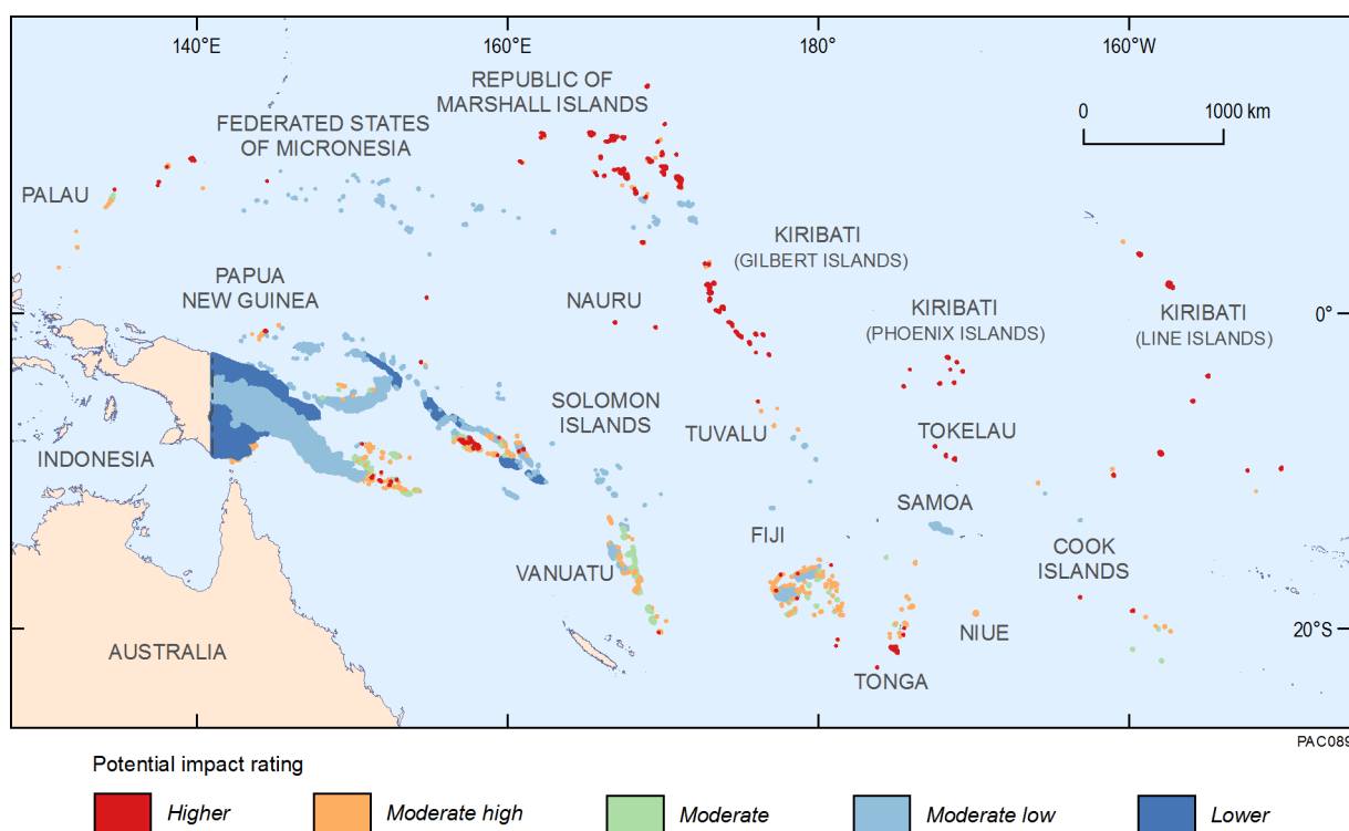
Figure 5.1 Potential impact of lowest mean annual rainfall in 2050 on fresh groundwater availability.
