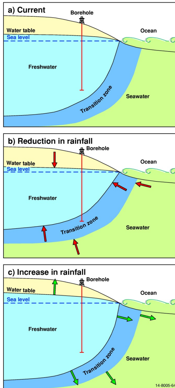
Appendix Figure E.5 Potential effect of b) reduction in rainfall or c) increase in rainfall on coastal aquifers of a Complex island compared to the a) current situation. Red arrows indicate a reduction in the size of the lens and green arrows indicate an increase in the size of the lens.
