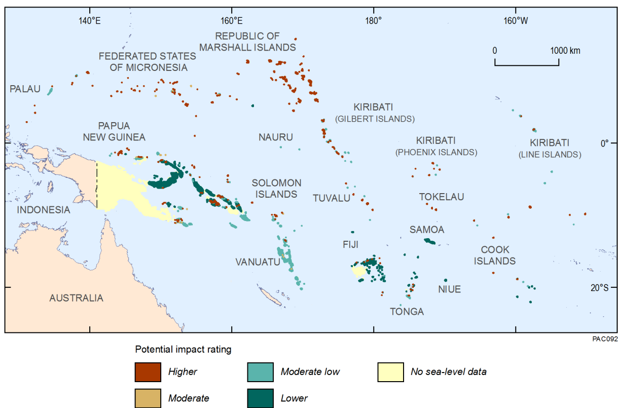
Figure 5.4 Potential impact of a rise in relative mean sea level in 2085.
