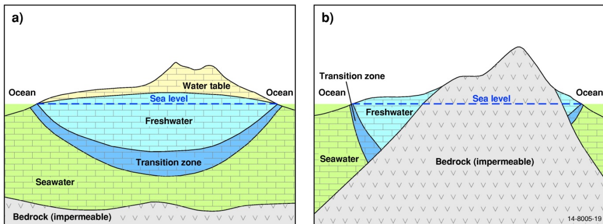
Figure 3.1 Island settings for a) freshwater lenses and b) coastal aquifers.
