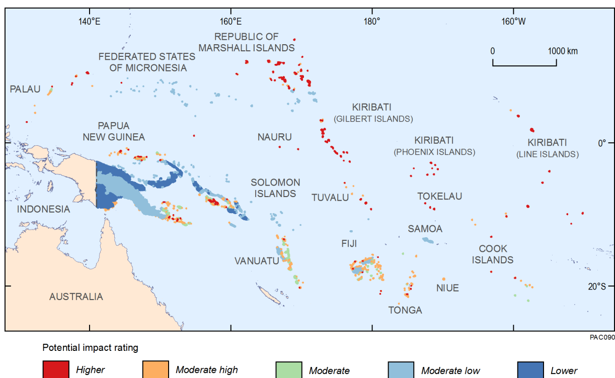
Figure 5.2 Potential impact of lowest mean annual rainfall in 2085 on fresh groundwater availability.
