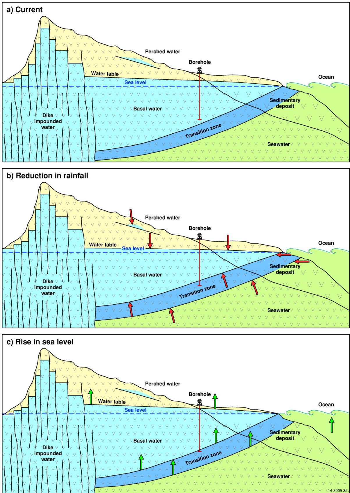
Figure 3.14 Potential effect of b) reduction in rainfall or c) rise in sea level on the aquifers of a Volcanic island compared to the a) current situation (modified from UNESCO 1991).
