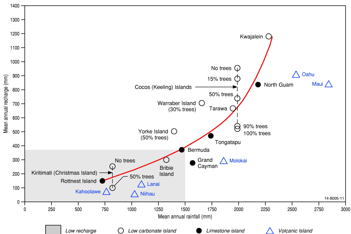
Appendix Figure F.1 Relationship between mean annual rainfall and mean annual recharge (for available data period) for a number of Low Carbonate, Limestone and Volcanic islands (modified from UNESCO 1991). The red curve has been fitted to the data for Low Carbonate and Limestone islands only. The figure also shows the influence of vegetation conditions on recharge.
