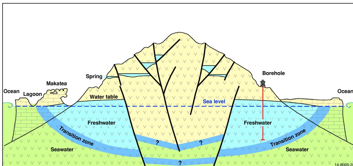
Figure 3.17 Main features of the aquifer system on a Composite island (modified from Waterhouse 1984). The question marks indicate that there may be connectivity from the basal aquifer across the dikes.
