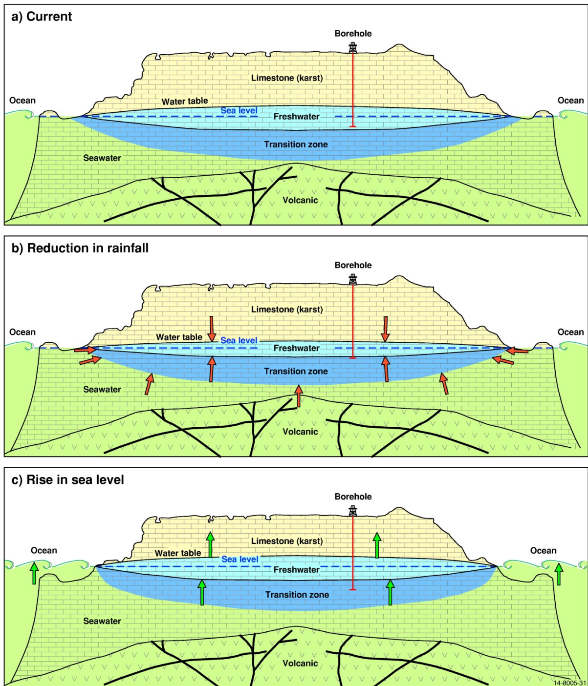
Figure 3.10 Potential effect of b) reduction in rainfall or c) rise in sea level on the freshwater lens of a Limestone island compared to the a) current situation (modified from Waterhouse 1984).
