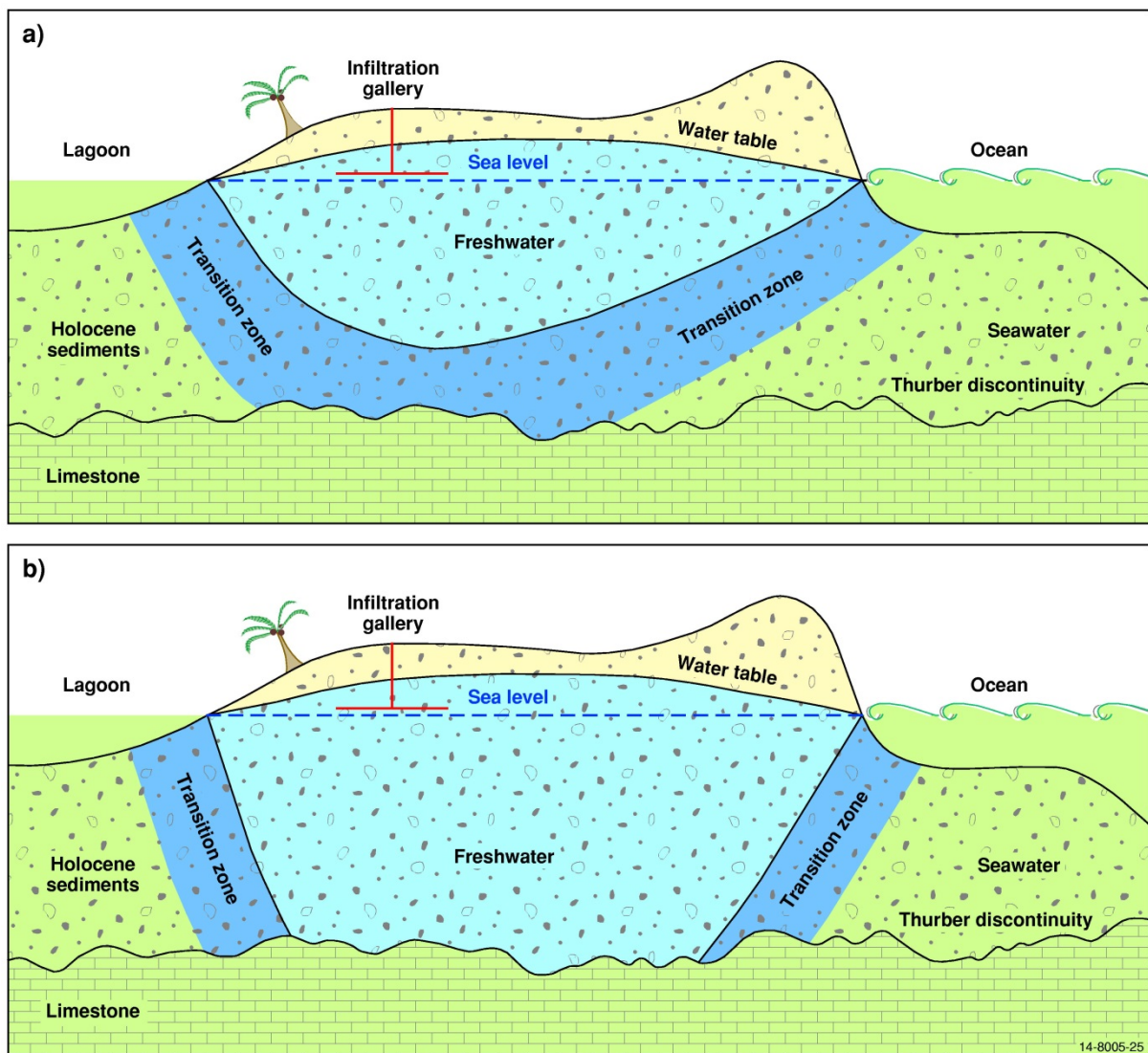
Figure 3.5 Main features of the aquifer system on a Low Carbonate island: a) thin freshwater lens that does not reach the Thurber Discontinuity; b) thick freshwater lens truncated at the Thurber Discontinuity.
