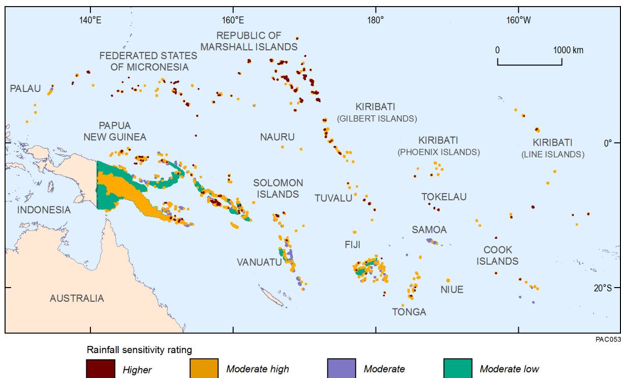
Figure 3.26 Aquifer sensitivity to change in rainfall-recharge for islands in the Pacific region with potential for fresh groundwater (refer to Table 3.3).
