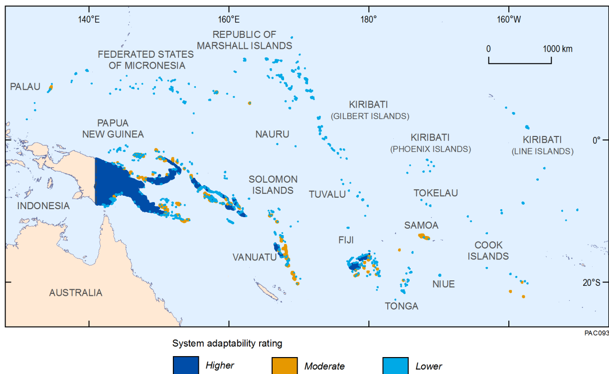
Figure 6.1 Adaptability of groundwater system (principal aquifer) to periods of low rainfall or mean SLR for islands in the Pacific region with potential for fresh groundwater (refer to Table 6.1).
