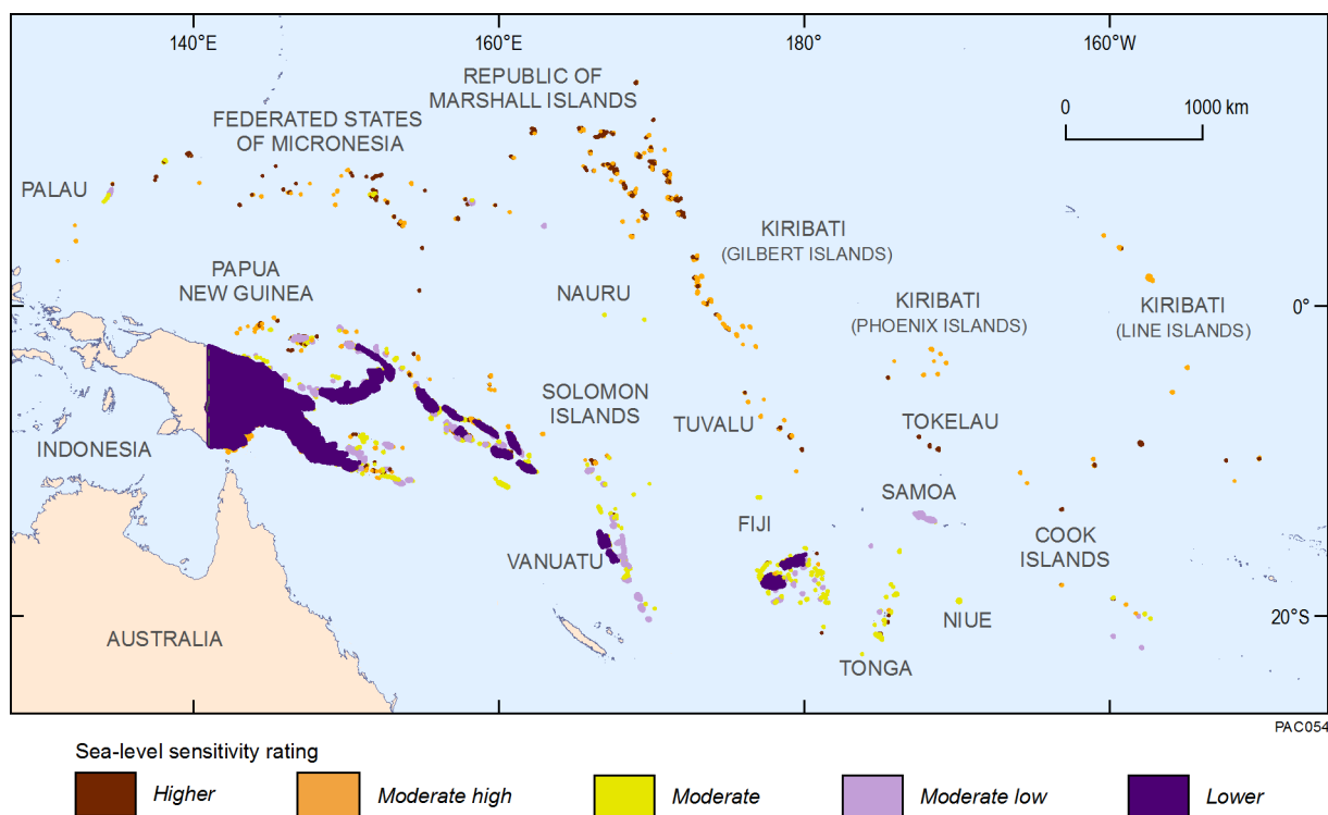
Figure 3.28 Aquifer sensitivity to mean SLR for islands in the Pacific region with potential for fresh groundwater (refer to Table 3.6).
