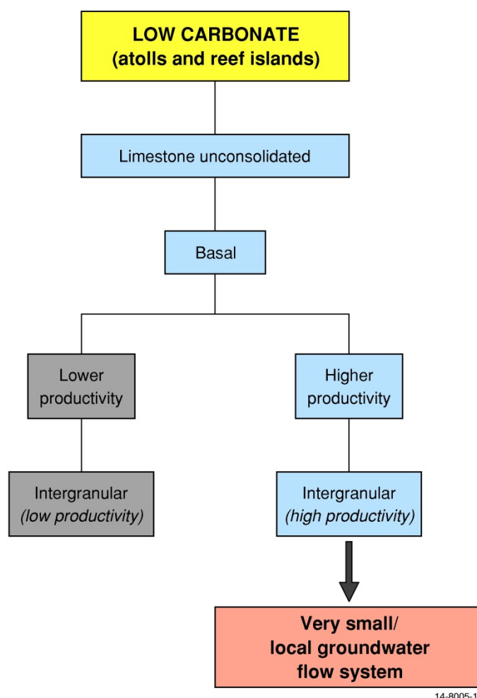
Figure 3.4 Typology for Low Carbonate islands. The yellow box indicates the island type; the blue boxes highlight the characteristics of the assumed principal aquifer; the grey boxes indicate characteristics of other possible aquifers within the island type and the pink box highlights the GFS which has been assumed to be typical of the principal aquifer.
