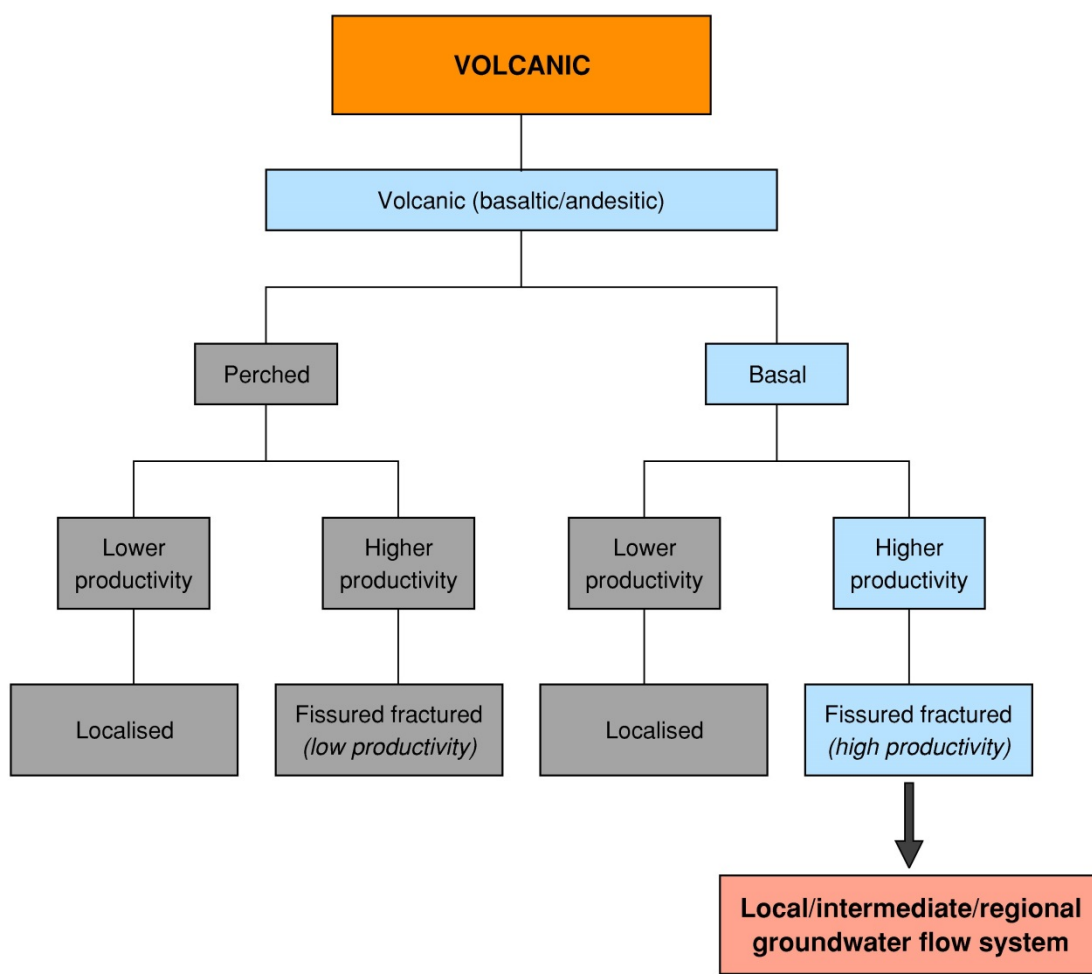
Figure 3.12 Typology for Volcanic islands. The orange box indicates the island type; the blue boxes highlight the characteristics of the assumed principal aquifer; the grey boxes indicate characteristics of other possible aquifers within the island type and the pink box highlights the GFS which has been assumed to be typical of the principal aquifer.
