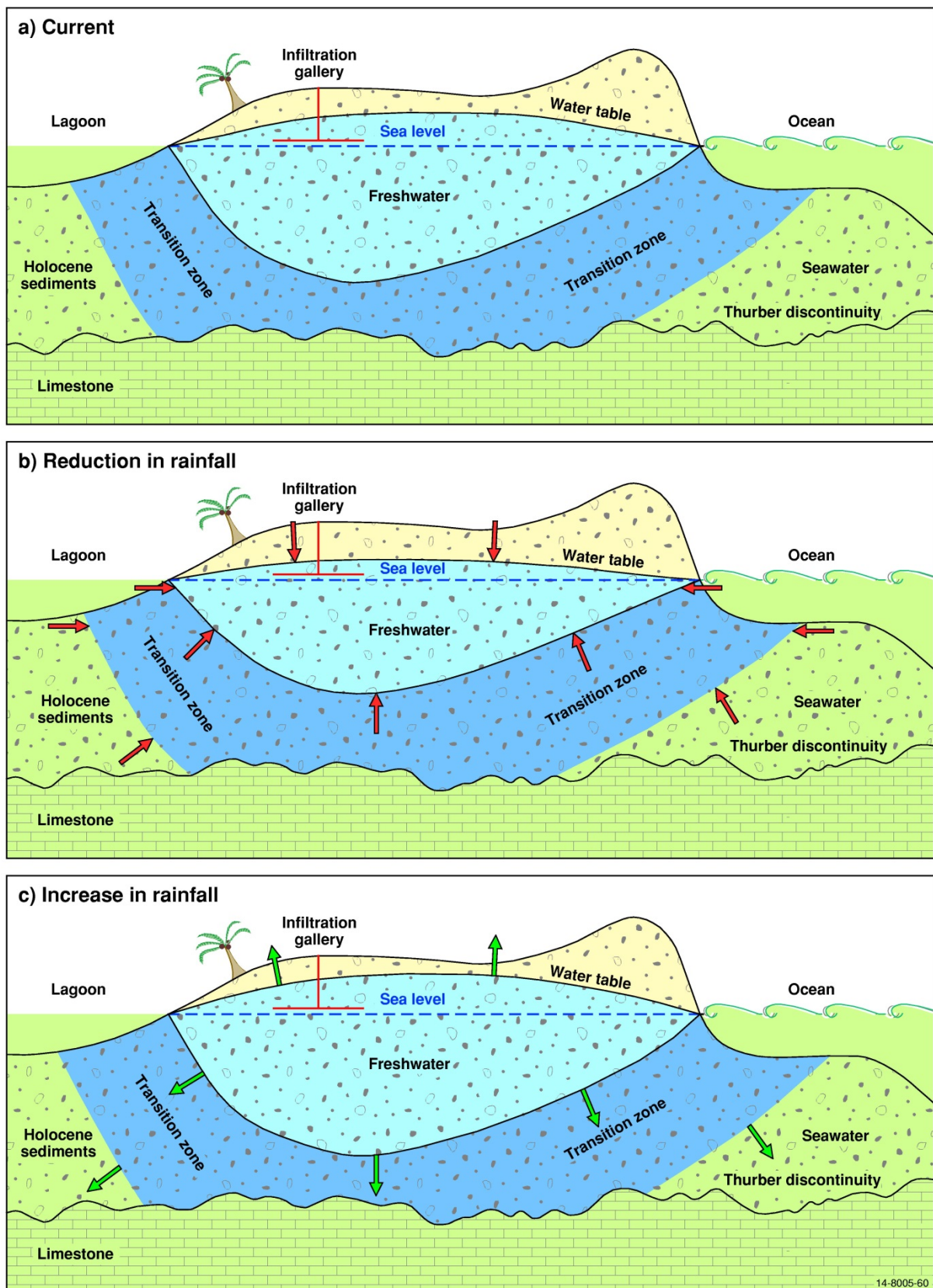
Appendix Figure E.1 Potential effect of b) reduction in rainfall or c) increase in rainfall on the freshwater lens of a Low Carbonate island compared to the a) current situation. Red arrows indicate a reduction in the size of the lens and green arrows indicate an increase in the size of the lens.
