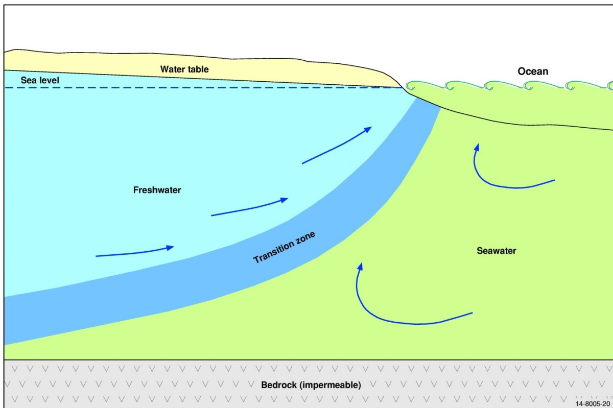
Figure 3.2 Schematic of the transition zone between freshwater and seawater in coastal aquifers (modified from Barlow 2003).
