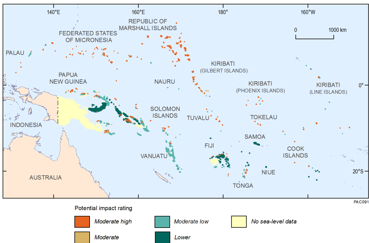
Figure 5.3 Potential impact of a rise in relative mean sea level in 2050.
