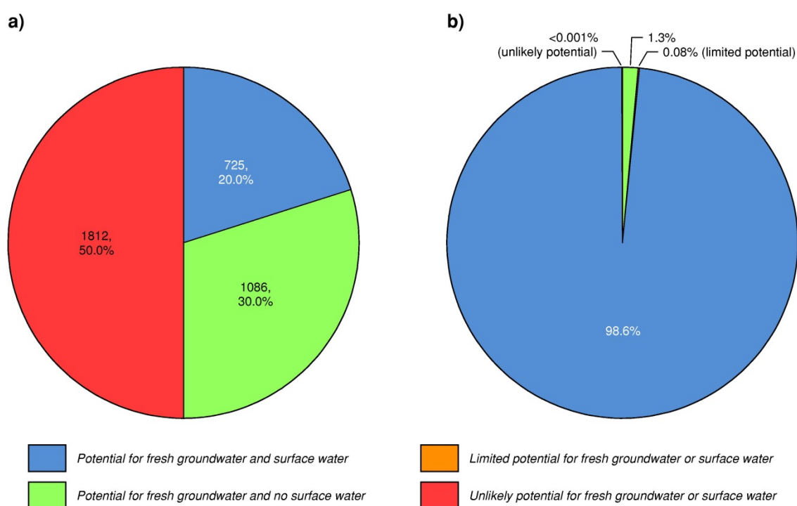
Figure 3.21 Number and percentage of islands of known types with and without potential for fresh groundwater and surface water across the Pacific region: a) island numbers and percentages of total islands; b) percentage of total island area.
