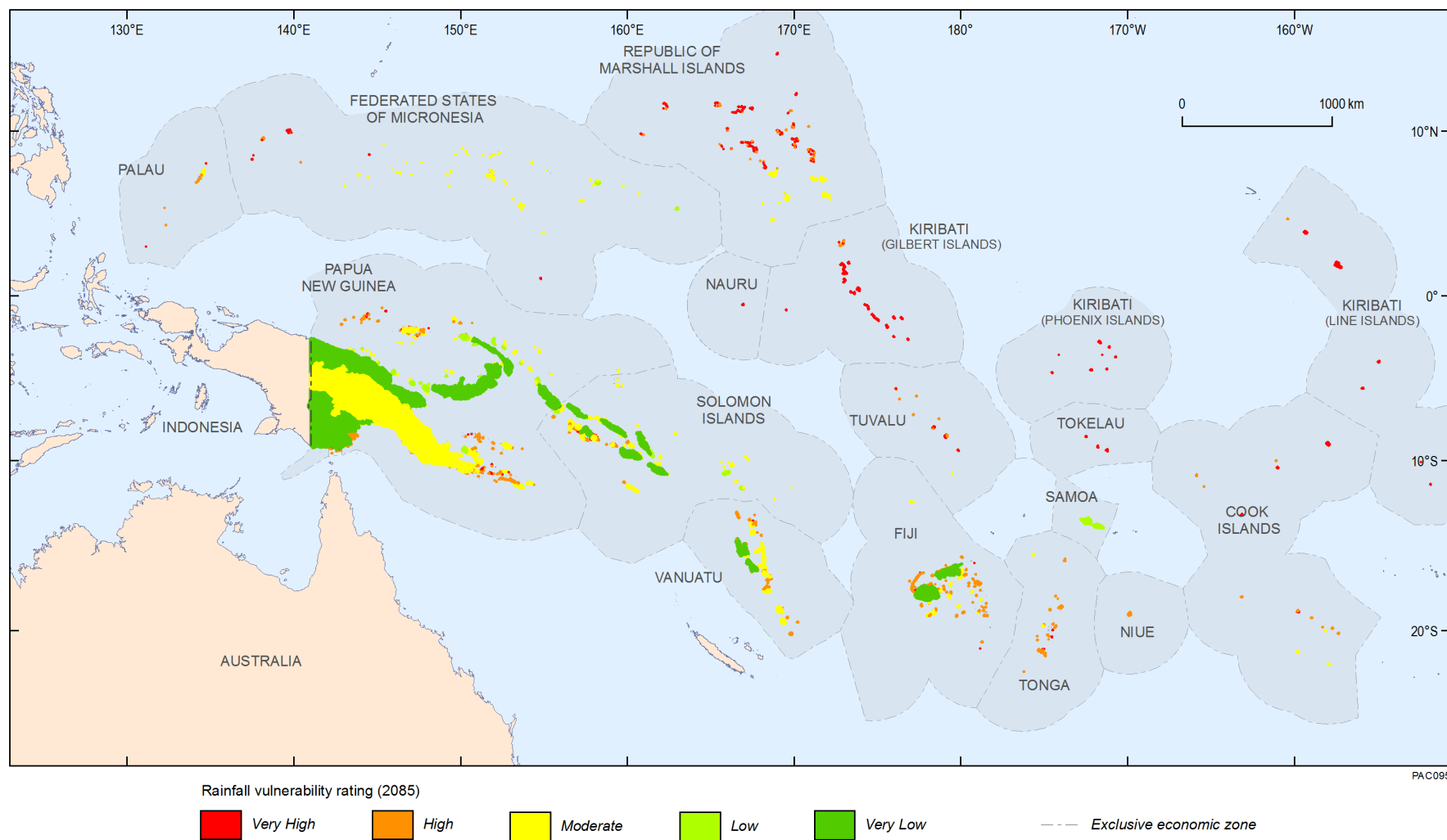
Figure 7.3 Regional map of potential vulnerability of groundwater systems on islands of the Pacific region to lowest mean annual rainfall in 2085.
