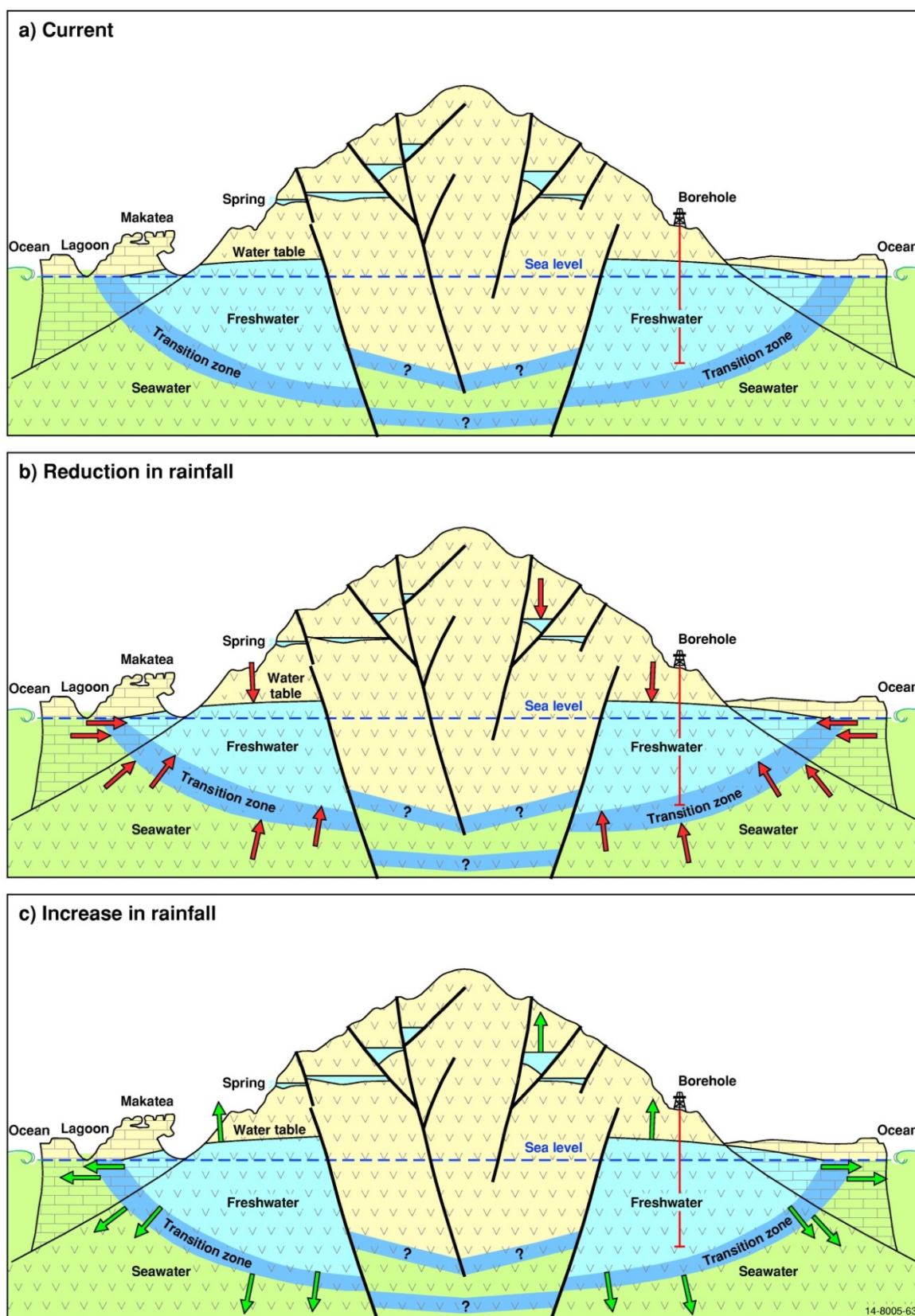
Appendix Figure E.4 Potential effect of b) reduction in rainfall or c) increase in rainfall on the aquifers of a Composite island compared to the a) current situation (modified from Waterhouse 1984). The question marks indicate that there may be connectivity from the basal aquifer across the dikes. Red arrows indicate a reduction in the size of the lens and green arrows indicate an increase in the size of the lens.
