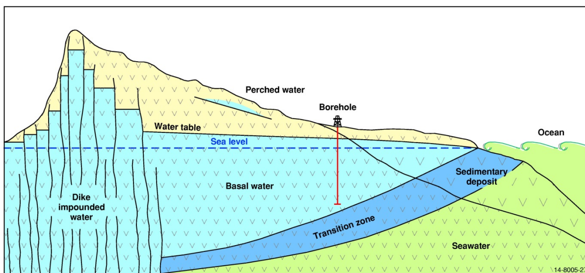
Figure 3.13 Main features of the aquifer system on a typical young basaltic Volcanic island (modified from UNESCO 1991).
