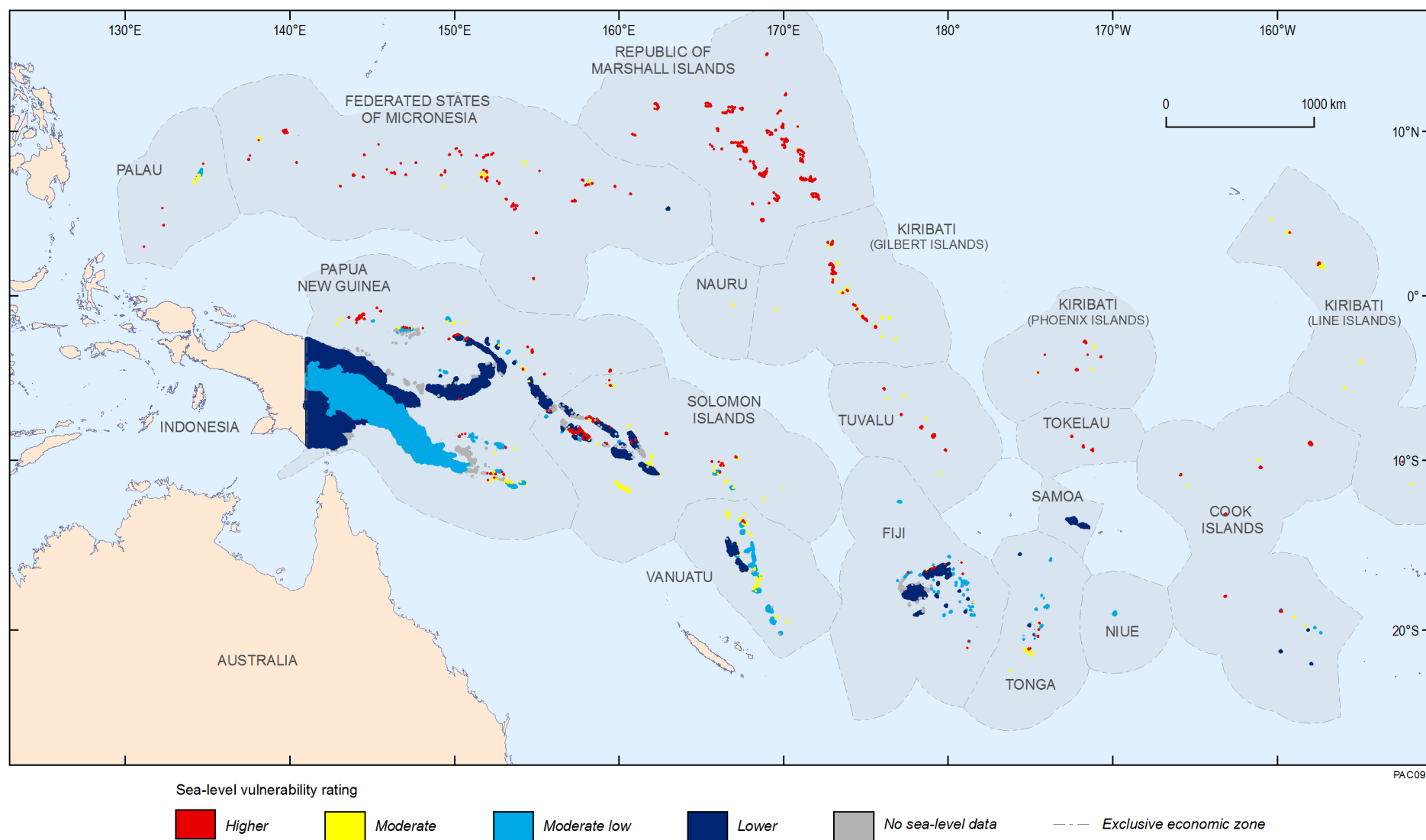
Figure 7.5 Regional map of relative potential vulnerability of groundwater systems on islands of the Pacific region to a rise in relative mean sea level in 2085.
