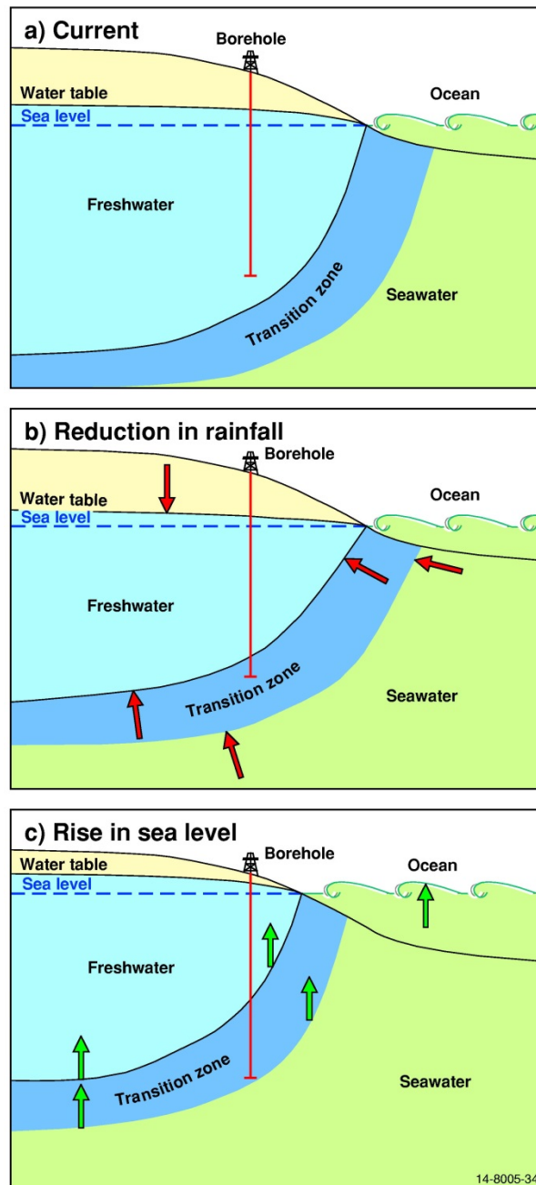
Figure 3.20 Potential effect of b) reduction in rainfall or c) rise in sea level on coastal aquifers of a Complex island compared to the a) current situation.
