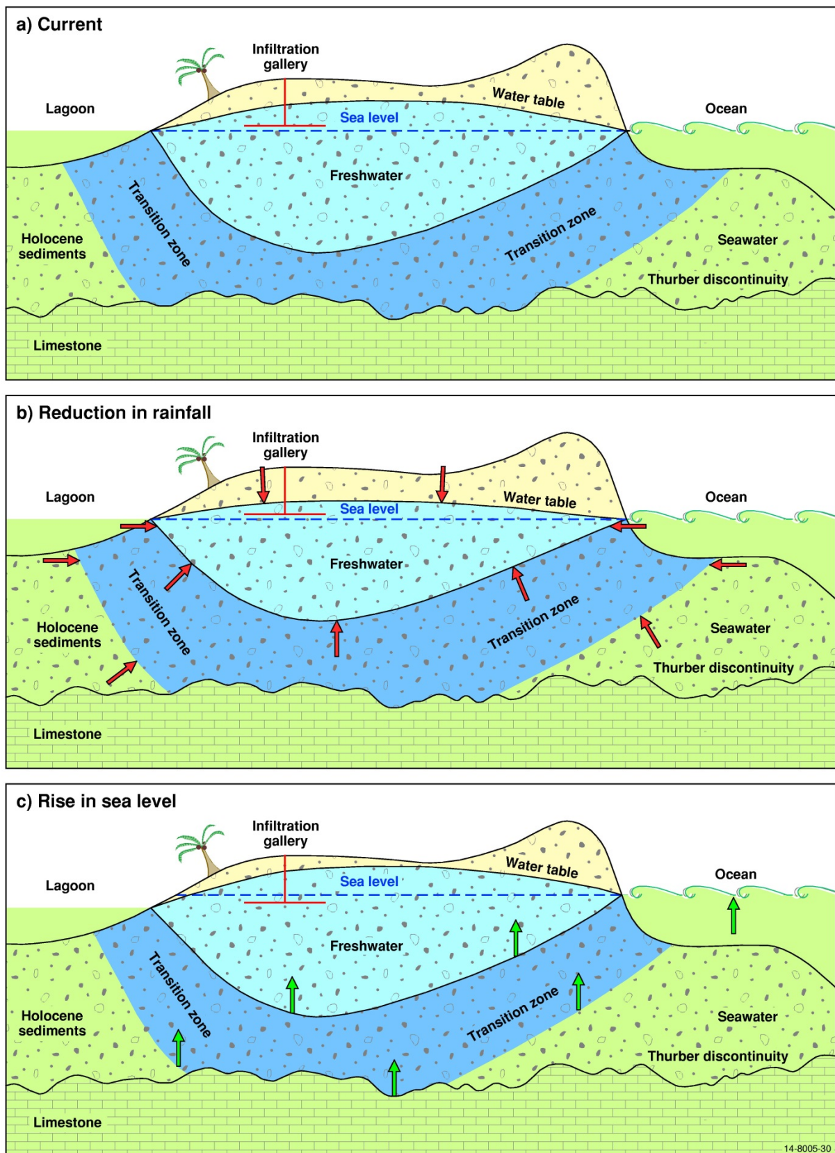
Figure 3.6 Potential effect of b) reduction in rainfall or c) rise in sea level on the freshwater lens of a Low Carbonate island compared to the a) current situation.
