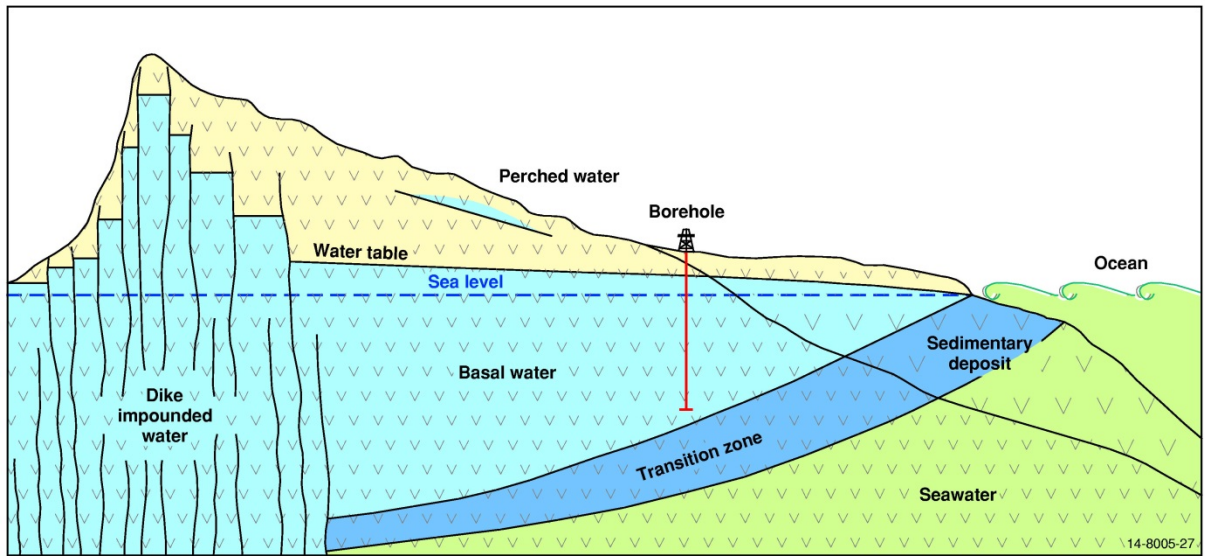
Appendix Figure D.6 Main features of the aquifer system on a typical young basaltic Volcanic island (modified from UNESCO 1991).
