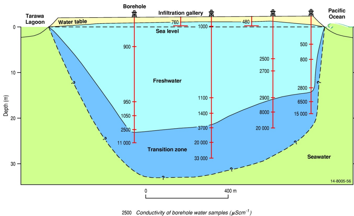
Appendix Figure D.2 Conceptual hydrogeological model for the freshwater lens on Bonriki island (Marshall and Jacobson 1985).
