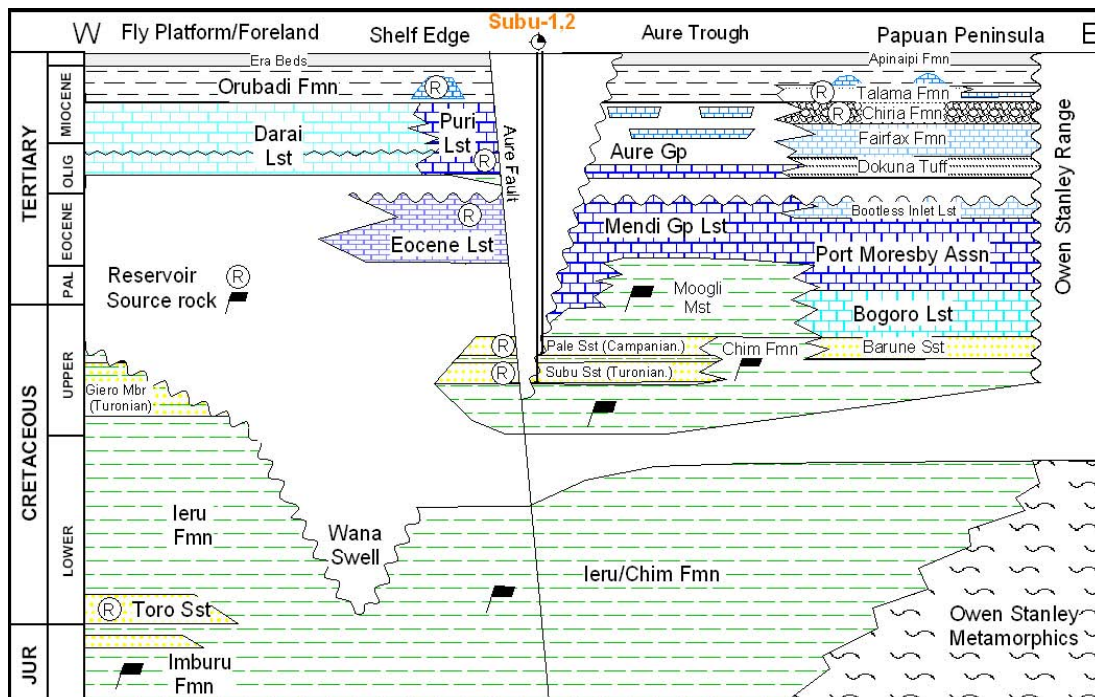
Figure 2. Stratigraphic chart, Eastern Papuan Basin and Papuan Peninsula. Note that source rocks are indicated with flag symbols whilst potential reservoirs intervals are shown with an ® symbol.
