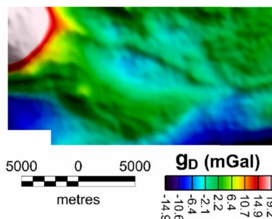
Figure 2. The conformed Falcon gravity product for location 1.
