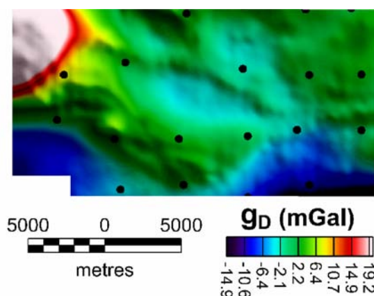
Figure 1. Reference gravity for location 1. Positions of the simulated regional data are shown as dots.
