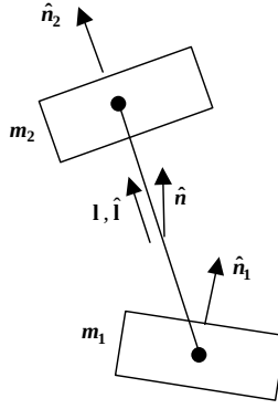
Figure 1. Schematic of in-line gravity gradiometer.
