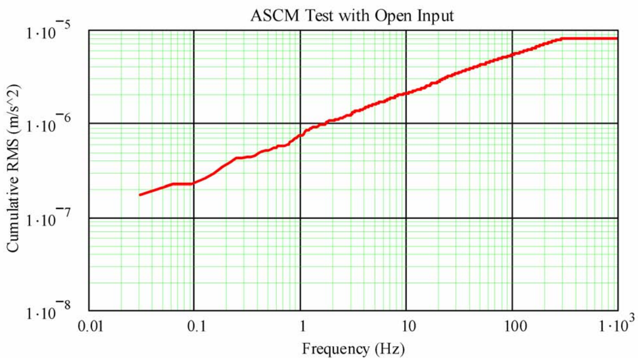
Figure 7. Cumulative rms noise in the gravimeter signal conditioning module.
