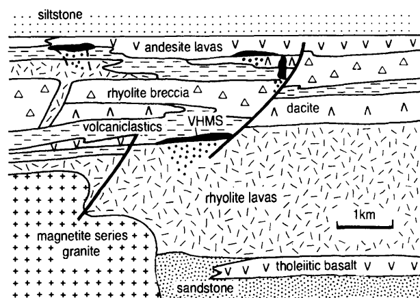
Figure 2. Regional schematic (based on Mt Windsor Province, Queensland).
