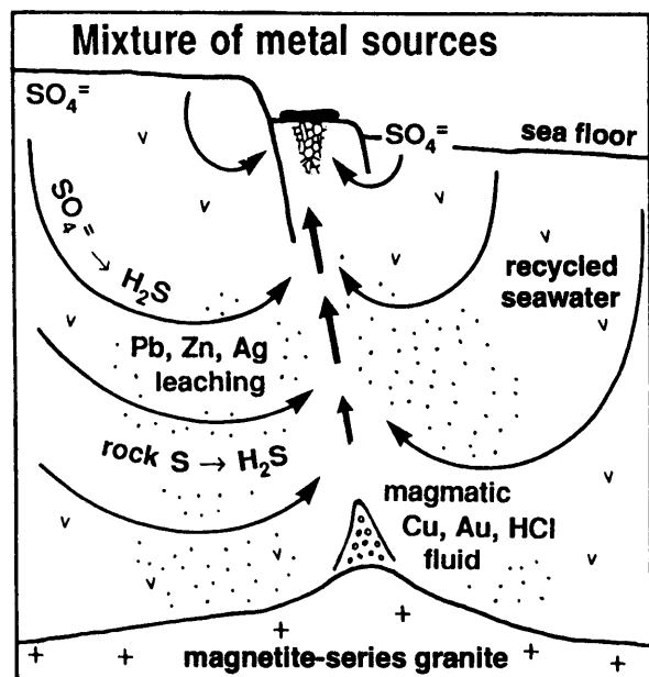
Figure 3. Possible sources of metals for VHMS deposits.
