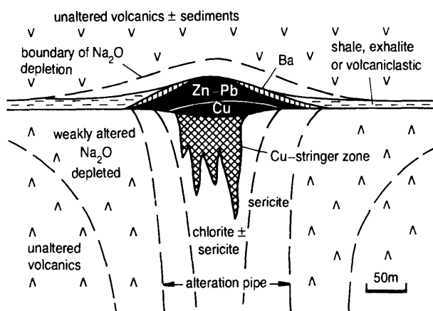
Figure 1. Cross-section of typical mound-style deposit.
