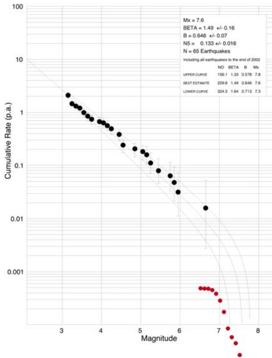
Figure 2 The cumulative recurrence rate of earthquakes in the SWSZ (black) from the GA catalogue and the SW WA neotectonics catalogue (red). The neotectonic catalogue has been scaled for time and area to match the earthquake catalogue.
