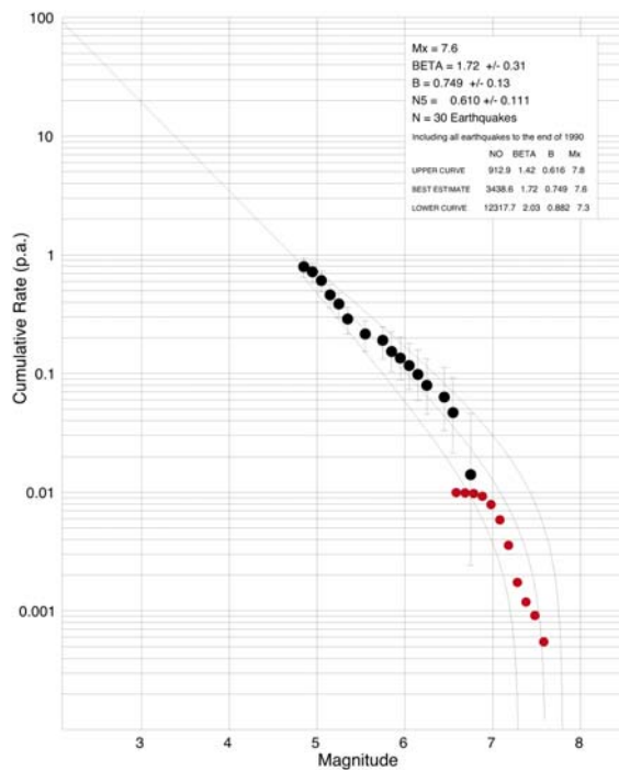
Figure 3 The recurrence rate for the Australian shield, from the world-wide CSS catalogue, and the scaled neotectonic catalogue.
