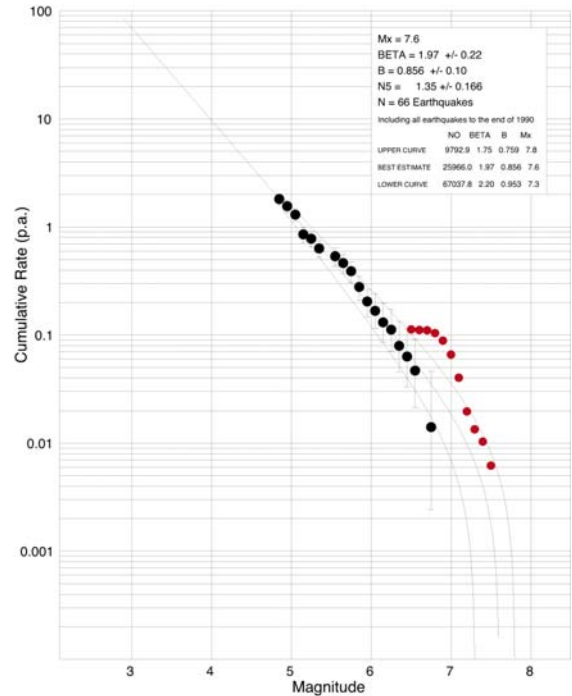
Figure 5 The recurrence rate for the world-wide SCC catalogue and the scaled neotectonic catalogue
