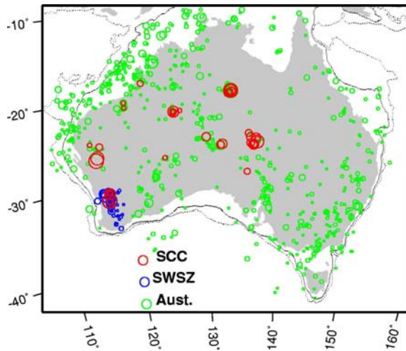
Figure 1 The three catalogues of Australian earthquakes used in this study. The green and blue data are from the GA catalogue and the red data is from the GSC Stable Continental Crust (SCC) database. The two isobaths are at 500m & 2500m.
