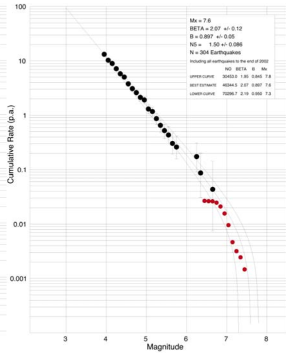
Figure 4 The recurrence rate for the Australian continent and the scaled neotectonic catalogue
