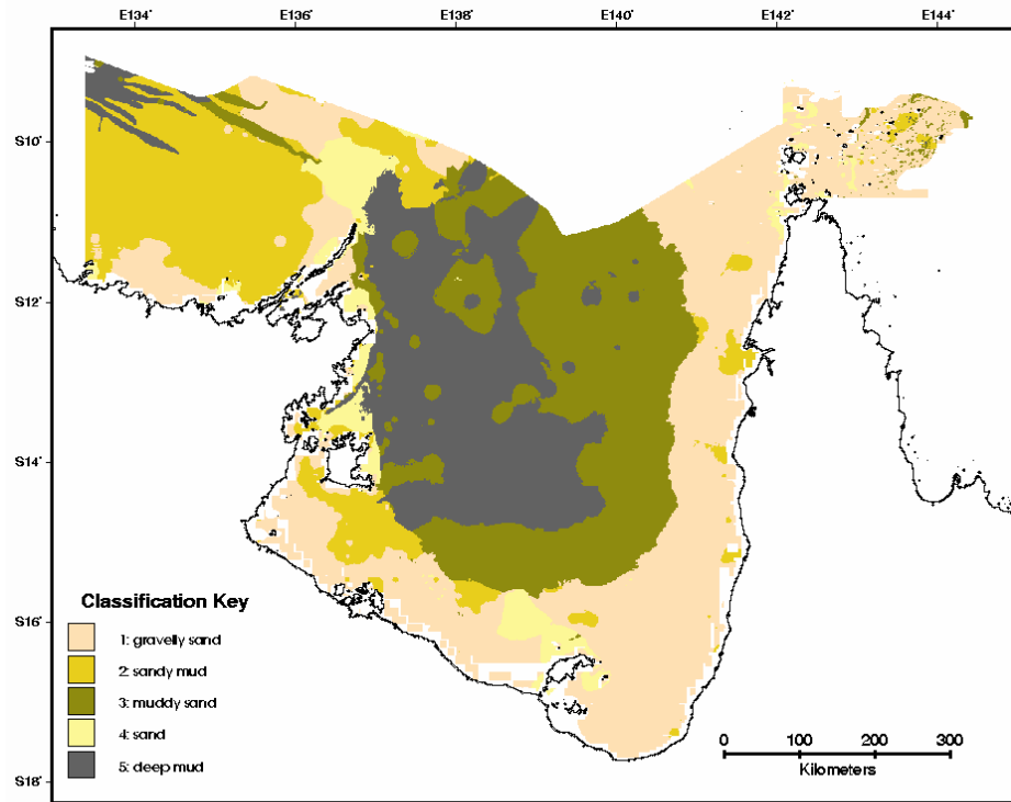
Figure 6.44. Run 2 – Seascape classification for the Northern Planning Area using 5 classes.
