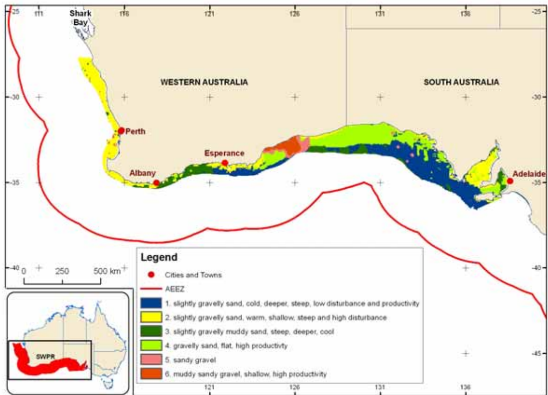
Figure 2.11. Seascape classification for the South West Planning Region (on-shelf zone) using 6 classes (Run 4SWPR – on-shelf).
