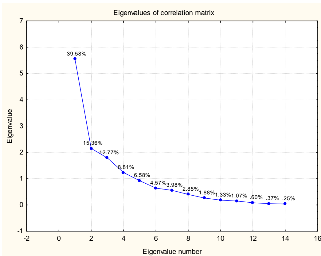
Figure 6.46. Run 3 – Eigenvalues of the correlation matrix for the Northern Planning Area (scree plot).
