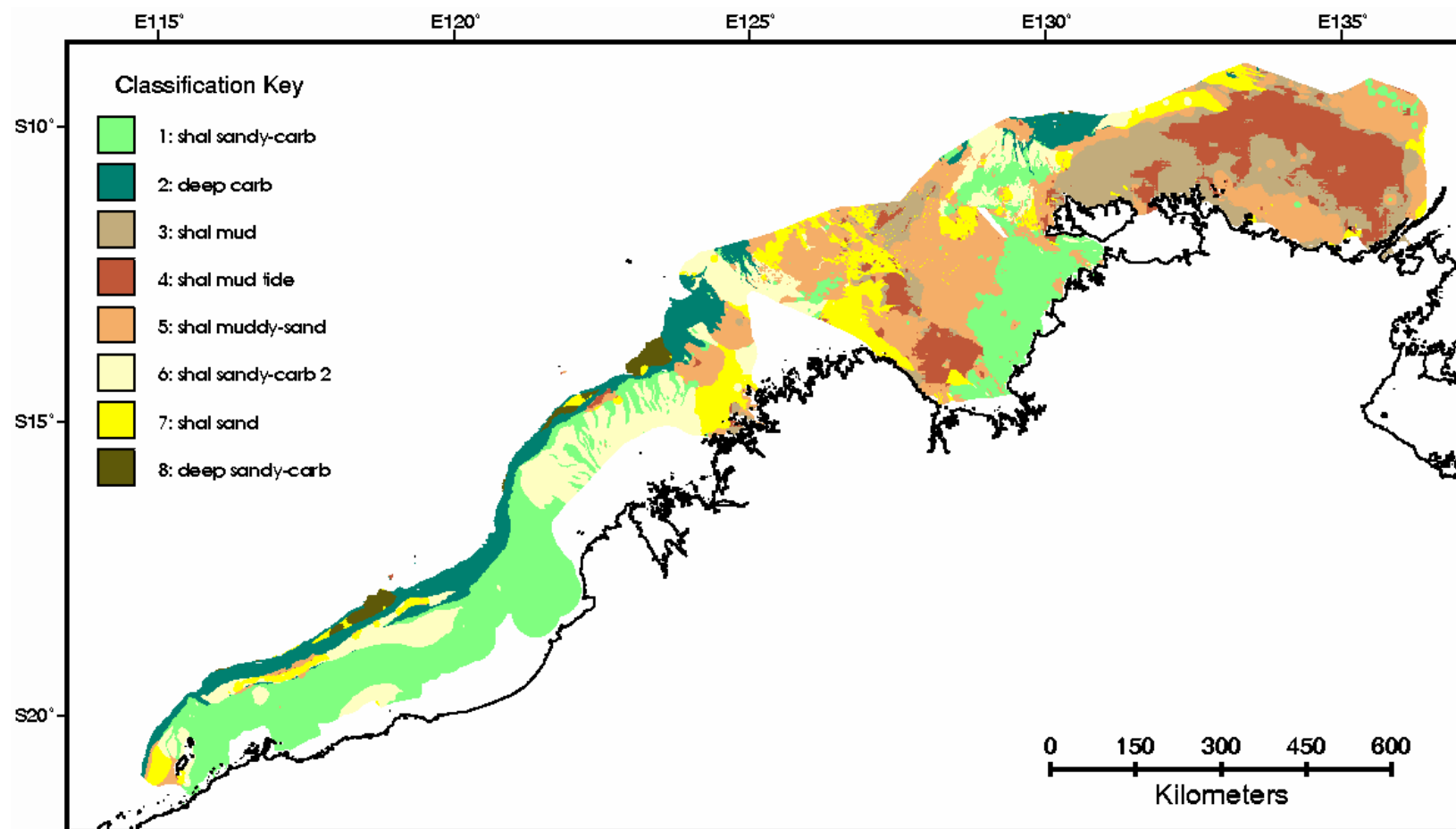
Figure 6.8 Seafloor classification for the North West area using 8 classes (run 1).
