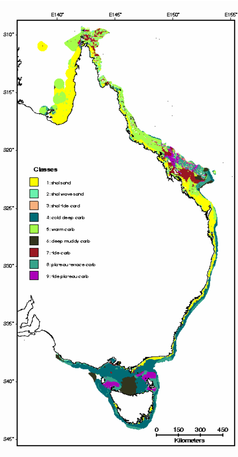
Figure 6.15. Seascape classification for East area using 9 classes (run 2).
