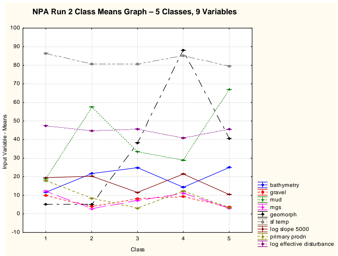
Figure 6.45. Run 2 – Class means for the Northern Planning Area.
