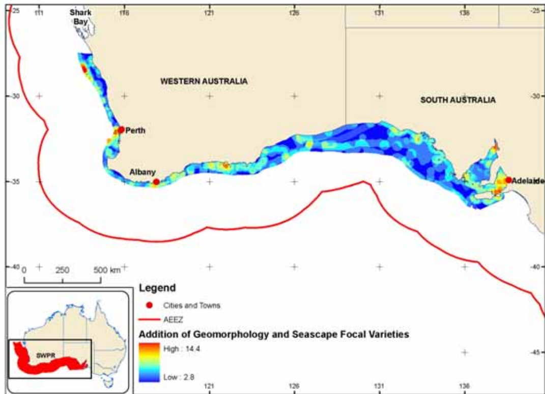
Figure 4.12. Combined geomorphology focal variety and seascape focal variety datasets (addition) in the South West Planning Region (on-shelf), showing areas of high combined habitat and geomorphic diversity in red and areas of combined low seascape and geomorphic diversity in blue.
