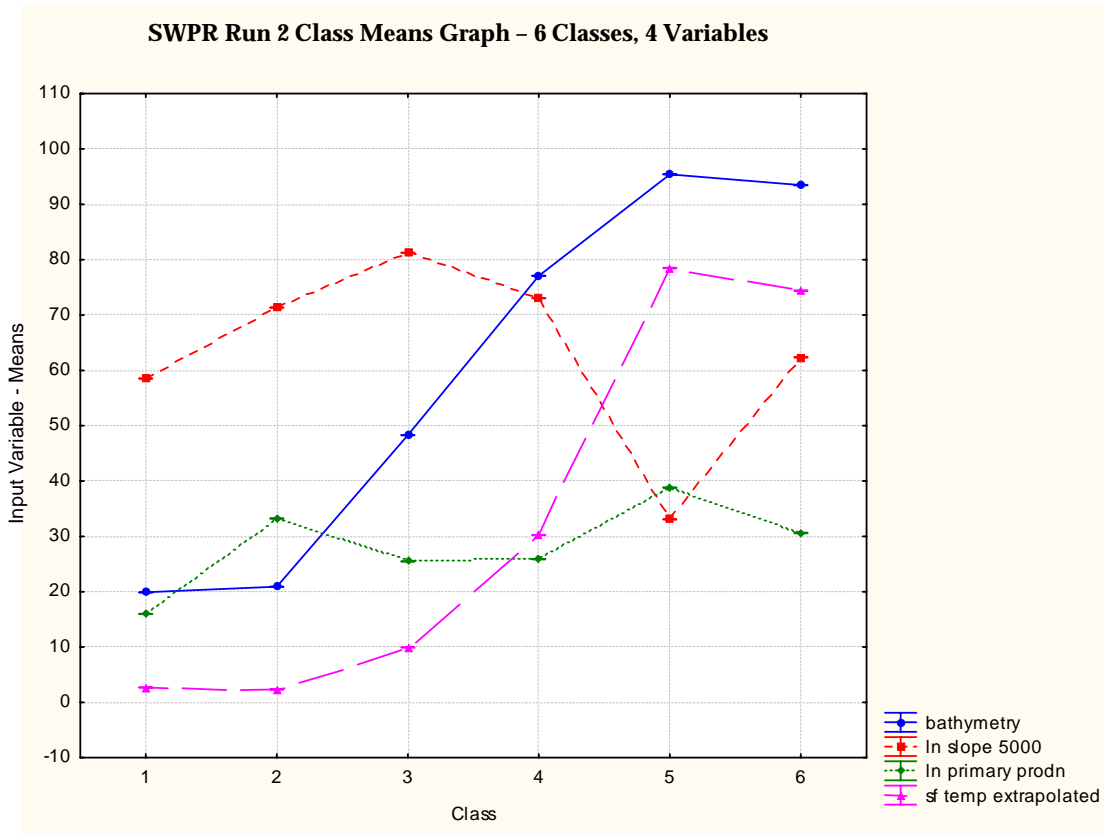
Figure 6.67. Class means for the South West Planning Region (sea floor temperature extrapolated).
