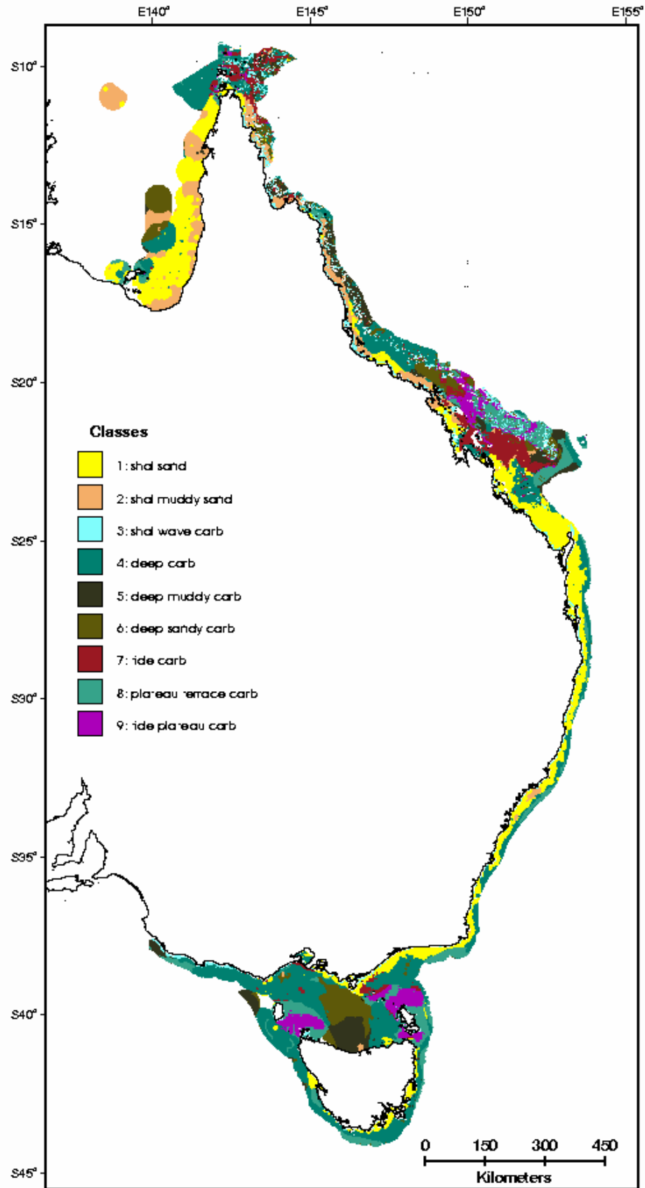
Figure 6.2. Seascape classification for the East area using 9 classes (run 1).
