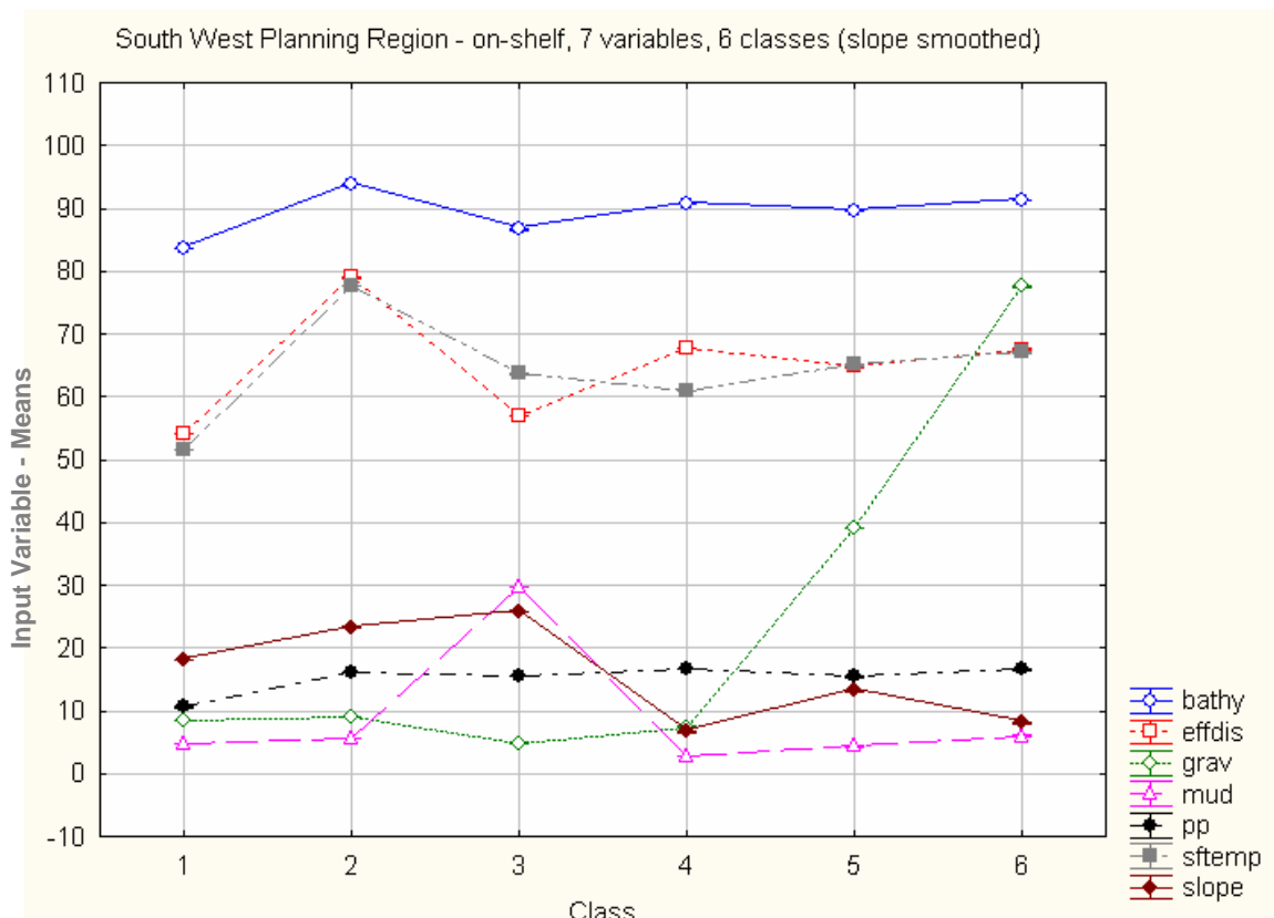
Figure 2.12. Class means for the South West Planning Region (Run 4SWPR – on-shelf).
