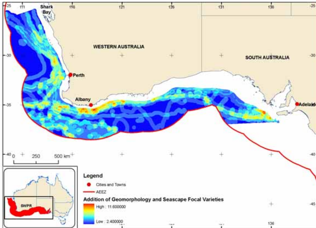
Figure 4.9. Combined geomorphology focal variety and seascape focal variety datasets (addition) in the South West Planning Region (off-shelf), showing areas of high combined habitat and geomorphic diversity in red and areas of combined low seascape and geomorphic diversity in blue.
