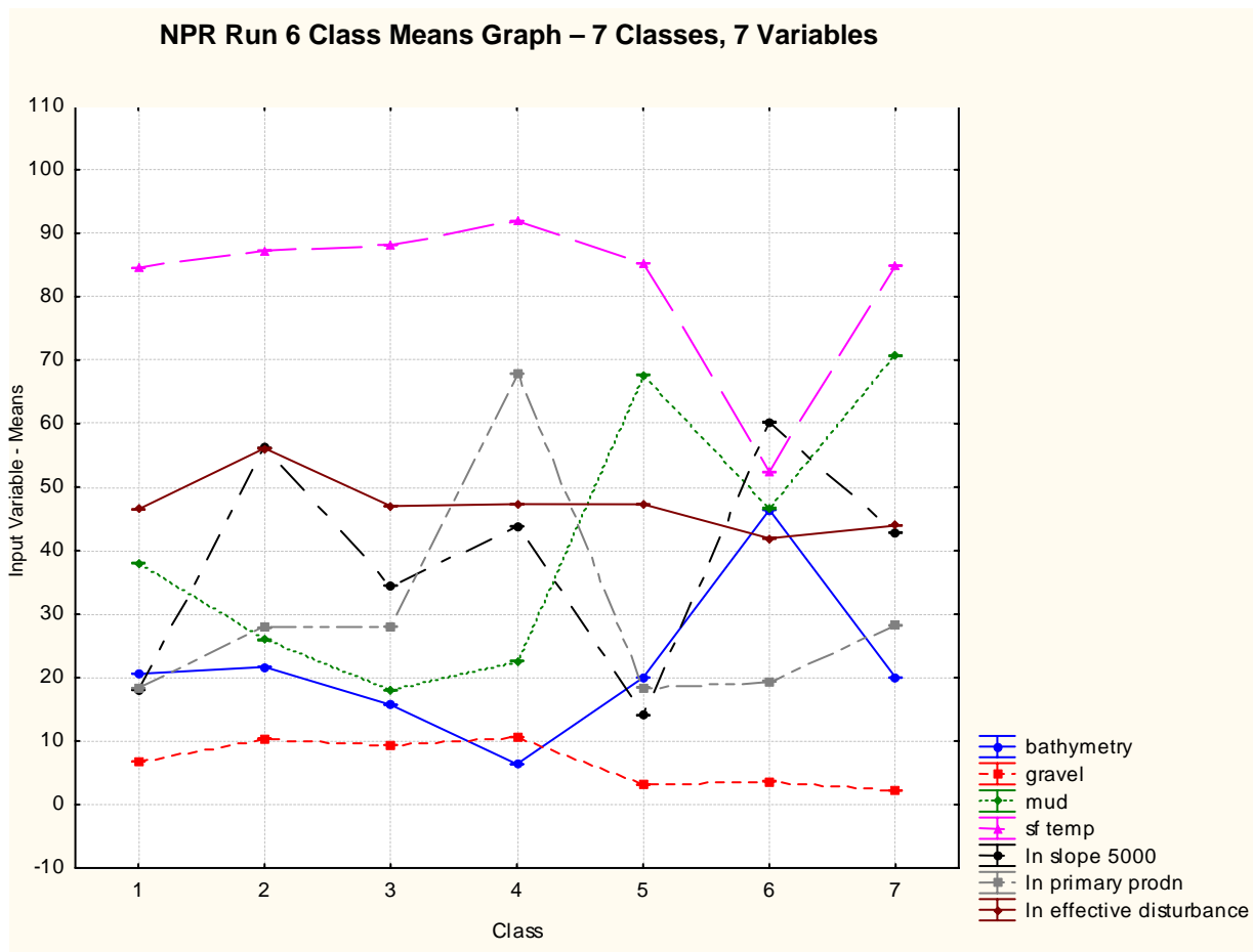
Figure 6.60. Run 6 – Class means for the Northern Planning Region.
