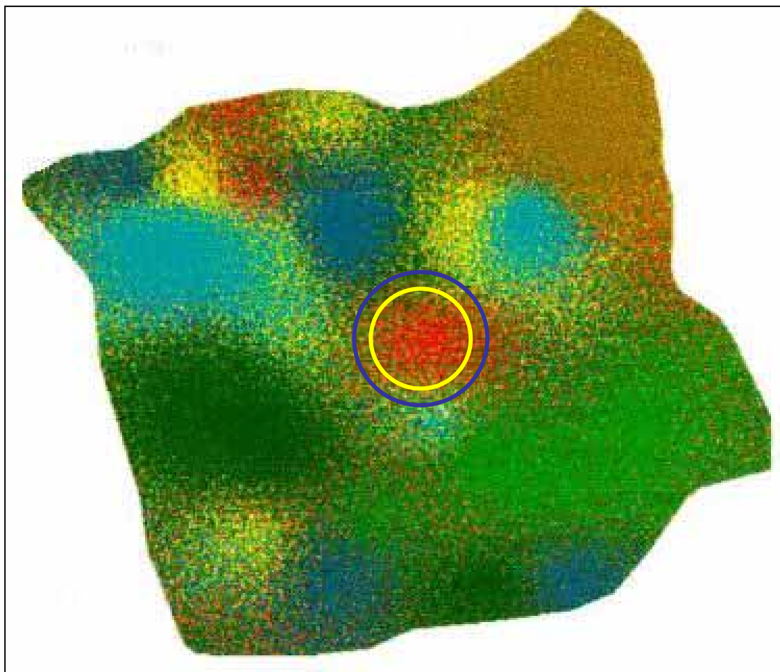
Figure 2.6. Map showing different definitions in cluster boundaries. In a fuzzy definition there is a gradient of membership so that one cell could belong to more than one class.
