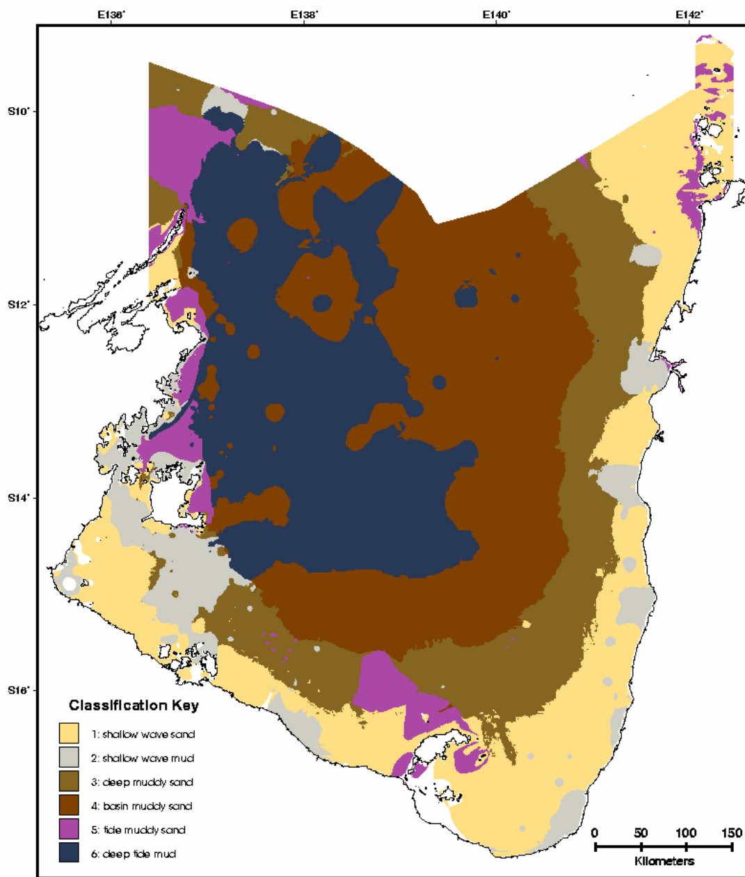
Figure 6.11. Seascape classification for the Gulf of Carpentaria using 6 classes (run 1).
