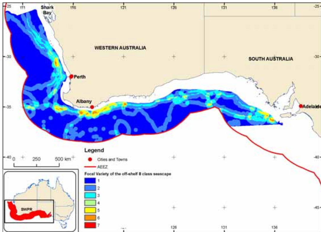
Figure 4.7. Focal variety analysis of seascape classification for the South West Planning Region (off-shelf), showing areas of high seascape diversity in red and areas of low seascape diversity in blue
