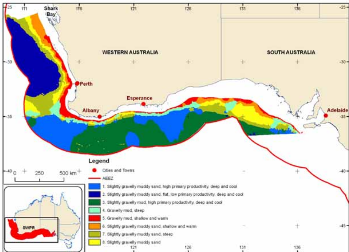
Figure 2.15. Seascape classification for the South West Planning Region (off-shelf zone) using 8 classes (Run 4SWPR – off-shelf).
