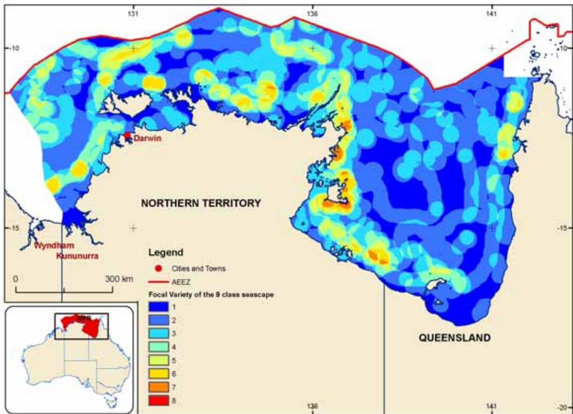
Figure 4.4. Focal variety analysis of seascape classification for the Northern Planning Region, showing areas of high seascape diversity in red and areas of low seascape diversity in blue.
