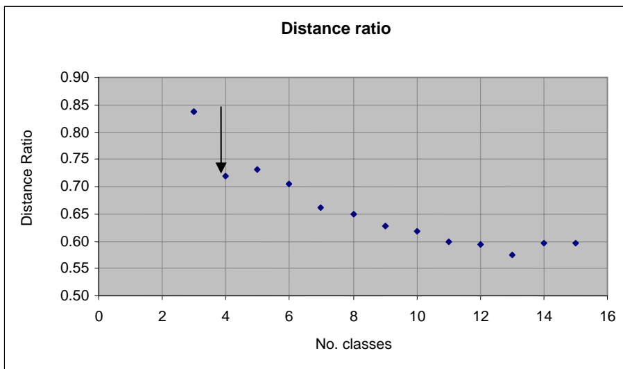
Figure 3.4. Distance ratio results for the unsupervised crisp methodology showing 4 classes as the optimal number of classes.
