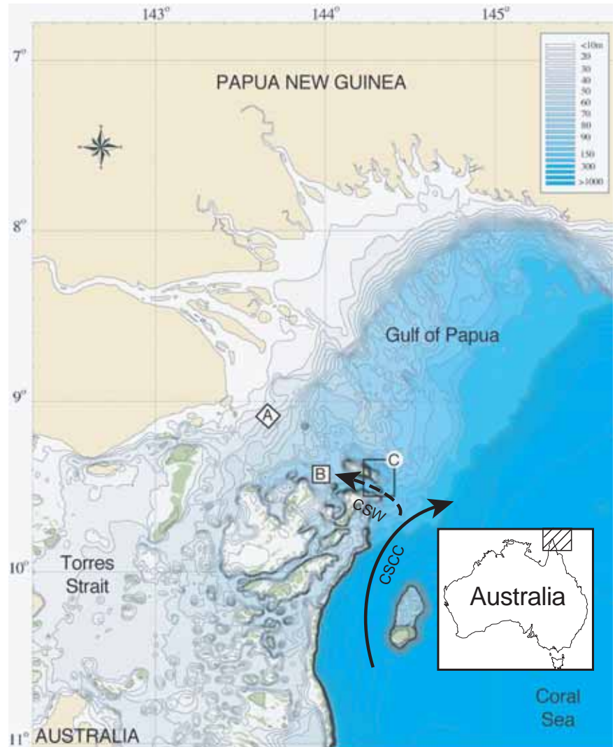
Figure 1. Regional bathymetric map of the Gulf of Papua, Torres Strait and northern Great Barrier Reef based upon a new compilation of digital data provided by the CSIRO Division of Marine Research and the Royal Australian Navy Hydrographic Office. Reefs are shaded green. Boxes show the location of surveys in Areas A and B reported in this paper from Geoscience Australia Survey 234 (Harris et al. , 2002). CSCC, Coral Sea Coastal Current; CSW, upwelling Coral Sea water.
