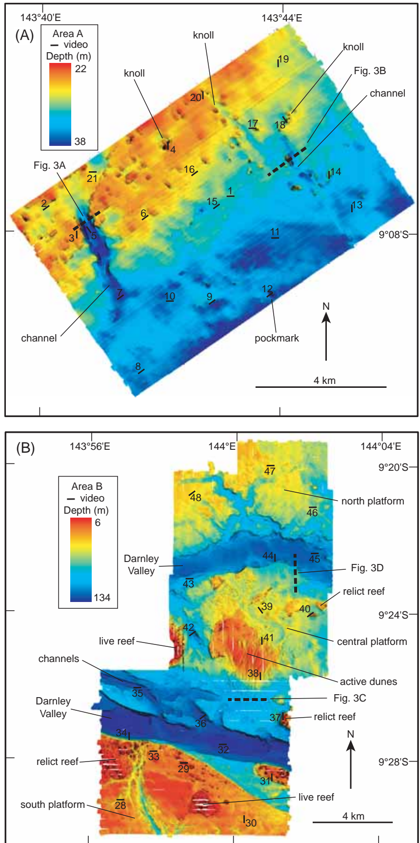
Figure 2. Sun-shaded bathymetric maps of the survey areas. (A) Area A on the Fly River distal-delta. Note the shallow channels aligned normal to the isobaths and the numerous low-relief knolls. (B) Area B on the northern Great Barrier Reef shelf. Note the presence of deep submarine valleys as two limbs of the Darnley Valley separated around a live reef in the west-central platform. Numbers refer to the video transect stations. Dashed lines refer to the positions of sub-bottom profiles in Figure 3.
