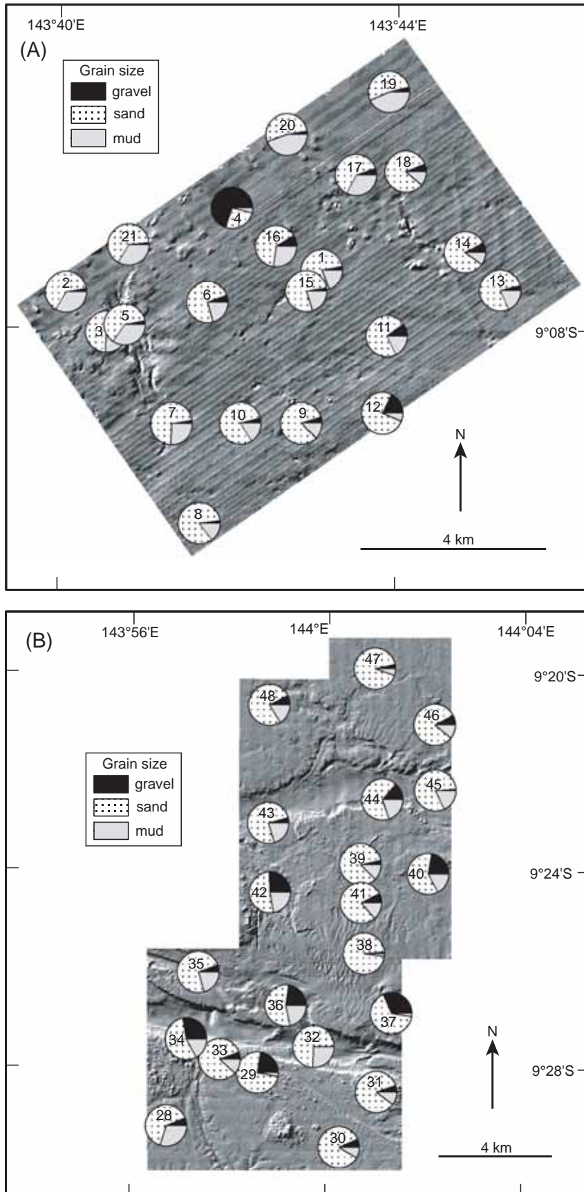
Figure 5. Gravel, sand and mud weight proportions from grab samples. (A) Area A. (B) Area B. Numbers refer to station numbers in Tables 3 and 4. There is a pattern of higher gravel proportions in samples obtained from low-relief limestone and pockmarks in Area A; and relict reefs, valley sides and channels in Area B.
