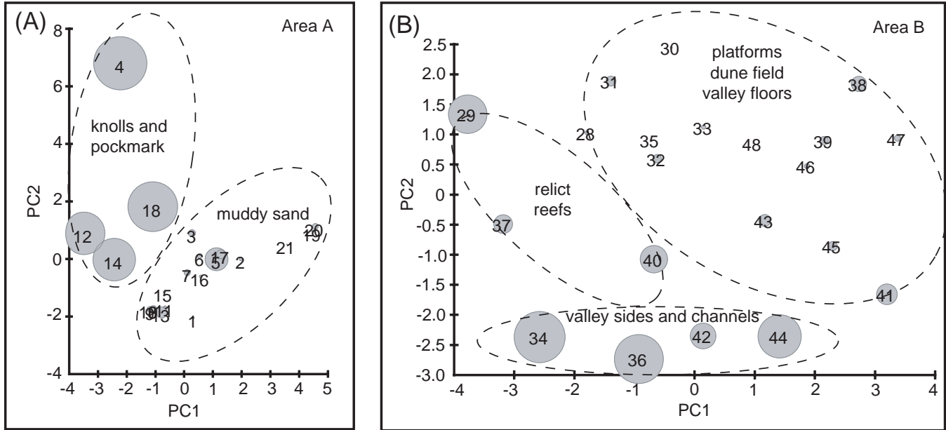
Figure 6. Ordination plots of PCA using Euclidean distance on Table 3 and Table 4 environmental data, showing circles of the relative size of slope at each station. (A) Area A variables are clustered into two groups: knolls and pockmarks; and muddy sand. (B) Area B variables are clustered into three groups: relict reefs; valley sides and channels; and platforms, dune field and valley floors.
