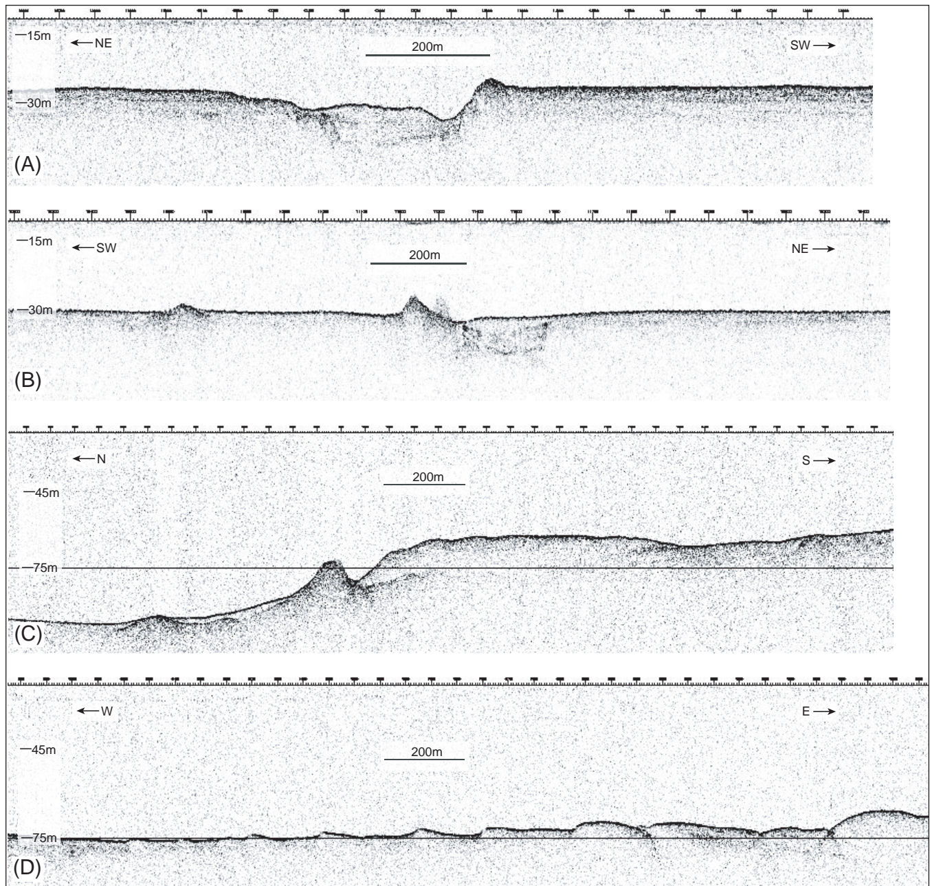
Figure 3. Example Chirp sub-bottom profiles. (A) Area A, showing an infilled channel. (B) Area A, showing sub-surface reflectors and infilled channel. (C) Area B, showing sub-surface reflectors on the margin of the north arm of the Darnley Valley. (D) Area B, showing an active dune field. See Figure 2 for locations.
