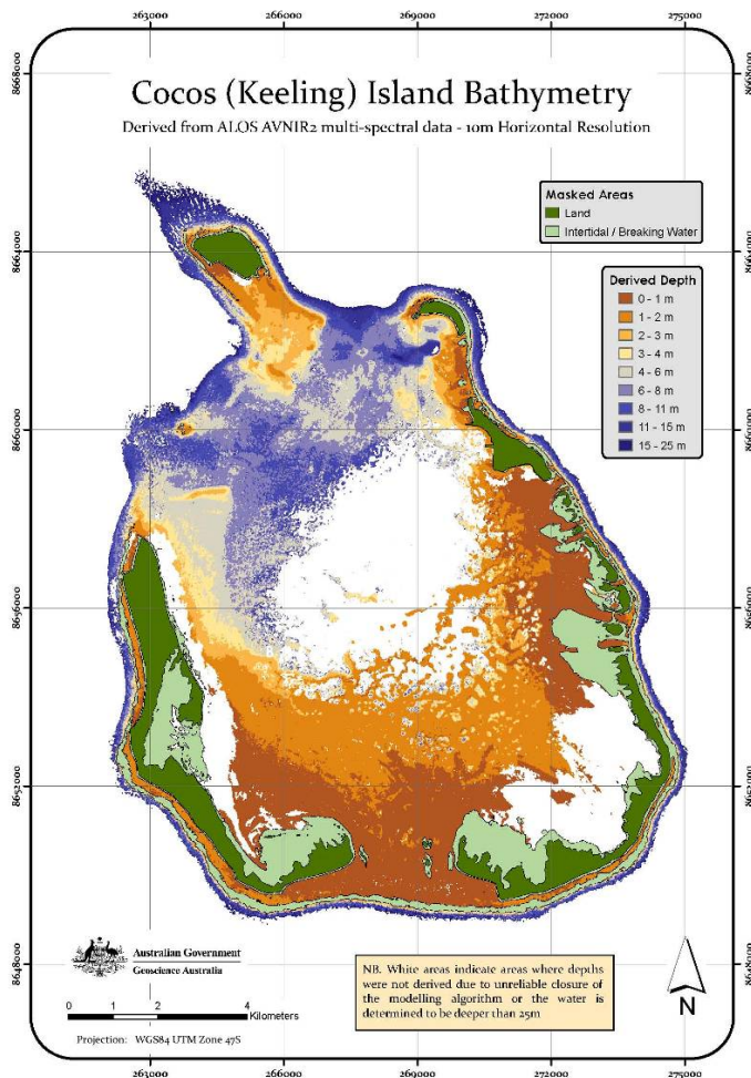
Figure 4-82. Cocos bathymetry
