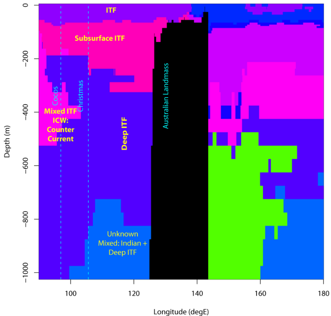
Figure 4-6. Cross-sectional profile of water mass types by longitude and depth down to 1000 m, taken at a latitude of 11.3^{\circ}\text{S} (intermediate between the latitudes of Christmas and Cocos (Keeling) Islands). The characterisation of water mass types is from the work of Lyne and Hayes (2005).
