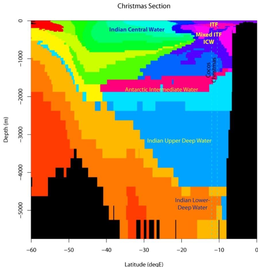
Figure 4-7. Cross-sectional profile of water mass types by latitude and depth, taken at a longitude of Christmas Island (105.6°E). The characterisation of water mass types is from the work of Lyne and Hayes (2005).
