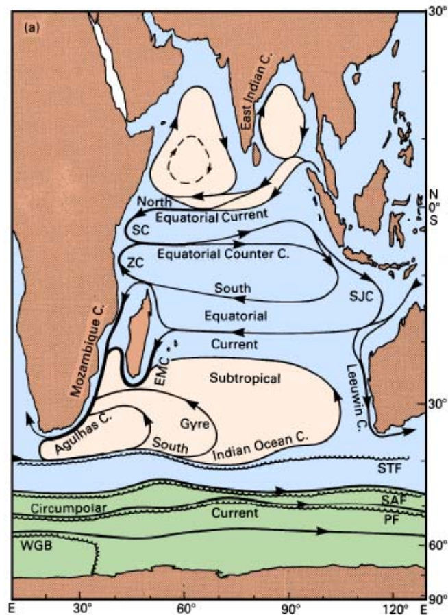
Figure 4-1. Tomczak and Godfrey's (2005) depiction of the surface currents in the Indian Ocean during the Northeast Monsoon (March-April) (after Tomczak and Godfrey, 2005).
