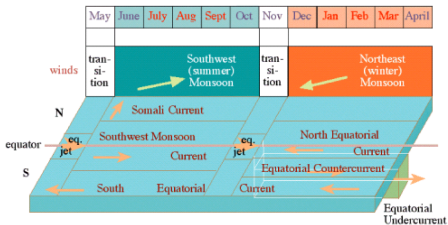
Figure 4-2. Tomczak and Godfrey's (2005) depiction of the monsoon system in the Indian Ocean. The top part indicates the wind cycle for the northern hemisphere, the lower part shows the major currents that develop in response to the wind for both hemispheres (after Tomczak and Godfrey, 2005). Southern hemisphere wind patterns are depicted in Figure 4-3.
