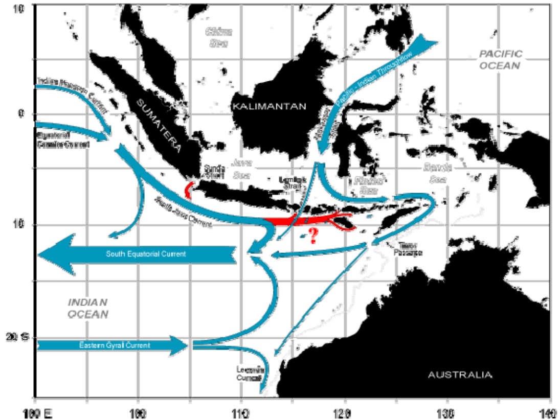
Figure 4-4. Schematic of the current system associated with the Indonesian Throughflow (see the article by Theresa K. Chereskin: http://tryfan.ucsd.edu/woce_ioe/woce_ioe.htm ).
