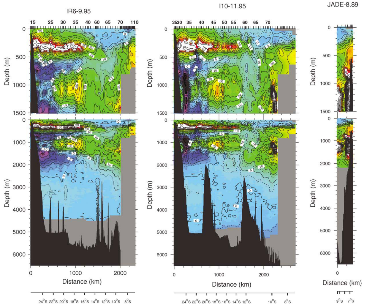
Figure b). Sections of normalised salinity anomaly from Wijffels et al. , (2002), along transects shown in Figure a).
