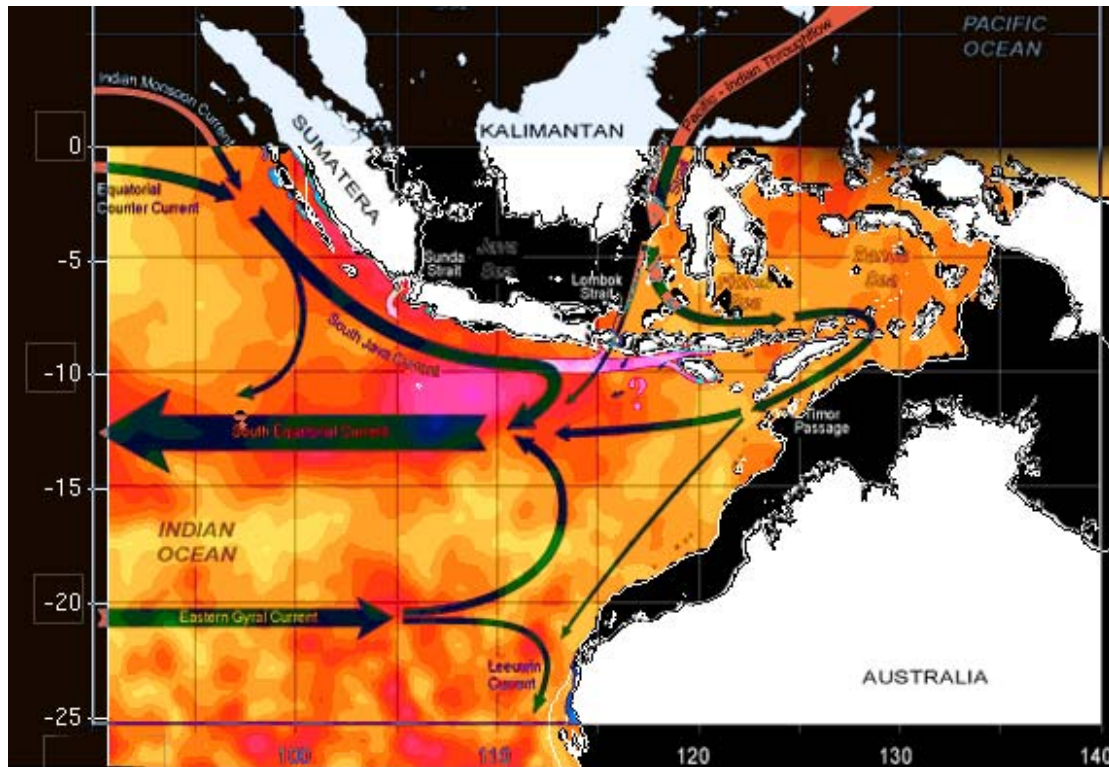
Figure 4-12. A montage overlay which attempts to depict the correspondence between the currents in the eastern Indian Ocean (see above) with the altimeter sea-surface height anomaly for the month of September (image from the work of Hayes et al (2005)). Pink represents high variance in sea-surface height and light orange, low variance.
