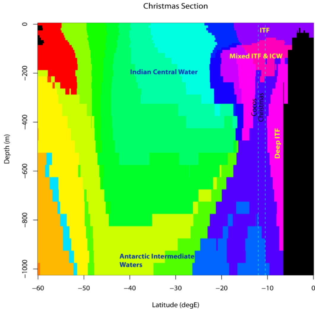
Figure 4-8. Cross-sectional profile of water mass types by latitude and depth down to 1000 m, taken at a longitude of Christmas Island (105.6°E). The characterisation of water mass types is from the work of Lyne and Hayes (2005).
