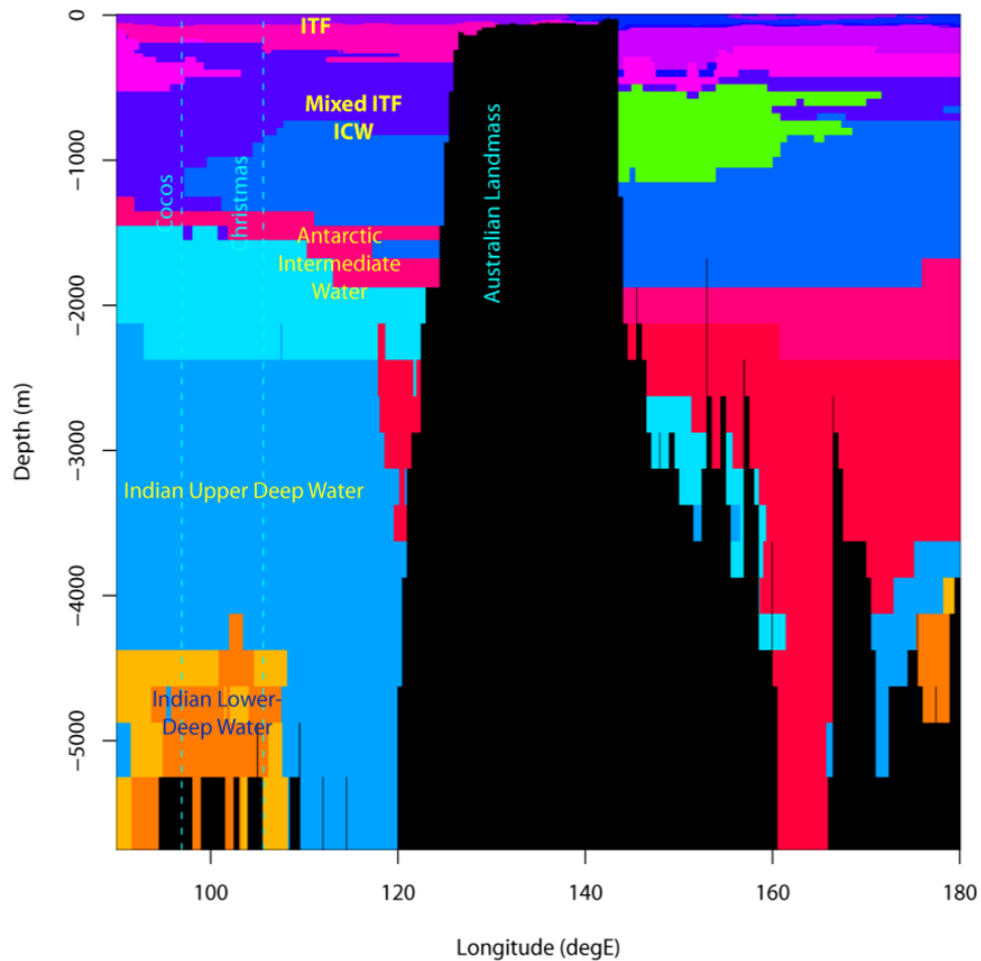
Figure 4-5. Cross-sectional profile of water mass types by longitude and depth, taken at a latitude of 11.3°S (intermediate between the latitudes of Cocos (Keeling) and Christmas Islands). The characterisation of water mass types is from the work of Lyne and Hayes (2005).
