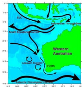
Figure 8 – Regional Circulation in the East Indian Ocean. Source: CSIRO
