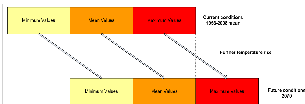
Figure 3 – Shift in the temperature pattern
