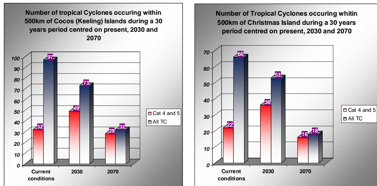
Figure 7 – Projections of the Number of Tropical Cyclones for the IOT
