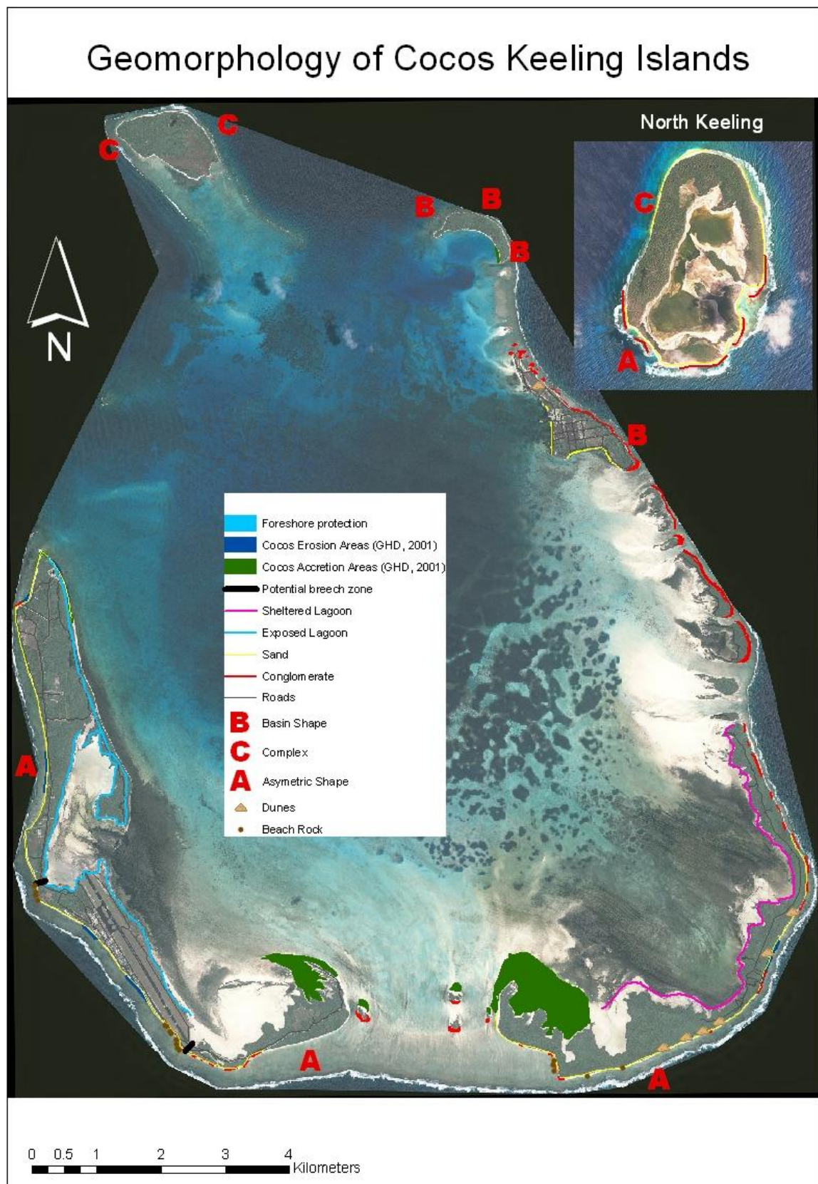
Figure 11 – Geomorphology of Cocos (Keeling) Islands
