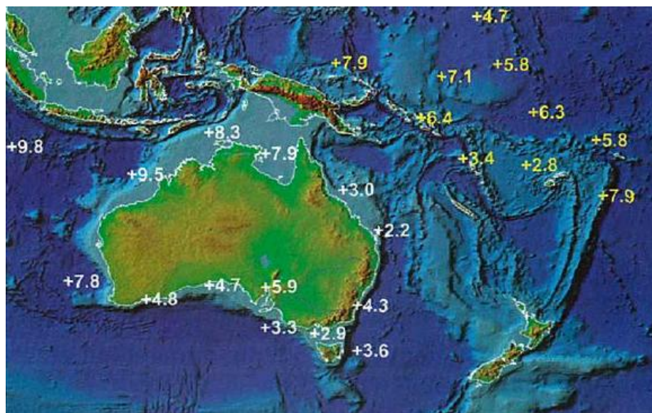
Figure 4 – Observed rate of relative mean sea level rise (mm per year, with the vertical motion of the gauge with respect to the land excluded) over the 1992 – 2007 period. Source: BoM/CSIRO 2007
