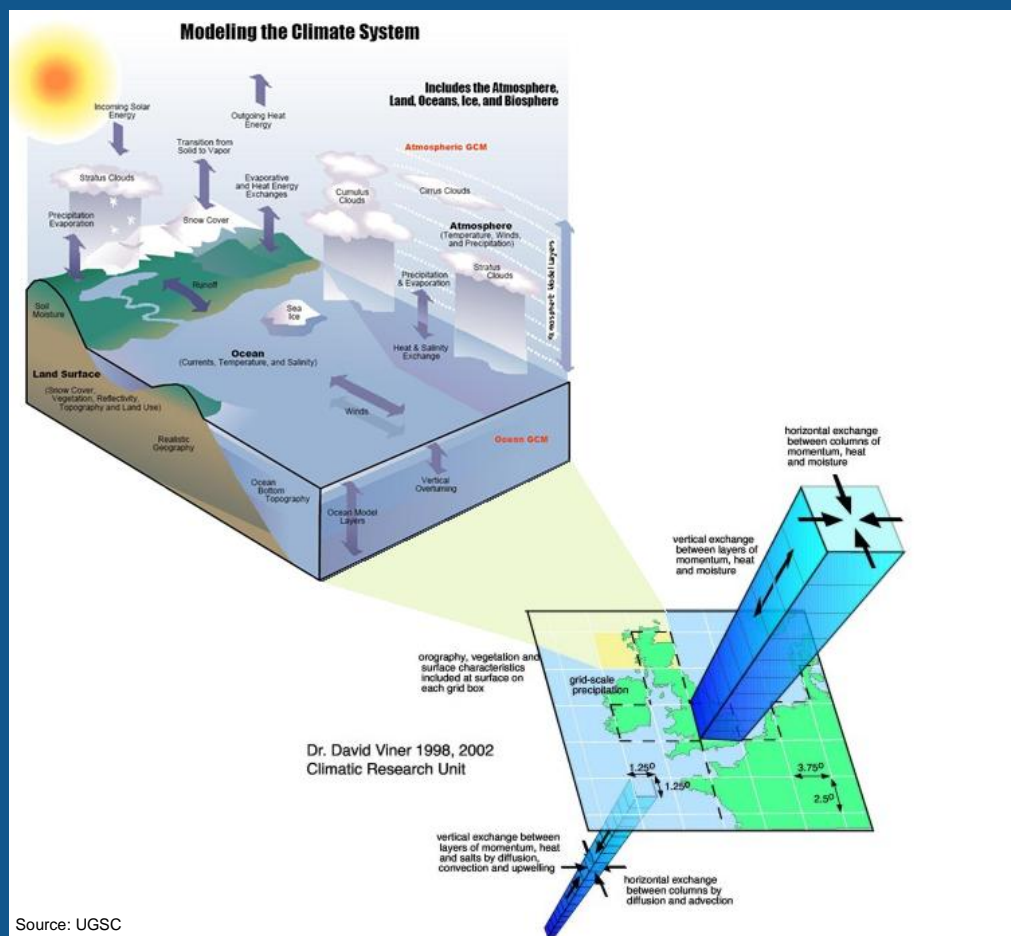
Figure 2 General Circulation Model Scheme
