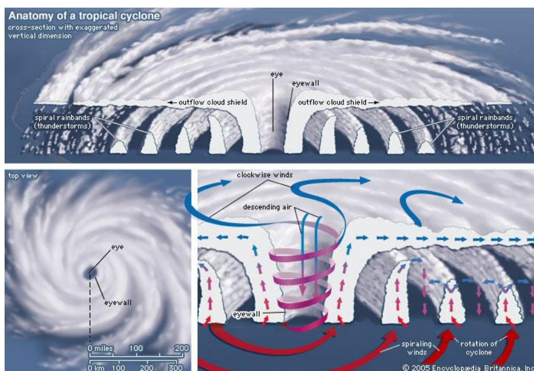
Figure 6 – Detailed representation of a tropical cyclone. Source: Encyclopaedia Britannica.
