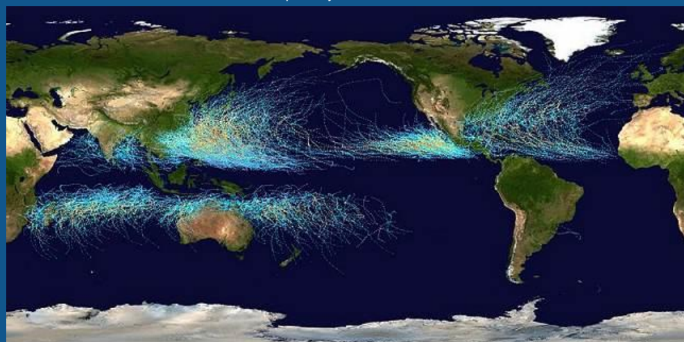
Global tropical cyclones tracks
