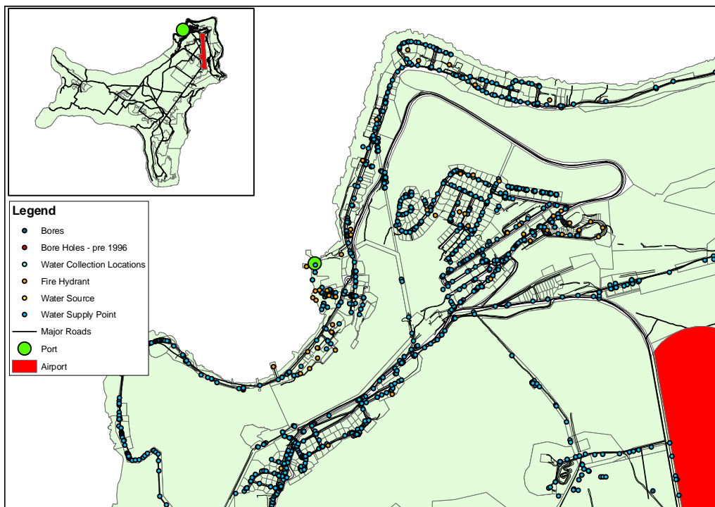
Figure 22 – Water Resource Infrastructure
