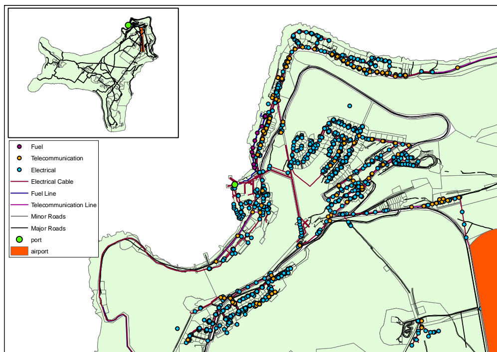
Figure 20 – Fuel, Power & Communication Infrastructure
