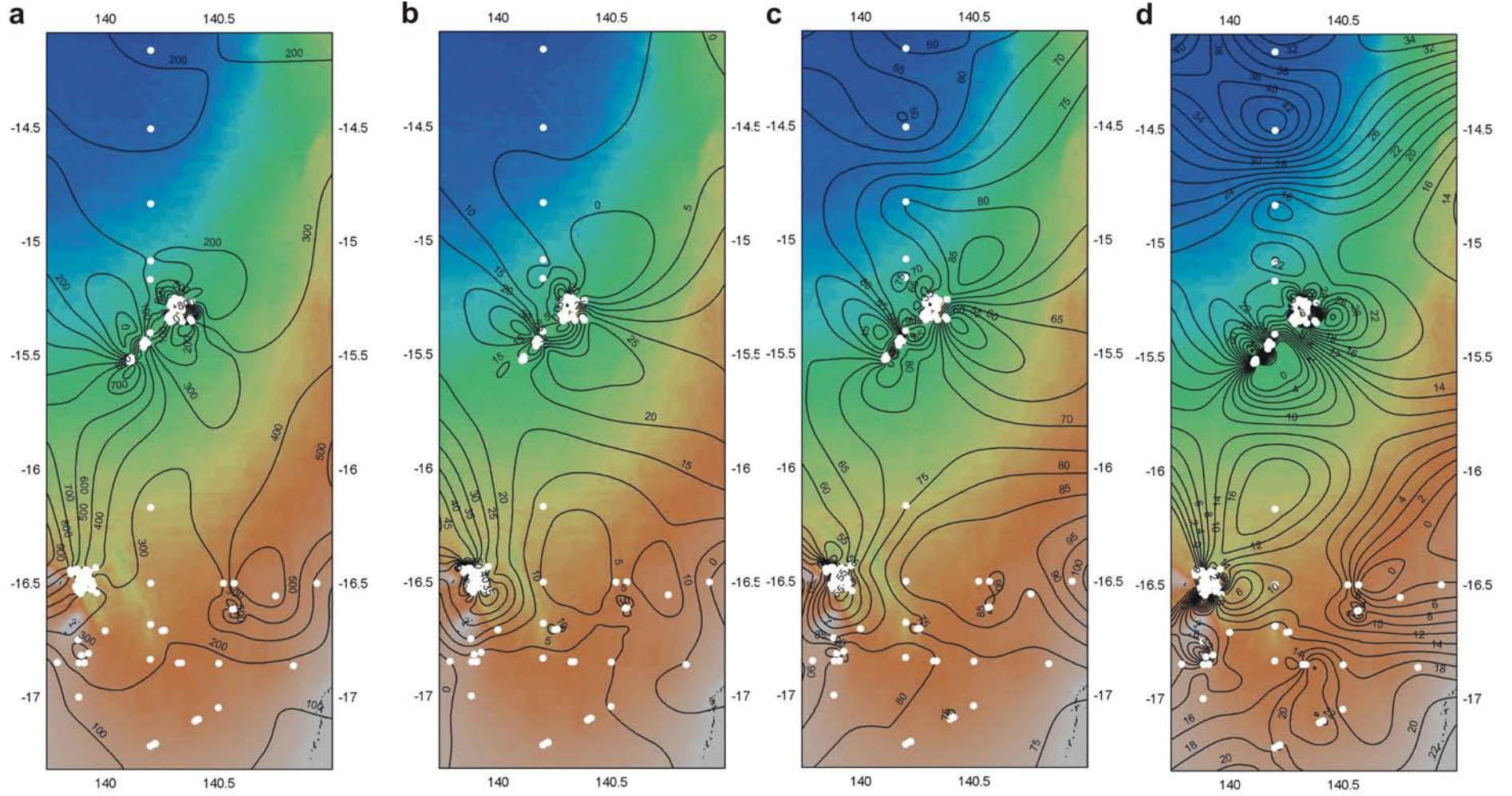
Figure 4.20. Maps showing: a) grain size ( \mu\text{m} ), b) %Gravel, c) %Sand, and d) %Mud from the surface sediments in Area A: Regional survey. Gravel and Sand are the dominant size fractions, with very little mud present. See text for full details. Textural and compositional data for the samples are reported in Appendix G.
