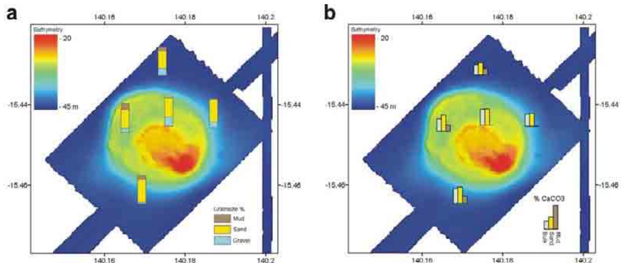
Figure 4.26. Maps showing: a) %Gravel, %Sand and %Mud, and b) %CaCO 3 (Bulk), %CaCO 3 (Sand) and %CaCO 3 (Mud) from samples collected in Area D: Reef R2. Due to the relatively low number of samples the data could not be contoured and are instead shown as bar charts. Sand and gravel are the dominant size fractions, with very little mud present. Carbonate concentrations are greatest on the shallow reef platform and decrease on the gulf floor. See text for full details. Textural and compositional data for the samples are reported in Appendix G .
