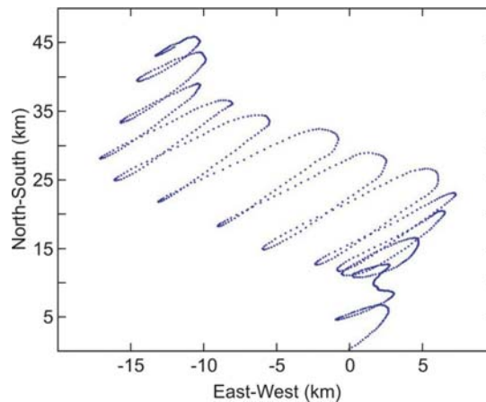
Figure 3.4. Progressive vector plot of tidal excursion recorded during the survey. During the deployment the residual tidal current direction was towards the northwest. Largest excursions were recorded during spring tides in the middle of the record.
