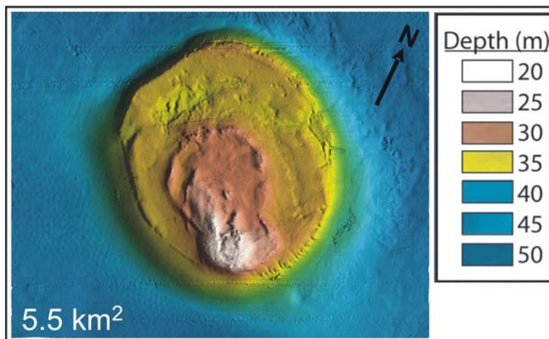
Figure 2.4. Map showing bathymetry derived from multi-beam sonar for Area D: Reef R2. This area consists of a relatively flat seabed surrounding a high-standing oval-shaped platform. The morphology of the platform indicates that is a submerged platform reef. Numerous broad, circular mounds of unknown origin occur to the southwest of the reef.
