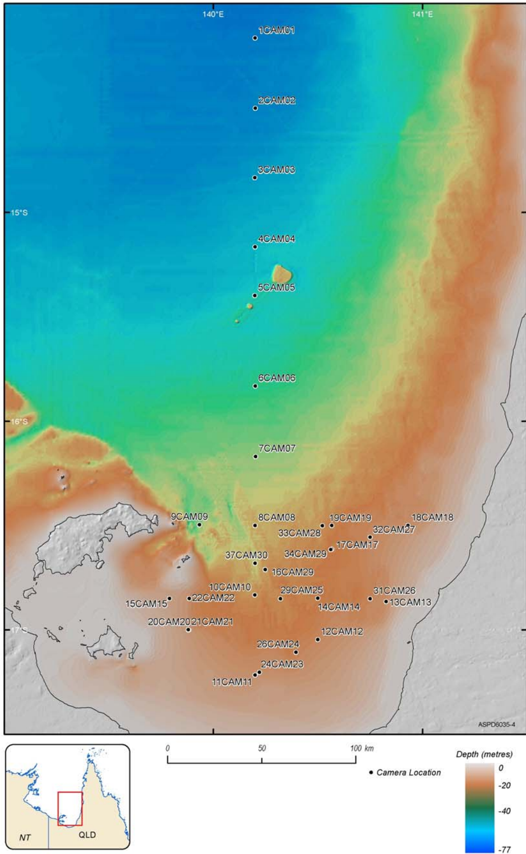
Figure 4.15. Bathymetry map showing location of camera stations occupied in Area A: Regional Survey.
