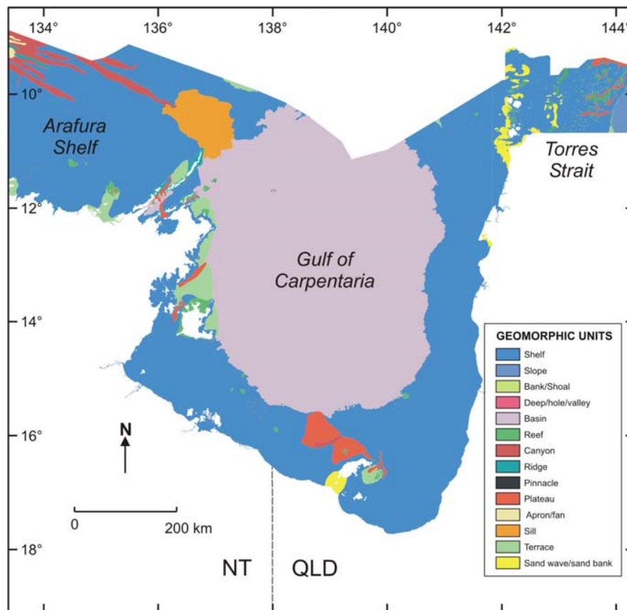
Figure 1.3. Map showing the major geomorphic features in the Gulf of Carpentaria. A total of 12 geomorphic features occur in the gulf, dominated by a broad, low-gradient basin. High standing terraces, plateaus and reef features occur in the southern and western regions of the gulf.
