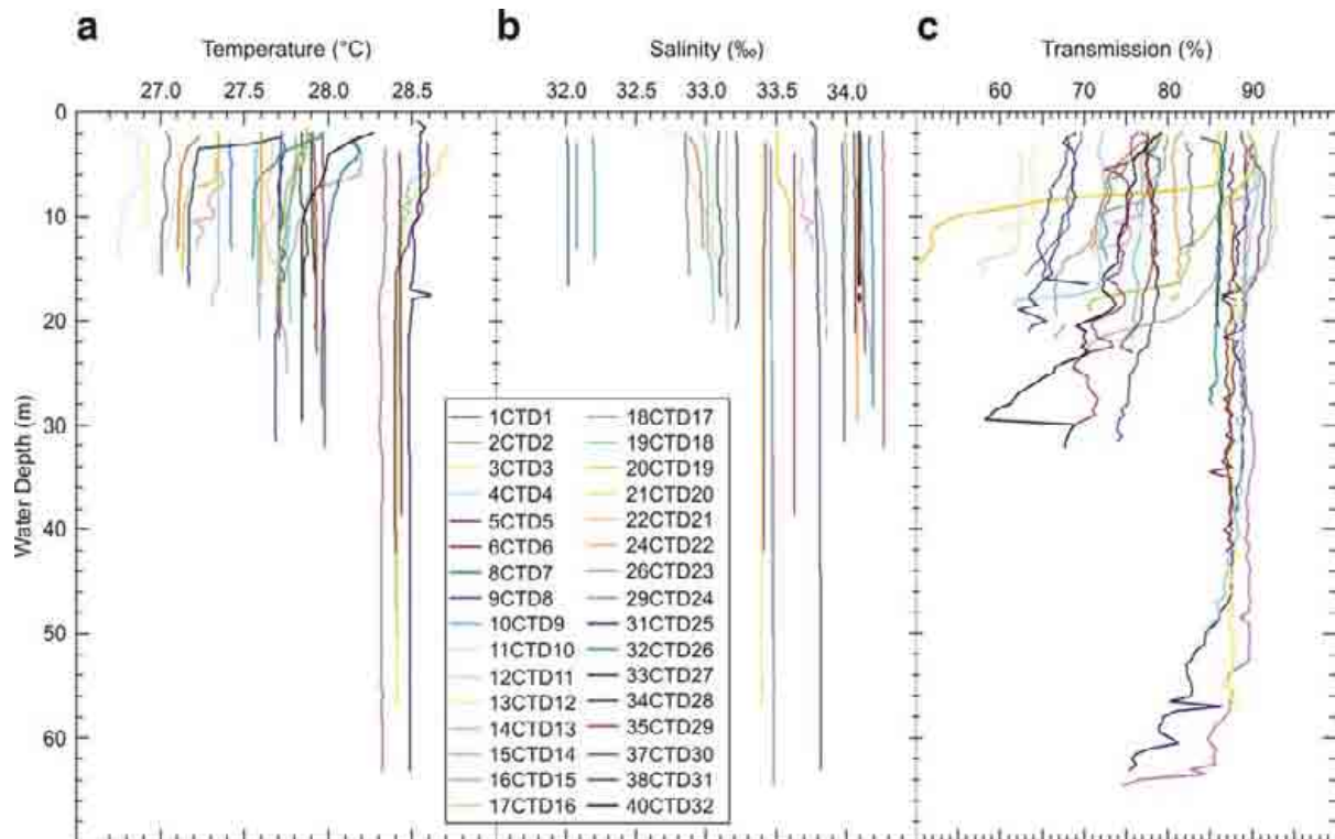
Figure 4.7. Graphs showing: a) temperature ( ^{\circ}\text{C} ), b) salinity ( \text{‰} ), and c) transmission (%) for the waters in Area A: Regional Survey from the CTD casts. A thermocline is evident between 2-5 m depth at some stations (e.g., 8CTD7). Transmission decreases with depth. Otherwise, the data indicate that the waters in Area A are mostly well-mixed and relatively clear.
