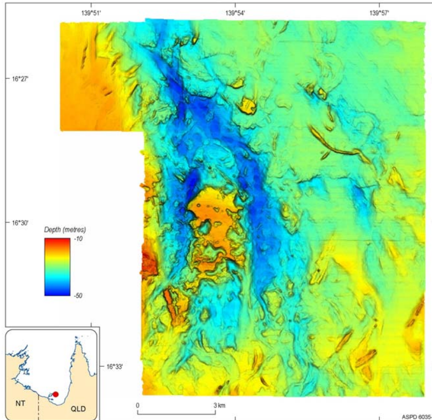
Figure 2.2. Map showing bathymetry derived from multi-beam sonar for Area B: Bryomol Reef. This area consists of a rugged seabed with a high-standing platform. The seabed surrounding the platform is characterised by hard-grounds that form curved and linear ridges up to 2 m high. The morphology of the platform indicates that it has been partially eroded and has a karst-like appearance. Sediment lobes (talus slopes) border the platform margins. Two “blind” depressions >50 m deep occur on either side of the platform.
