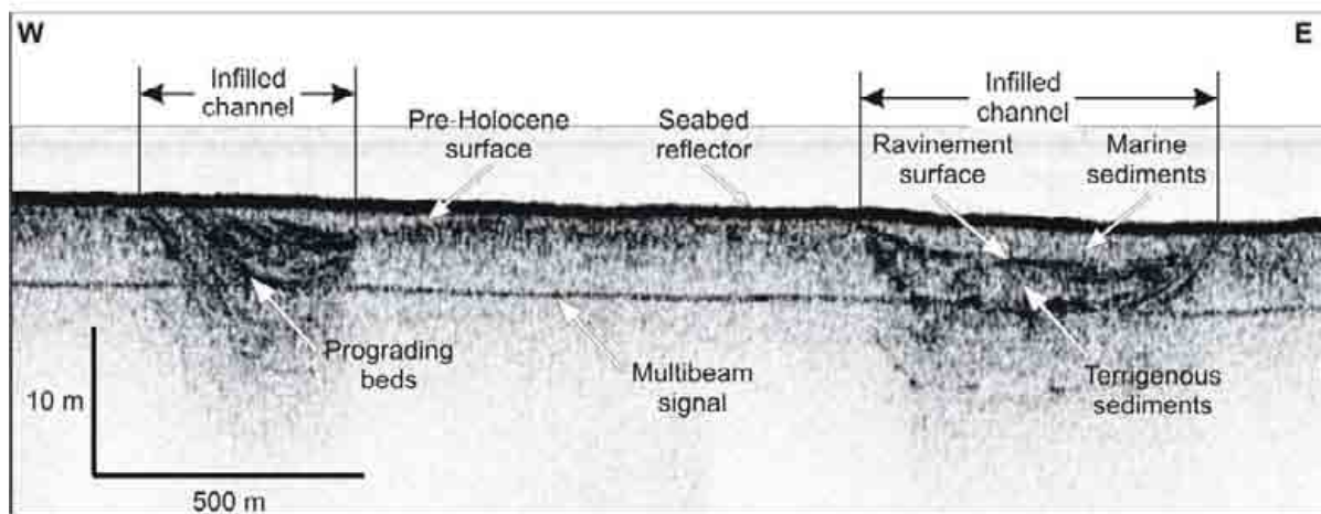
Figure 2.9. Chirp shallow seismic profile showing the typical nature of sub-surface reflections. Sub-surface reflections occur locally and are commonly discontinuous with variable amplitudes. These reflections trace underlying surfaces characterised by variable morphology, which are in contrast to the relatively flat pre-Holocene and seabed reflector. While the origin of these reflections is unknown, they presumably trace the deformed strata of the underlying acoustic basement.
