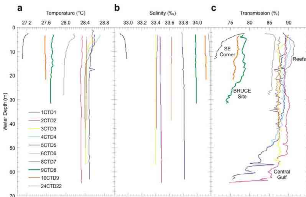
Figure 4.14. Graphs showing: a) temperature, b) salinity, and c) transmission for CTD casts collected from a north-south transect in the southern Gulf of Carpentaria. There are clear differences in the water properties between the relatively deep central Gulf regions and the shallow SE regions. See text for full details and analysis.
