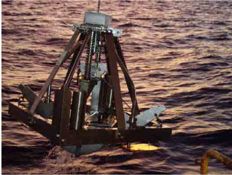
Figure 4.3. Photograph showing Smith-McIntyre grab sampler used on the survey.
