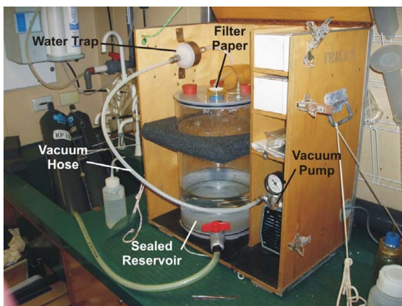
Figure 4.6. Photograph showing Geoscience Australia's purpose-built water filtering system. A total of 1 litre of seawater is filtered through 45 \mu\text{m} mesh filters. The filter papers are then weighed in the laboratory to determine total suspended solids (sediments).
