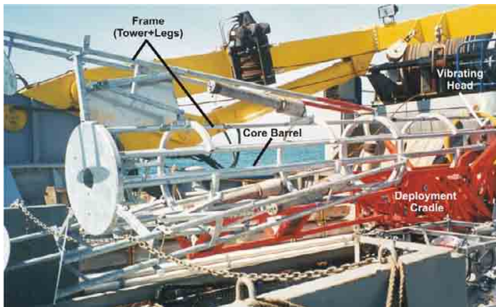
Figure 4.5. Photograph showing the vibrocorer used on the survey. The 6.5 m-long frame is deployed using a hydraulically powered deployment cradle. Power to the vibrating head unit is transmitted down an armoured cable from the vessel.
