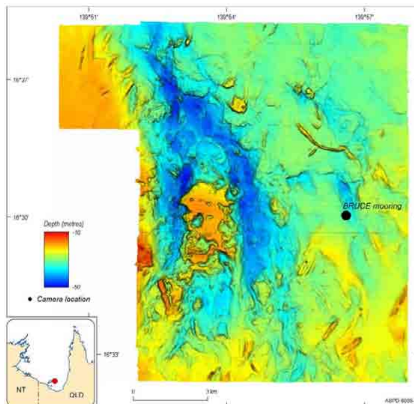
Figure 3.1. Map showing the location of the Benthic Research Underwater sediment Concentration Experiment (BRUCE) oceanographic mooring. BRUCE was deployed on the hard-grounds to the east of the Bryomol Reef in Area B in 34 m water depth. The total length of the deployment was approximately 14 days. BRUCE contains an acoustic current meter, two optical backscatter sensors, an in-situ laser particle sizer, and CTD (conductivity, temperature, depth) probe.
