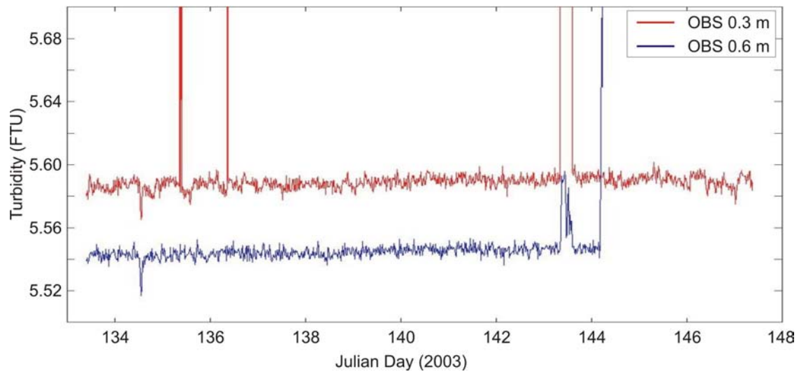
Figure 3.6. Graph showing detailed near-bed turbidity records during the survey. For most of the deployment near-bed turbidity was very low (<5.6 FTU) with daily variations of <0.02 FTU at both 0.3 m and 0.6 m positions. Elevated turbidity is recorded on Julian Day 143 by both sensors.
