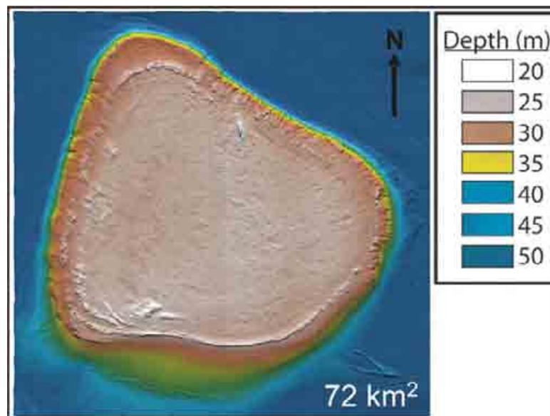
Figure 2.3. Map showing bathymetry derived from multi-beam sonar for Area C: Reef R1. This area consists of a relatively flat seabed surrounding a high-standing irregularly-shaped platform. The morphology of the platform indicates that it is a submerged platform reef.
