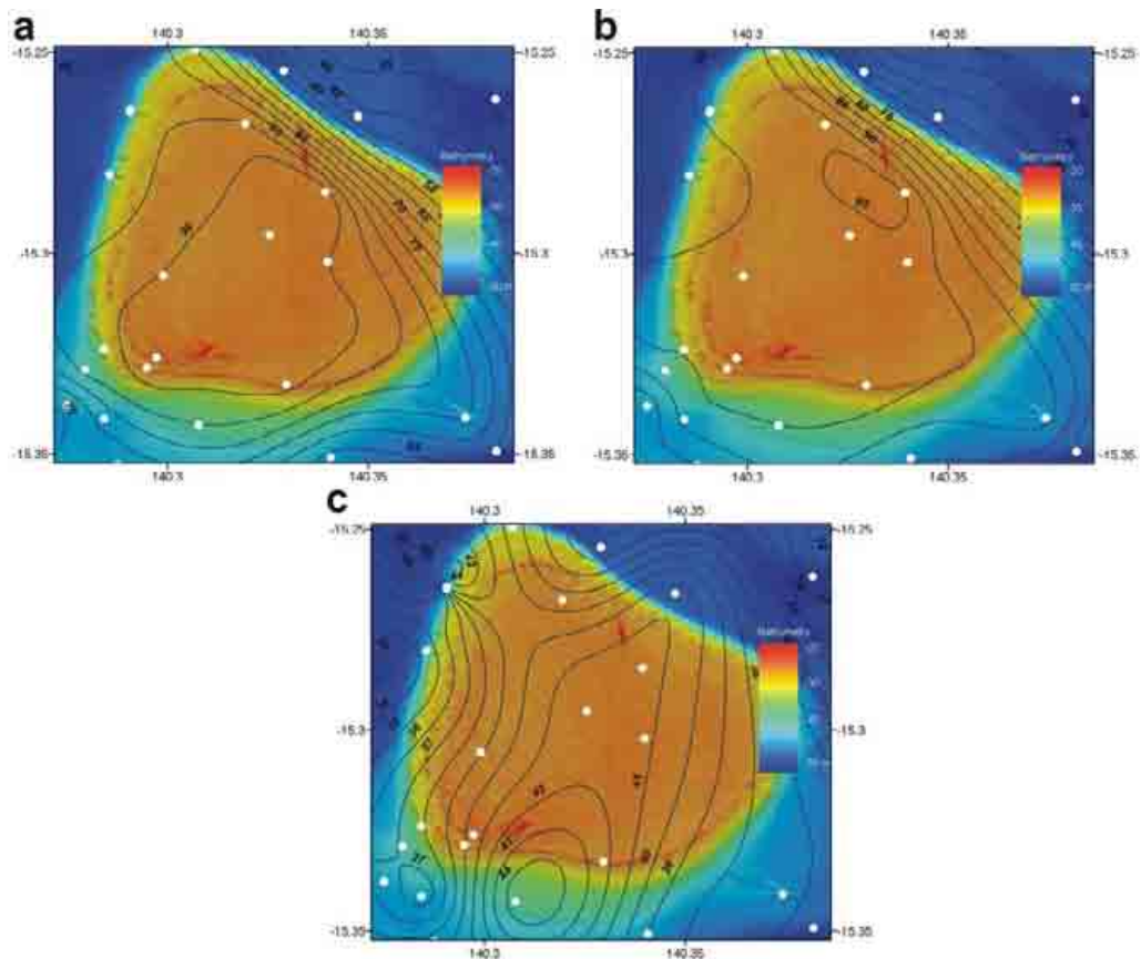
Figure 4.25. Maps showing: a) %CaCO 3 (Bulk), b) %CaCO 3 (Sand), and c) %CaCO 3 (Mud) from the surface sediments in Area C: Reef R1. Carbonate concentrations are greatest on the shallow reef platform and decrease on the gulf floor. See text for full details. Textural and compositional data for the samples are reported in Appendix G .
