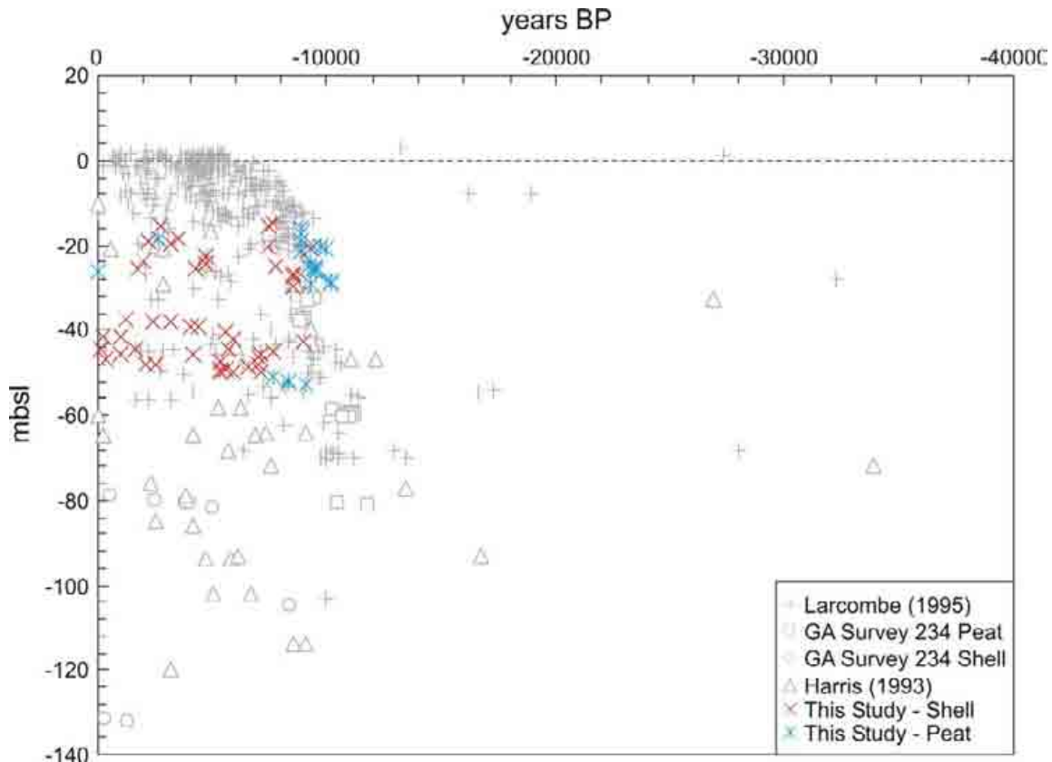
Figure 5.3. Graph of radiocarbon ages <40 kyr BP for samples collected from northeast Australia. Except for two cases, ages from peat samples from this study help to constrain the Holocene sea level curve for the region below -20 m. Ages from shell material from this study are relatively young compared with the curve.
