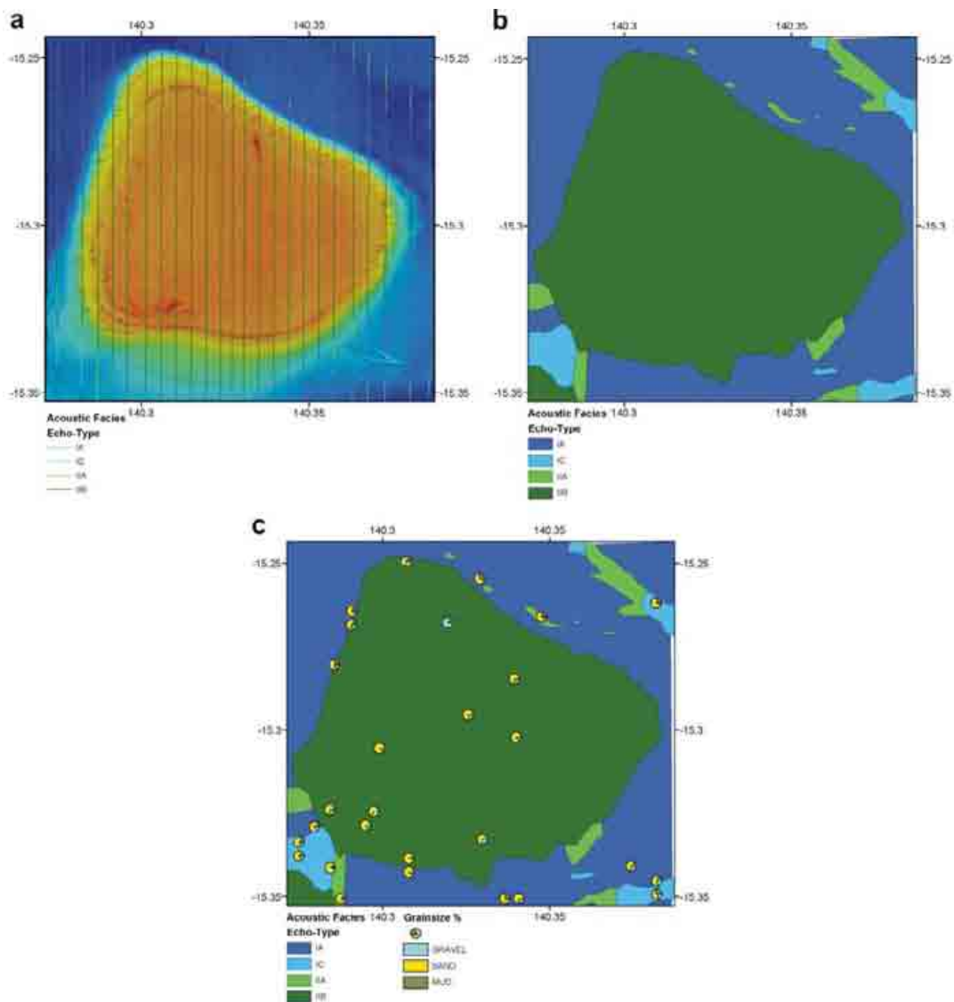
Figure 2.13. Maps showing: a) acoustic facies classification of the seabed from the Chirp sub-bottom profiler records, b) acoustic facies polygons, and c) corresponding textural and composition of seabed sediments. Broadly, echo-type IIA corresponds to sediments with relatively high sand concentrations.
