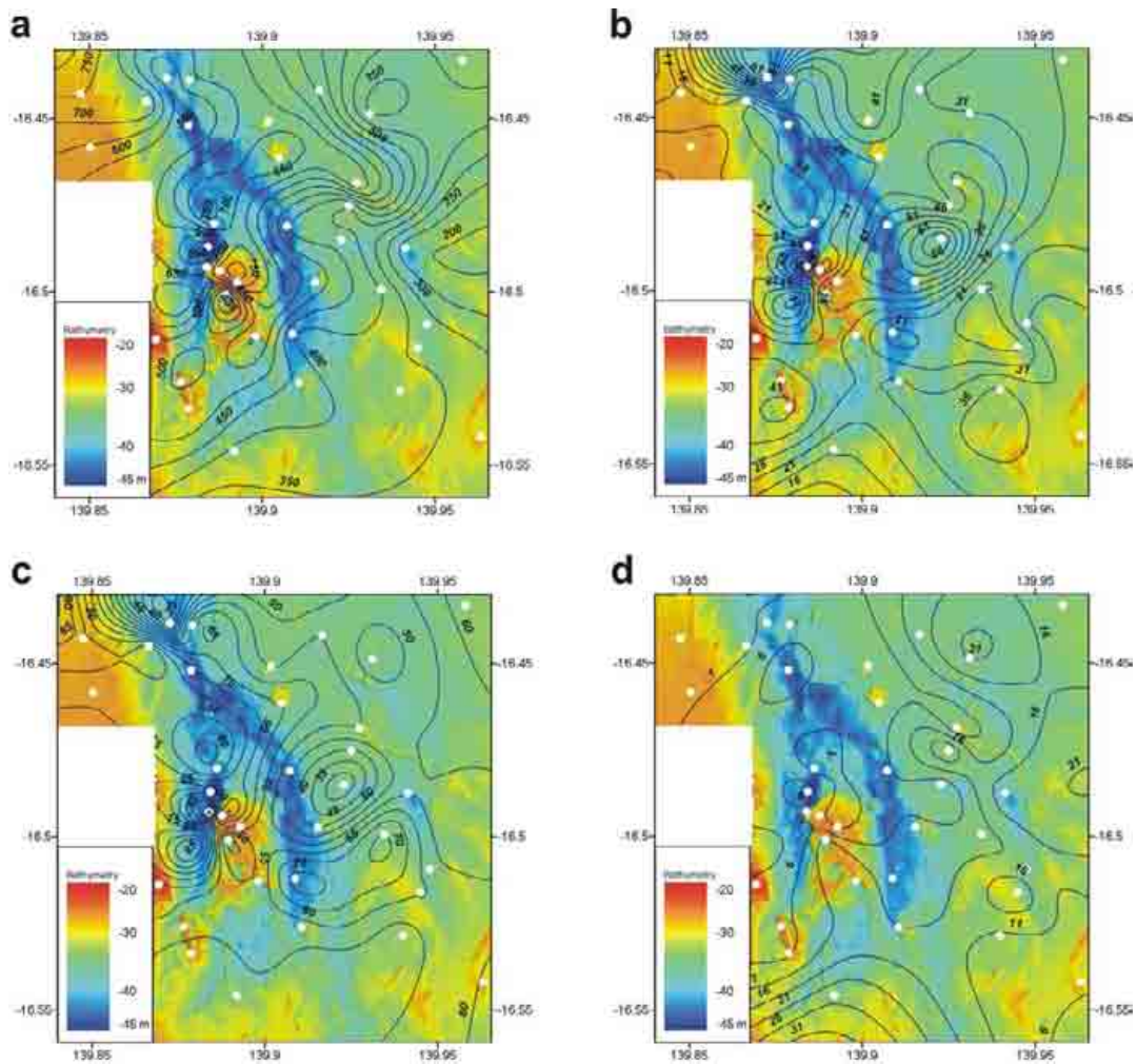
Figure 4.22. Maps showing: a) mean grain size ( \mu\text{m} ), b) %Gravel, c) %Sand, and d) %Mud from the surface sediments in Area B: Bryomol Reef. Sand and gravel are the dominant size fractions, with very little mud present. See text for full details. Textural and compositional data for the samples are reported in Appendix G .
