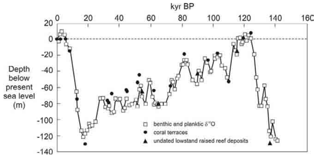
Figure 5.2. Late Quaternary eustatic sea level curve for northeast Australia and PNG derived from coral terraces at Huon Peninsula and benthic and planktic deep sea core \delta^{18}\text{O} data. (Redrawn from Chappell et al., 1996).
