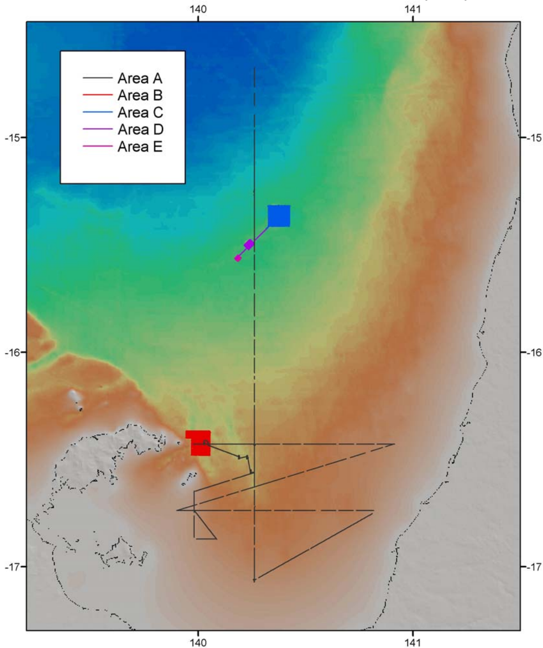
Figure 1.4. Map showing the general survey plan. The long survey lines represent the regional survey (Area A). This survey was designed to provide a regional picture of the seabed sedimentology of the southern Gulf. The smaller surveys (Areas B, C, D, and E) focussed on individual features that were revealed by the regional survey. The sampling programs designed for each of the study areas was tailored to the size and objectives for each area.
