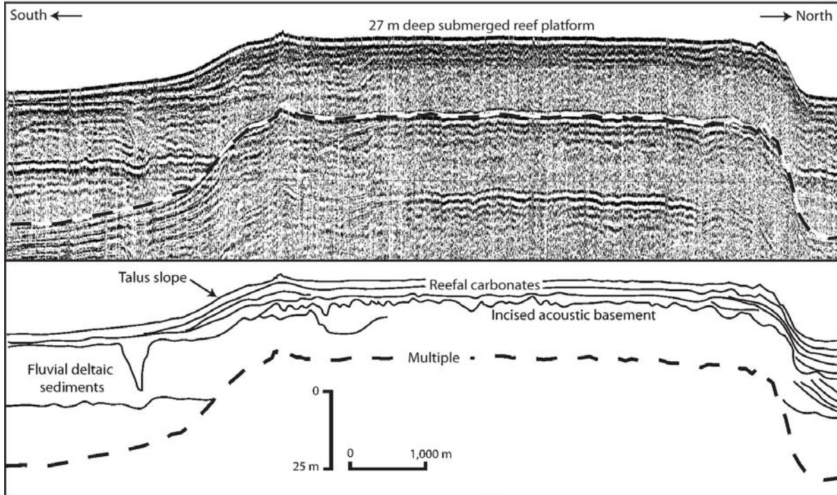
Figure 2.8. Sparker shallow seismic reflection profile over Reef R1 showing reefal carbonates overlying incised acoustic basement having positive relief. The horizontal reflections and talus deposits indicate that reef growth has taken place over numerous sea level cycles.
