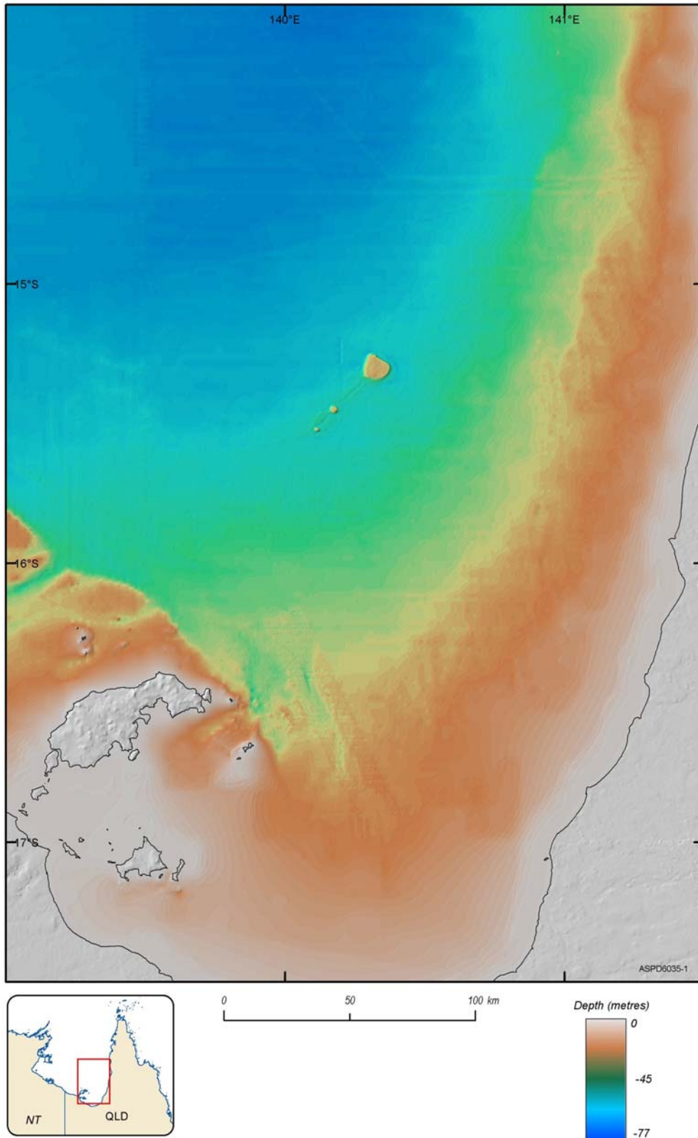
Figure 2.1. Map showing bathymetry derived from multi-beam sonar and Geoscience Australia's 250 m bathymetry grid for Area A: Regional Survey. The southern Gulf of Carpentaria is a shallow tropical shelf environment with a relatively flat and sedimented seabed. The seabed inclines gently towards the margins and water depths range from 70 m in the north of the study area to <20 m in the south and east. Three high-standing carbonate platforms occur in the north of the study area. The platforms rise from >45 m water depth to within 20 m of the water surface.
