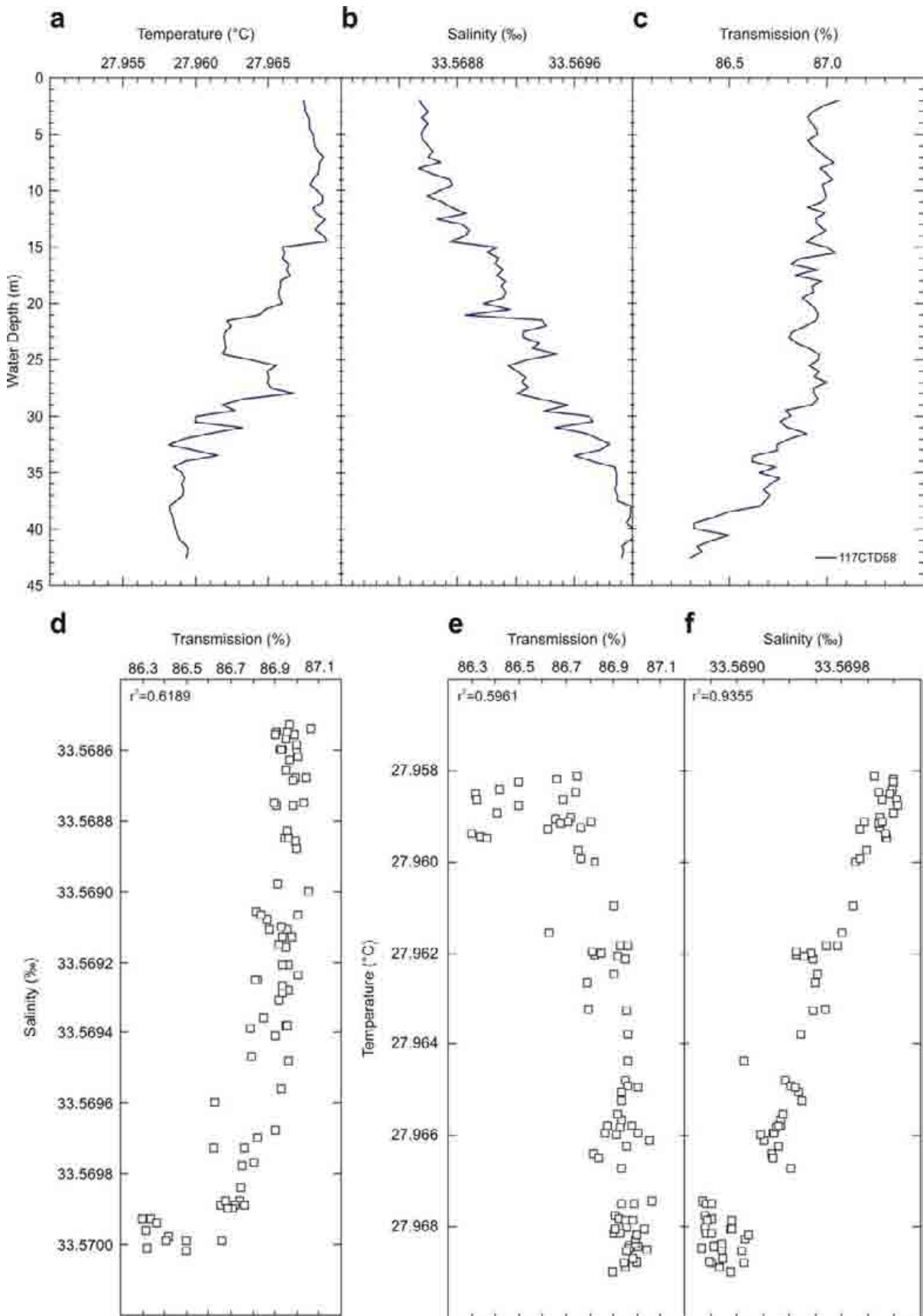
Figure 4.13. Graphs showing: a) temperature (°C), b) salinity (‰), c) transmission, d) salinity v transmission, e) temperature v transmission, and e) temperature v salinity for the CTD cast taken in Area D: Reef R2. The data indicate that the water near the reef is relatively well mixed and clear. There is a strong inverse relationship between temperature and salinity, positive relationship between temperature and transmission, and an inverse relationship between salinity and transmission.
