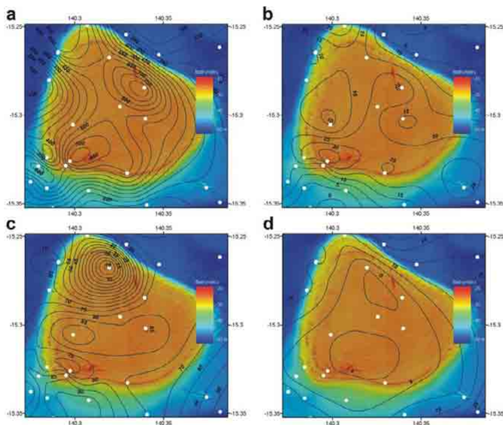
Figure 4.24. Maps showing: a) mean grain size ( \mu\text{m} ), b) %Gravel, c) %Sand, and d) %Mud from the surface sediments in Area C: Reef R1. Sand and gravel are the dominant size fractions, with very little mud present. See text for full details. Textural and compositional data for the samples are reported in Appendix G .
