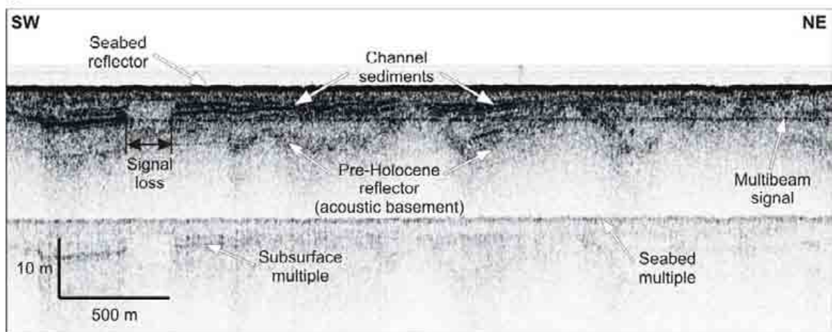
Figure 2.10. Chirp shallow seismic profiles showing: a) infilled channels, and b) infilled depressions of the pre-Holocene surface. The channels are the most numerous sub-surface features observed in the shallow seismic profiles; however they could not be traced across the study area. Channel (fluvial-deltaic) sediments have also infilled depressions of the underlying acoustic basement. These well-bedded deposits have been preserved in the depressions. A wave- or tidal-ravinement surface occurs at the top of these fluvial-deltaic sequences and separates them from the overlying marine (shallow shelf) sequence.
