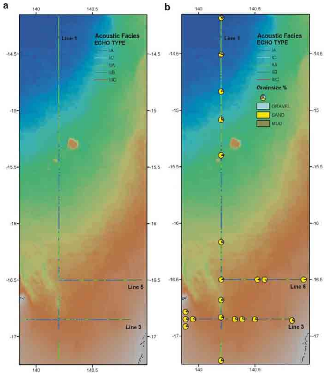
Figure 2.11. Maps showing: a) acoustic facies classification of the seabed from the Chirp sub-bottom profiler records, and b) corresponding texture and composition of seabed sediments. Broadly, major changes in echo-type do not correspond to changes in the texture and composition of the seabed.
