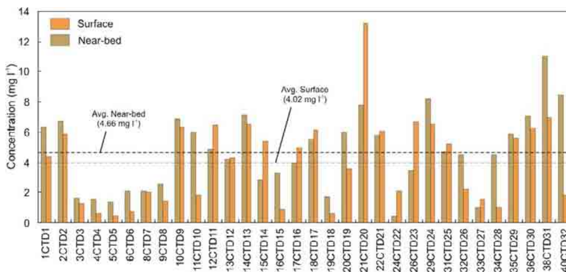
Figure 4.8. Graph showing near-bed and surface suspended sediment concentrations from Area A: Regional Survey. Near-bed concentrations are slightly higher than surface concentrations. However, this difference is not statistically significant.
