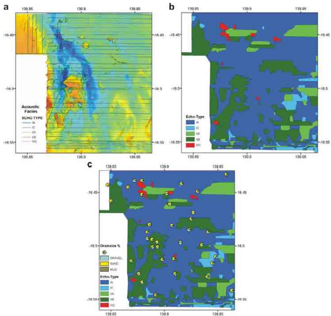
Figure 2.12. Maps showing: a) acoustic facies classification of the seabed from the Chirp sub-bottom profiler records, b) acoustic facies polygons, and c) corresponding textural and composition of seabed sediments. Broadly, major changes in echo-type do not correspond to changes in the texture and composition of the seabed.
