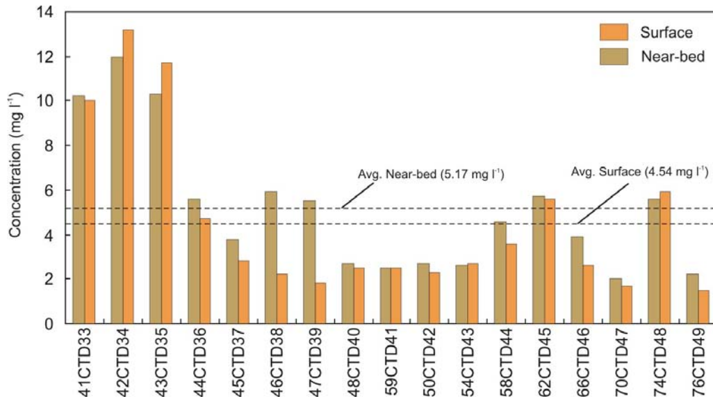
Figure 4.10. Graph showing near-bed and surface suspended sediment concentrations from Area B: Bryomol Reef. Near-bed concentrations are slightly higher than surface concentrations. However, this difference is not statistically significant.
