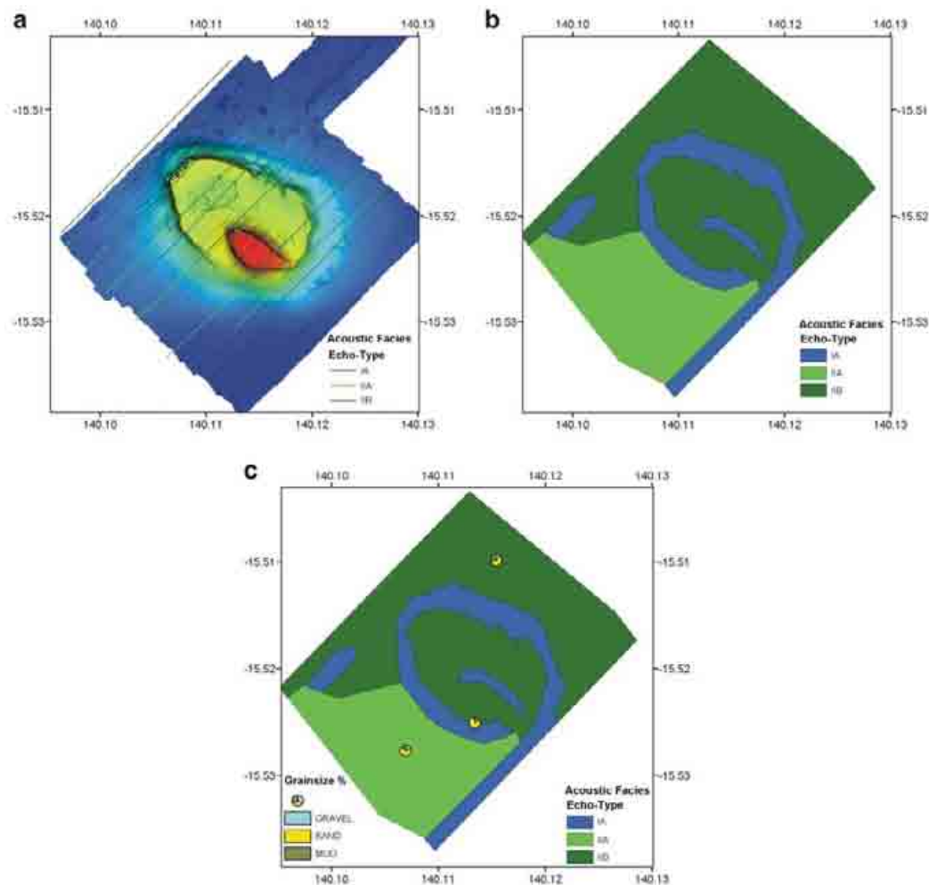
Figure 2.15. Maps showing: a) acoustic facies classification of the seabed from the Chirp sub-bottom profiler records, b) acoustic facies polygons, and c) corresponding textural and composition of seabed sediments. Despite the small number of samples, echo-type IA corresponds gravely sand and echo-types IIA and IIB correspond to muddy gravely sand.
