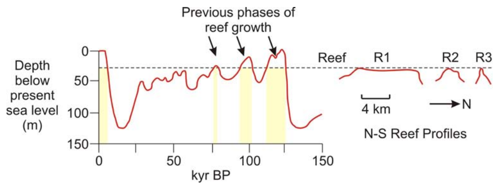
Figure 5.5. Sea level curve for the past 150,000 years (after Chappell et al., 1996) showing the times when the reefs in the southern Gulf of Carpentaria were submerged. Reef growth and main deposition of the reefs probably occurred during the three highstands between 110-125 kyr BP, 90-102 kyr BP, and 76-80 kyr BP.
