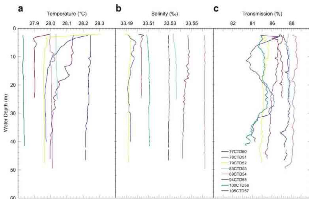
Figure 4.11. Graphs showing: a) temperature ( ^{\circ}\text{C} ), b) salinity ( \text{‰} ), and c) transmission (%) for the waters in Area C: Reef R1 from the CTD casts. There is a slight decrease in transmission with water depth. Otherwise, the data indicate that the waters in Area B are mostly well-mixed and relatively clear. Transmission in Area C is the highest for all study areas.
