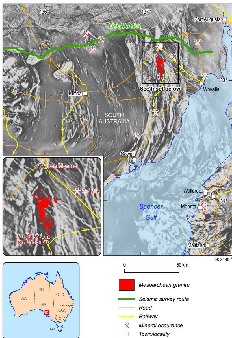
Figure 1. Magnetic image of the northeastern Eyre Peninsula showing the trace of the recently collected seismic line (bold green line), and the location of Mesoarchean granite (highlighted in red) between the Iron Monarch and Iron Baron mines (inset).
