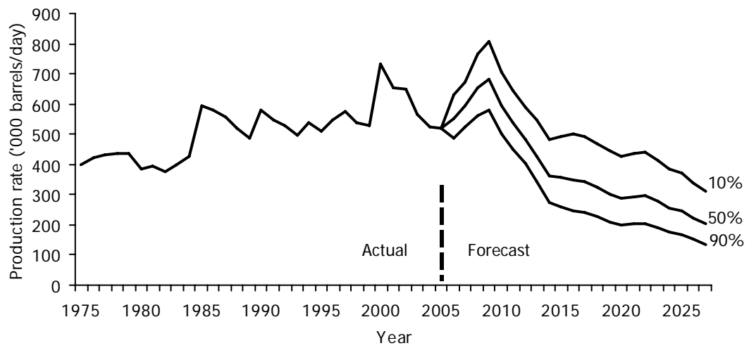
Production Figure 1 Australia's annual production of crude oil and condensate 1975–2005 and forecast annual production at 90%, 50% and 10% cumulative probability 2006–2025
