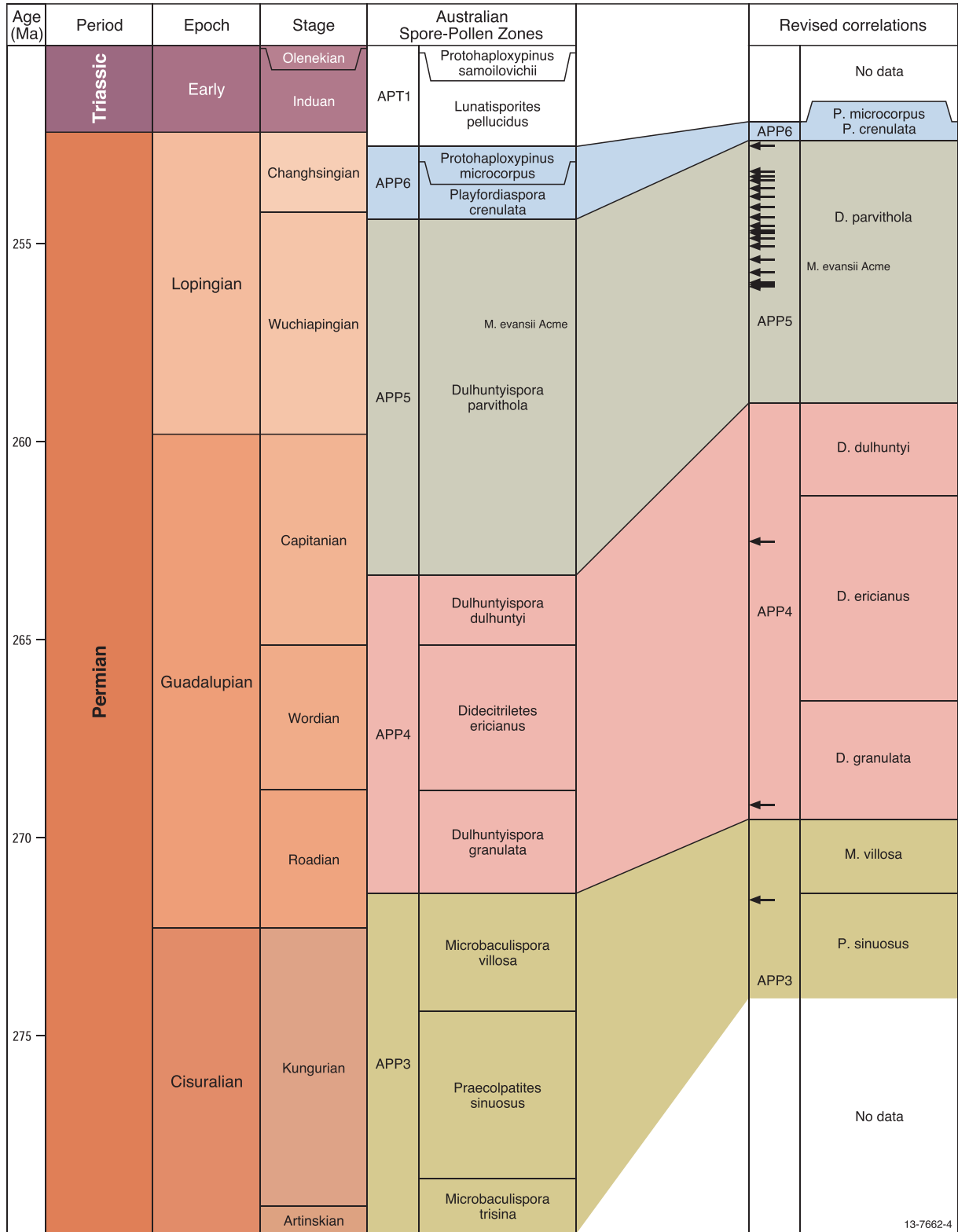
Figure 4: Revised calibration of the palynostratigraphic scheme for part of the Australian Permian based on CA IDTIMS dates (black arrows). Left: the standard chronostratigraphy of Gradstein et al. (2012). Centre: the most recent correlation based on Mantle et al. (2010) updated to The Geologic Time Scale 2012. Right: a new correlation based on CA IDTIMS dating of palynostratigraphically controlled tuffs.
