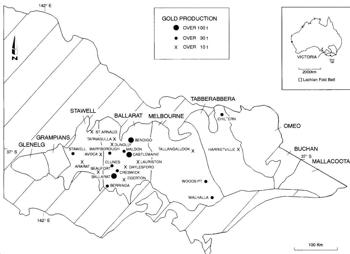
Figure 1. Victorian gold province, showing outcrop of the Palaeozoic succession and the separate geological zones. The zones are based primarily on age, lithology, metamorphism and deformational history. Goldfields over 10 t production are confined to west of the Omeo zone and east of the Grampians subzone of the Glenelg zone. The Palaeozoic succession is overlain by sediments of the Murray Basin to the north, and Cainozoic basalts and sediments to the south.
