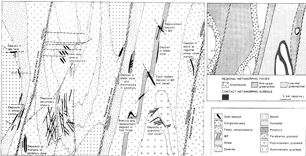
Figure 3. Schematic representation of the nature of Archaean lode-Au mineralisation, illustrating variable structural styles, host rocks and metamorphic settings (from Groves et al. 1990).
