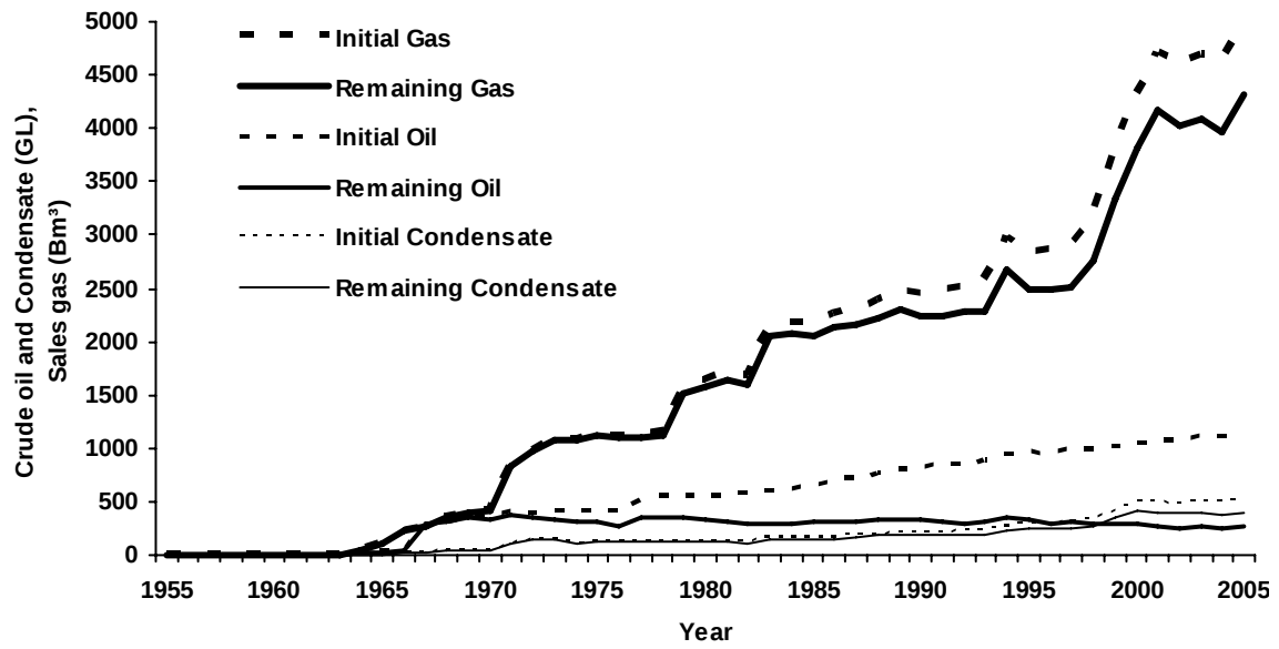
Reserves Figure 2 Australia's initial and remaining commercial plus non-commercial reserves of crude oil, condensate and sales gas
