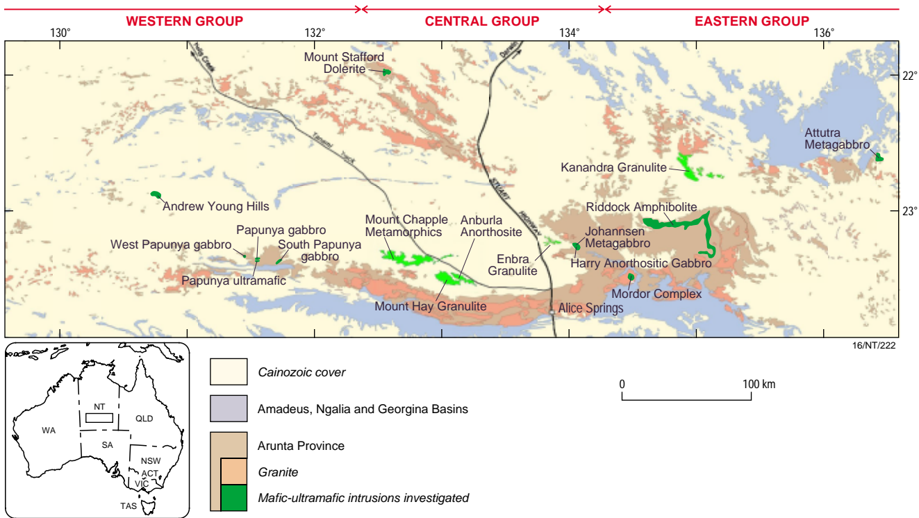
Figure 1. Mafic-ultramafic intrusions investigated in the Arunta Province.
