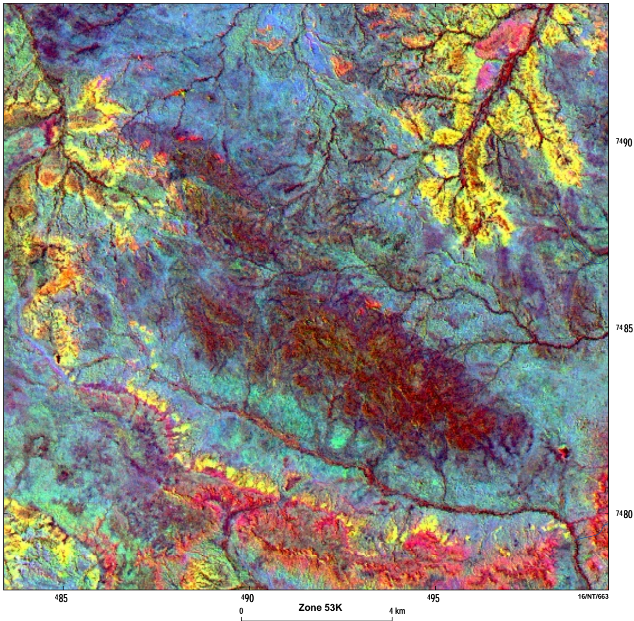
Figure 23. Landsat-5 Thematic Mapper spectrally-enhanced colour image of the Kanandra Granulite displaying ‘clays’ (red), ‘iron oxides’ (green) and ‘silica’ (blue). The area shown is the same as that for the geological map of Figure 22.
