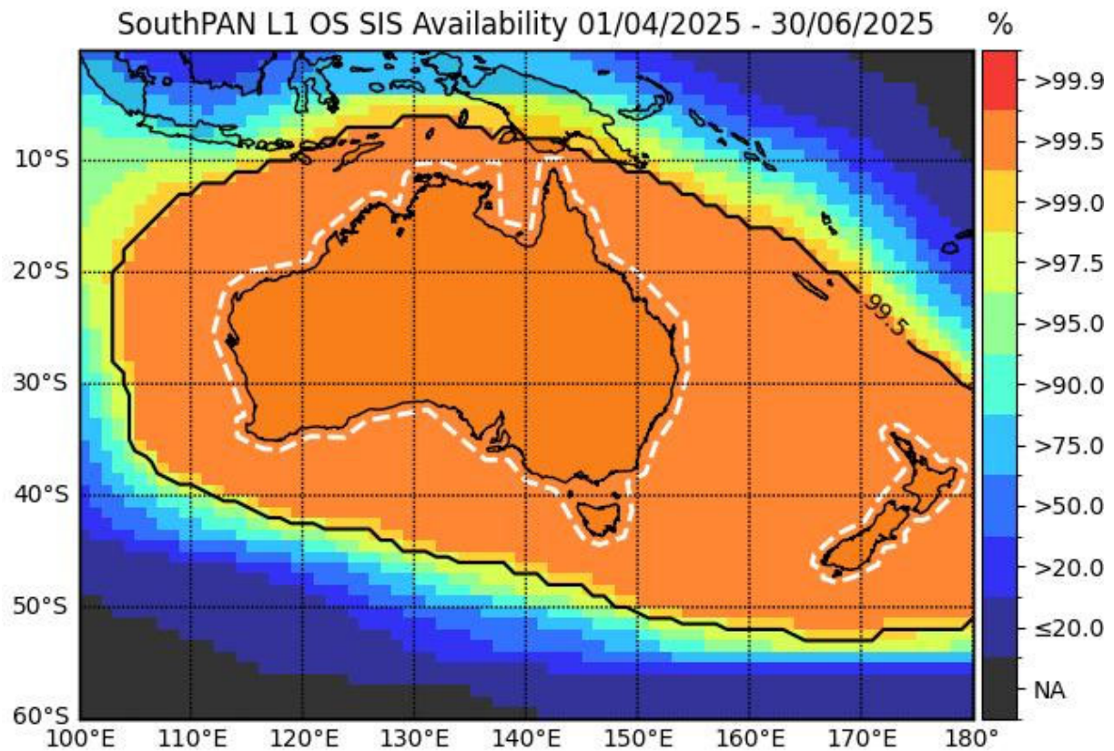
Figure 5: OS-L1-SIS availability (01/04/2025 - 30/06/2025). The solid black line is the 99.5% availability contour and the dashed white line is the OS-L1 service volume.
