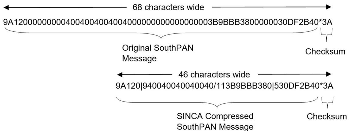
Figure 12: Example of SINCA Compression
