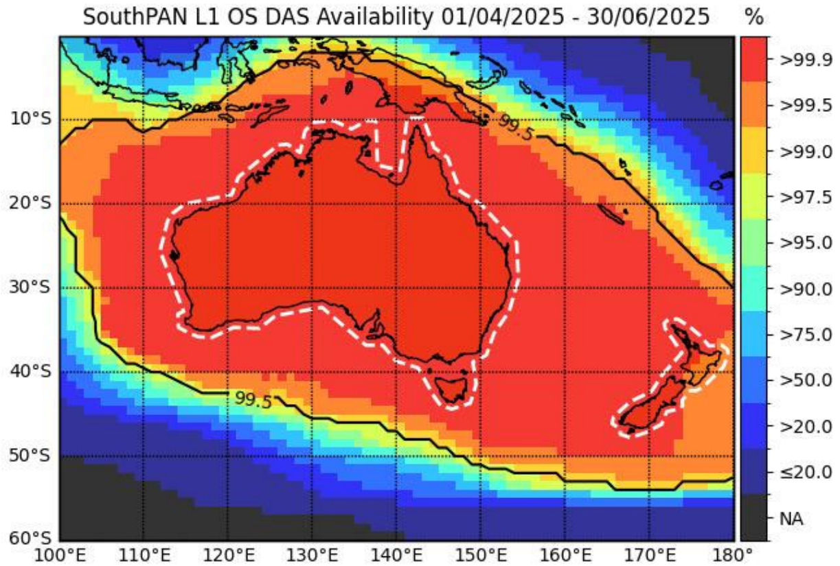
Figure 9: OS-L1-DAS availability (01/04/2025 - 30/06/2025). The solid black line is the 99.5% availability contour and the dashed white line is the OS-L1 service volume.
