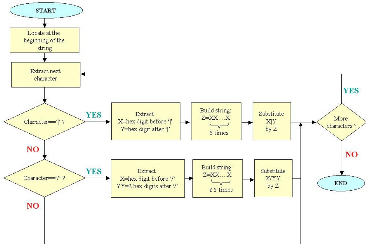
Figure 13: SINCA Decompression Algorithm
