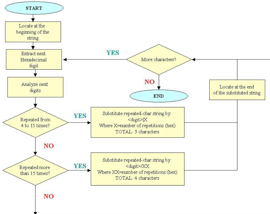
Figure 11: SINCA Compression Algorithm
