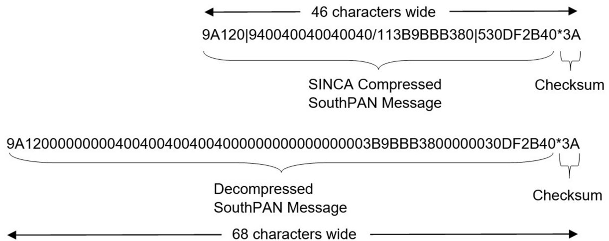
Figure 14: Example of SINCA Decompression
