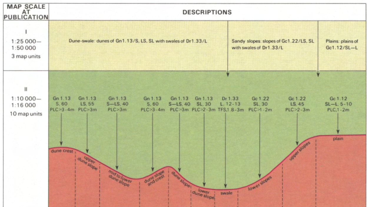
Figure 8. Diagrammatic Cross-section of Soil-landscapes. Based on Northcote (1951) for an area near Coomealla, N.S.W. (upstream on Murray River from Wentworth), and expressed in terms of the Factual Key for the Recognition of Australian Soils.
